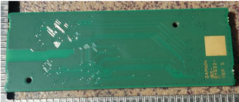
ICB-C Board Bottom (All Models)
