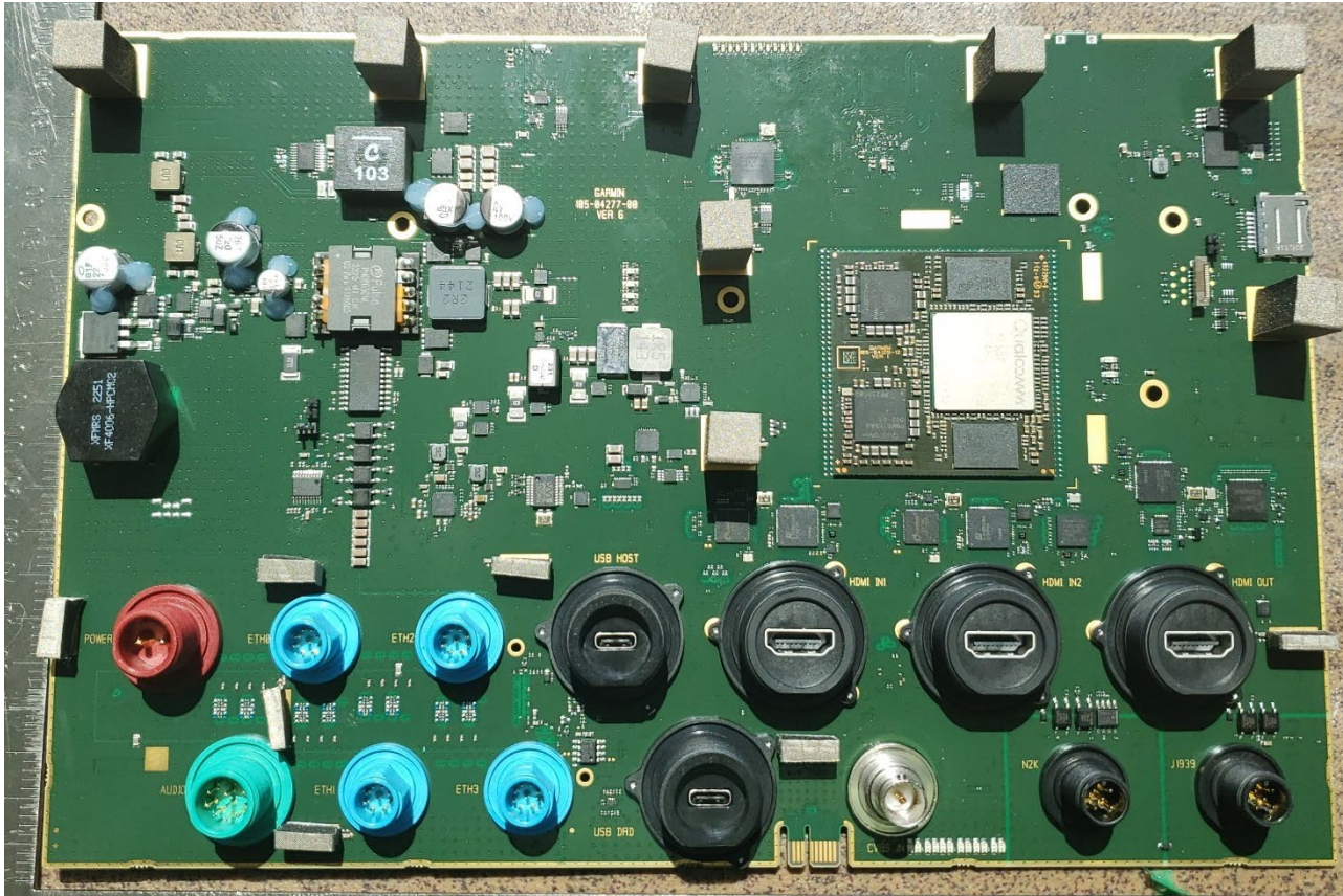
Main Digital Board Front (All Models)
