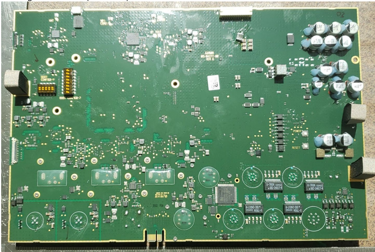
Main digital Board Back (All Models)
