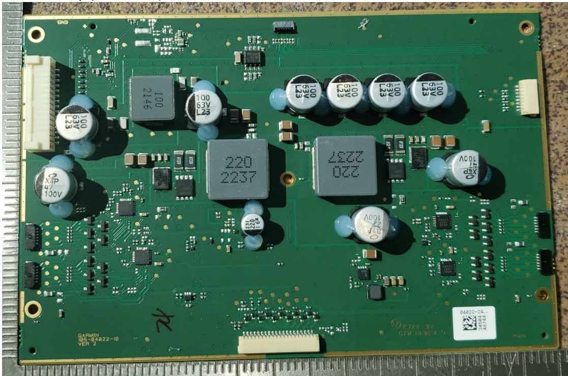
ICB Board Top (All Models)
