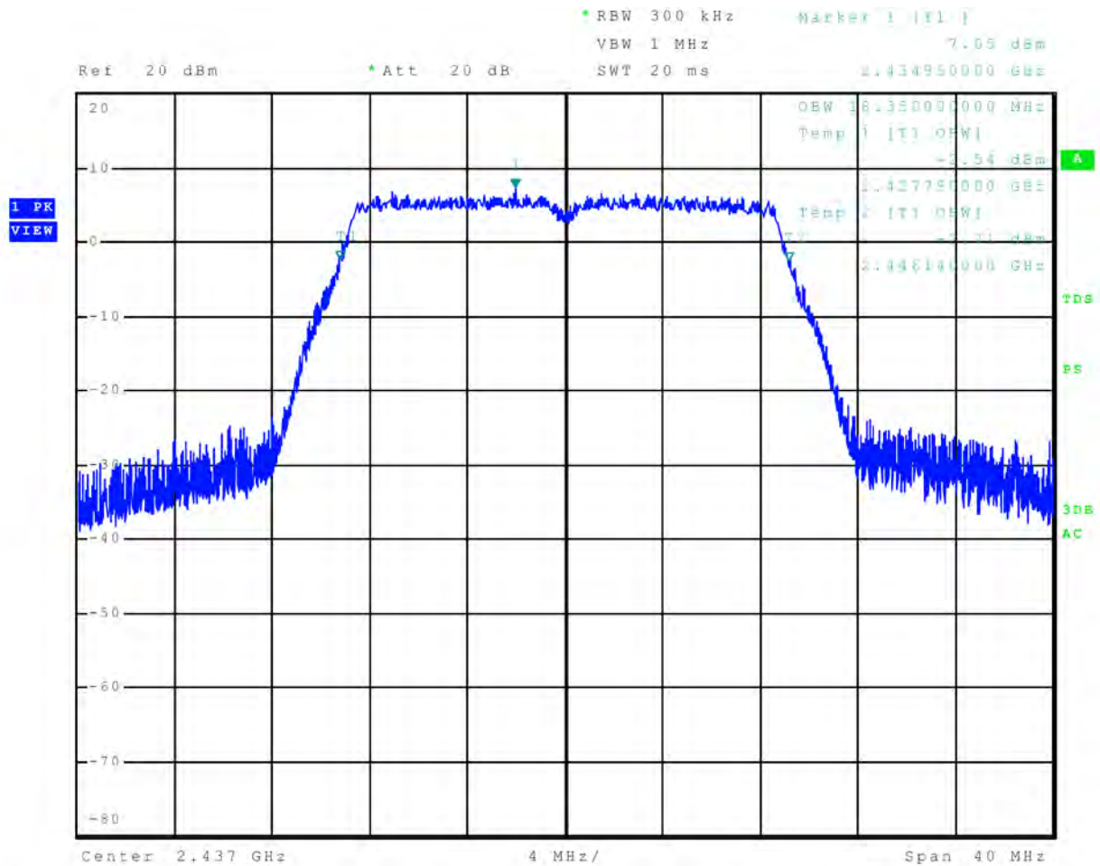
Figure 30 Plot of 99% Occupied Bandwidth Mode 8, 802.11n (MSC)
