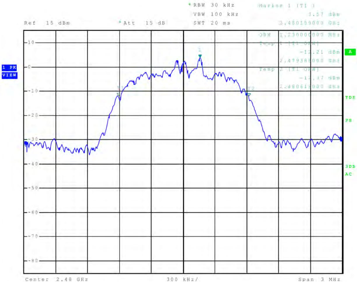
Figure 22 Plot of 99% Occupied Bandwidth Mode 4, BT 3EDR (8DPSK)
