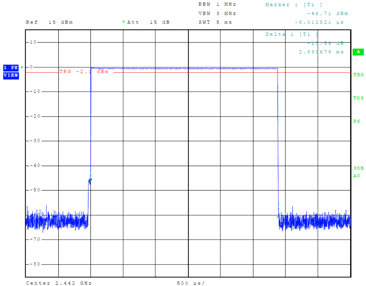
Figure 11 Plot of Dwell time On Channel Mode 1, BT BR
