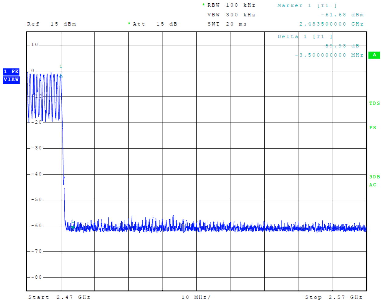
Figure 14 Plot of Transmitter Emissions High Band Edge Mode 1, BT BR
