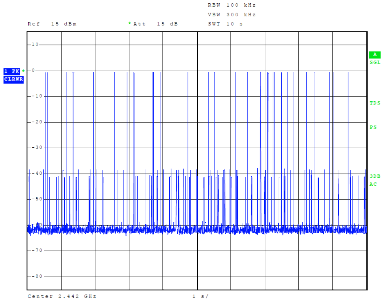
Figure 12 Plot of Number of Times on Channel over 10 Second Period Mode 1, BT BR
