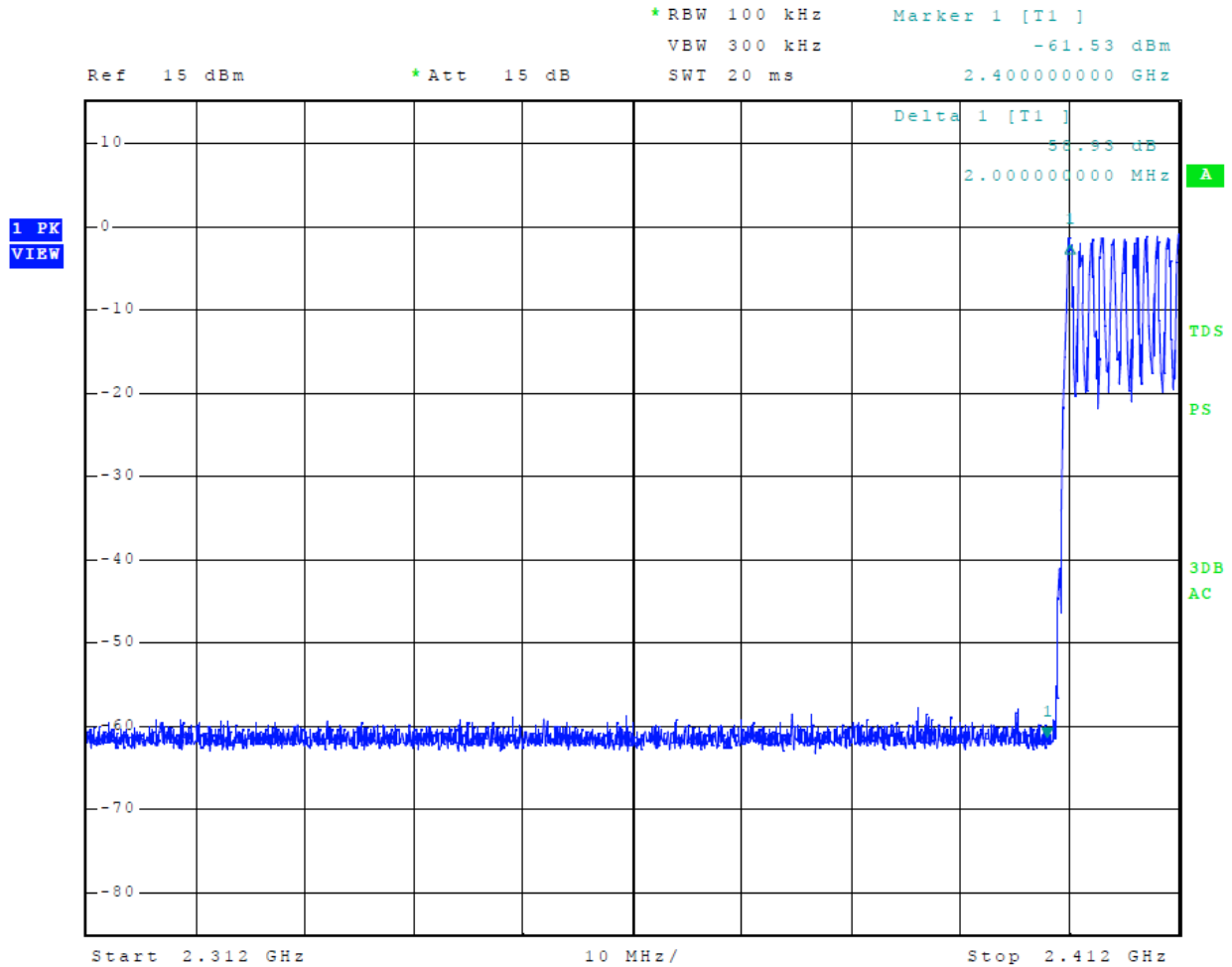
Figure 13 Plot of Transmitter Emissions Low Band Edge Mode 1, BT BR
