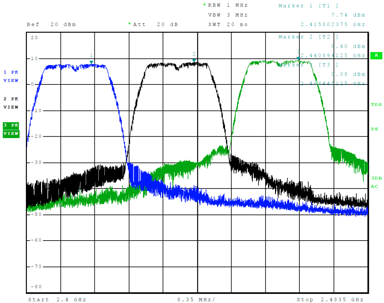
Figure 7 Plot of Transmitter Operation in 2402-2480 MHz Mode 6, Radio 1, 802.11g
