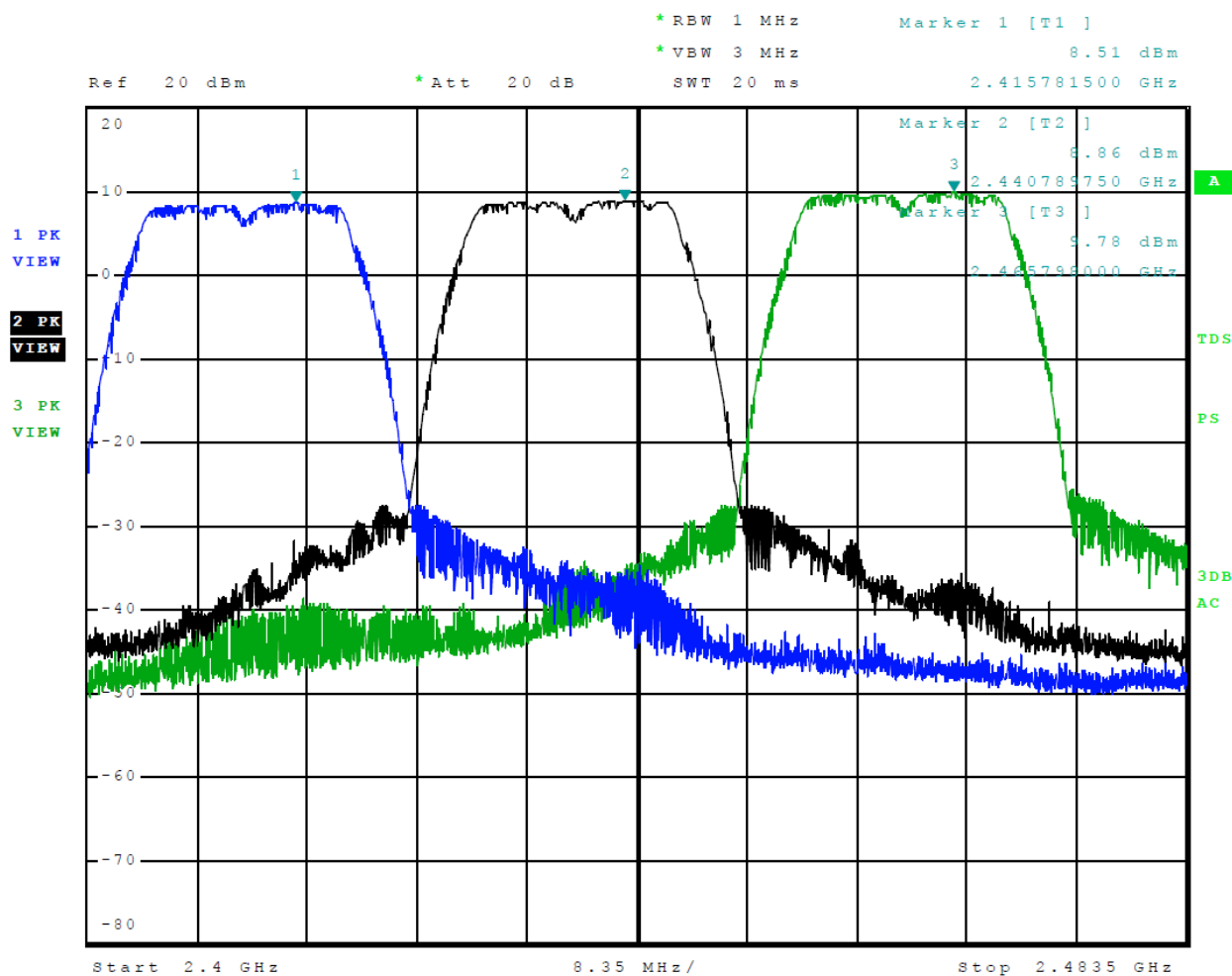
Figure 10 Plot of Transmitter Operation in 2402-2480 MHz Mode 15, Radio 2, 802.11g
