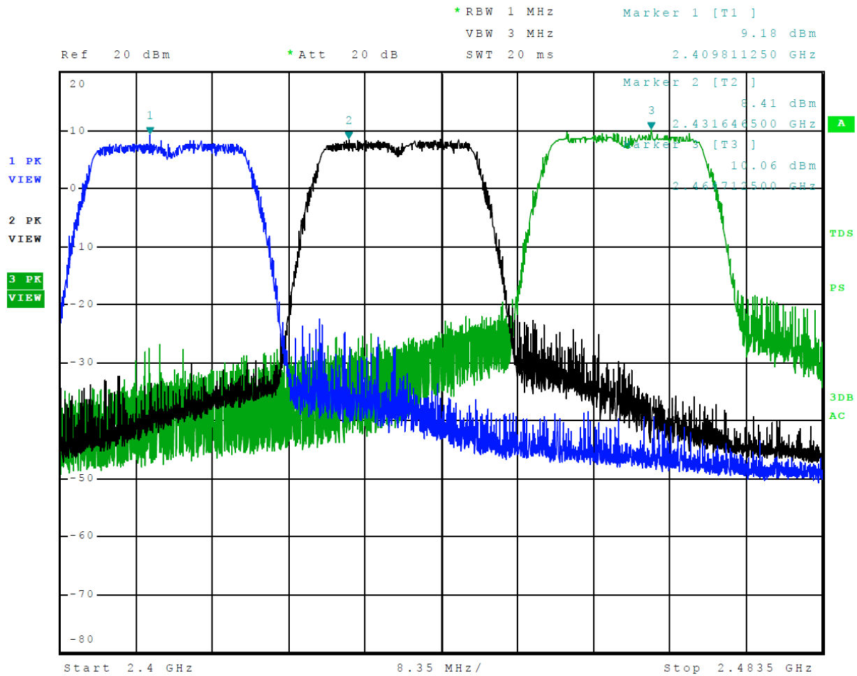
Figure 8 Plot of Transmitter Operation in 2402-2480 MHz Mode 7, Radio 1, 802.11n
