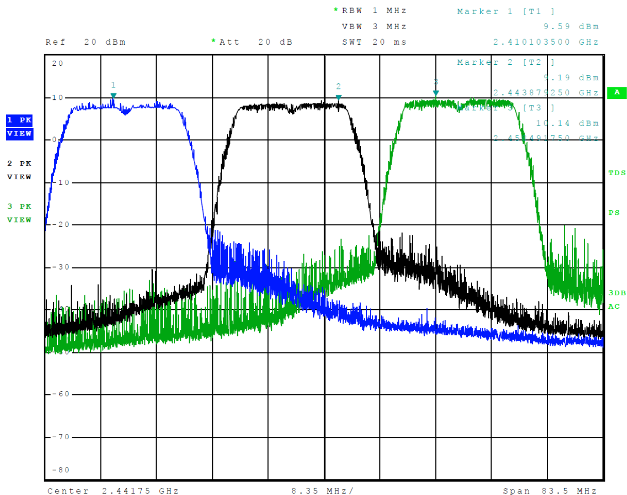
Figure 11 Plot of Transmitter Operation in 2402-2480 MHz Mode 16, Radio 2, 802.11n
