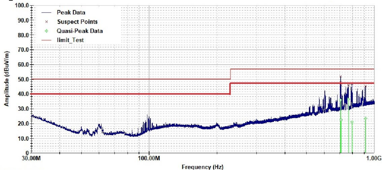
Figure 2 Plot of General Radiated Emissions – Vertical Polarization
