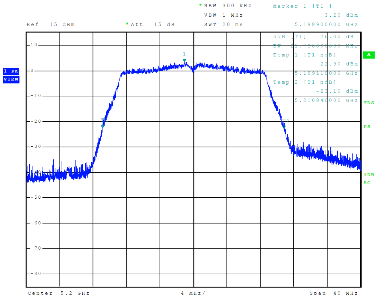
Figure 47 Plot of 26-dB Occupied Bandwidth 5150-5250 MHz Radio 2, Mode 20 U-NII-1 (802.11ac20)
