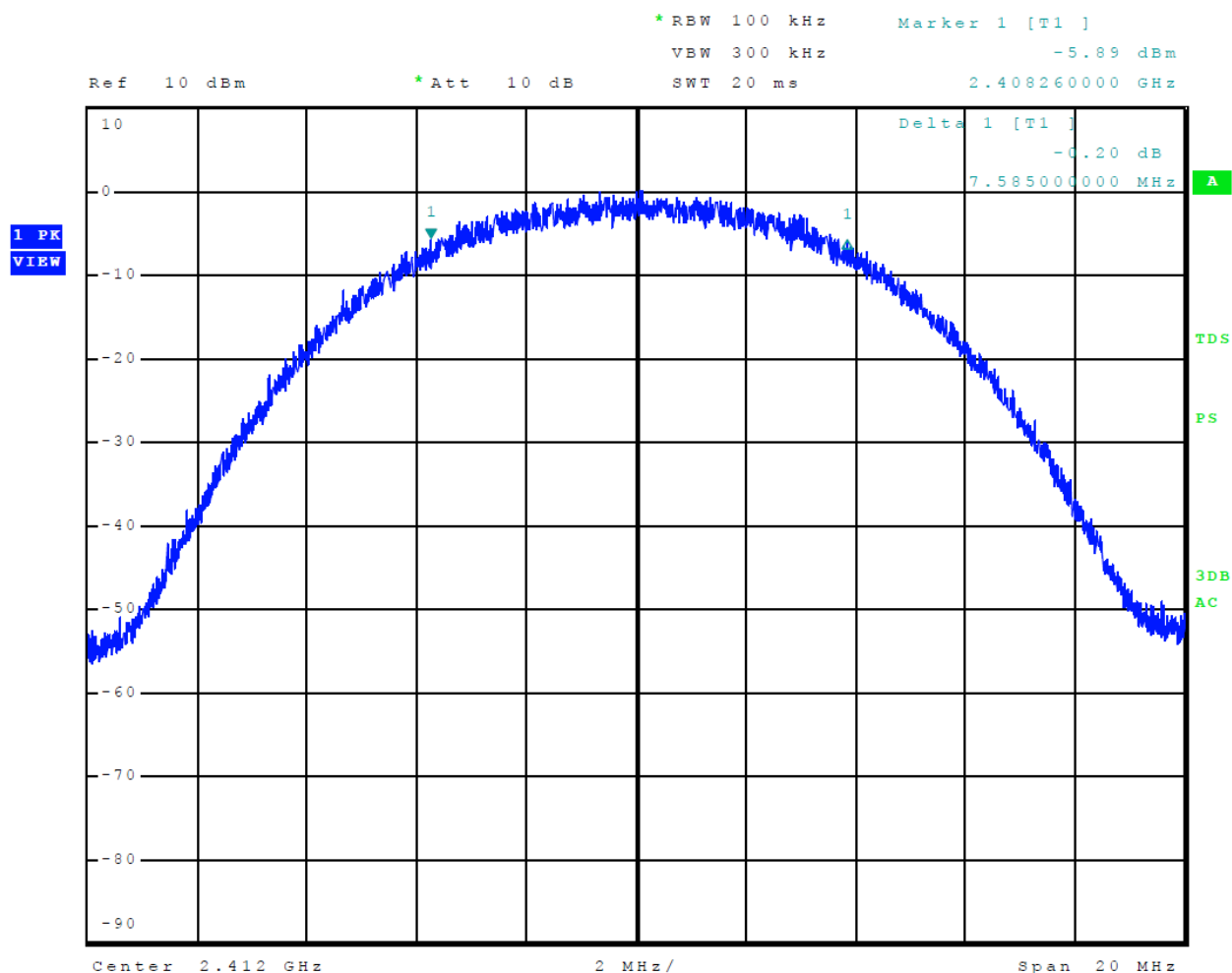
Figure 42 Plot of 6-dB Occupied Bandwidth Mode 14, Radio 2, 802.11b
