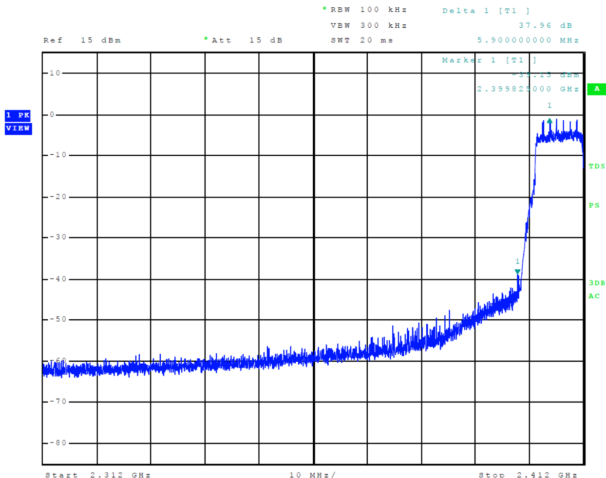
Figure 20 Plot of Emissions Low Band Edge Mode 16, Radio 2, 802.11n
