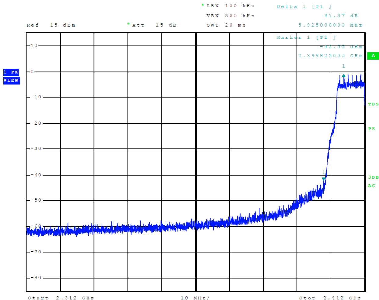
Figure 19 Plot of Emissions Low Band Edge Mode 15, Radio 2, 802.11g
