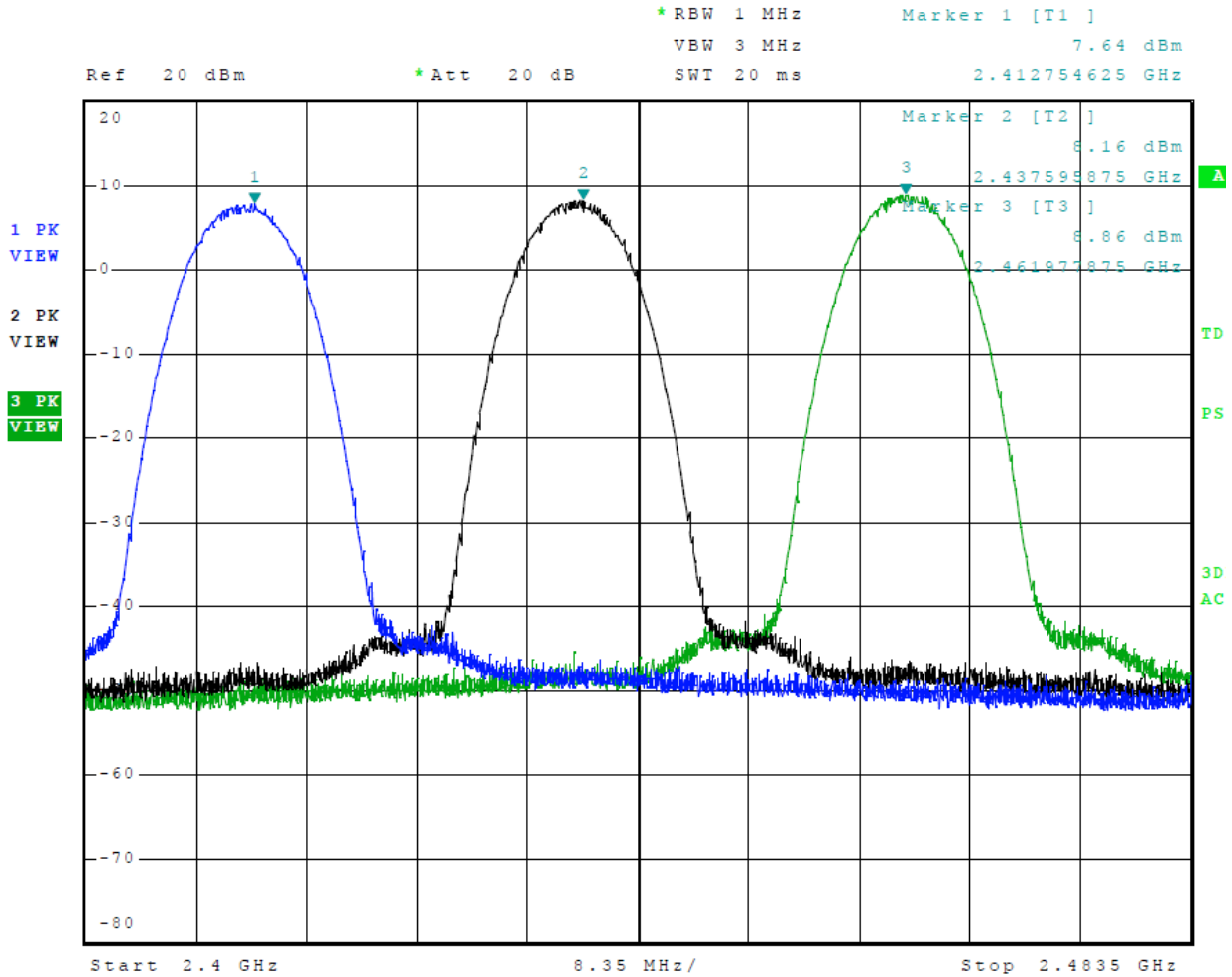
Figure 6 Plot of Transmitter Operation in 2412-2462 MHz Mode 5, Radio 1, 802.11b
