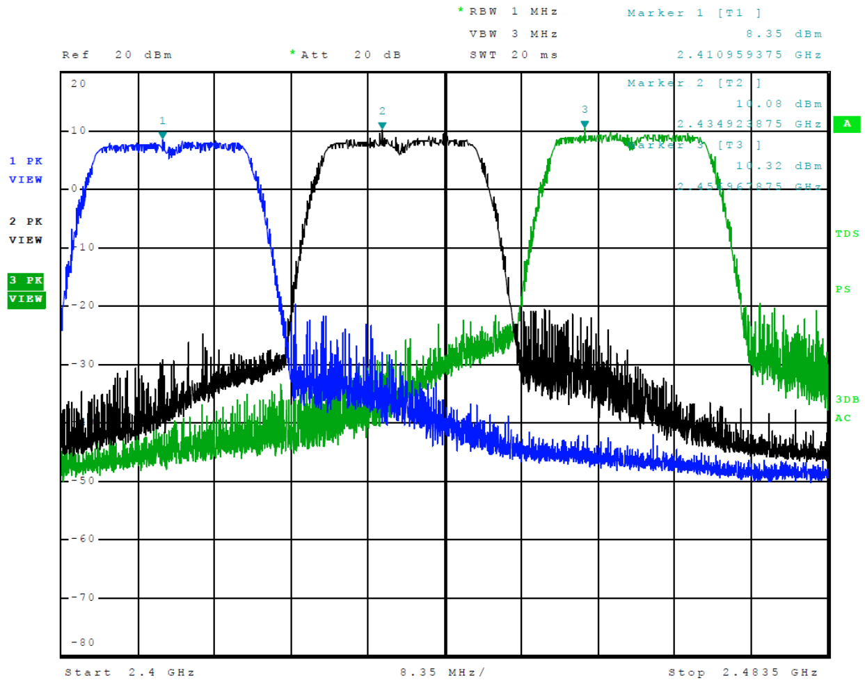
Figure 11 Plot of Transmitter Operation in 2412-2462 MHz Mode 16, Radio 2, 802.11n
