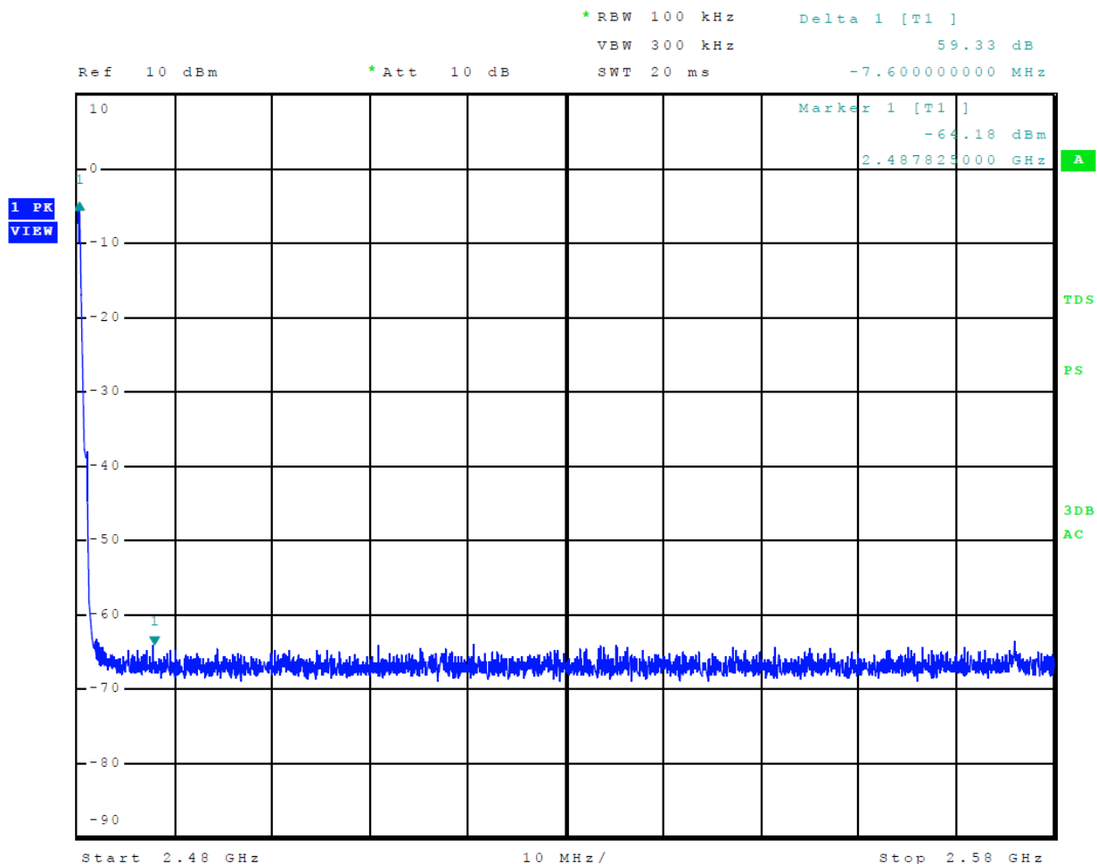
Figure 23 Plot of Transmitter Emissions High Band Edge Mode 4, Radio 1, BT BLE
