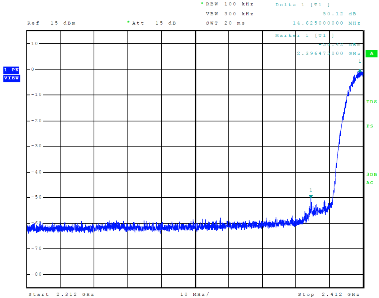
Figure 18 Plot of Emissions Low Band Edge Mode 14, Radio 2, 802.11b
