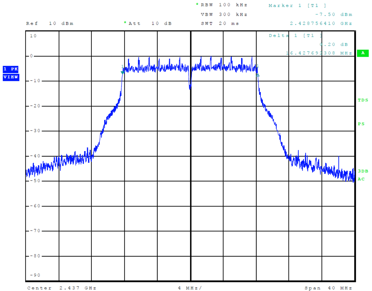
Figure 44 Plot of 6-dB Occupied Bandwidth Mode 15, Radio 2, 802.11g
