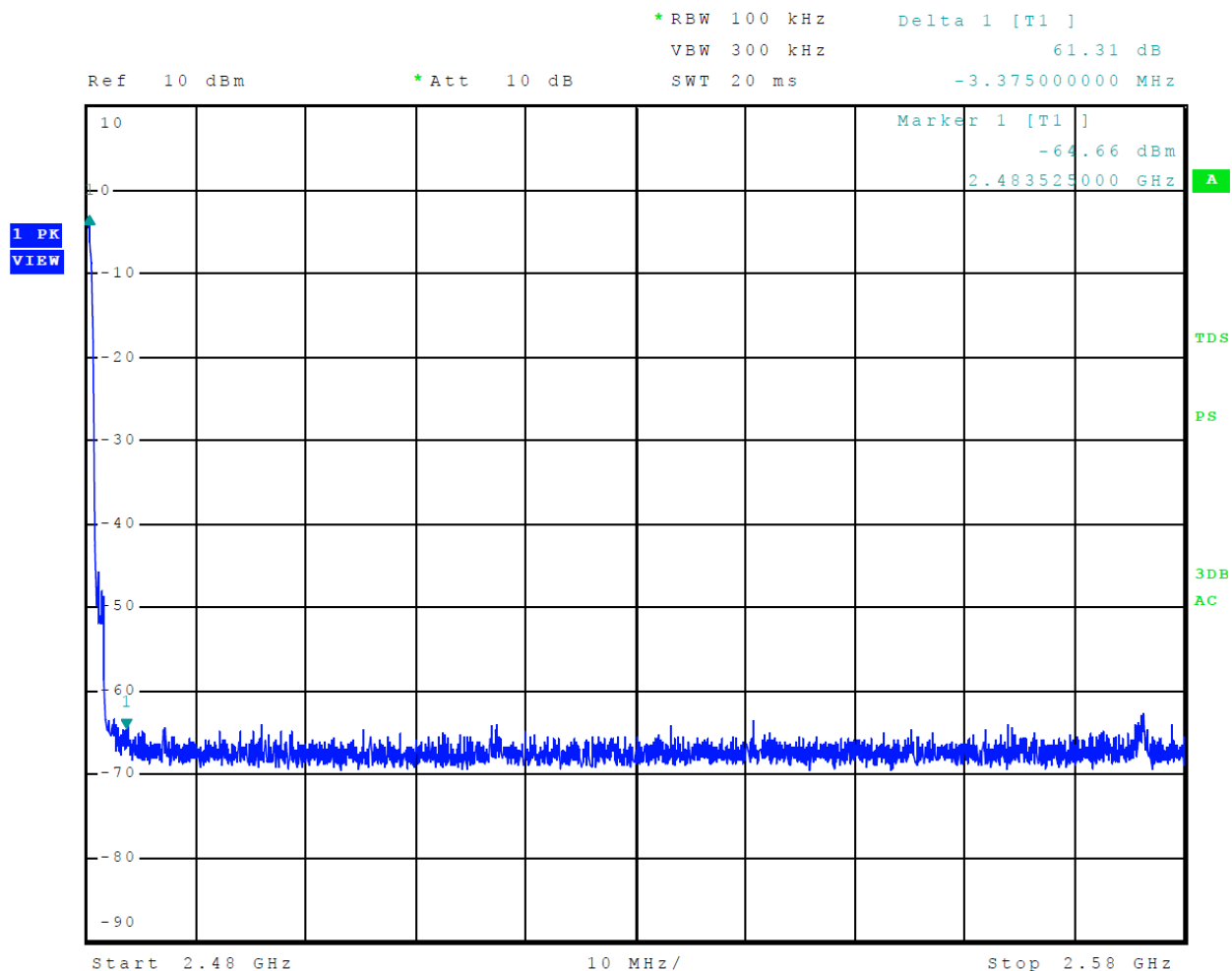
Figure 22 Plot of Transmitter Emissions High Band Edge Mode 3, Radio 1, BT (3EDR)
