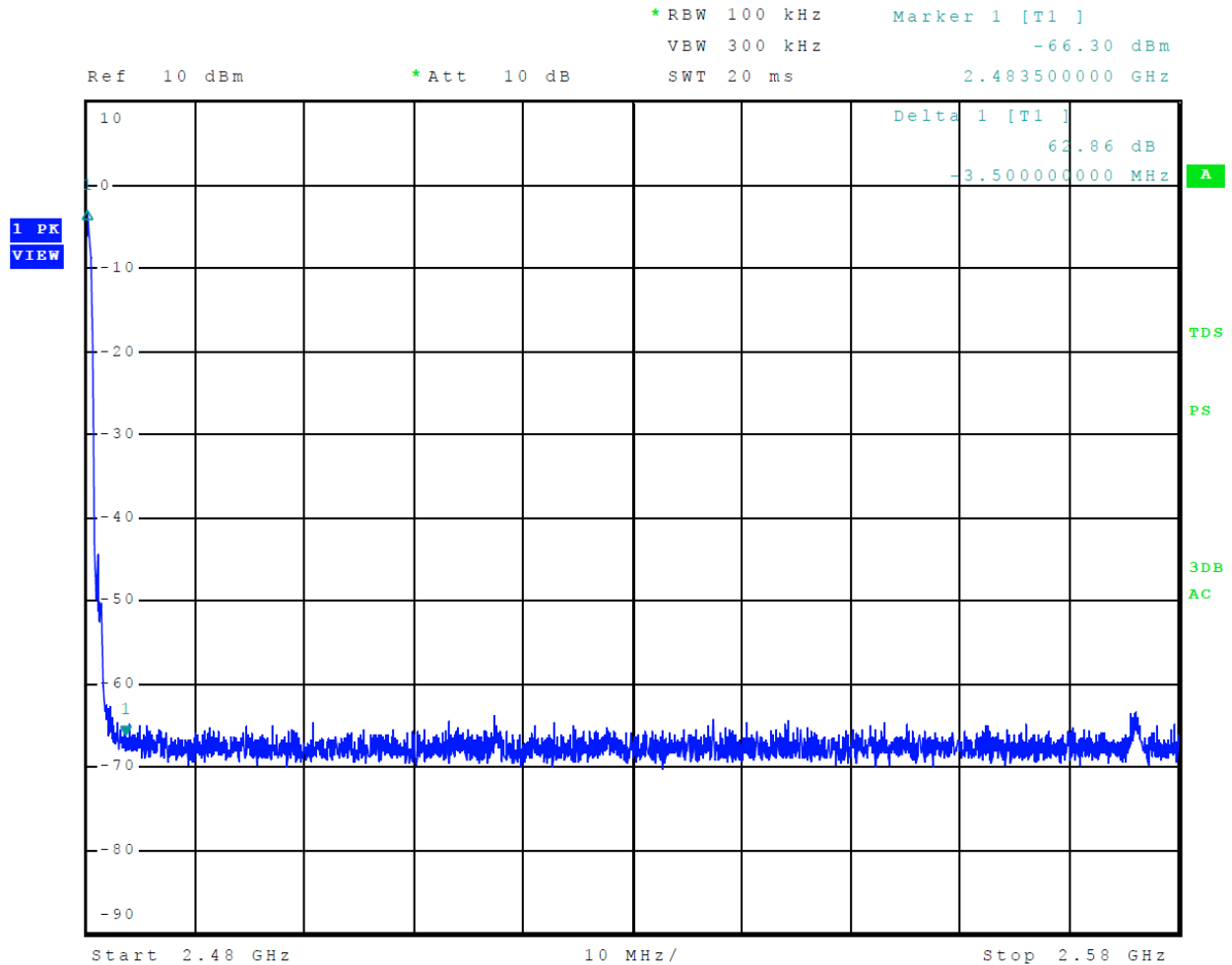
Figure 21 Plot of Transmitter Emissions High Band Edge Mode 2, Radio 1, BT (2EDR)
