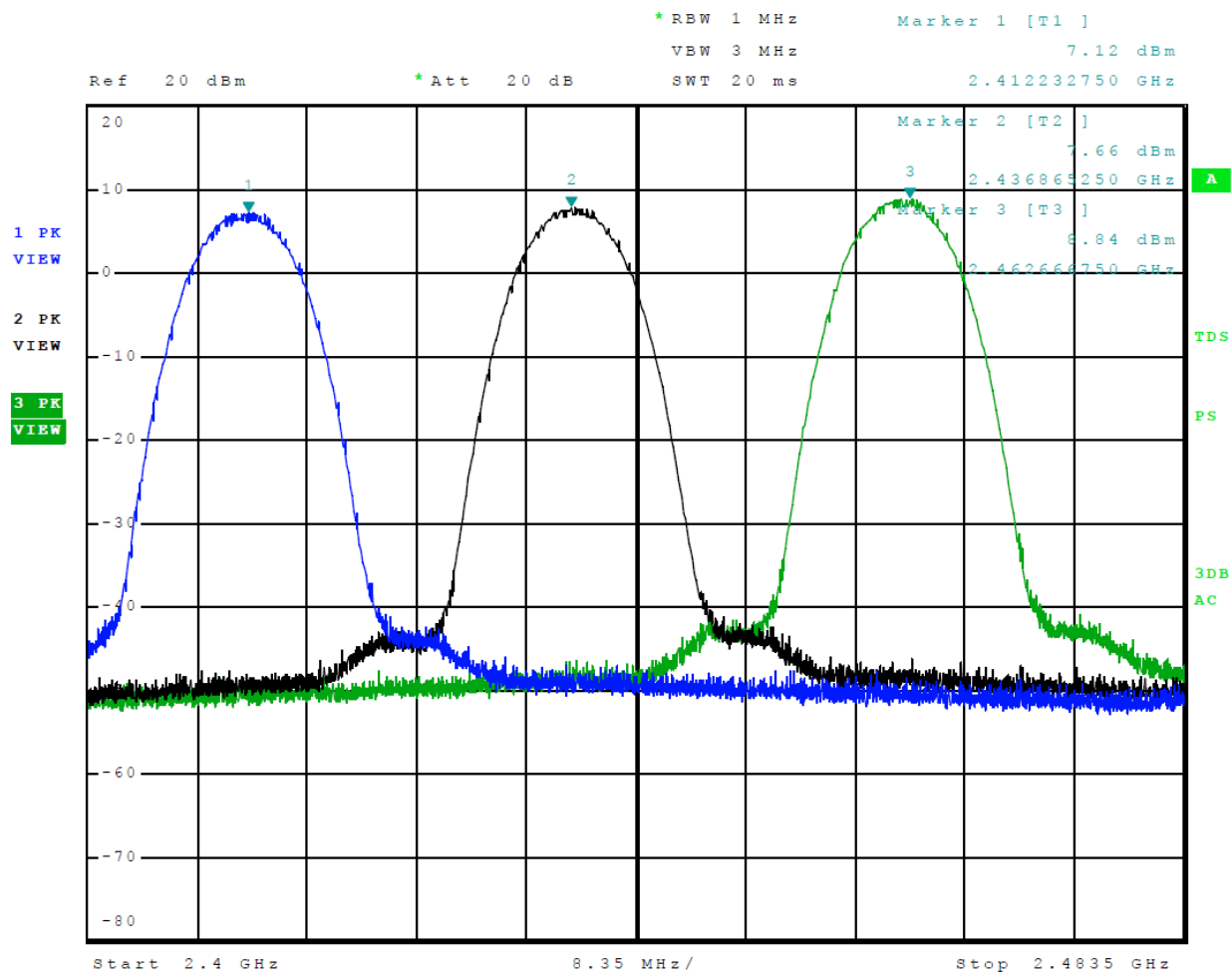
Figure 9 Plot of Transmitter Operation in 2412-2462 MHz Mode 14, Radio 2, 802.11b
