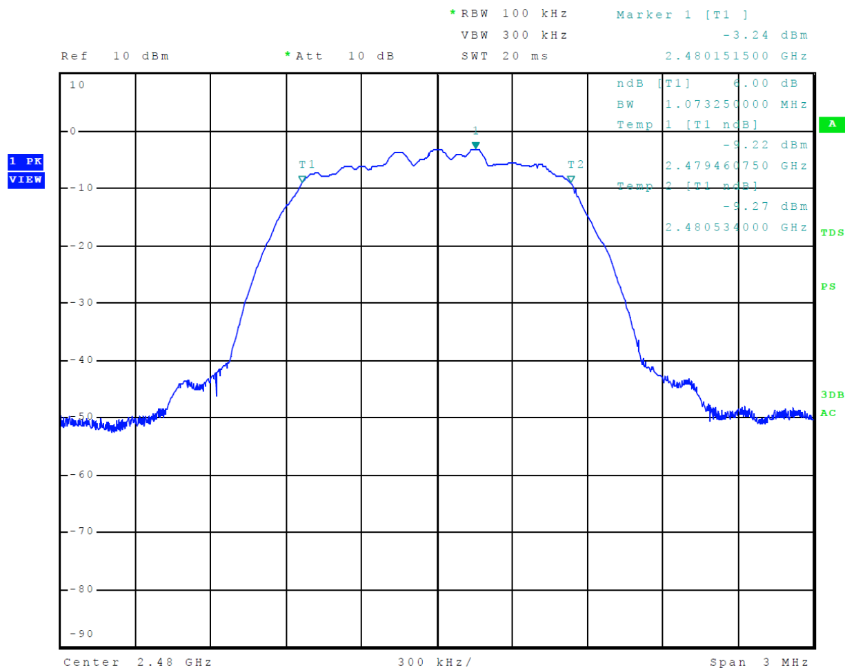
Figure 30 Plot of 6-dB Occupied Bandwidth Mode 2, Radio 1, BT (2EDR)
