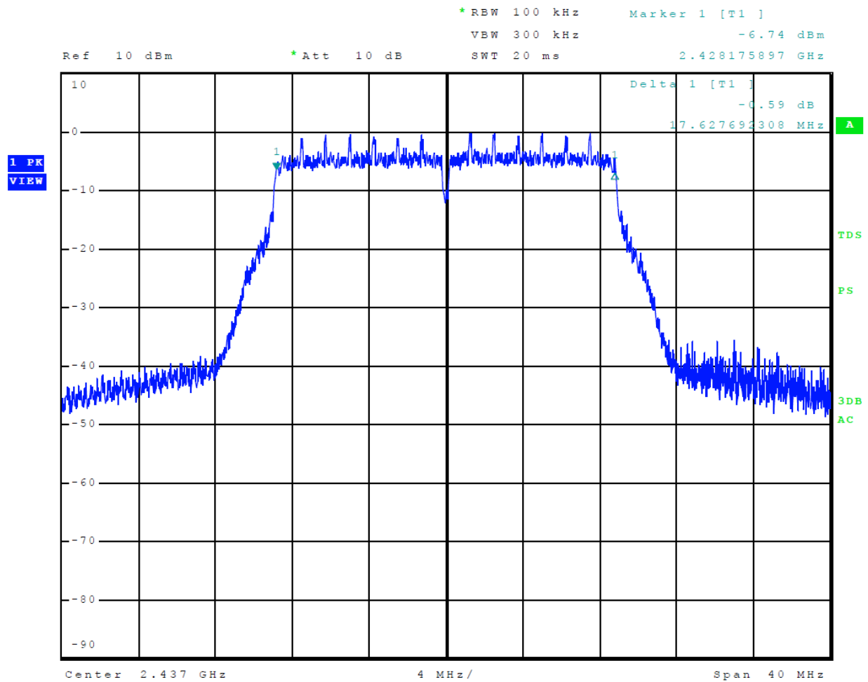
Figure 46 Plot of 6-dB Occupied Bandwidth Mode 16, Radio 2, 802.11n
