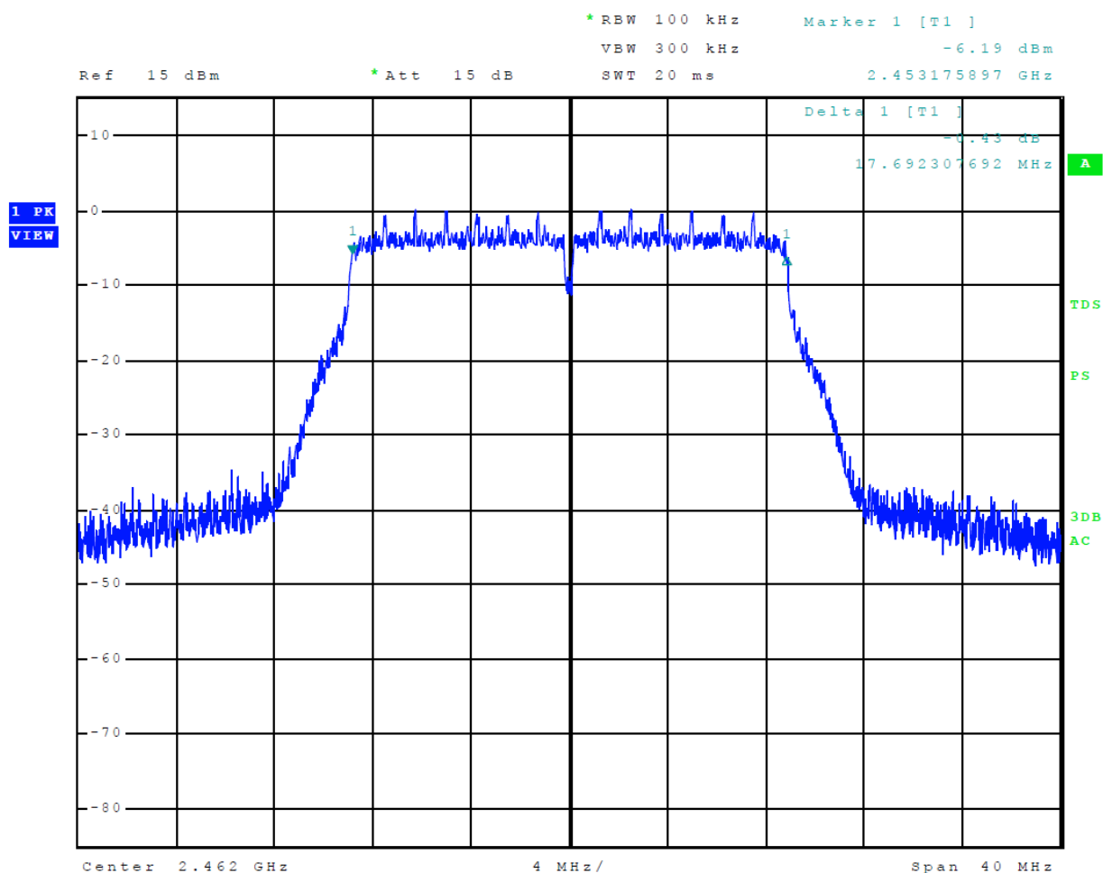
Figure 40 Plot of 6-dB Occupied Bandwidth Mode 7, Radio 1, 802.11n
