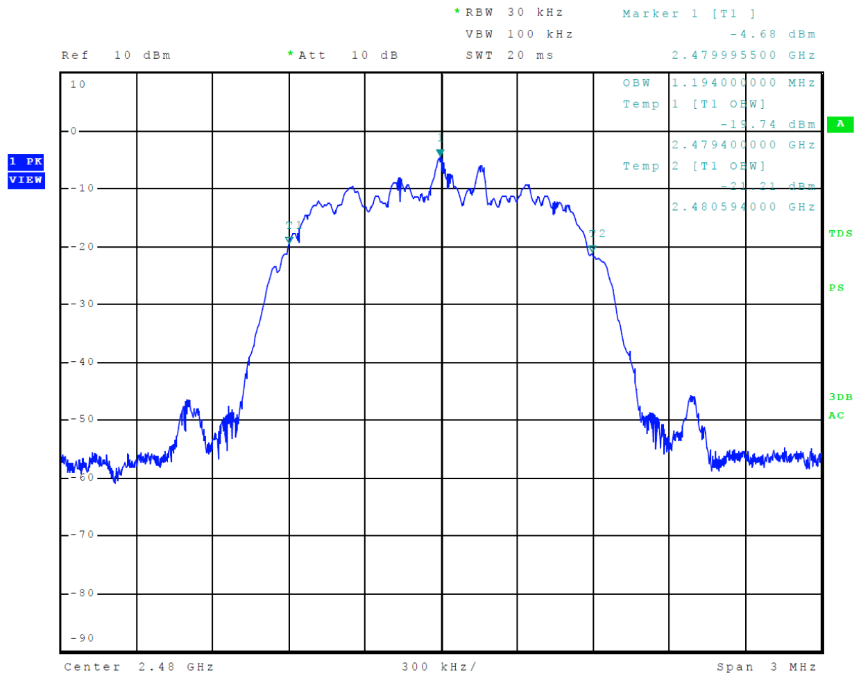
Figure 31 Plot of 99% Occupied Bandwidth Mode 2, Radio 1, BT (2EDR)
