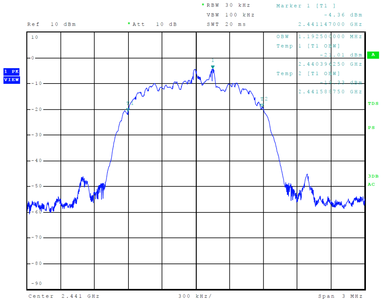
Figure 33 Plot of 99% Occupied Bandwidth Mode 3, Radio 1, BT (3EDR)
