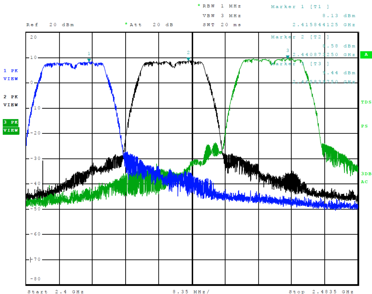
Figure 10 Plot of Transmitter Operation in 2412-2462 MHz Mode 15, Radio 2, 802.11g
