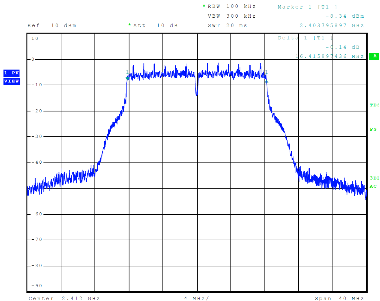
Figure 38 Plot of 6-dB Occupied Bandwidth Mode 6, Radio 1, 802.11g
