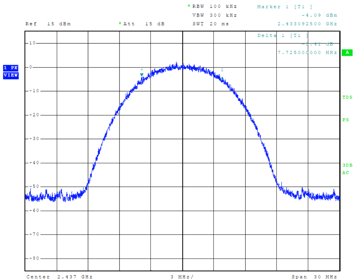
Figure 36 Plot of 6-dB Occupied Bandwidth Mode 5, Radio 1, 802.11b
