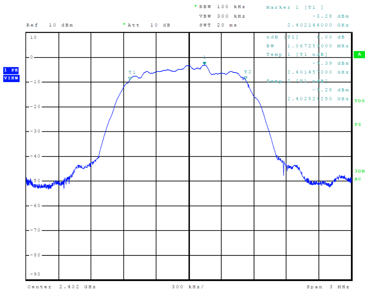
Figure 32 Plot of 6-dB Occupied Bandwidth Mode 3, Radio 1, BT (3EDR)
