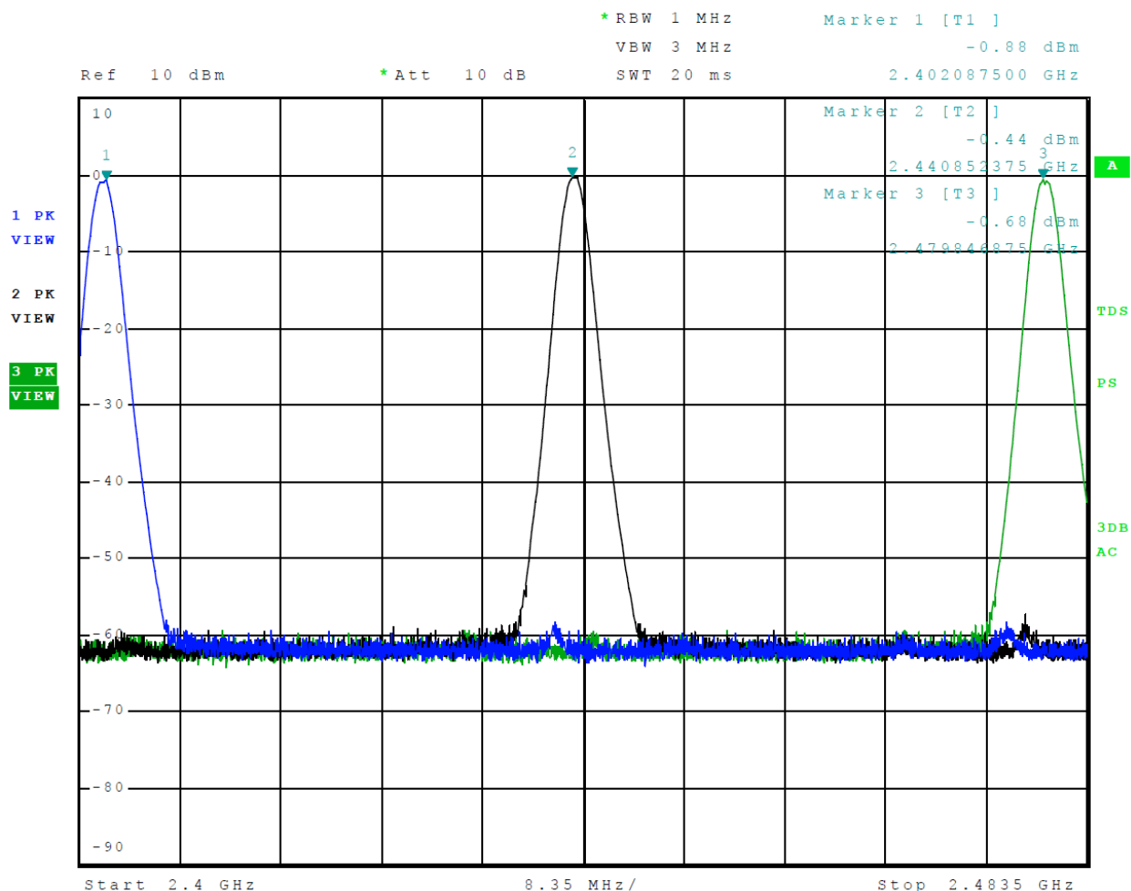
Figure 3 Plot of Transmitter Operation in 2402-2480 MHz Mode 2, Radio 1, BT (2EDR)
