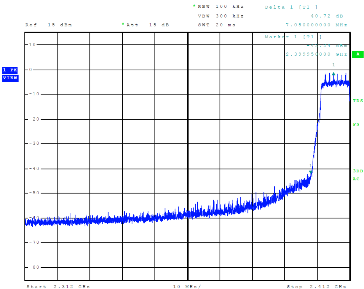
Figure 17 Plot of Emissions Low Band Edge Mode 7, Radio 1, 802.11n
