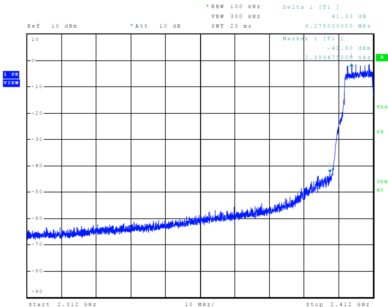
Figure 16 Plot of Emissions Low Band Edge Mode 6, Radio 1, 802.11g
