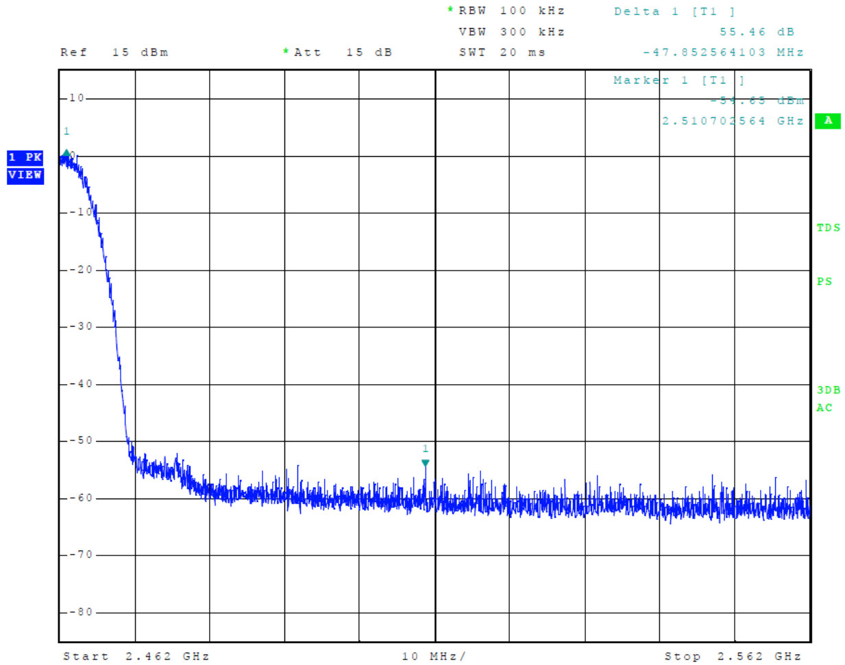
Figure 24 Plot of Transmitter Emissions High Band Edge Mode 5, Radio 1, 802.11b
