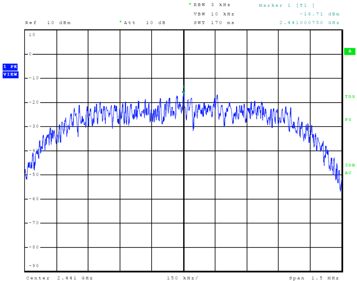
Figure 49 Plot of Transmitter Power Spectral Density Mode 3, Radio 1, BT (3EDR)
