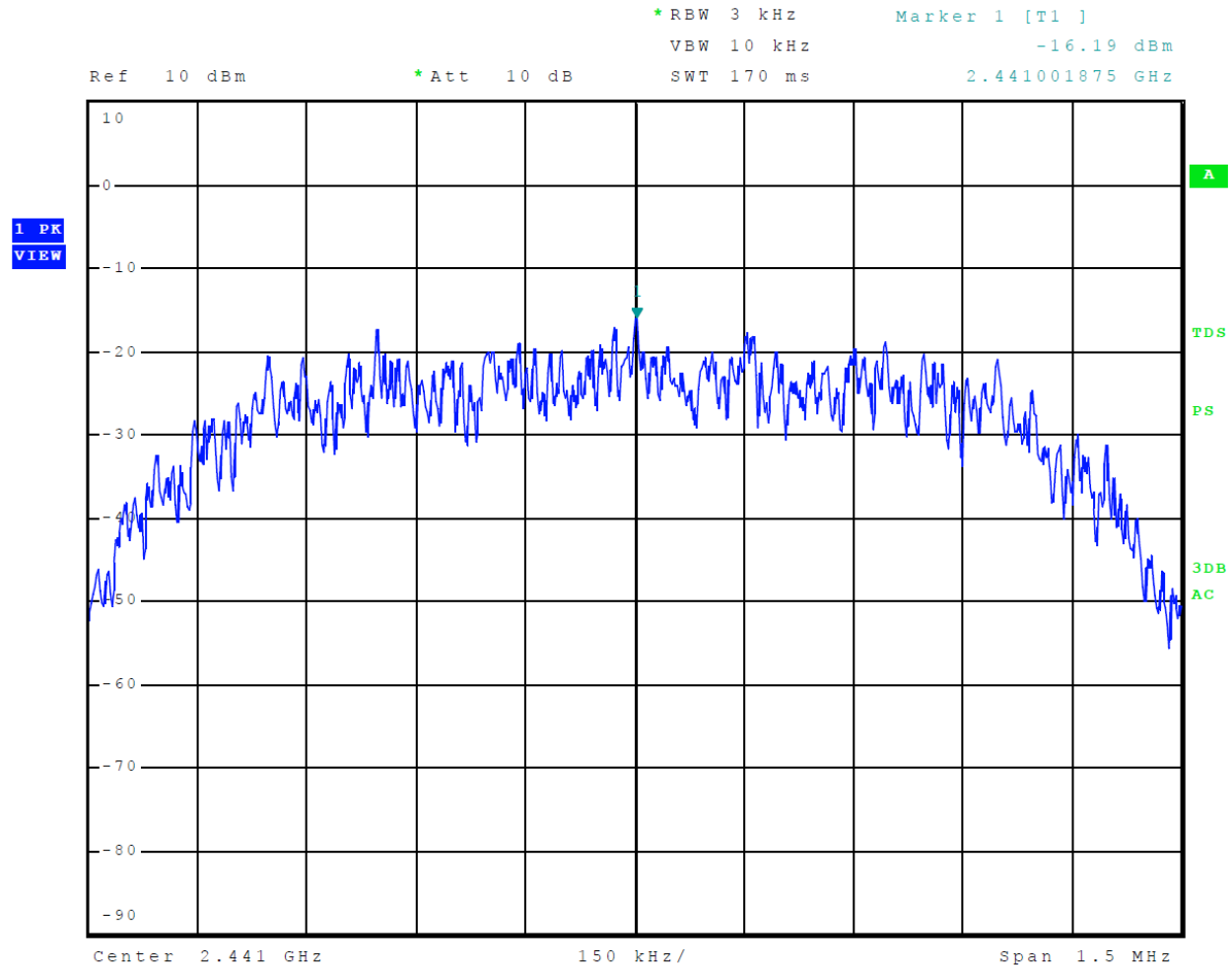
Figure 48 Plot of Transmitter Power Spectral Density Mode 2, Radio 1, BT (2EDR)
