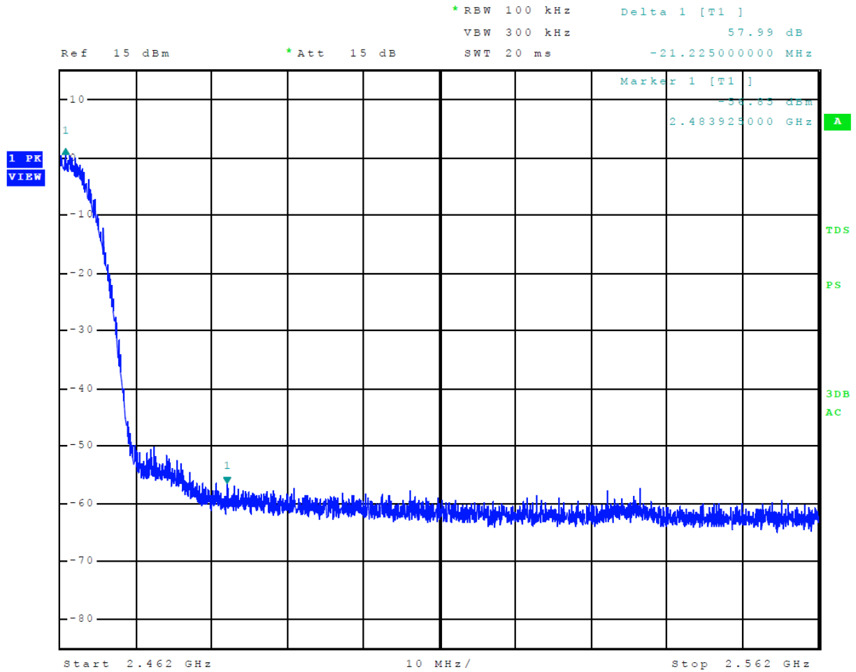
Figure 27 Plot of Transmitter Emissions High Band Edge Mode 14, Radio 2, 802.11b
