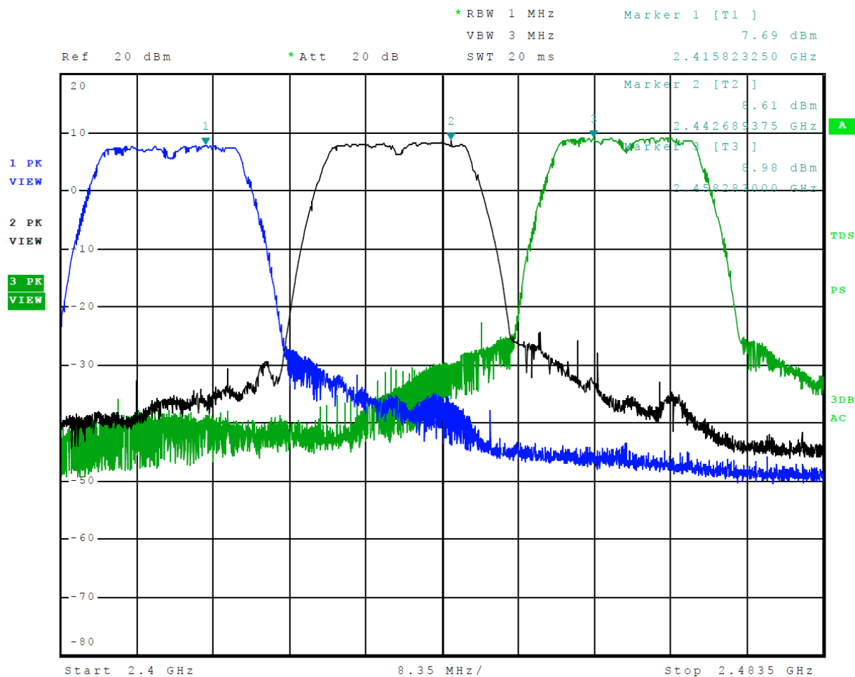
Figure 7 Plot of Transmitter Operation in 2412-2462 MHz Mode 6, Radio 1, 802.11g
