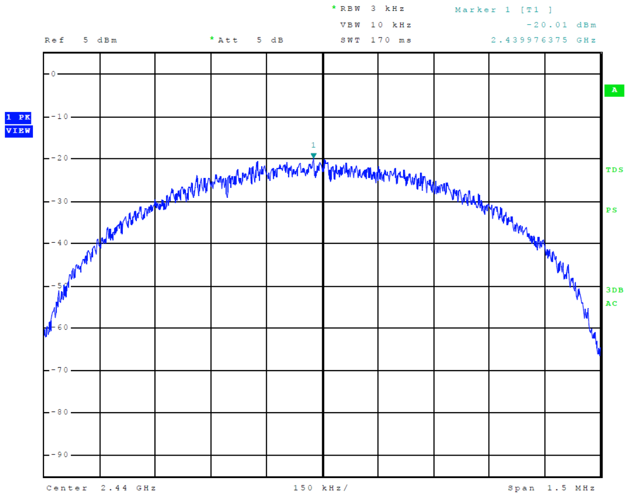
Figure 50 Plot of Transmitter Power Spectral Density Mode 4, Radio 1, BT BLE
