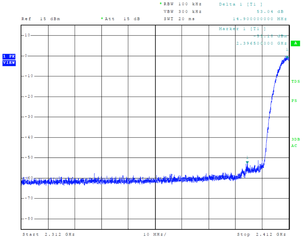
Figure 15 Plot of Emissions Low Band Edge Mode 5, Radio 1, 802.11b
