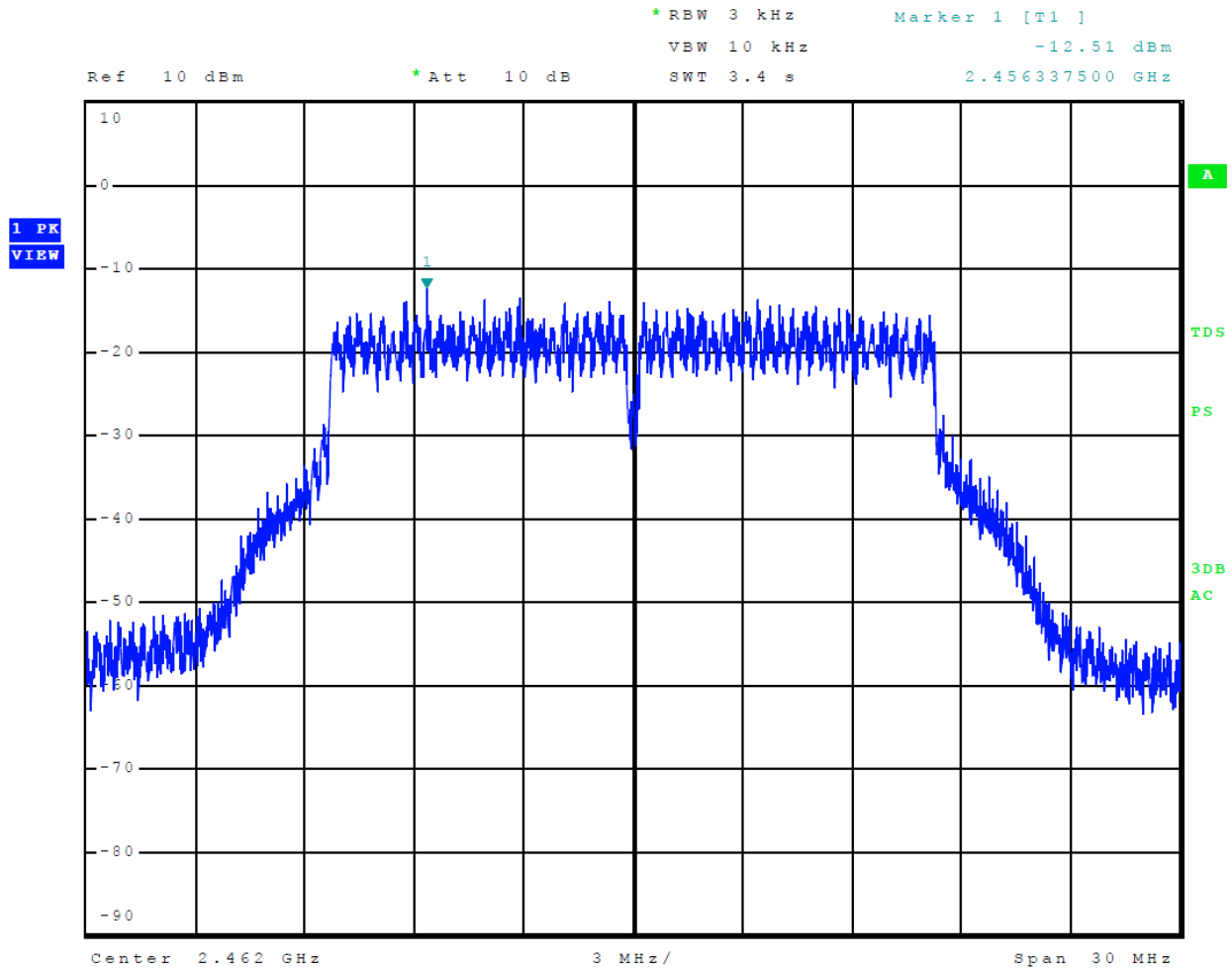
Figure 55 Plot of Transmitter Power Spectral Density Mode 15, Radio 2, 802.11g
