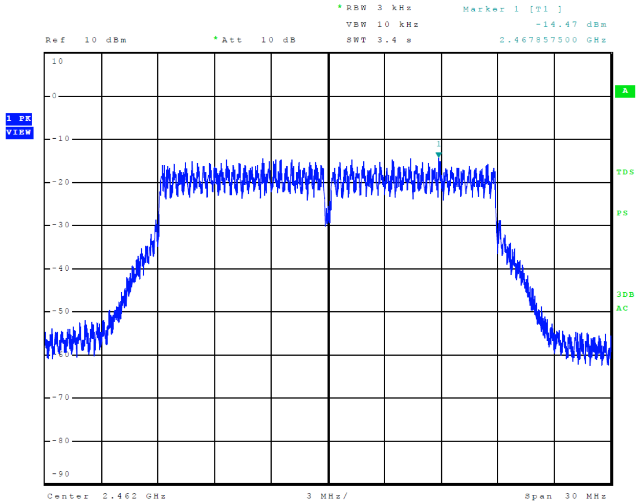
Figure 53 Plot of Transmitter Power Spectral Density Mode 7, Radio 1, 802.11n
