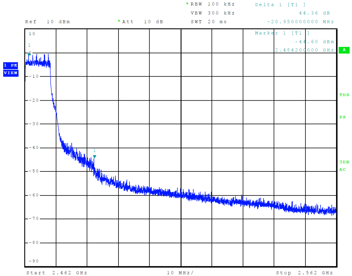
Figure 25 Plot of Transmitter Emissions High Band Edge Mode 6, Radio1, 802.11g
