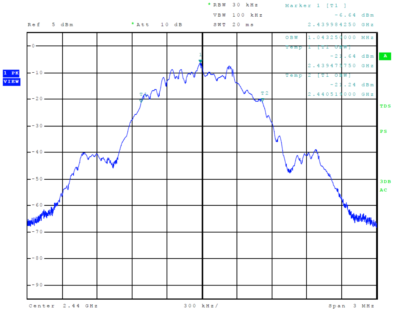
Figure 35 Plot of 99% Occupied Bandwidth Mode 4, Radio 1, BT BLE
