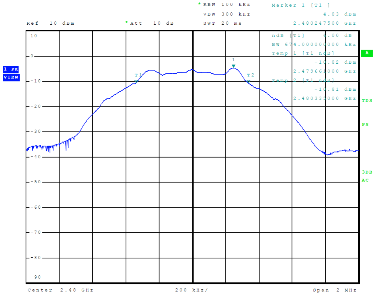
Figure 34 Plot of 6-dB Occupied Bandwidth Mode 4, Radio 1, BT BLE
