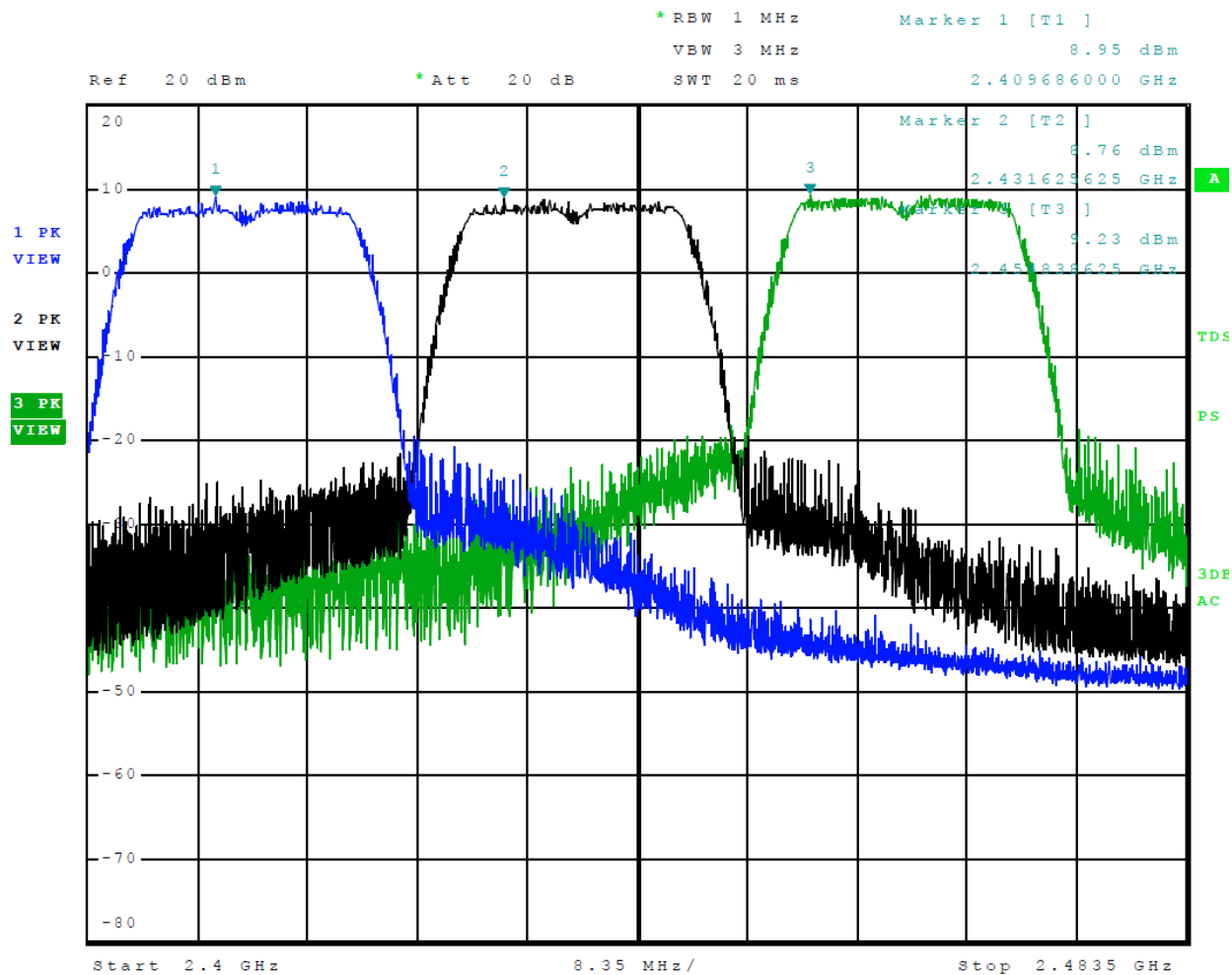
Figure 8 Plot of Transmitter Operation in 2412-2462 MHz Mode 7, Radio 1, 802.11n
