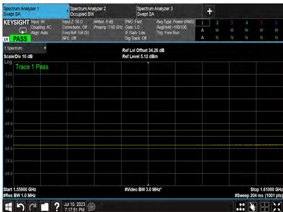
Figure 101 – 1616.020833 MHz - Carrier-off state Emissions
