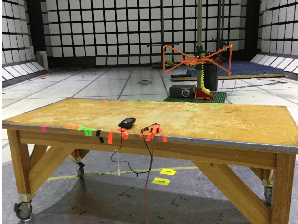
Figure 1 - Radiated Emissions Setup, 30MHz – 1GHz
