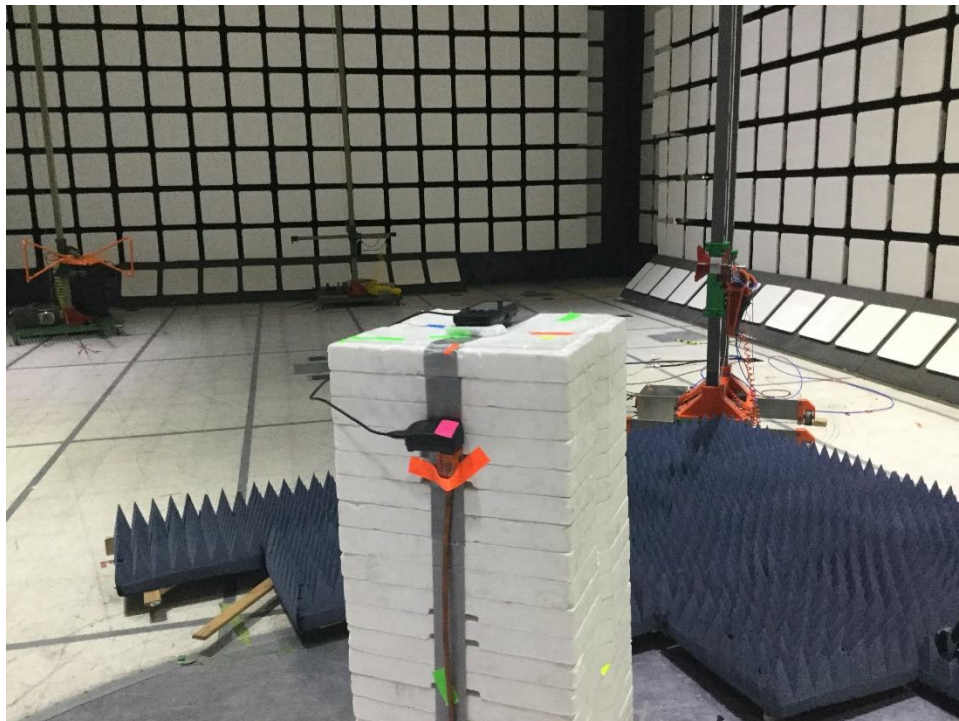
Figure 2 - Radiated Emissions Setup, >1GHz
