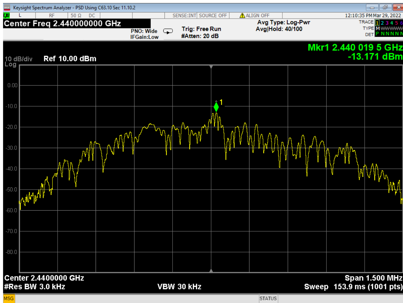
8 PSD, Mid Channel, GMSK
