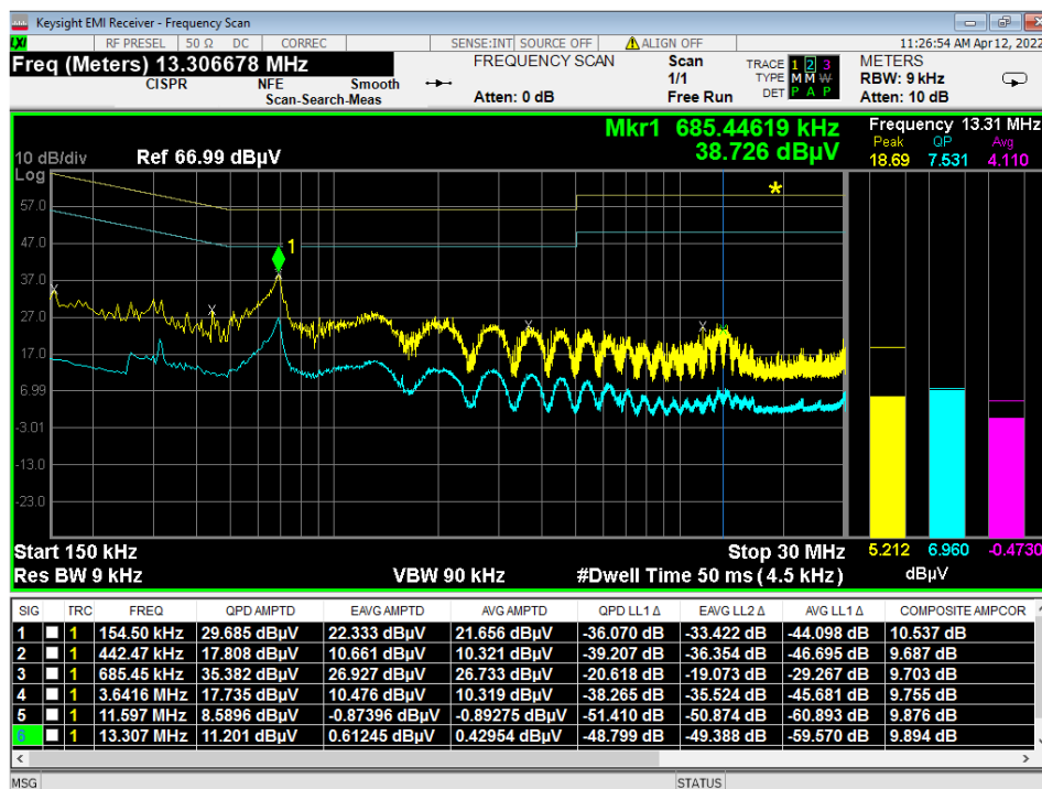
Figure 10 - Conducted Emissions Plot, Neutral, GMSK
