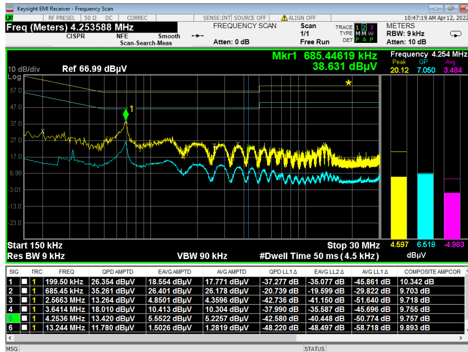
Figure 12 - Conducted Emissions Plot, Neutral, Receive
