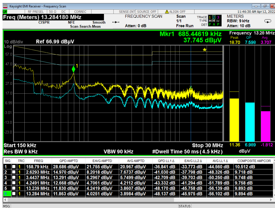
Figure 9 - Conducted Emissions Plot, Line, GMSK
