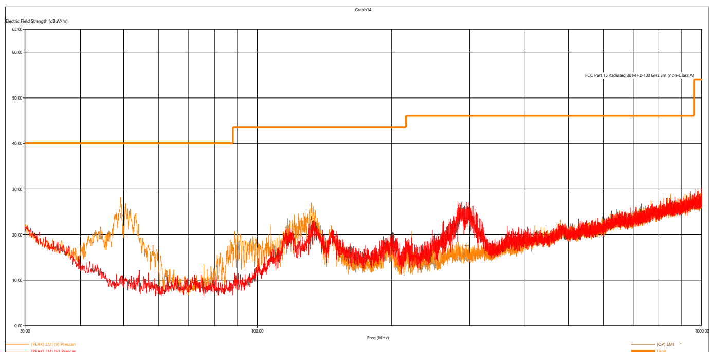
Figure 5 - Radiated Emissions Plot, GMSK
