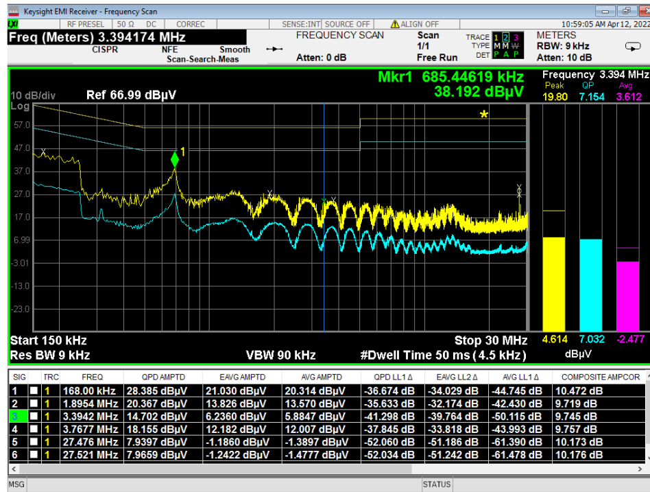
Figure 11 - Conducted Emissions Plot, Line, Receive
