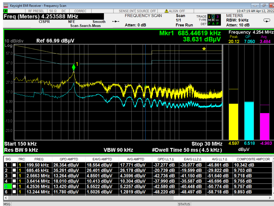
Figure 12 - Conducted Emissions Plot, Idle, Neutral
