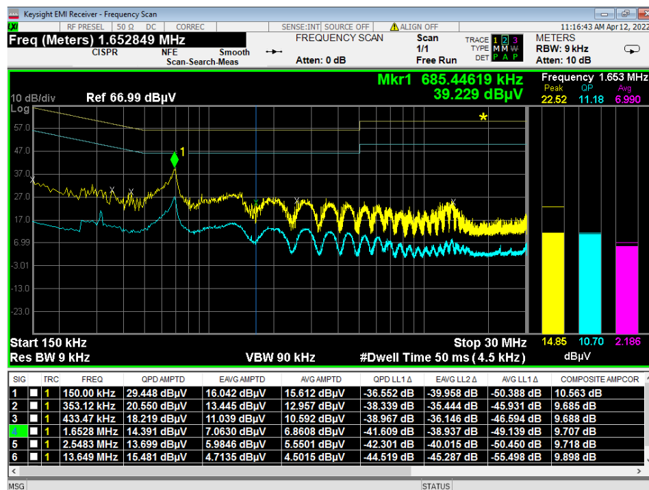
Figure 10 - Conducted Emissions Plot, TX, Neutral
