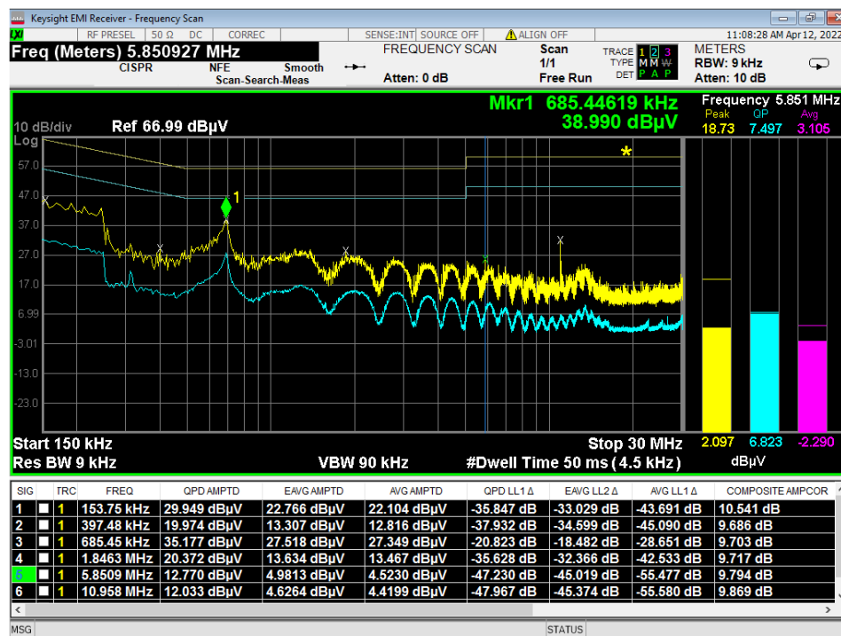
Figure 9 - Conducted Emissions Plot, TX, Line
