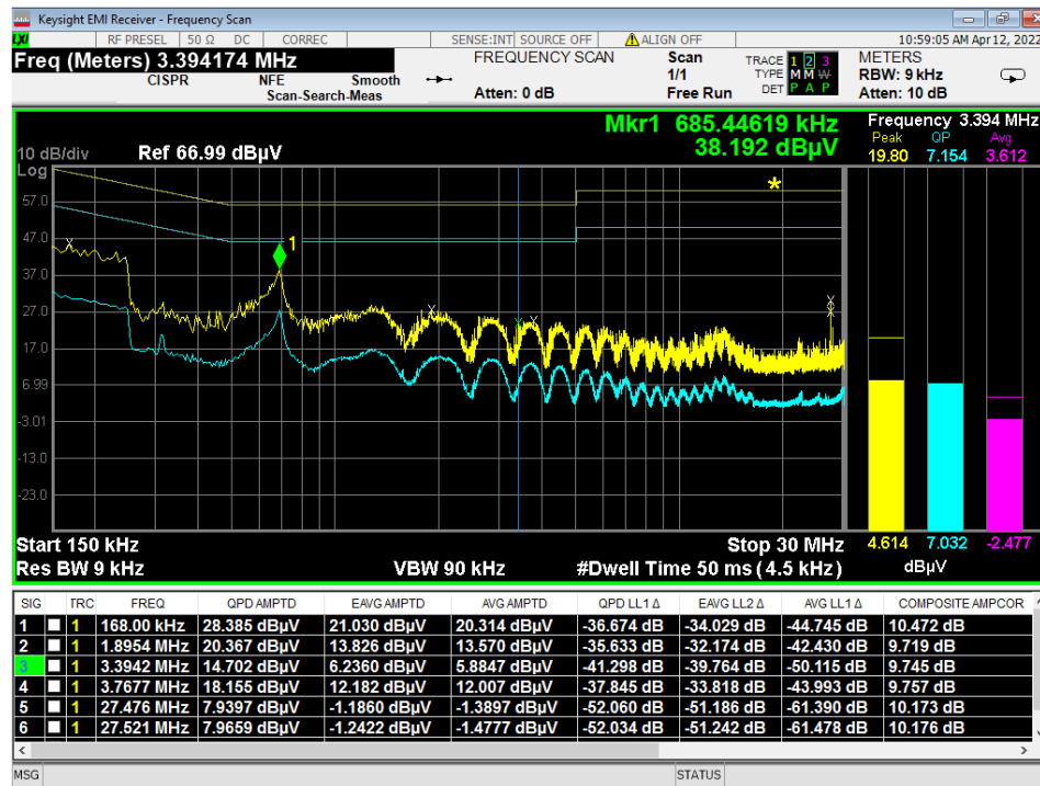
Figure 11 - Conducted Emissions Plot, Idle, Line
