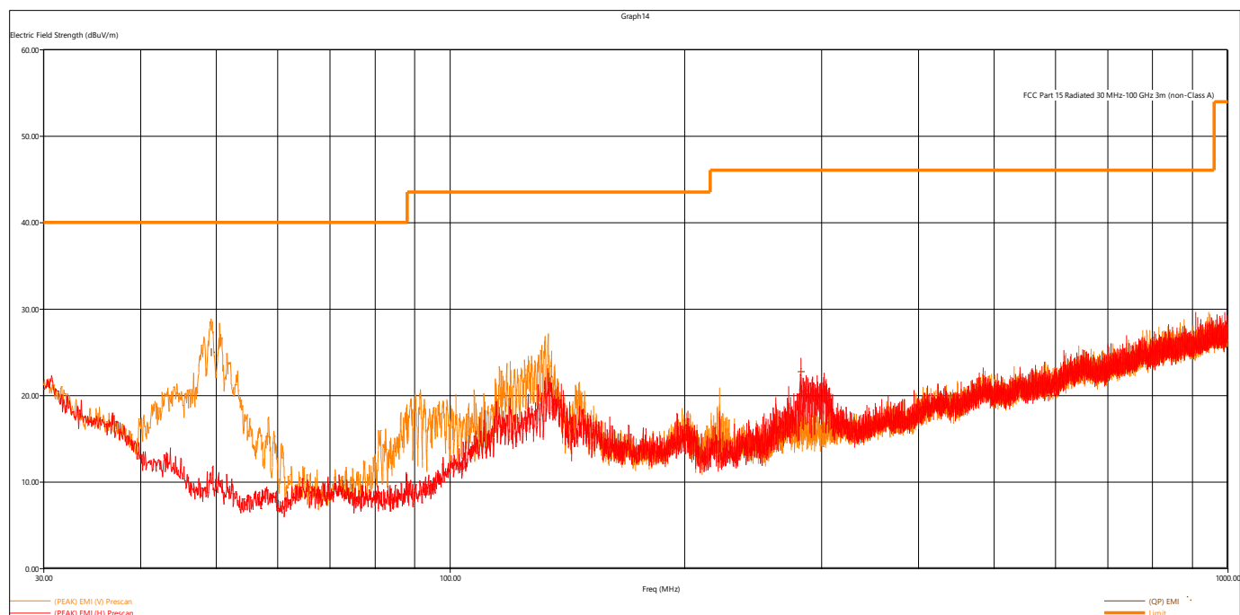
Figure 5 - Radiated Emissions Plot, Low Channel, GFSK
