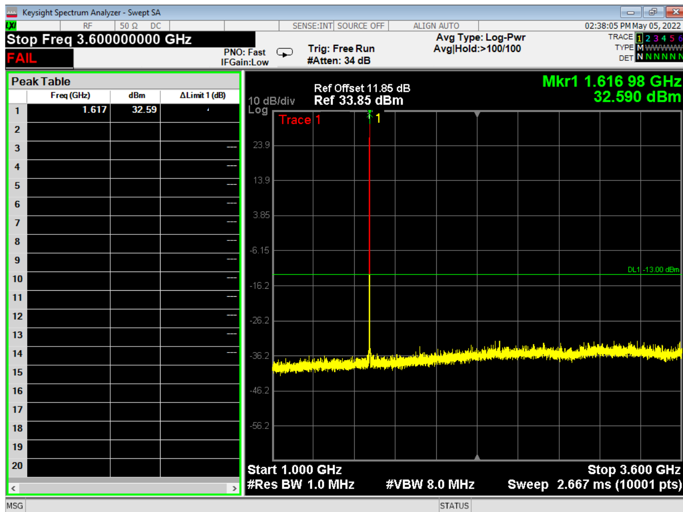
Figure 15 - Conducted Spurious Plot, 1G – 3.6G, Fundamental
