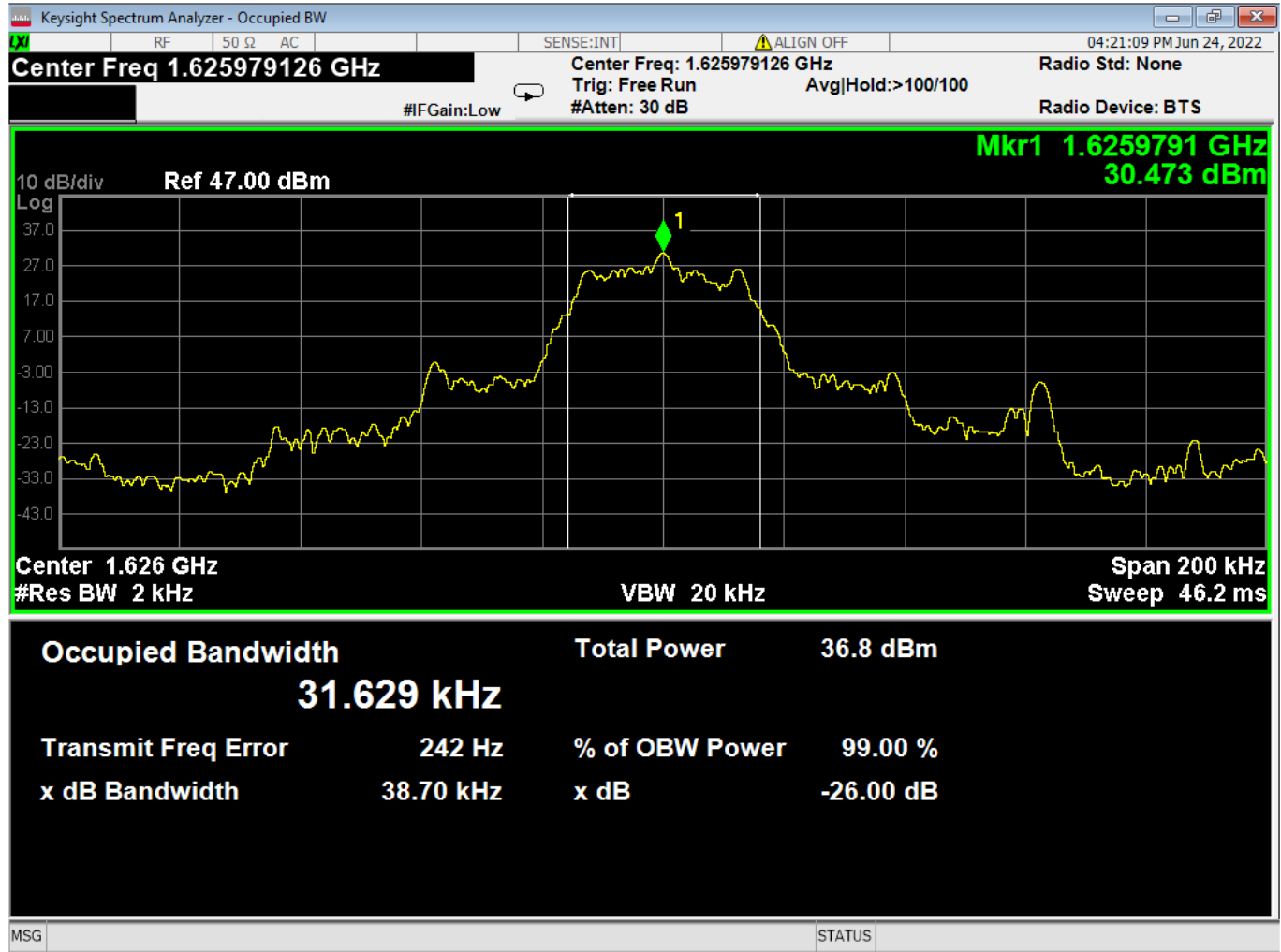
Figure 19 – Supporting Plots for modulation characteristic, High Channel
