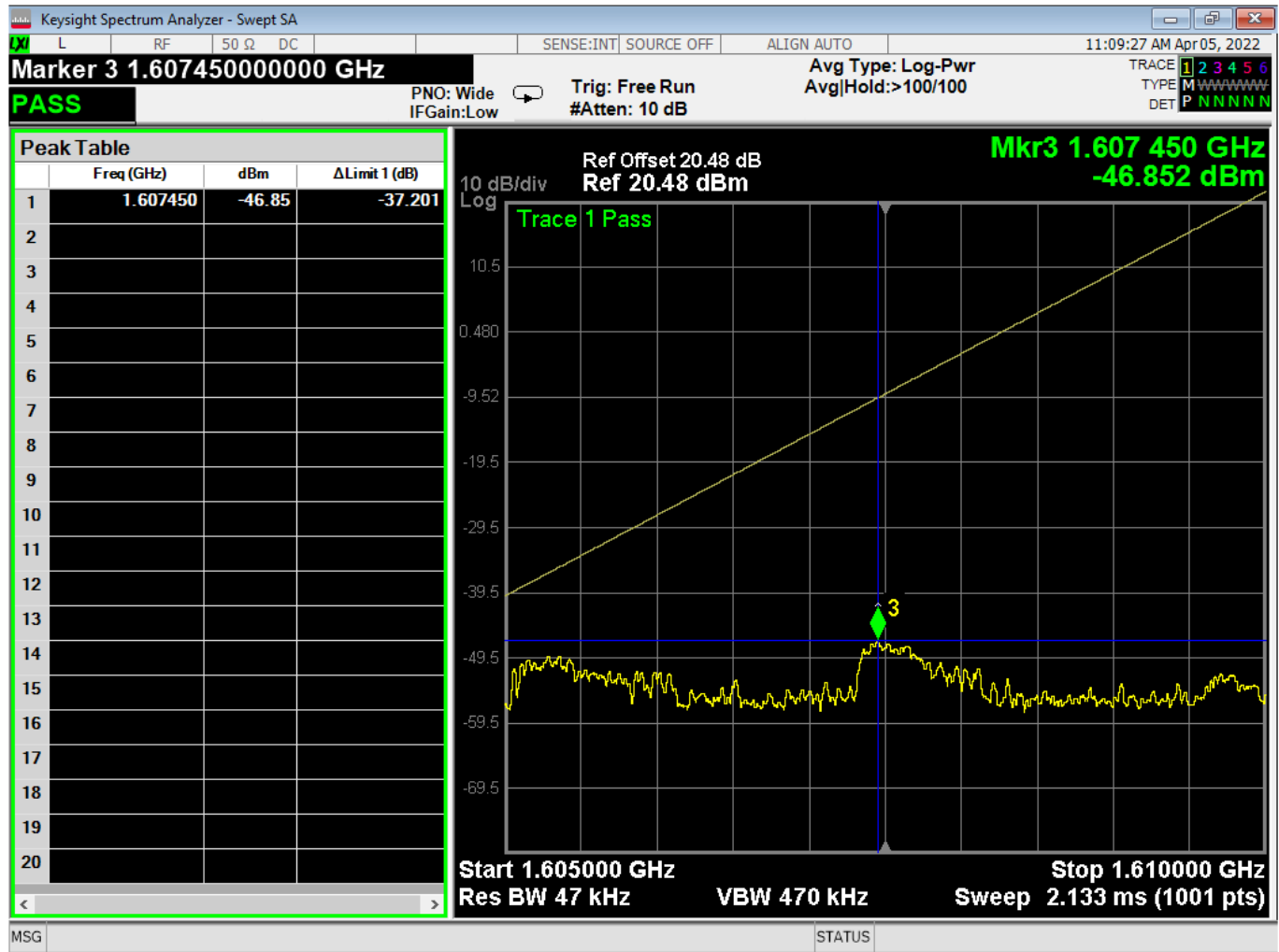
Figure 12 – Part 25.216(g), Transmitting at 1620.979126 MHz, Conducted Measurement
