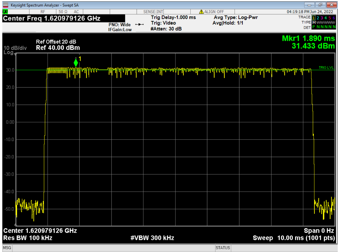
Figure 21 – Supporting Plots for modulation characteristic, Mid Channel
