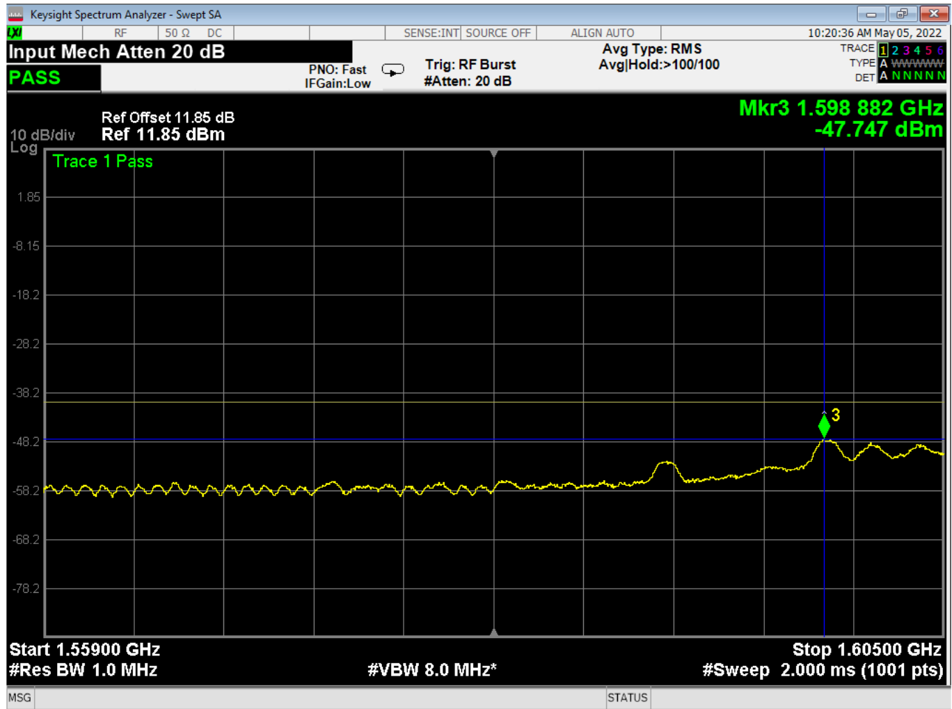
Figure 8 – Part 25.216(c), Transmitting at 1616.020752 MHz, Conducted Measurement
