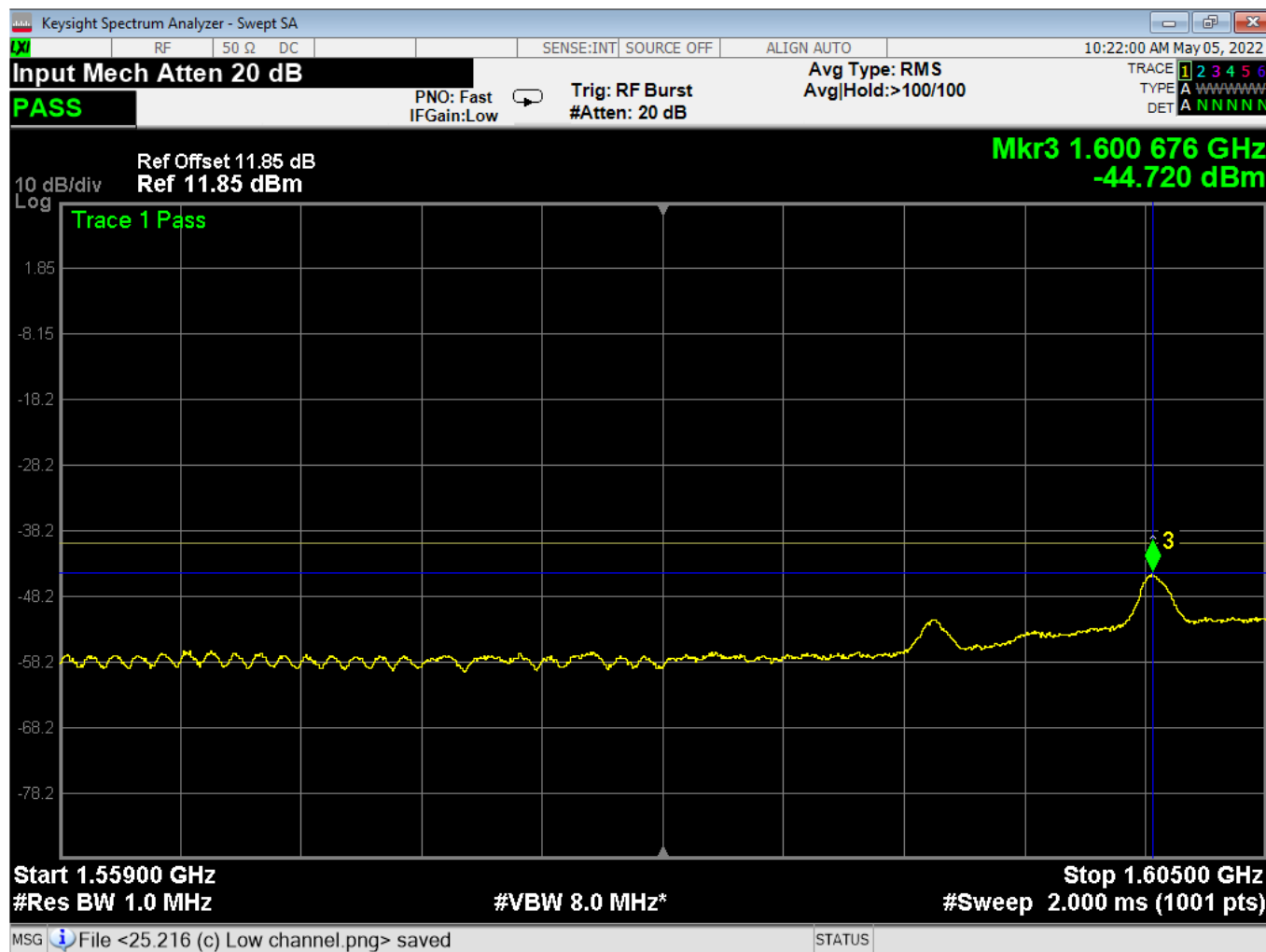
Figure 10 – Part 25.216(c), Transmitting at 1625.979126 MHz, Conducted Measurement
