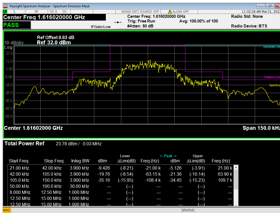
Figure 5 – Part 25.202(f) Mask, Transmitting at 1616.020752 MHz
