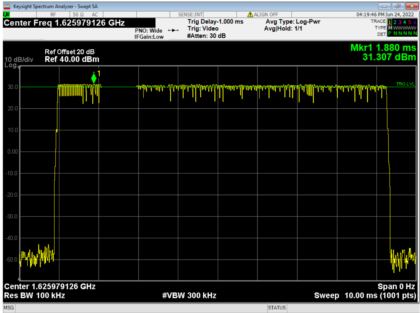
Figure 22 – Supporting Plots for modulation characteristic, High Channel
