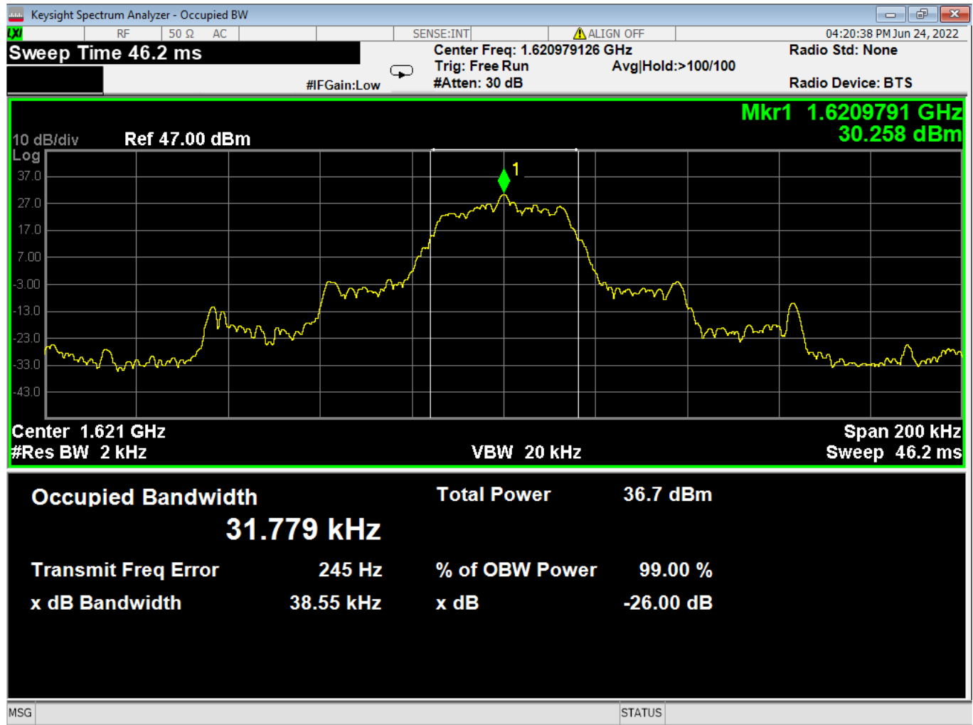
Figure 18 – Supporting Plots for modulation characteristic, Mid Channel
