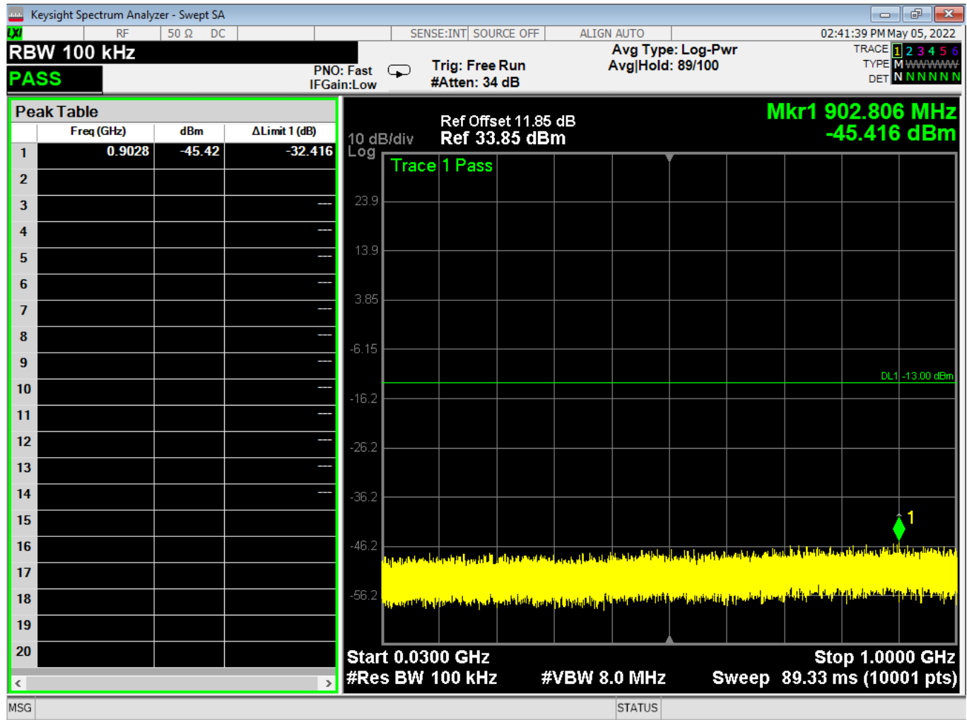
Figure 14 - Conducted Spurious Plot, 30M – 1G
