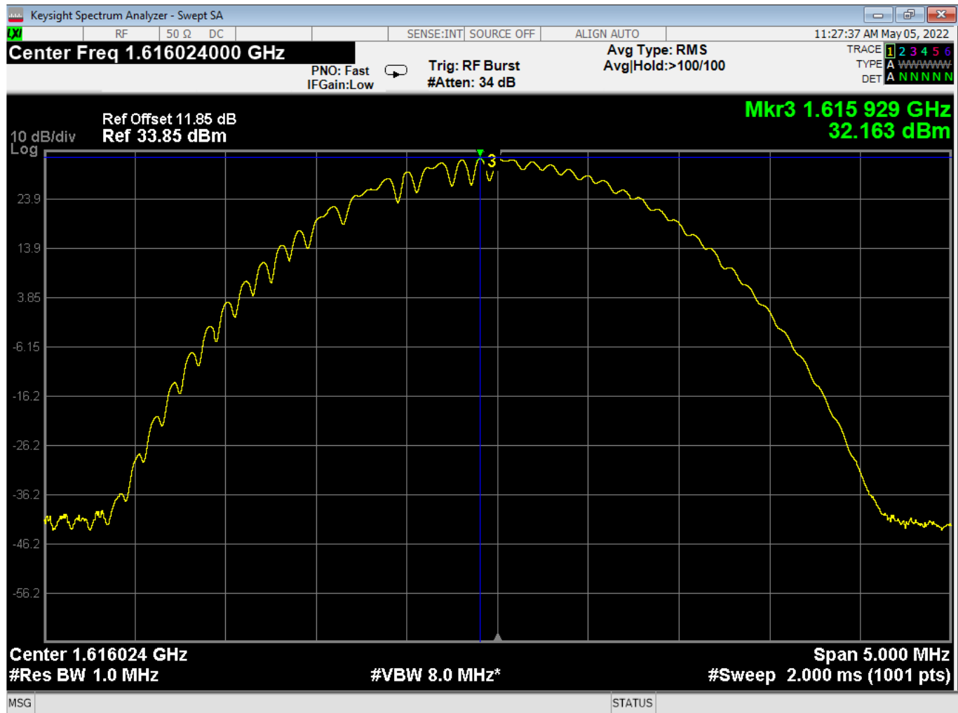
Figure 2 – Conducted Average Output Power, Transmitting at 1616.020752 MHz
