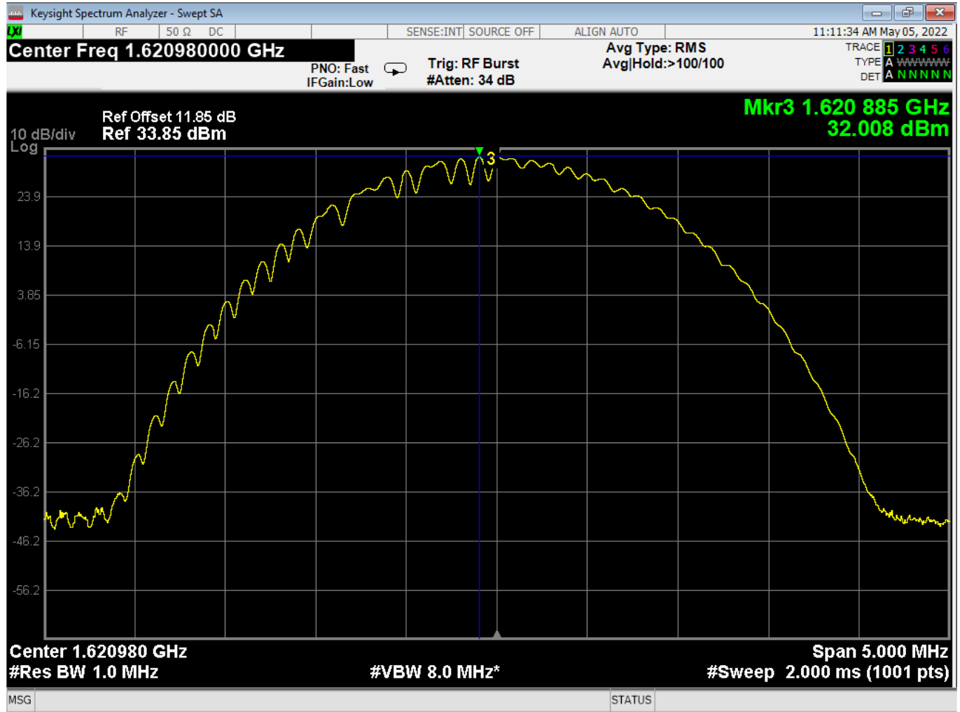
Figure 3 – Conducted Average Output Power, Transmitting at 1620.979126 MHz
