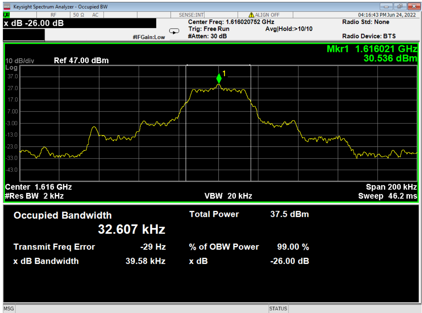
Figure 17 – Supporting Plots for modulation characteristic, Low Channel
