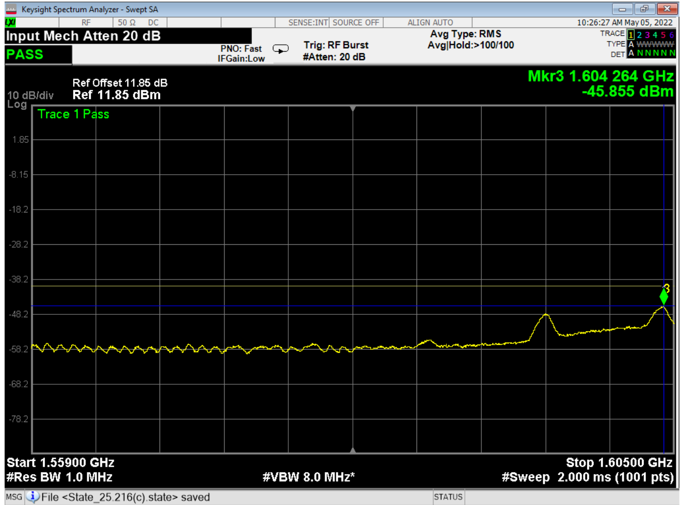
Figure 9 – Part 25.216(c), Transmitting at 1620.979126 MHz, Conducted Measurement *Limits have been converted from dBW to dBm. dBW = dBm + 30
