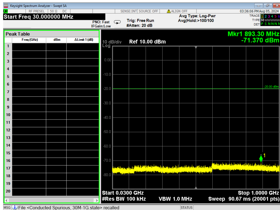
Figure 12 - Conducted Spurious emissions, GMSK 2MB, 30MHz – 1GHz, Mid
