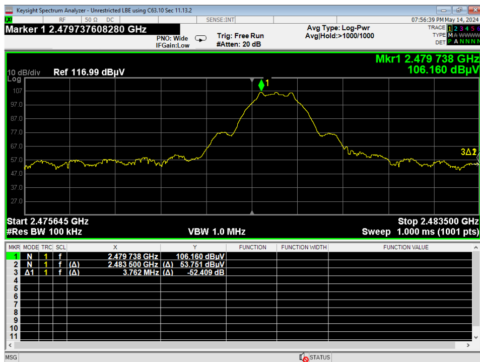
11 Higher Bandedge, Unrestricted, GMSK 1MB
