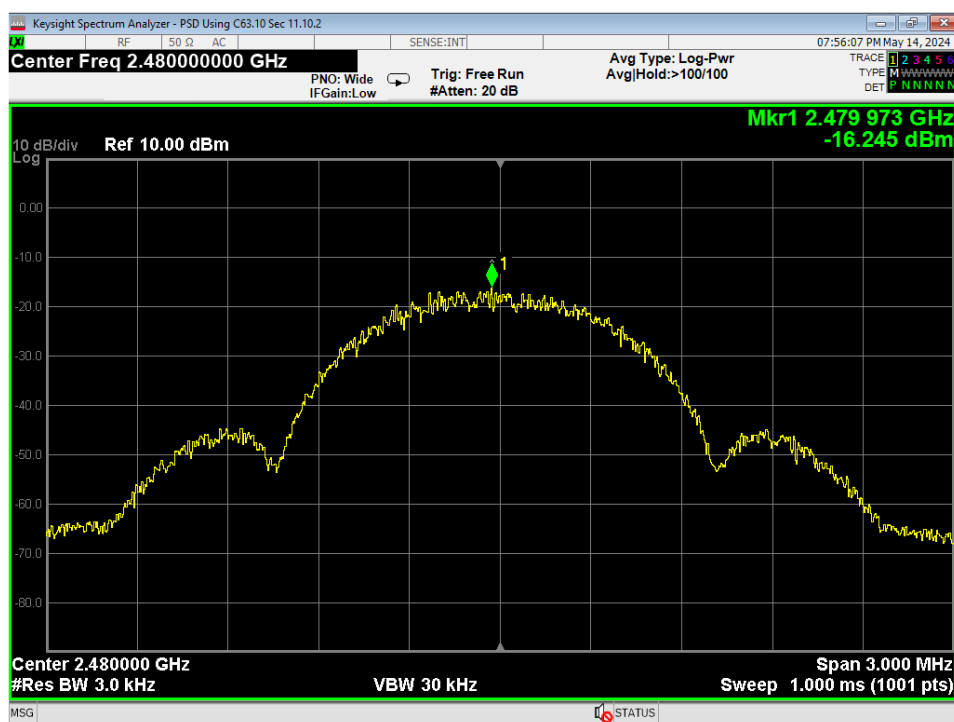
09 PSD, High Channel, GMSK 1MB
