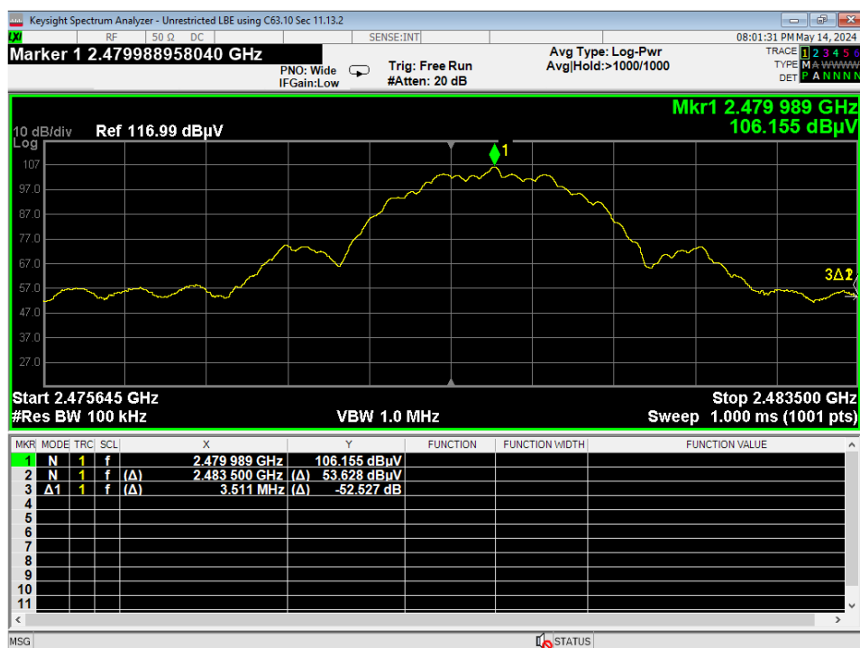
24 Higher Bandedge, Unrestricted, GMSK 2MB
