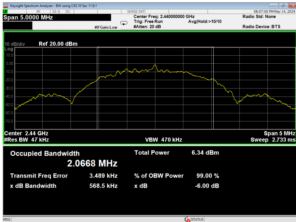
31 Occupied Bandwidth, Mid Channel, GMSK 2MB
