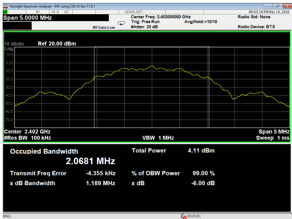
17 6dB Bandwidth, Low Channel, GMSK 2MB
