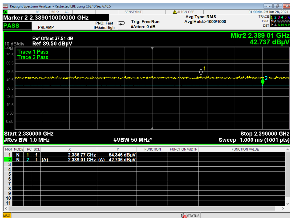
12 Lower Bandedge, Restricted, GMSK 1MB
