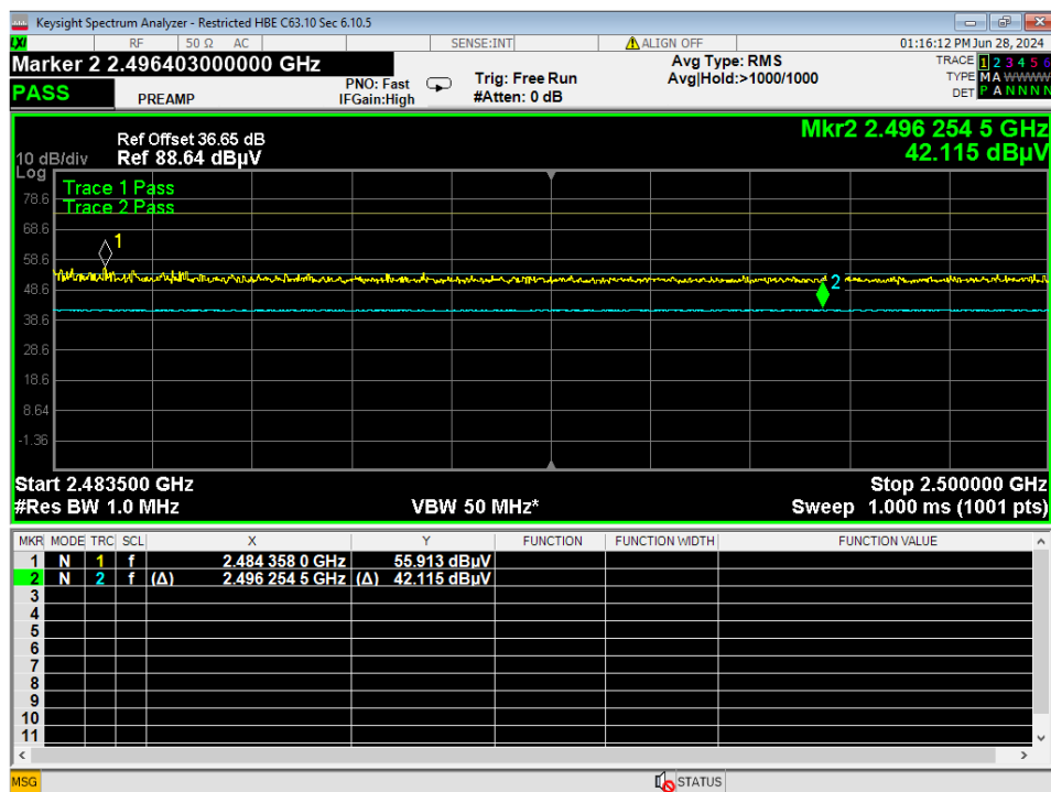
13 Higher Bandedge, Restricted, GMSK 1MB
