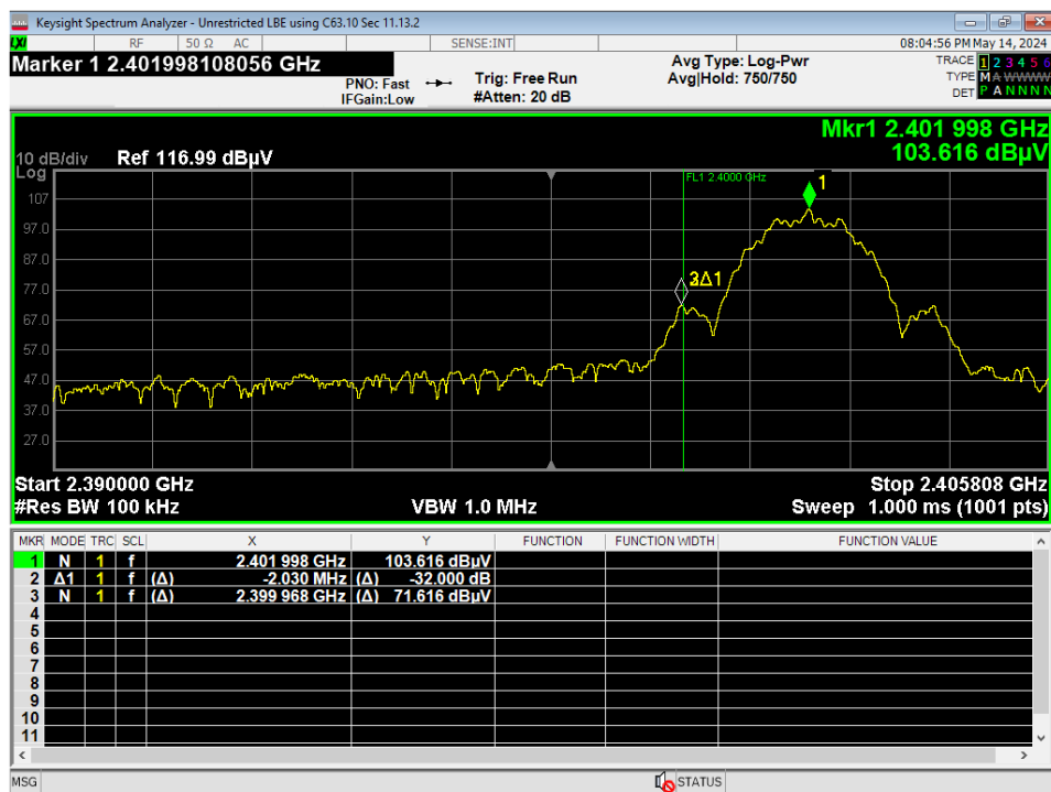
23 Lower Bandedge, Unrestricted, GMSK 2MB
