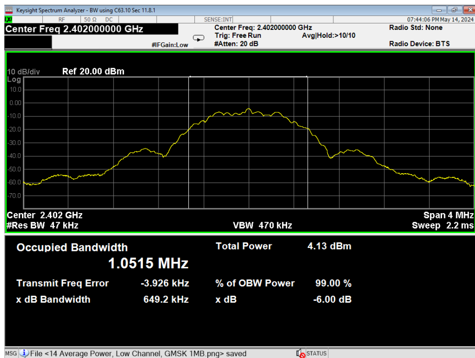
27 Occupied Bandwidth, Low Channel, GMSK 1MB
