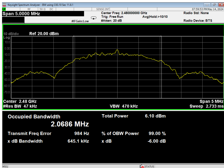
32 Occupied Bandwidth, High Channel, GMSK 2MB
