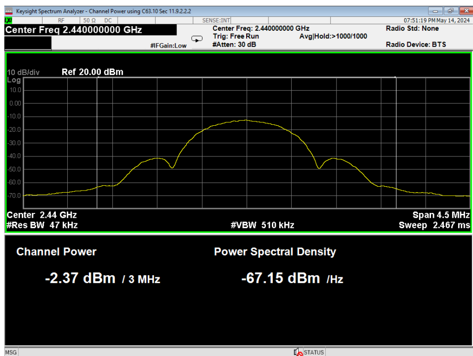
02 Average Power, Mid Channel, GMSK 1MB
