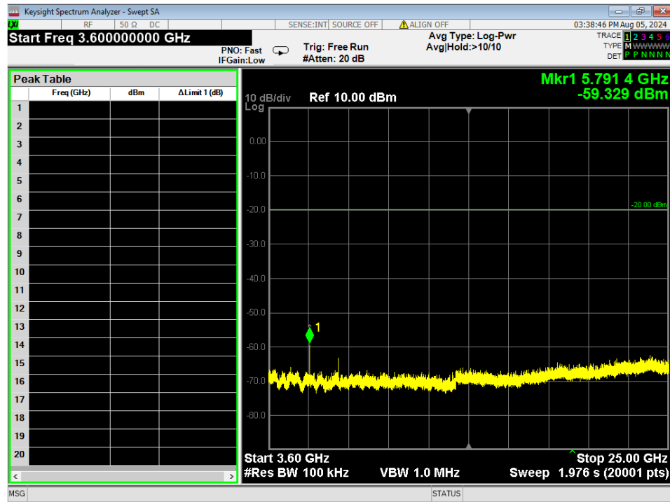
Figure 11 - Conducted Spurious emissions, GMSK 1MB, 3.6GHz – 25GHz, Mid
