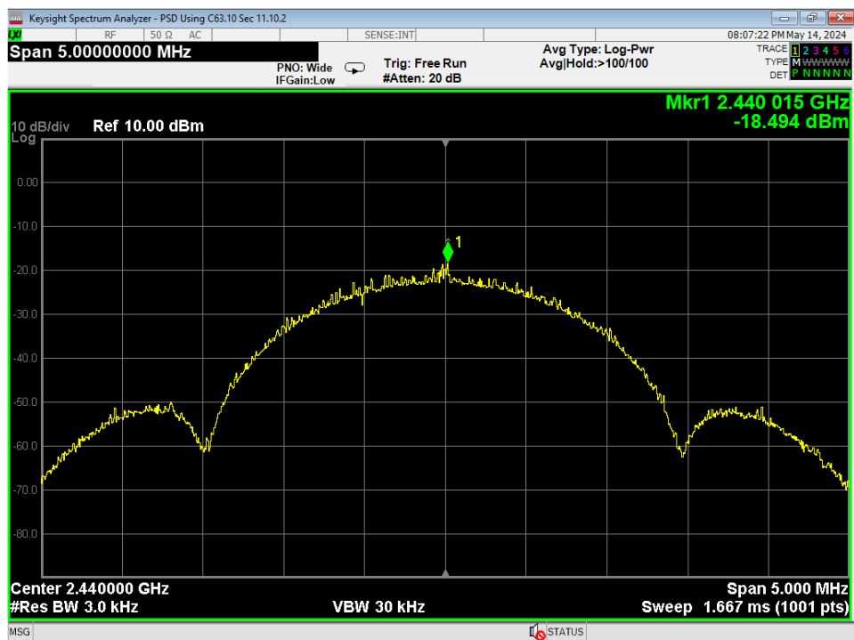
21 PSD, Mid Channel, GMSK 2MB
