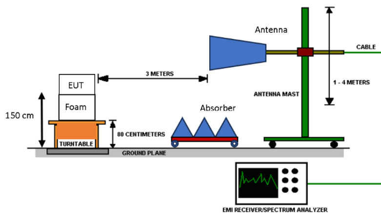
Figure 3 - Radiated Emissions Test Setup, >1GHz
