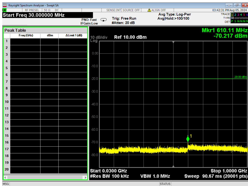
Figure 9 - Conducted Spurious emissions, GMSK 1MB, 30MHz – 1GHz, Mid
