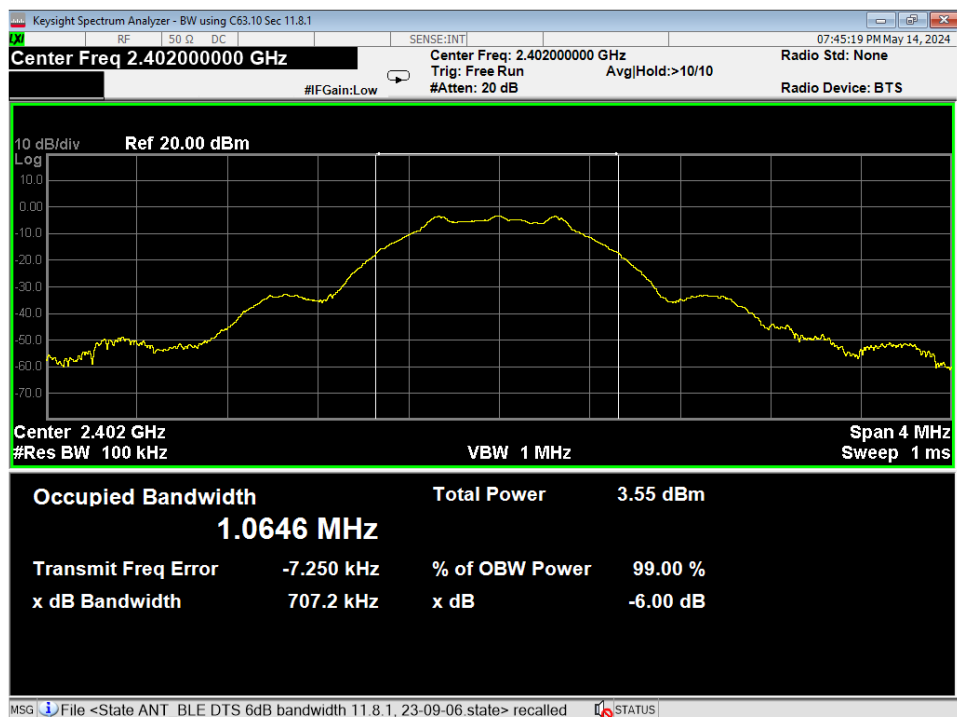
04 6dB Bandwidth, Low Channel, GMSK 1MB
