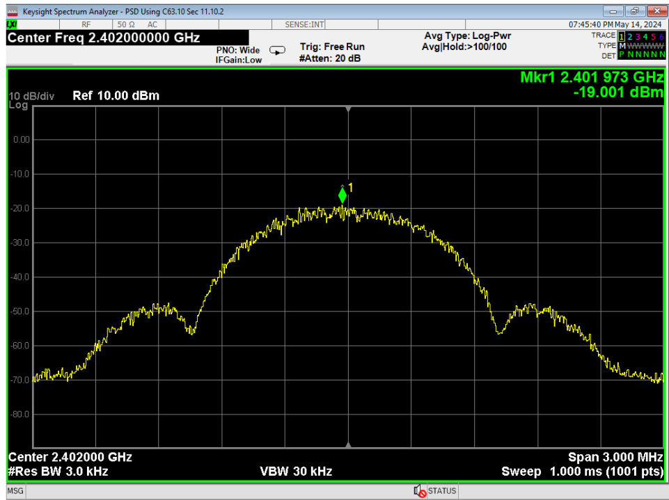
07 PSD, Low Channel, GMSK 1MB
