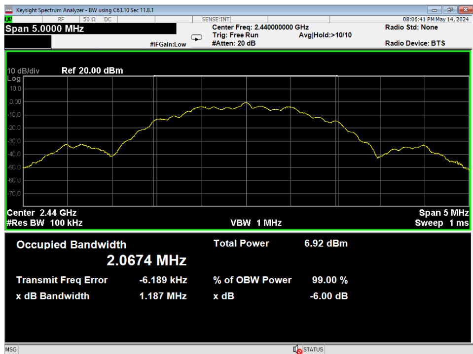
18 6dB Bandwidth, Mid Channel, GMSK 2MB
