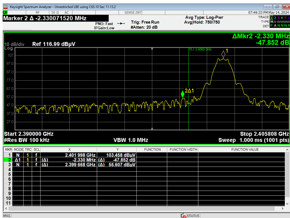
10 Lower Bandedge, Unrestricted, GMSK 1MB
