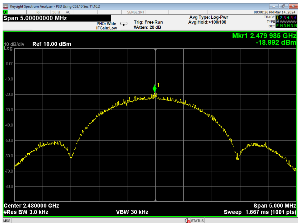
22 PSD, High Channel, GMSK 2MB
