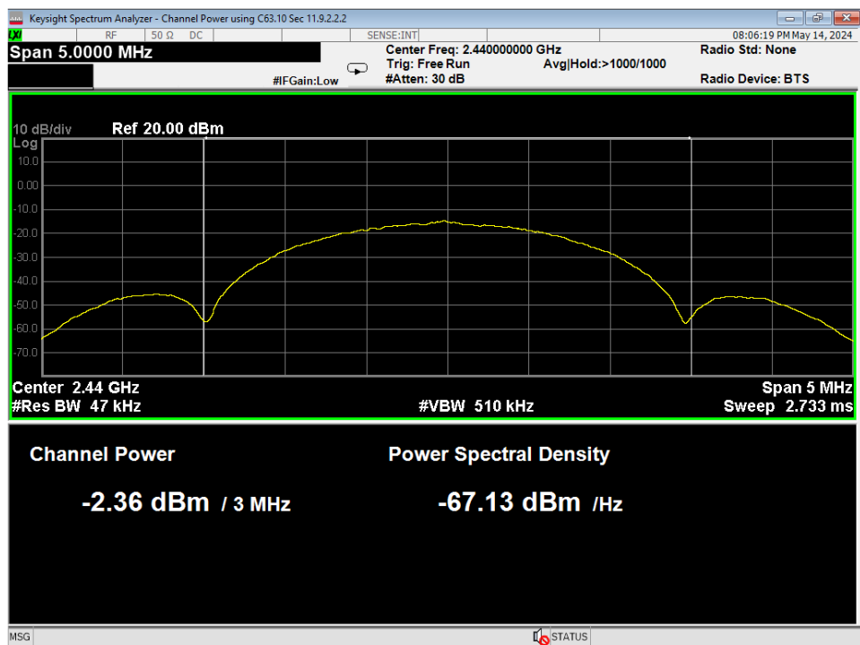
15 Average Power, Mid Channel, GMSK 2MB
