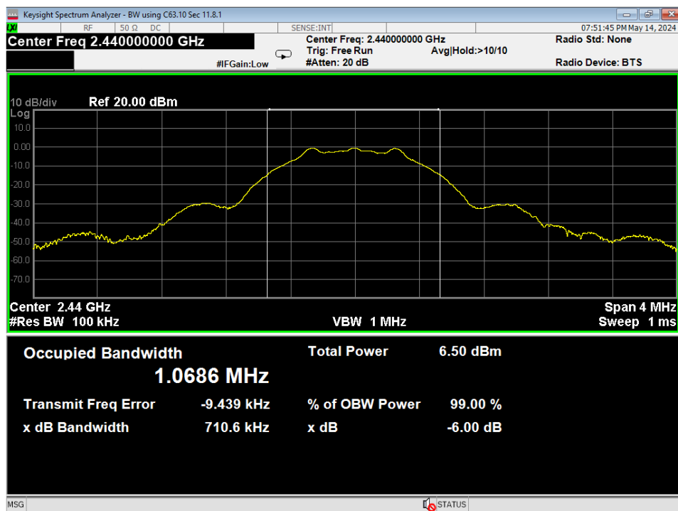
05 6dB Bandwidth, Mid Channel, GMSK 1MB
