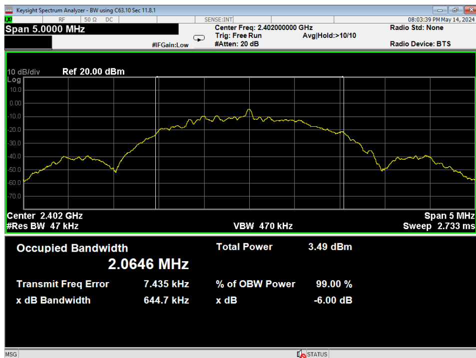
30 Occupied Bandwidth, Low Channel, GMSK 2MB
