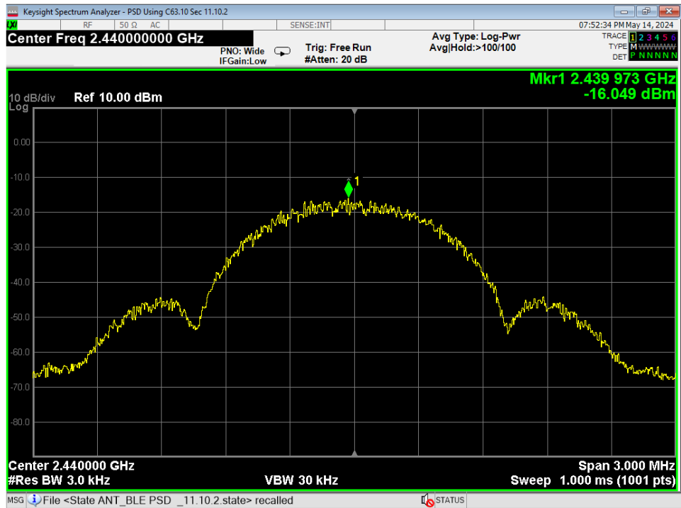
08 PSD, Mid Channel, GMSK 1MB
