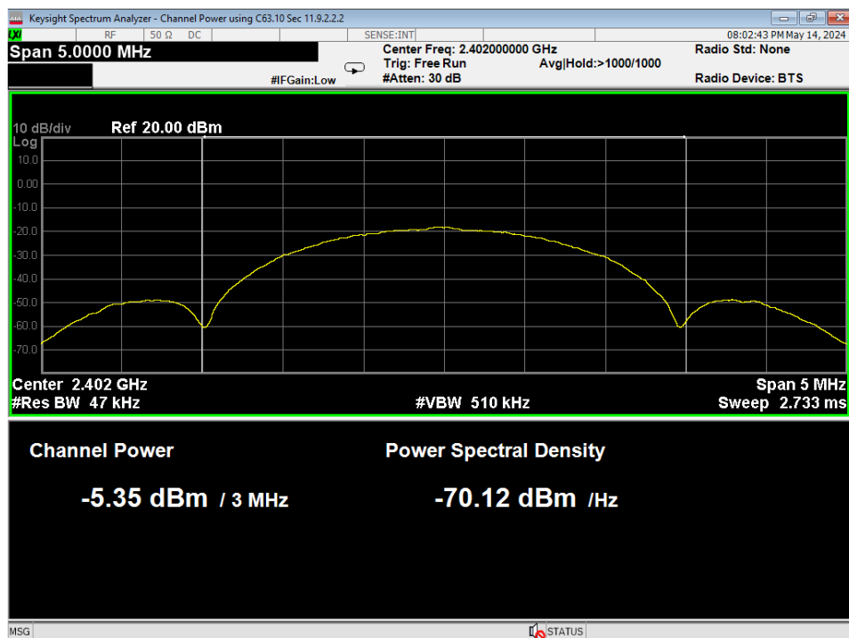
14 Average Power, Low Channel, GMSK 2MB
