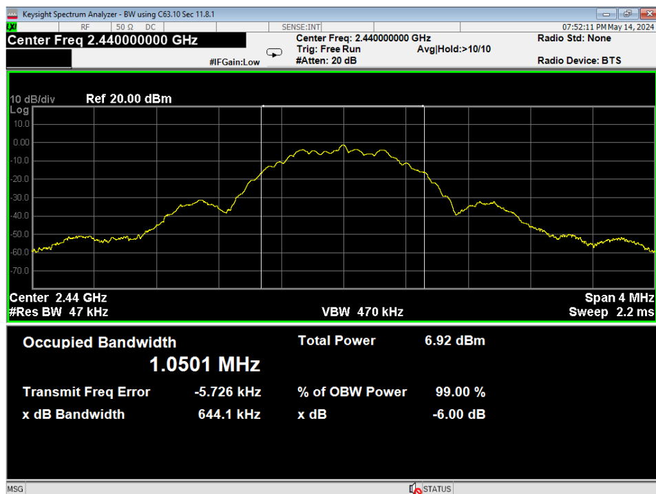
28 Occupied Bandwidth, Mid Channel, GMSK 1MB
