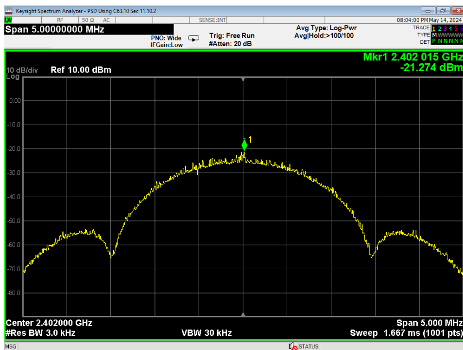
20 PSD, Low Channel, GMSK 2MB
