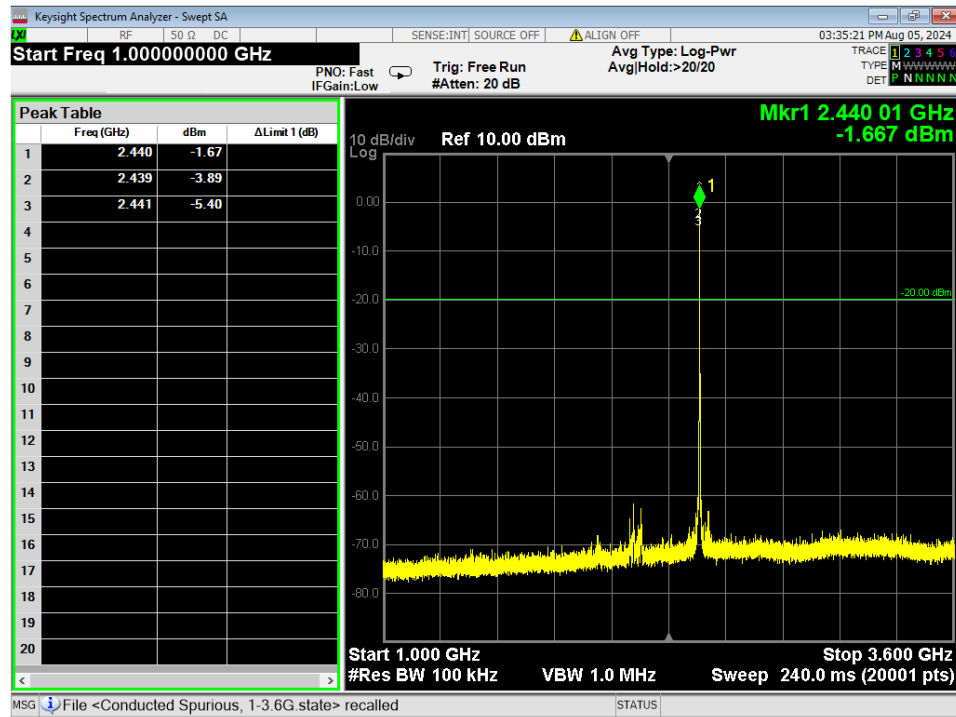
Figure 13 – Conducted Spurious emissions, GMSK 2MB, 1GHz – 3.6GHz, Mid
