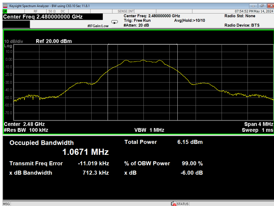
06 6dB Bandwidth, High Channel, GMSK 1MB
