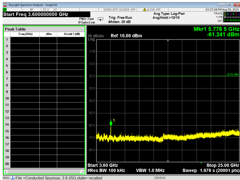
Figure 14 - Conducted Spurious emissions, GMSK 2MB, 3.6GHz – 25GHz, Mid
