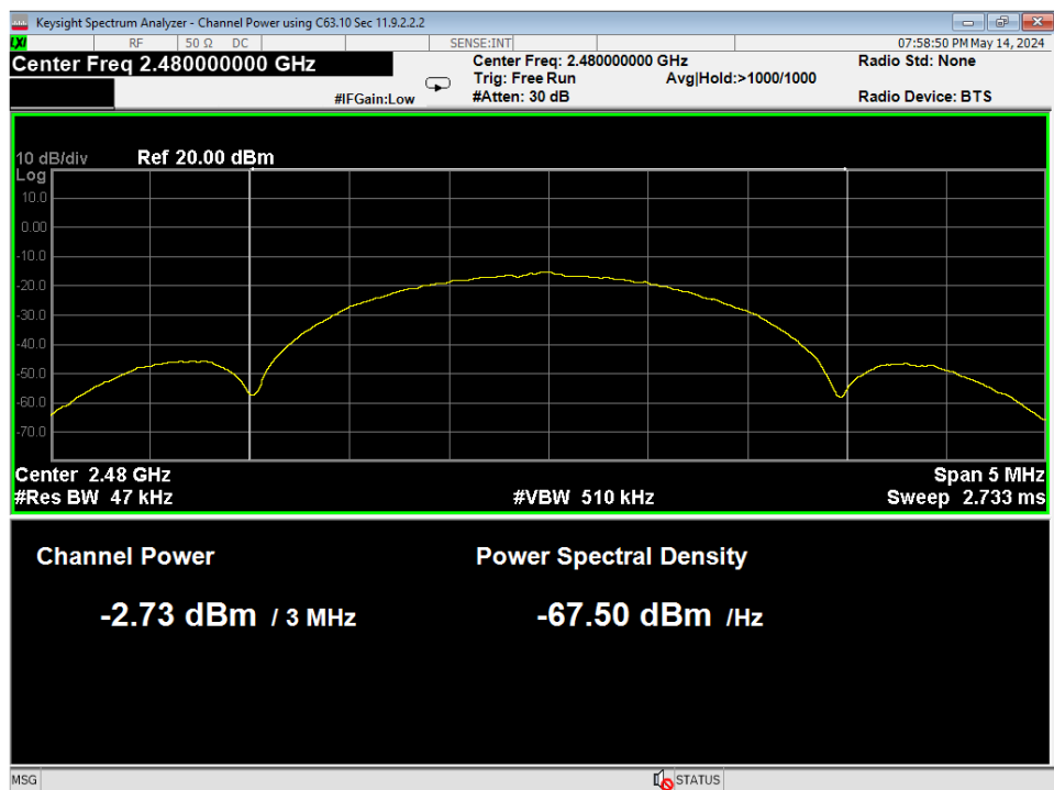
16 Average Power, High Channel, GMSK 2MB
