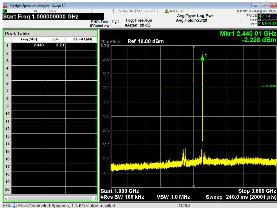
Figure 10 - Conducted Spurious emissions, GMSK 1MB, 1GHz – 3.6GHz, Mid
