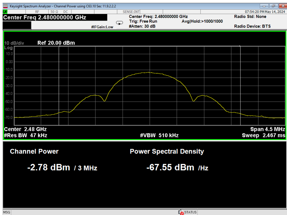
03 Average Power, High Channel, GMSK 1MB
