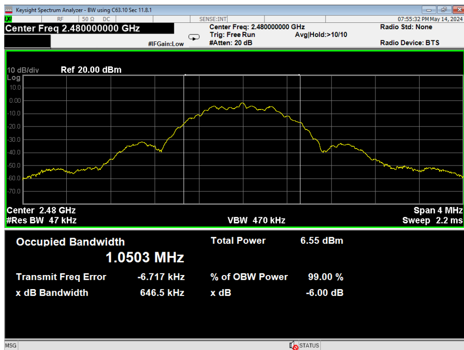
29 Occupied Bandwidth, High Channel, GMSK 1MB
