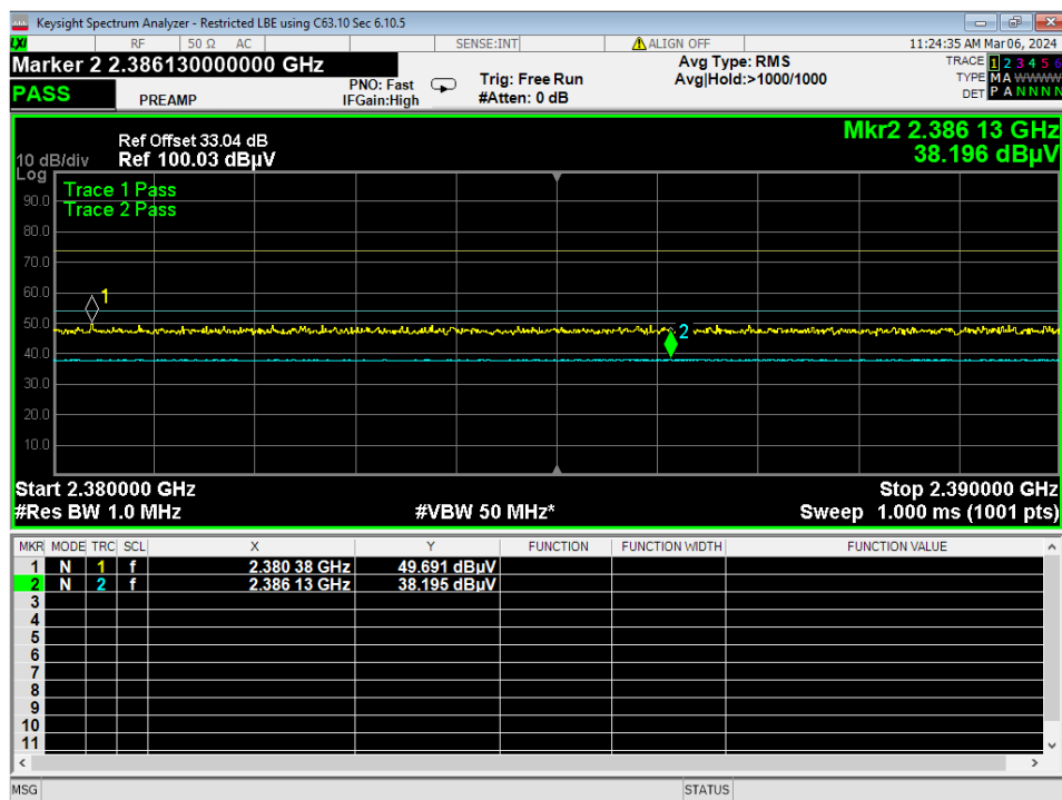
25 Lower Bandedge, Restricted, GMSK 2MB
