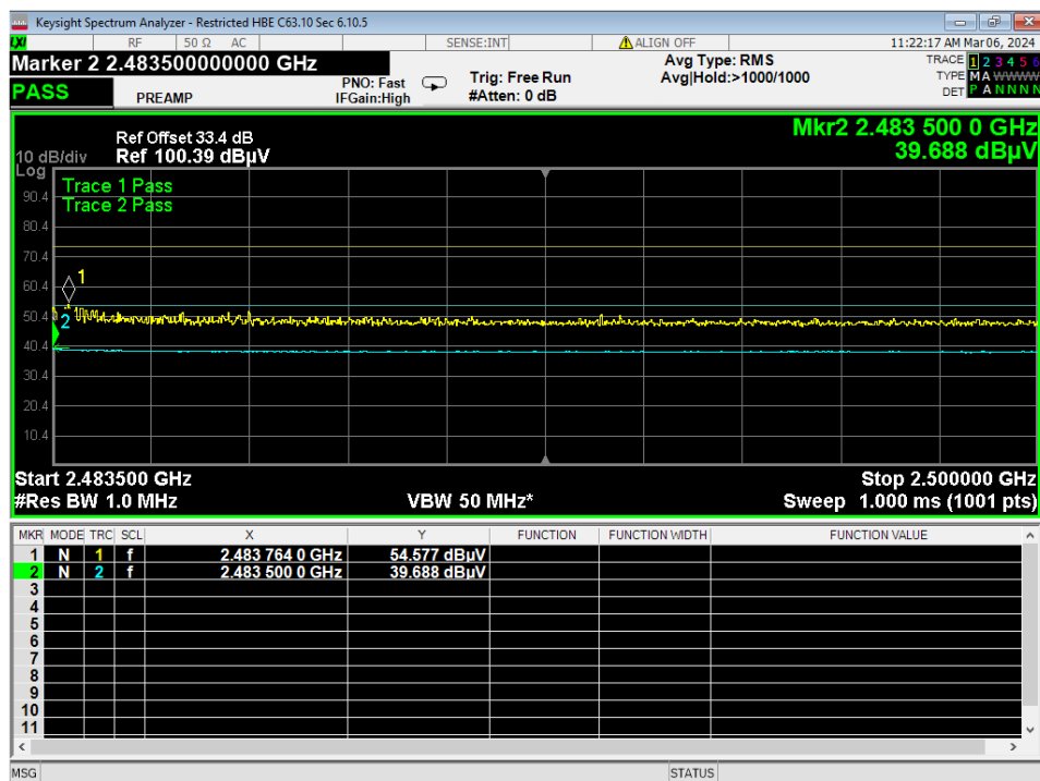
26 Higher Bandedge, Restricted, GMSK 2MB
