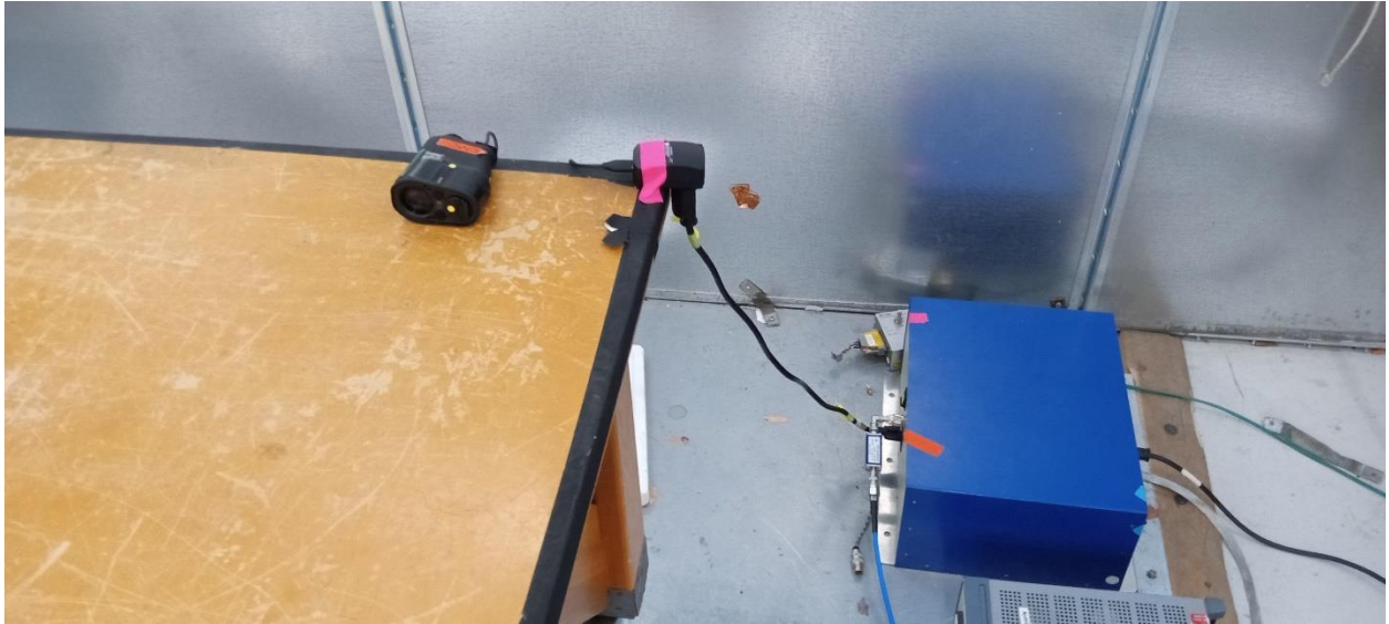
Conducted Emissions
