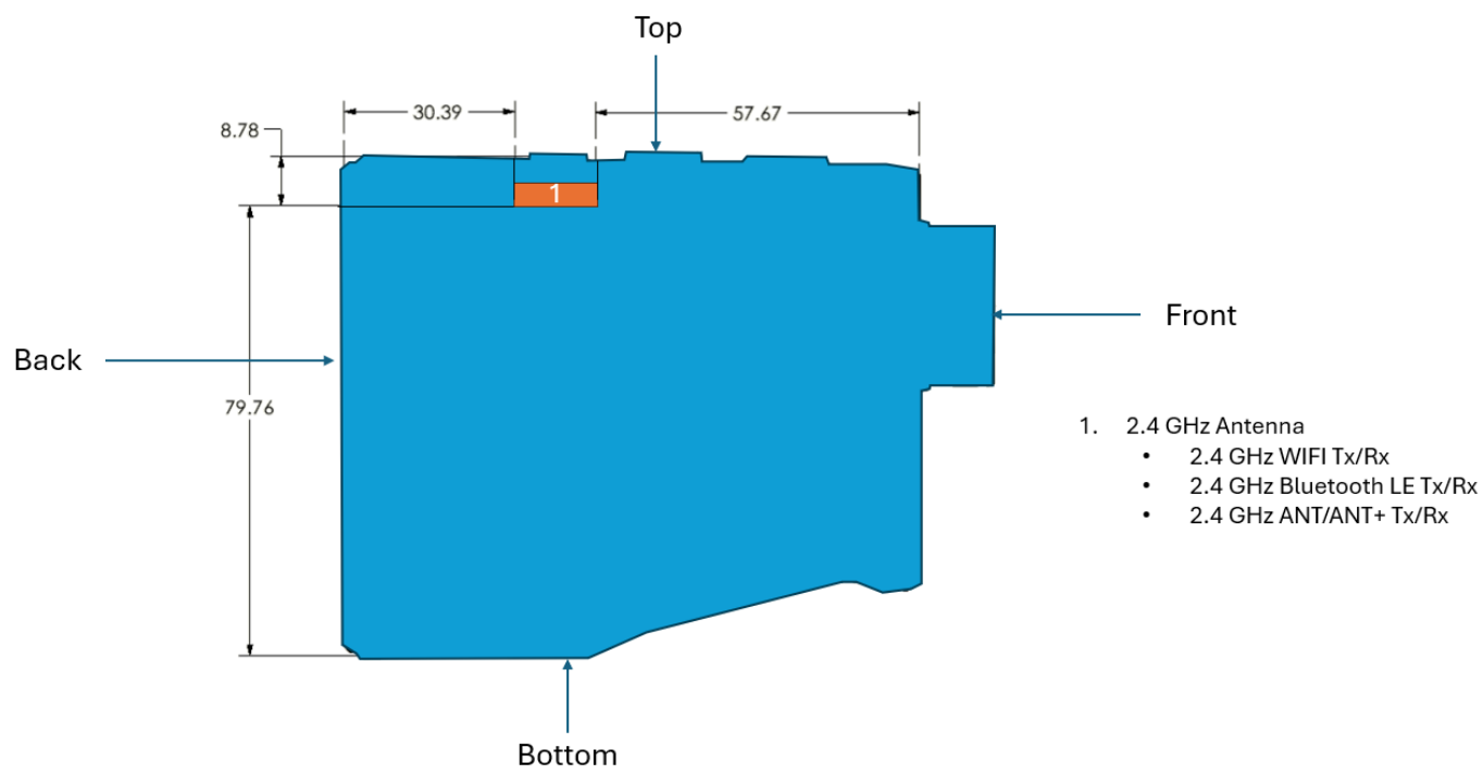
Figure A DUT Antenna Diagram
