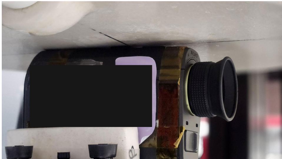
Figure C SAR Test Setup – Body/Extremity – Top 0mm
