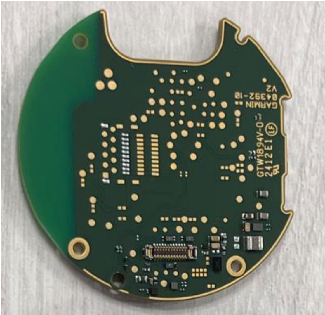
Photograph 6-2 : Back side view of the main board
