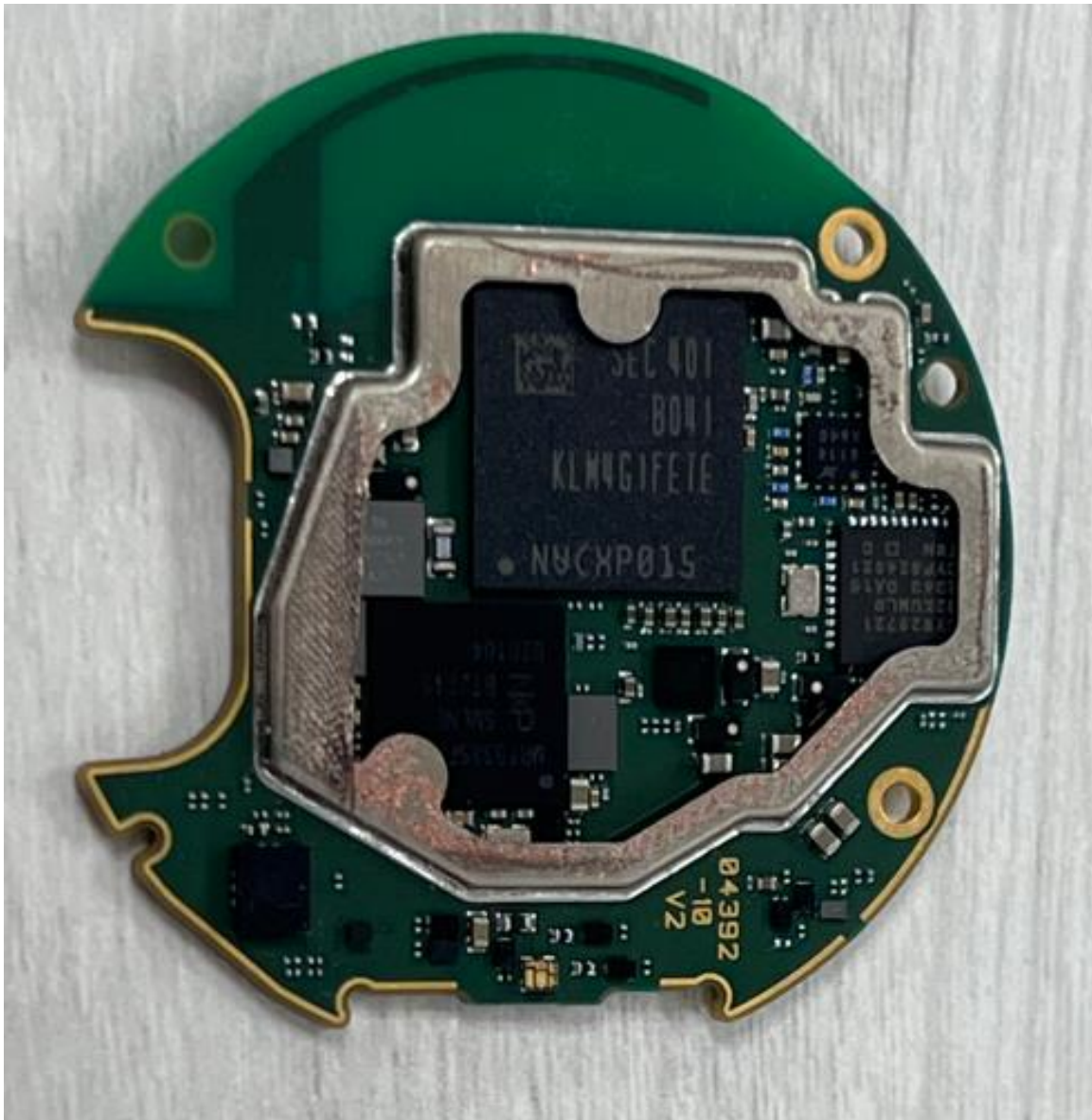
Photograph 6-3 : Front side view of the main board, shields removed
