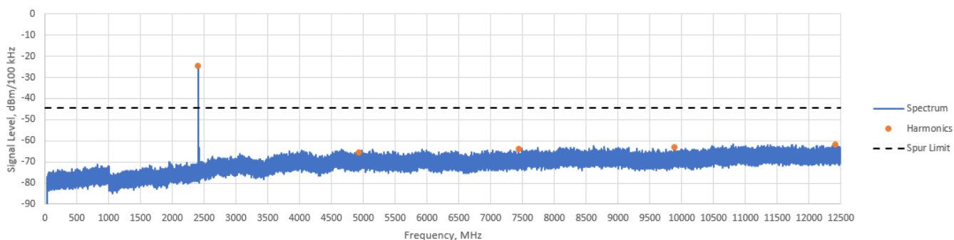
Figure TR34.1: Spectral data, 30 MHz to 12.5 GHz
