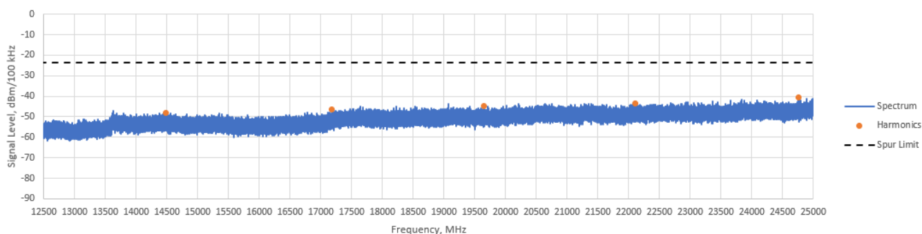
Figure TR32.2: Spectral data, 12.5 GHz to 25 GHz
