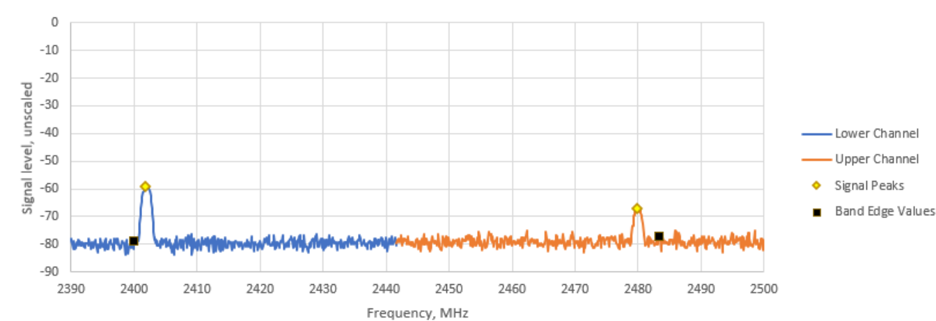
Figure TR26.4: Measured data for BLE at 10.2 Vdc
