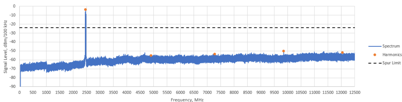
Figure TR32.1: Spectral data, 30 MHz to 12.5 GHz
