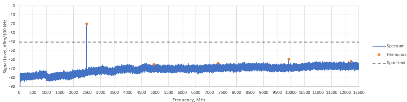
Figure TR33.1: Spectral data, 30 MHz to 12.5 GHz
