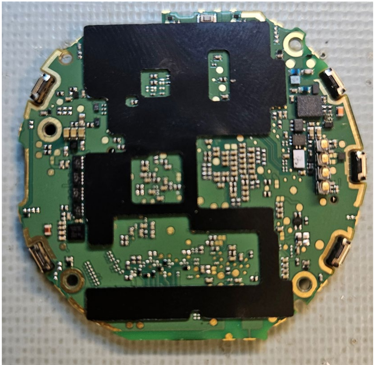
Bottom side – Insulation on
