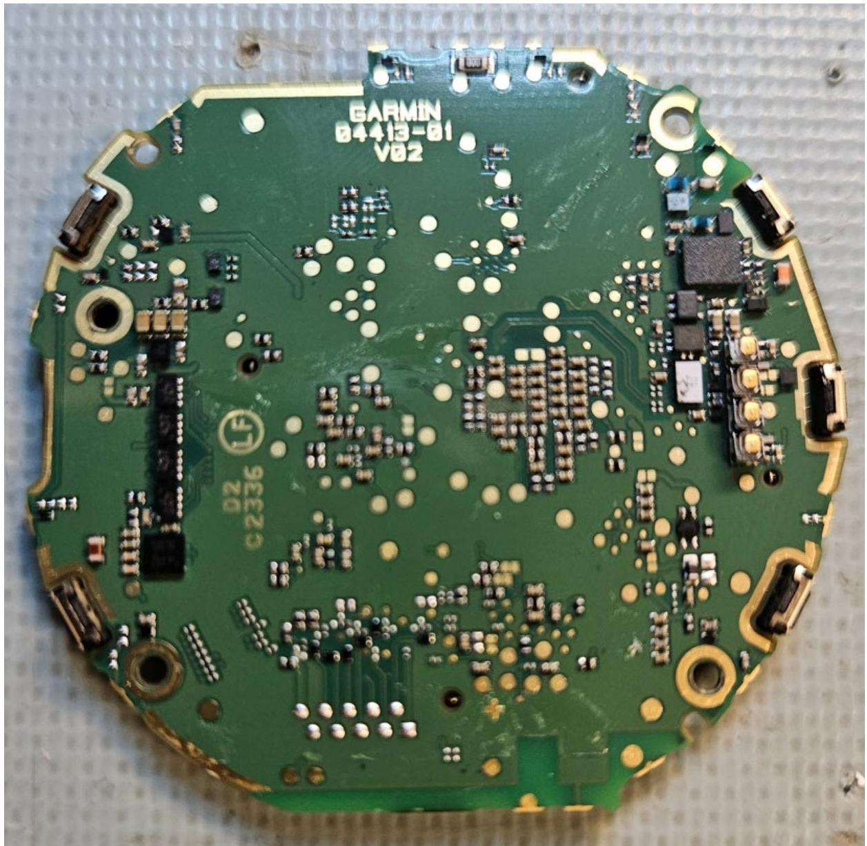
Bottom side of PCB
