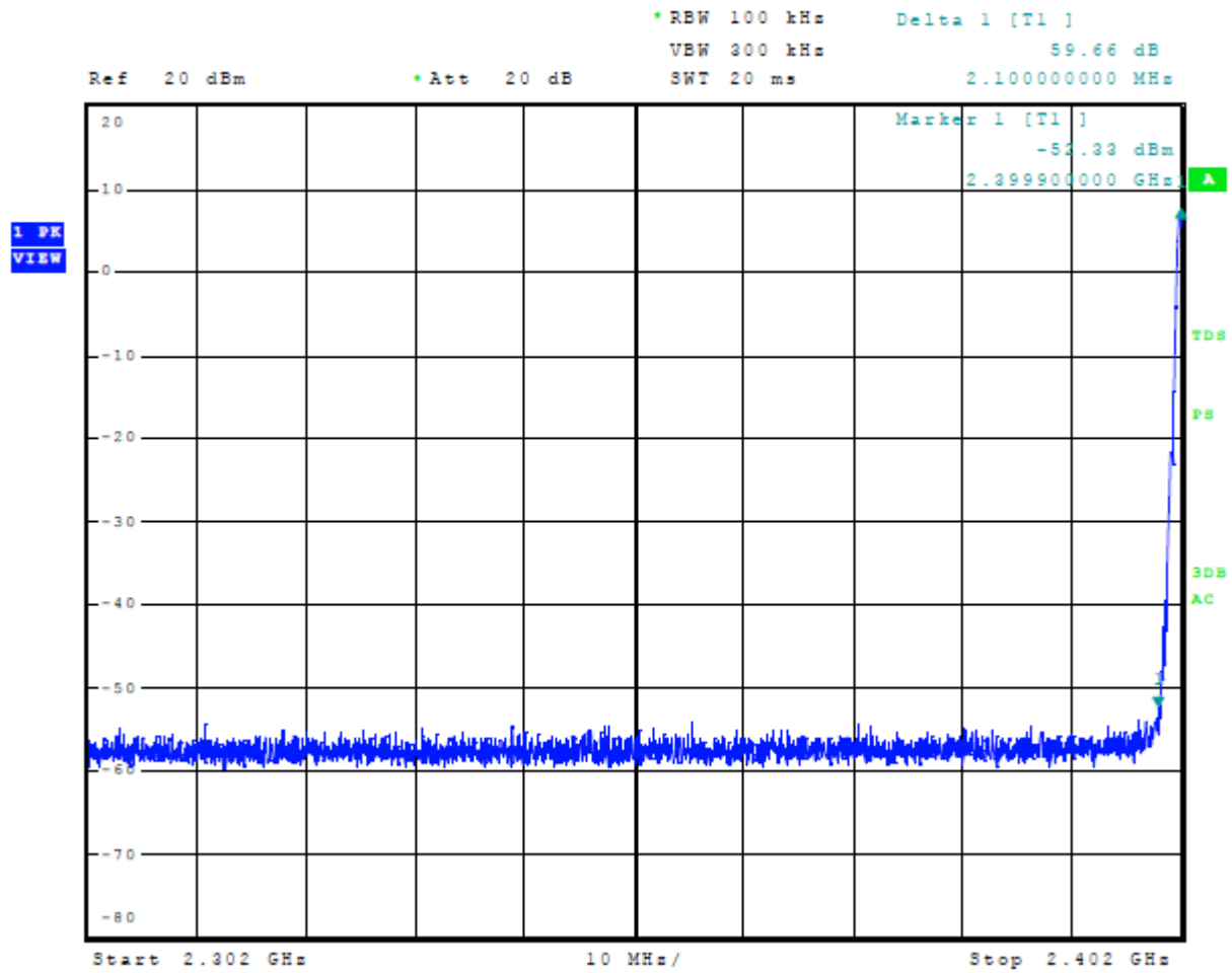
Figure 9 Plot of Emissions Low Band Edge Mode 5, BT BLE
