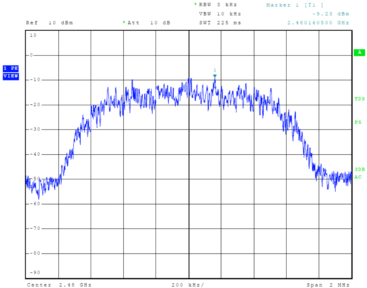
Figure 31 Plot of Transmitter Power Spectral Density Mode 3, BT 2EDR
