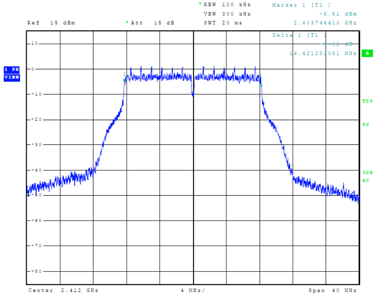
Figure 27 Plot of 6-dB Occupied Bandwidth Mode 7, 802.11g
