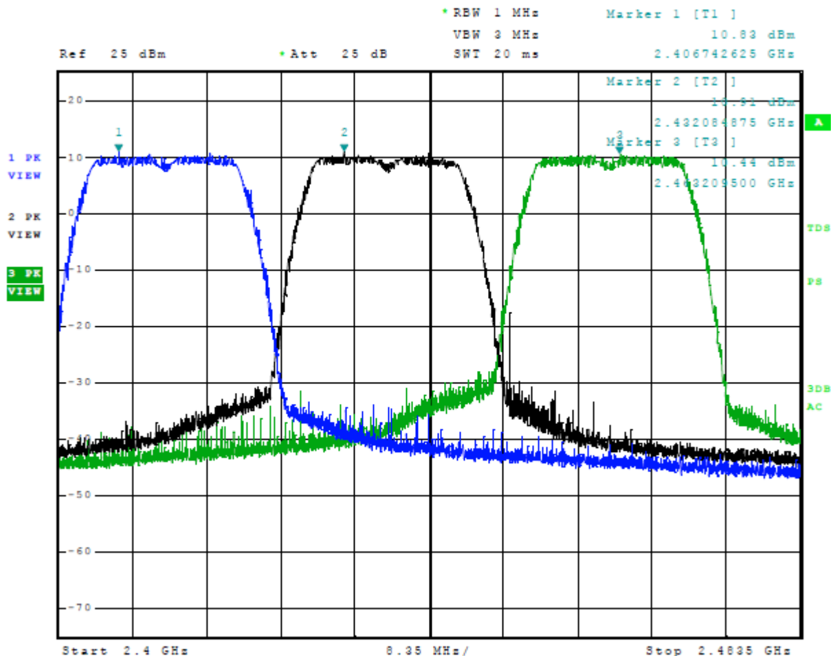
Figure 6 Plot of Transmitter Operation in 2402-2480 MHz Mode 8, 802.11n
