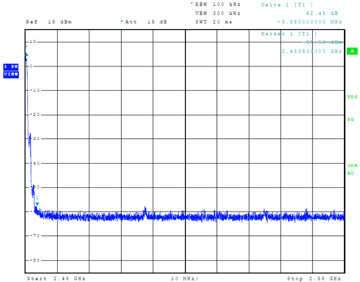
Figure 13 Plot of Transmitter Emissions High Band Edge Mode 3, BT 2EDR
