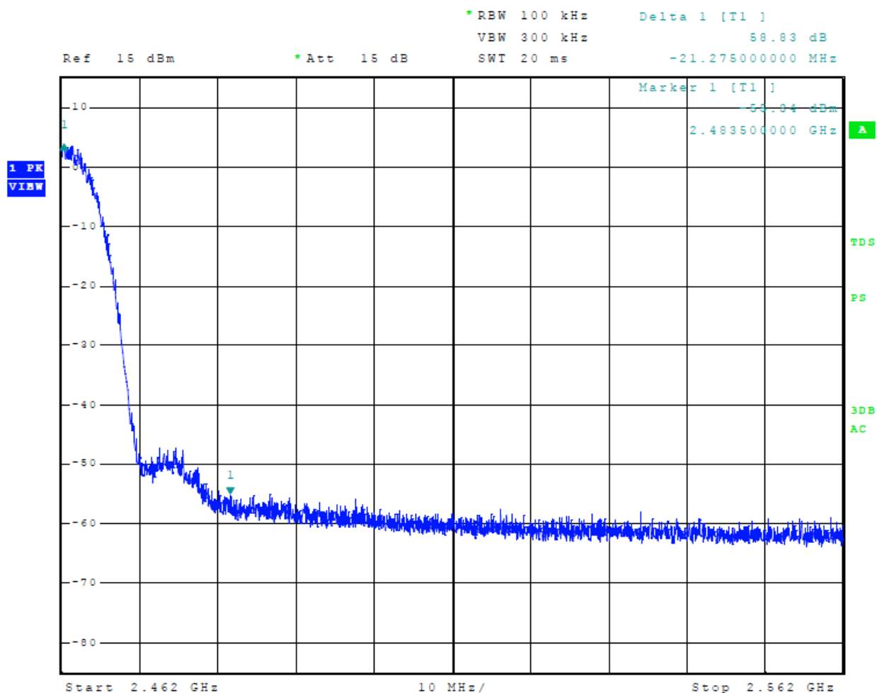
Figure 16 Plot of Transmitter Emissions High Band Edge Mode 6, 802.11b
