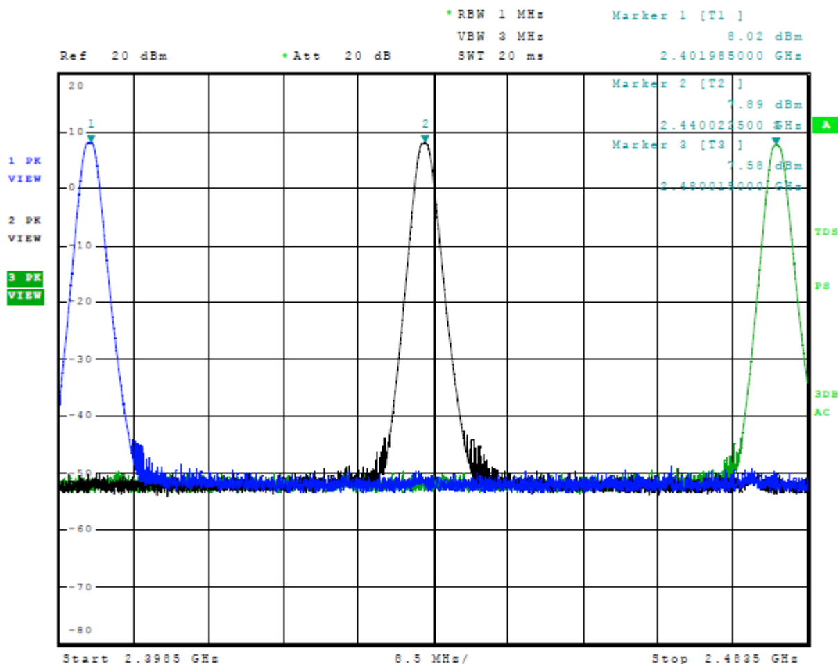
Figure 3 Plot of Transmitter Operation in 2402-2480 MHz Mode 5, BT BLE
