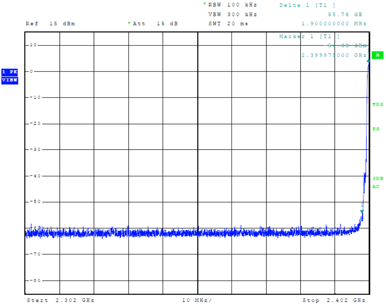
Figure 7 Plot of Emissions Low Band Edge Mode 3, BT 2EDR
