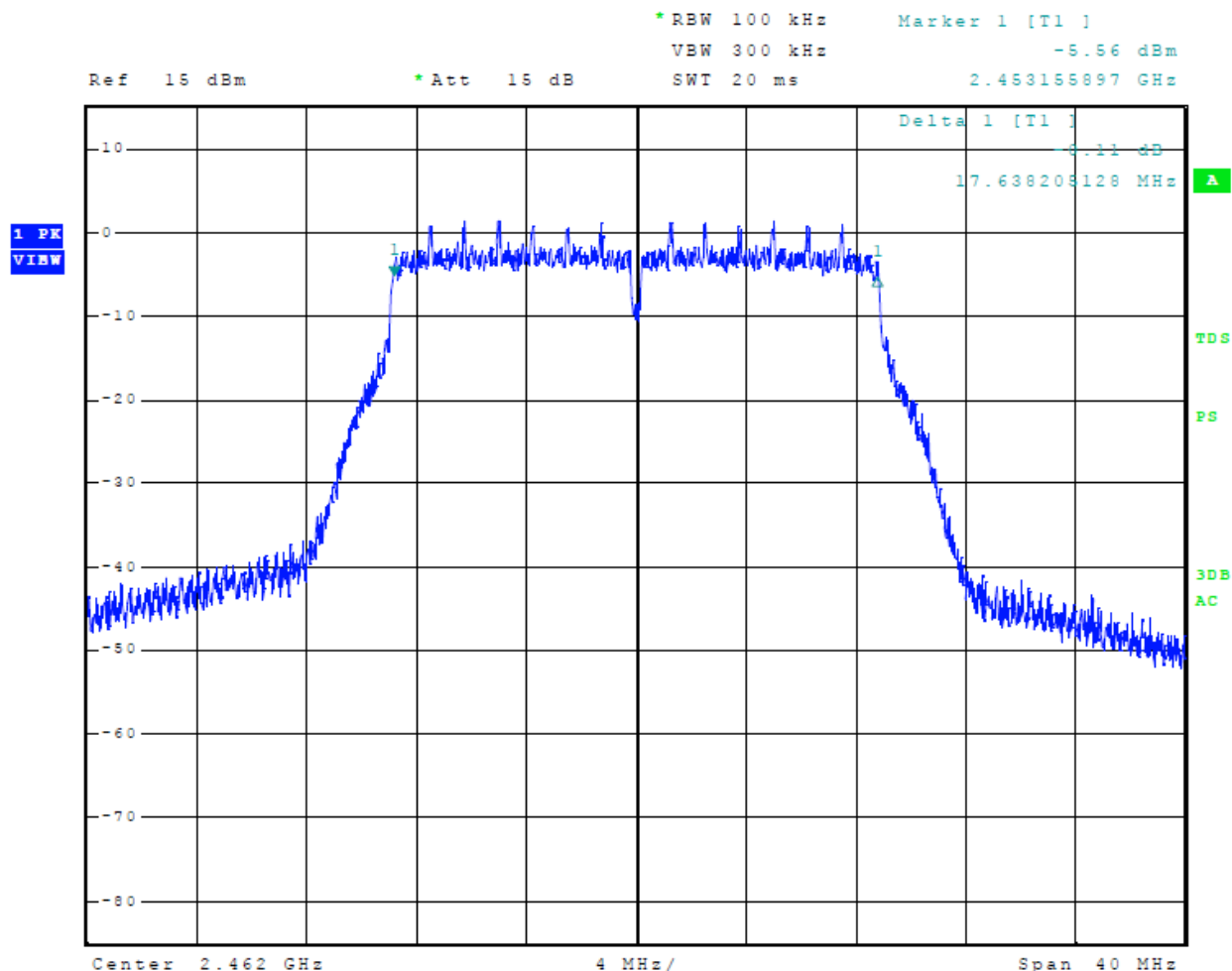
Figure 29 Plot of 6-dB Occupied Bandwidth Mode 8, 802.11n
