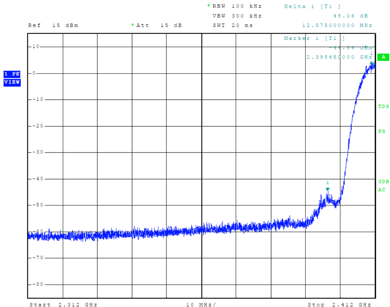
Figure 10 Plot of Emissions Low Band Edge Mode 6, 802.11b
