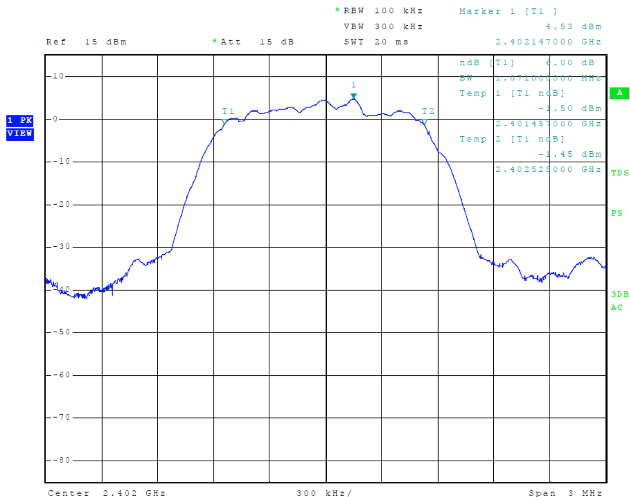
Figure 21 Plot of 6-dB Occupied Bandwidth Mode 4, BT 3EDR
