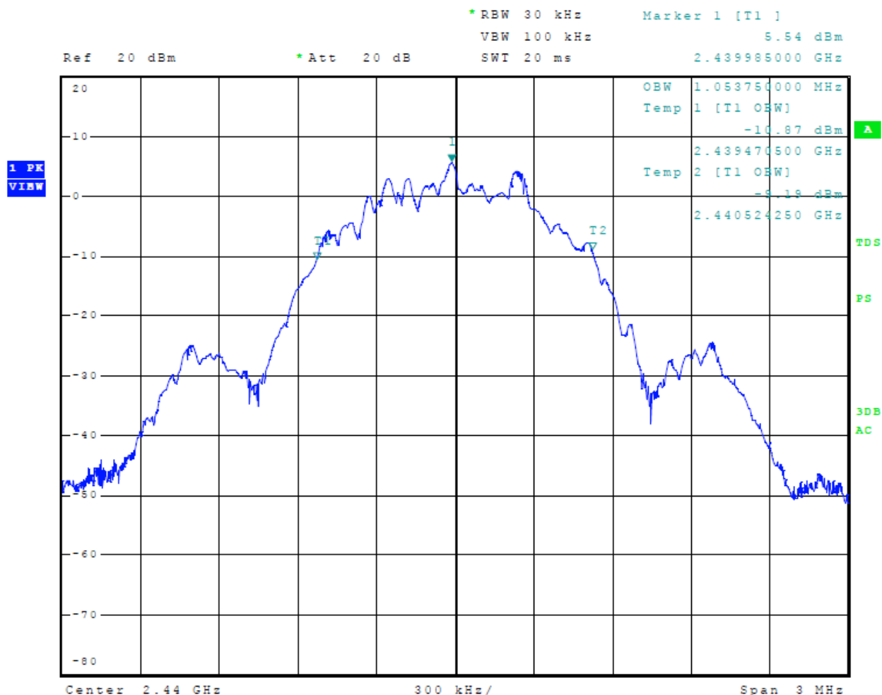
Figure 24 Plot of 99% Occupied Bandwidth Mode 5, BT BLE
