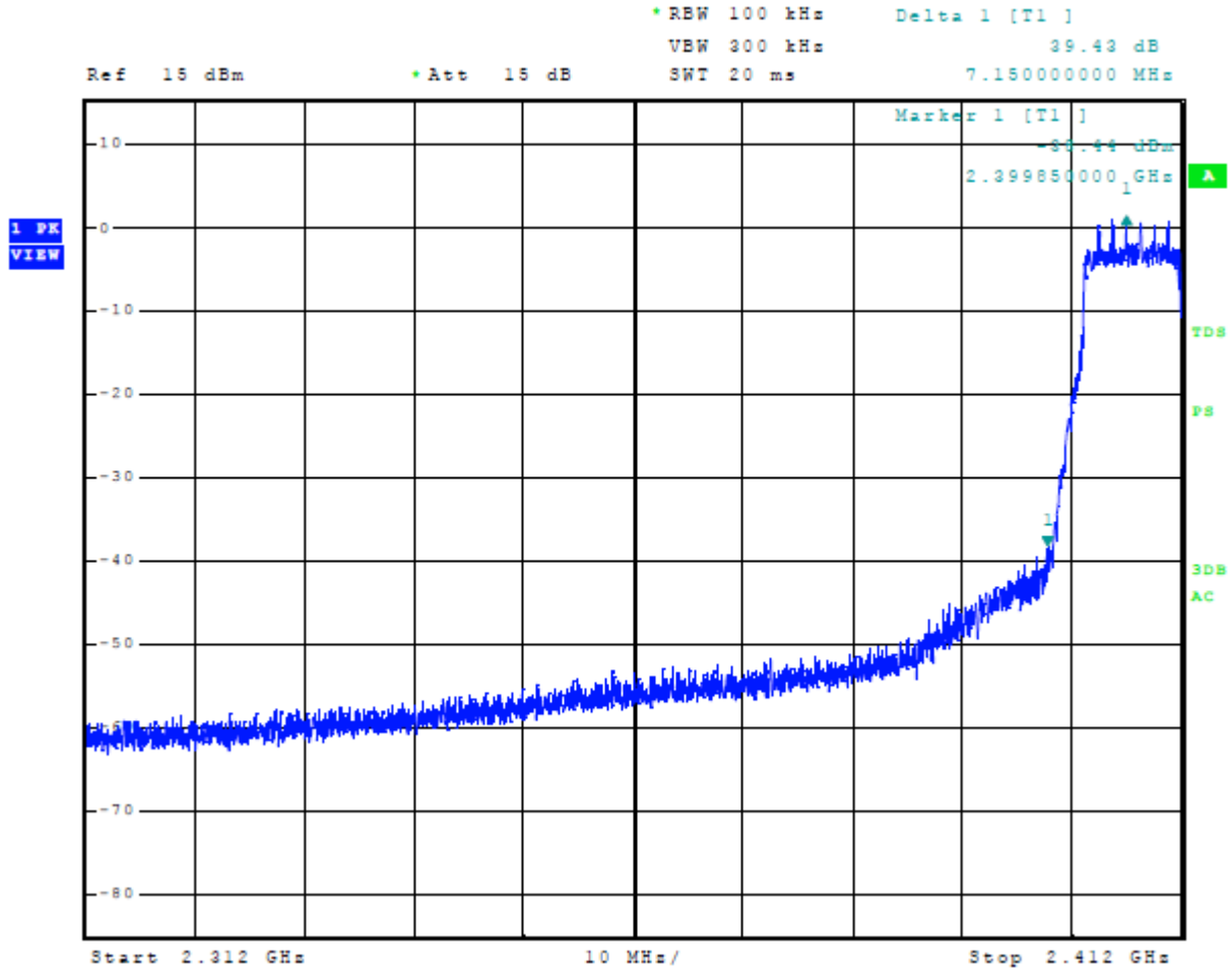
Figure 12 Plot of Emissions Low Band Edge Mode 8, 802.11n
