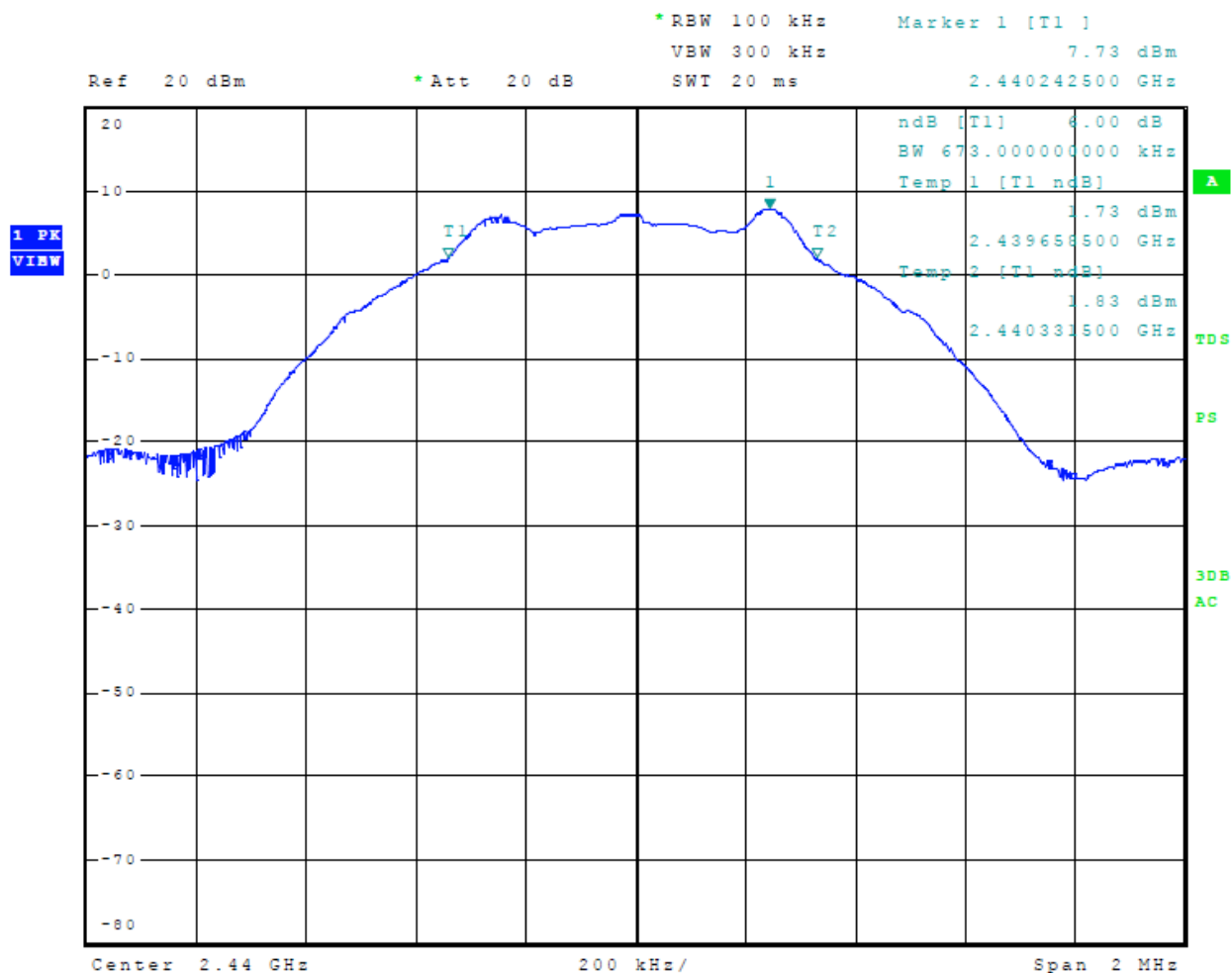
Figure 23 Plot of 6-dB Occupied Bandwidth Mode 5, BT BLE
