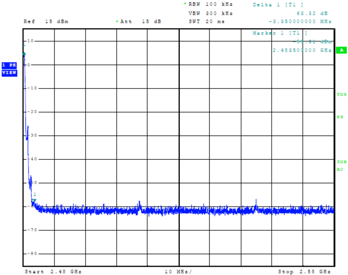
Figure 14 Plot of Transmitter Emissions High Band Edge Mode 4, BT 3EDR
