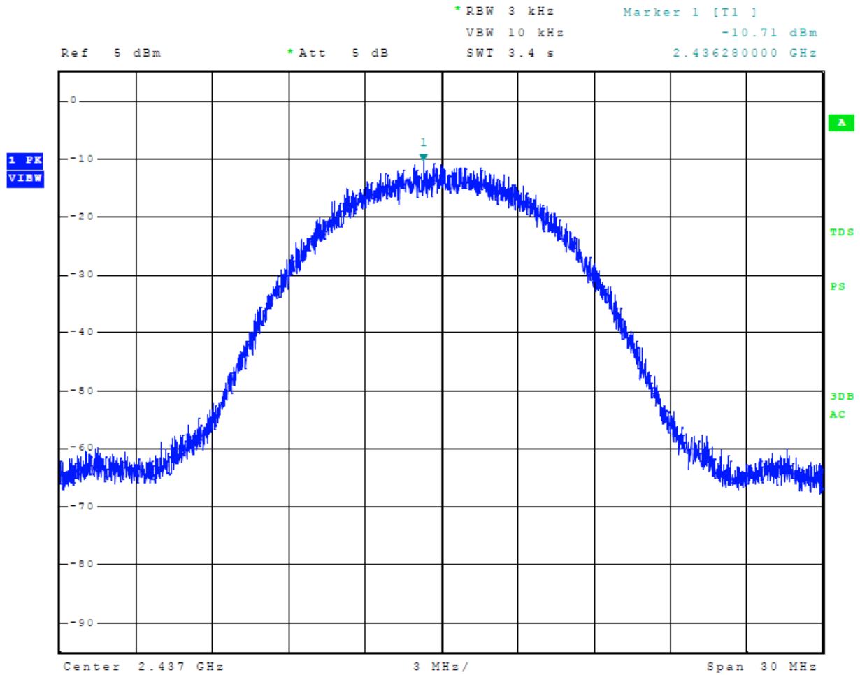
Figure 34 Plot of Transmitter Power Spectral Density Mode 6, 802.11b
