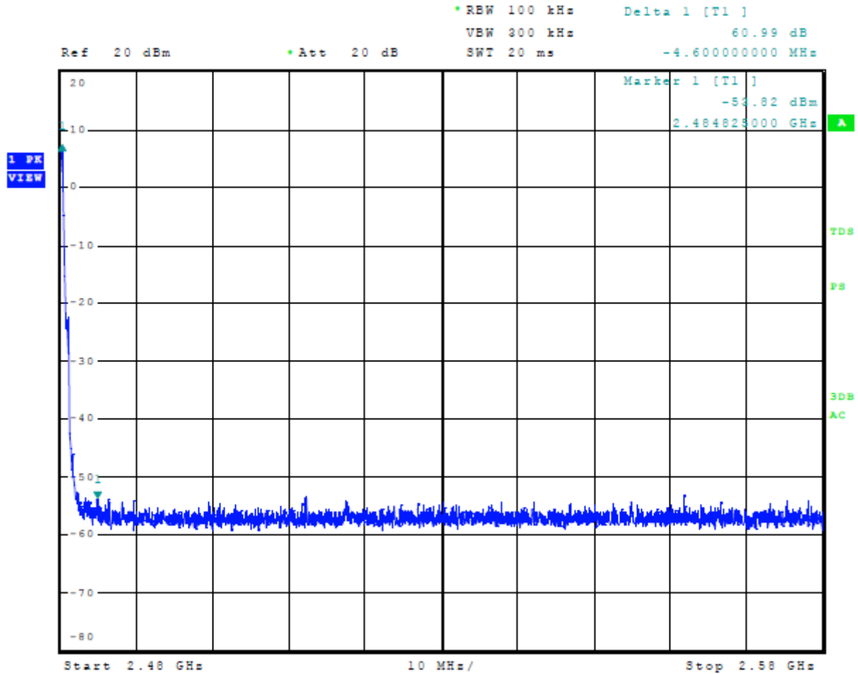
Figure 15 Plot of Transmitter Emissions High Band Edge Mode 5, BT BLE
