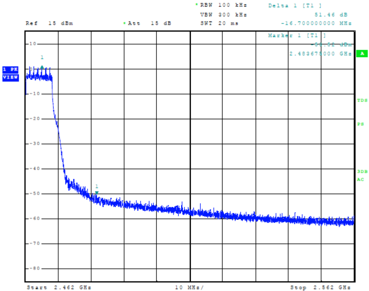
Figure 17 Plot of Transmitter Emissions High Band Edge Mode 7, 802.11g
