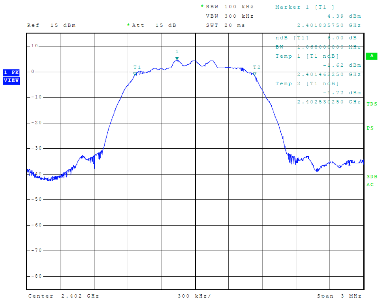
Figure 19 Plot of 6-dB Occupied Bandwidth Mode 3, BT 2EDR
