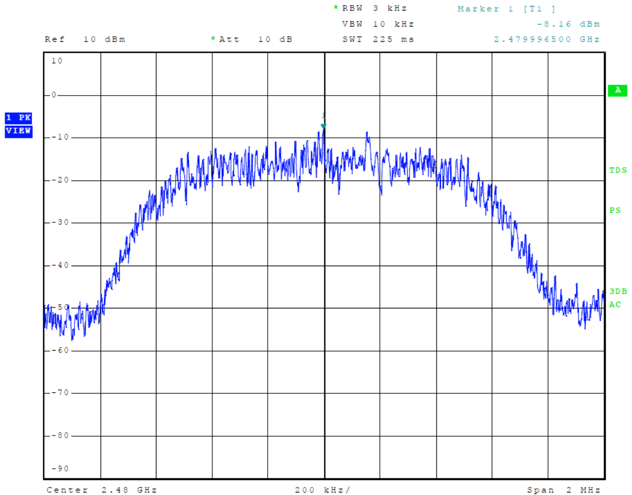
Figure 32 Plot of Transmitter Power Spectral Density Mode 4, BT 3EDR
