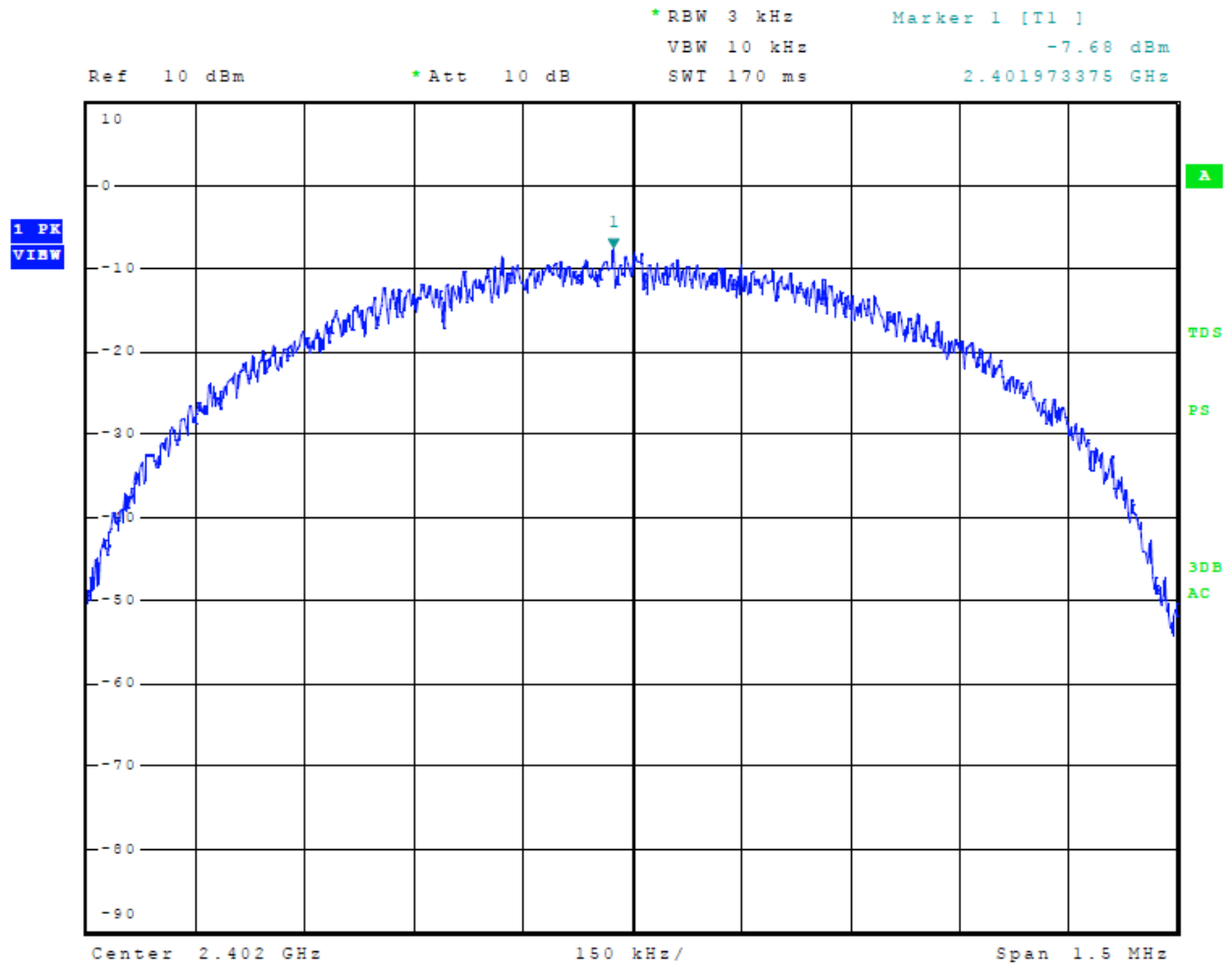
Figure 33 Plot of Transmitter Power Spectral Density Mode 5, BT BLE
