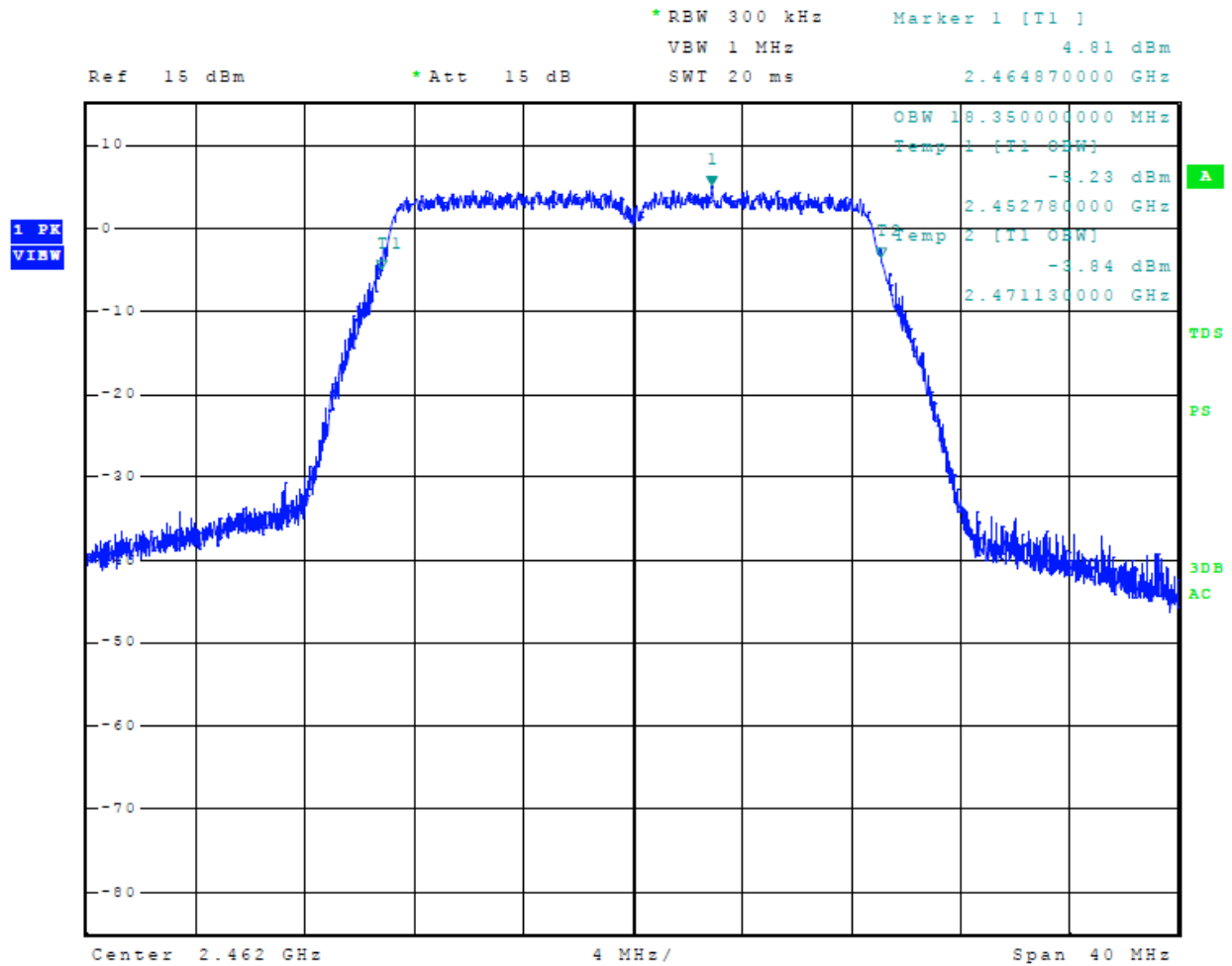
Figure 30 Plot of 99% Occupied Bandwidth Mode 8, 802.11n
