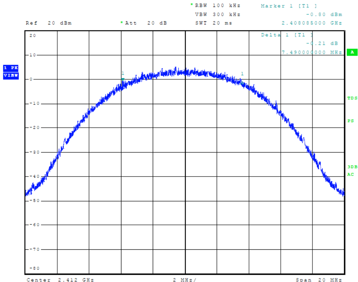
Figure 25 Plot of 6-dB Occupied Bandwidth Mode 6, 802.11b
