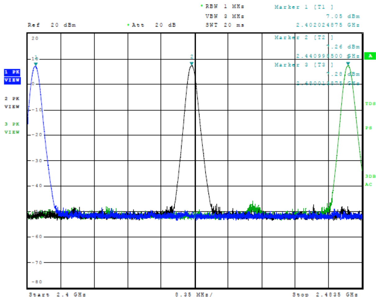
Figure 2 Plot of Transmitter Operation in 2402-2480 MHz Mode 4, BT 3EDR
