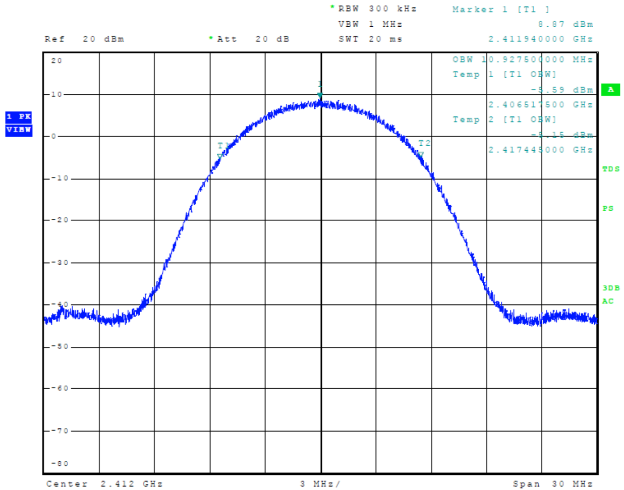
Figure 26 Plot of 99% Occupied Bandwidth Mode 6, 802.11b
