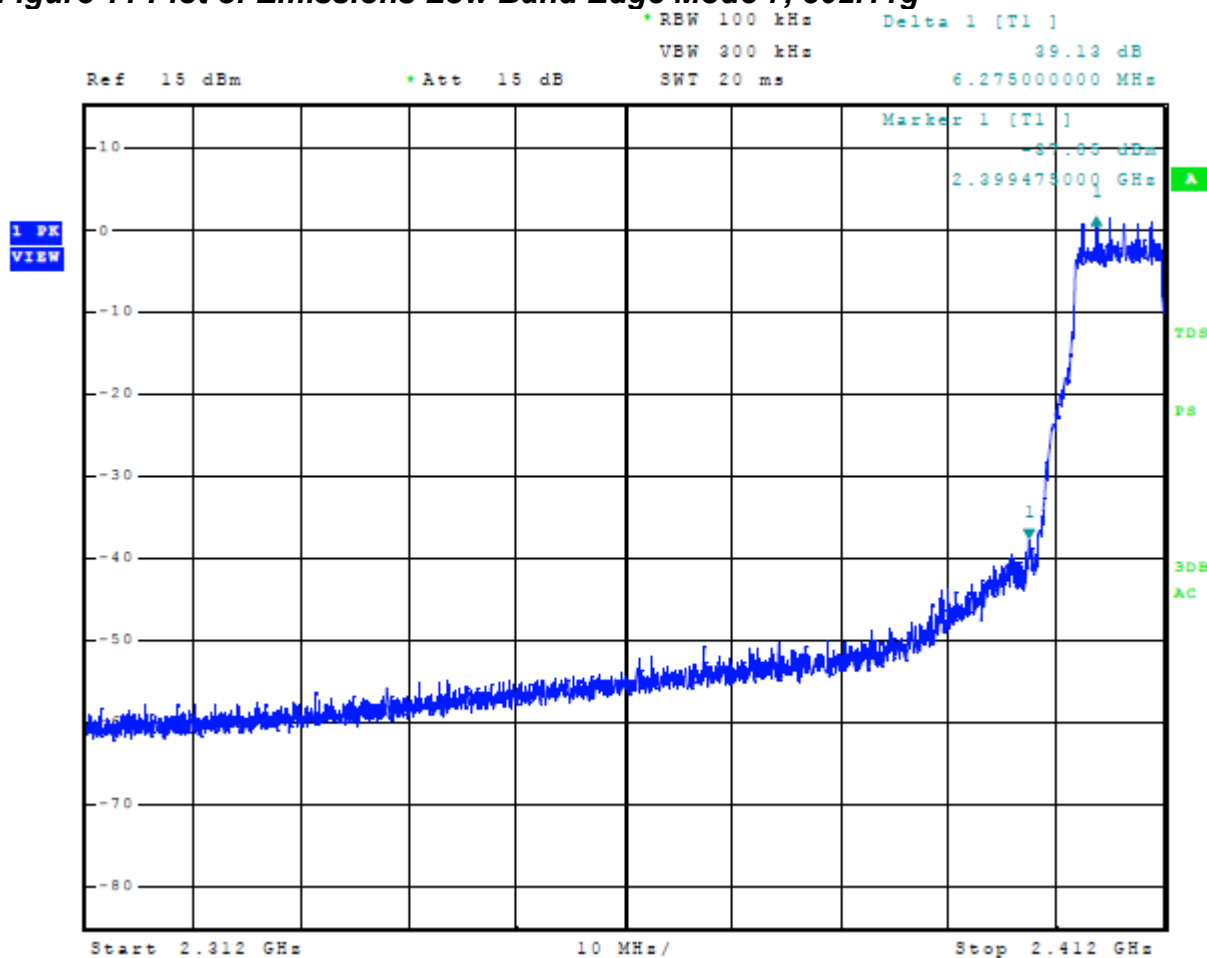
Figure 11 Plot of Emissions Low Band Edge Mode 7, 802.11g
