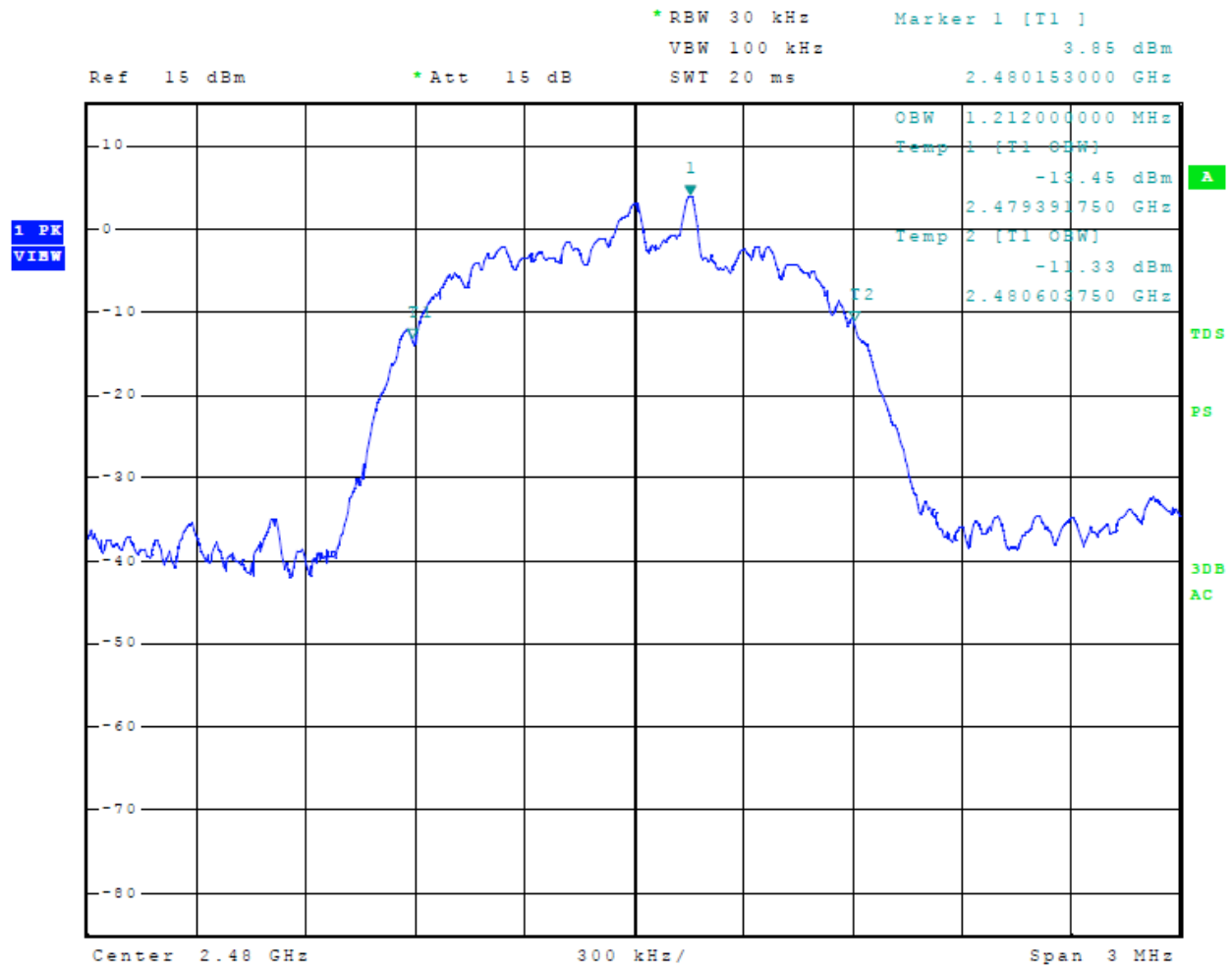
Figure 22 Plot of 99% Occupied Bandwidth Mode 4, BT 3EDR
