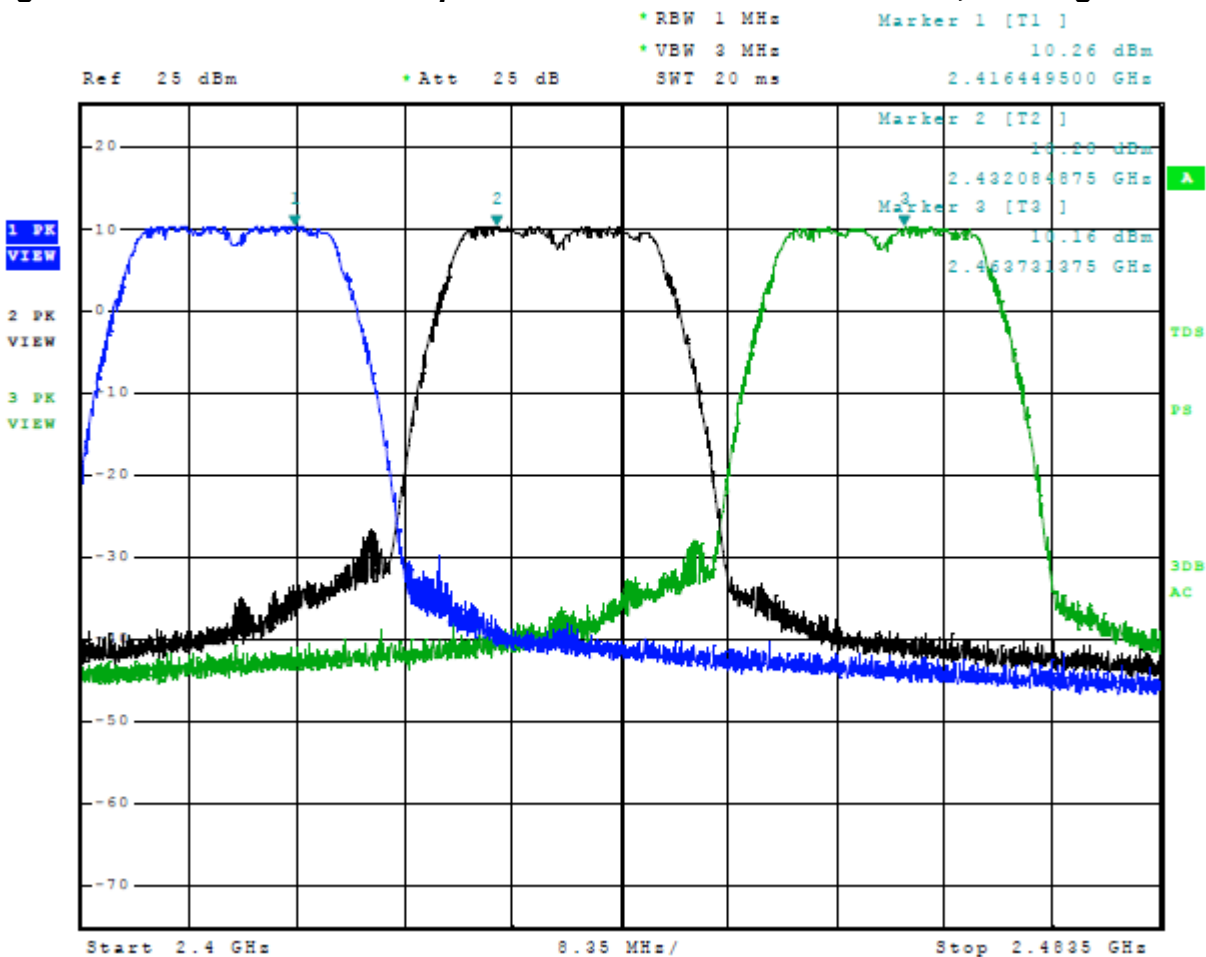
Figure 5 Plot of Transmitter Operation in 2402-2480 MHz Mode 7, 802.11g
