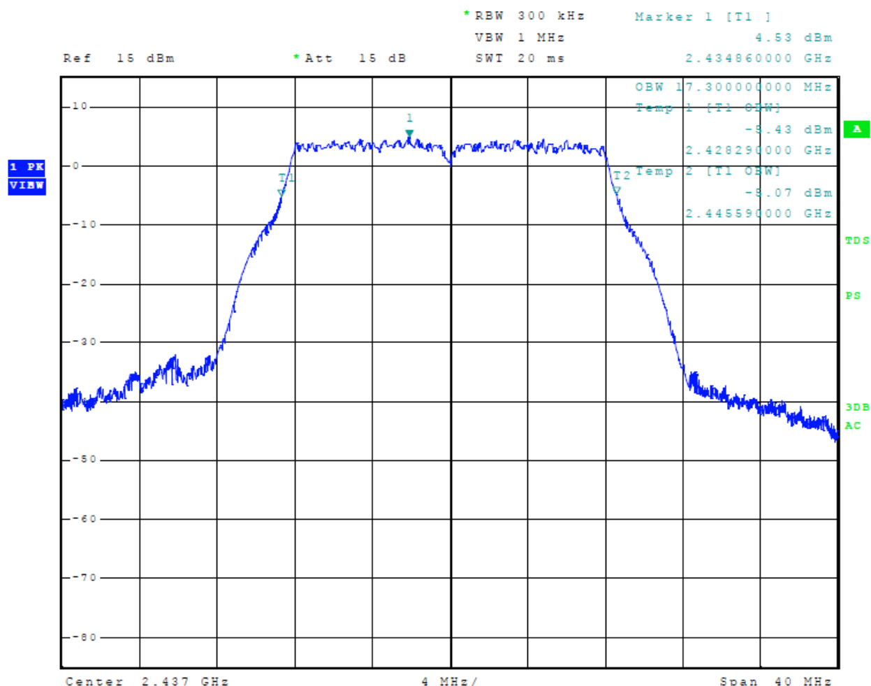
Figure 28 Plot of 99% Occupied Bandwidth Mode 7, 802.11g
