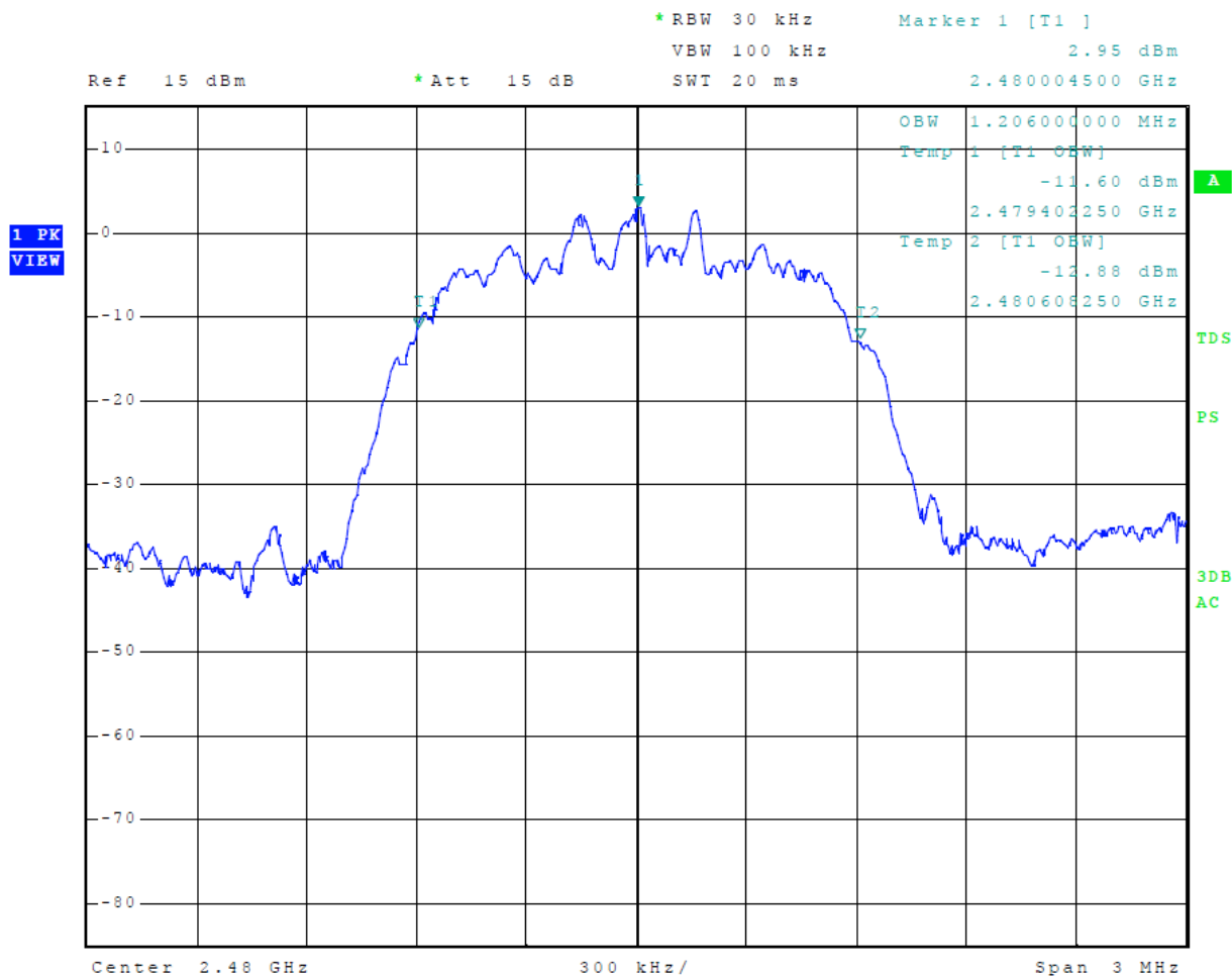
Figure 20 Plot of 99% Occupied Bandwidth Mode 3, BT 2EDR
