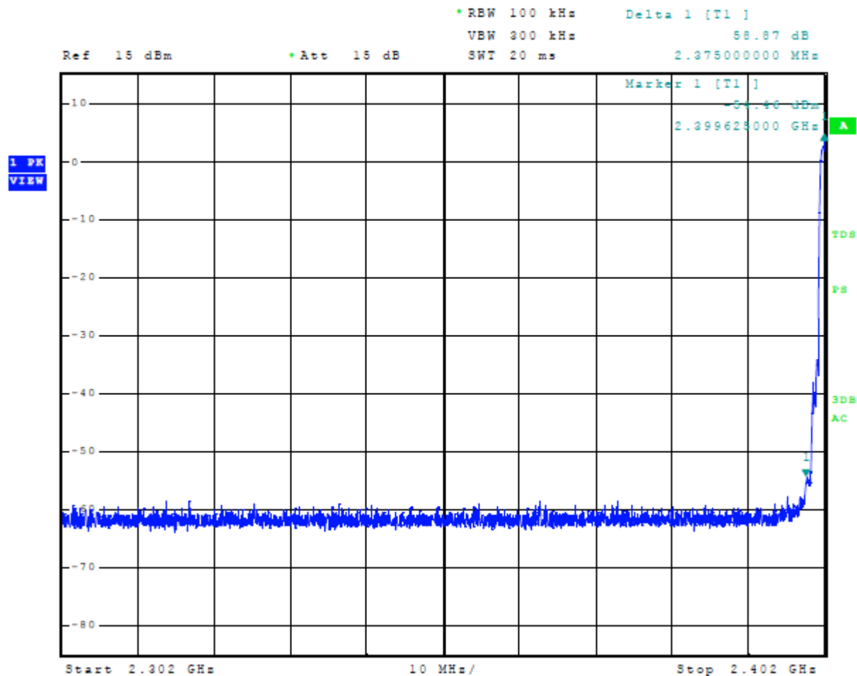
Figure 8 Plot of Emissions Low Band Edge Mode 4, BT 3EDR
