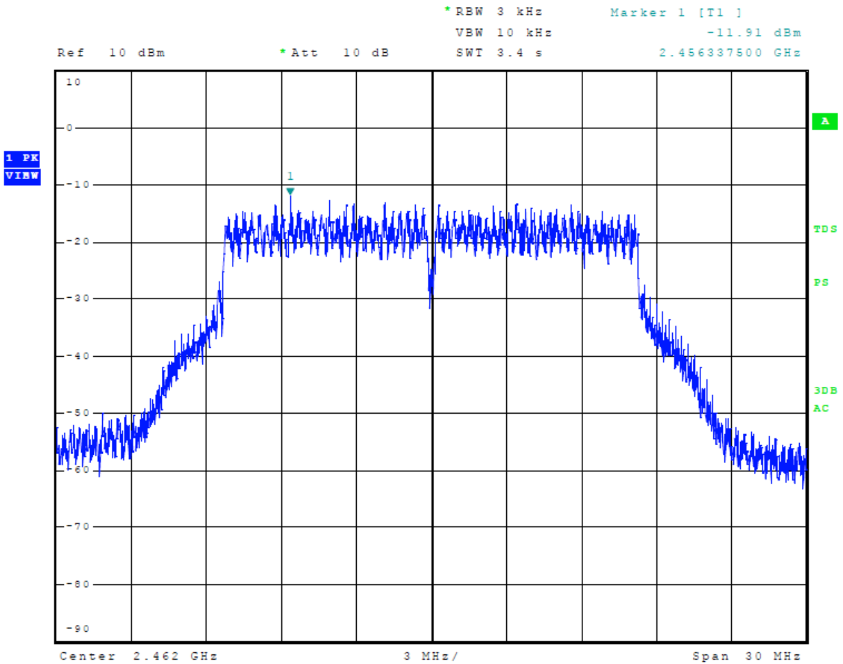
Figure 35 Plot of Transmitter Power Spectral Density Mode 7, 802.11g
