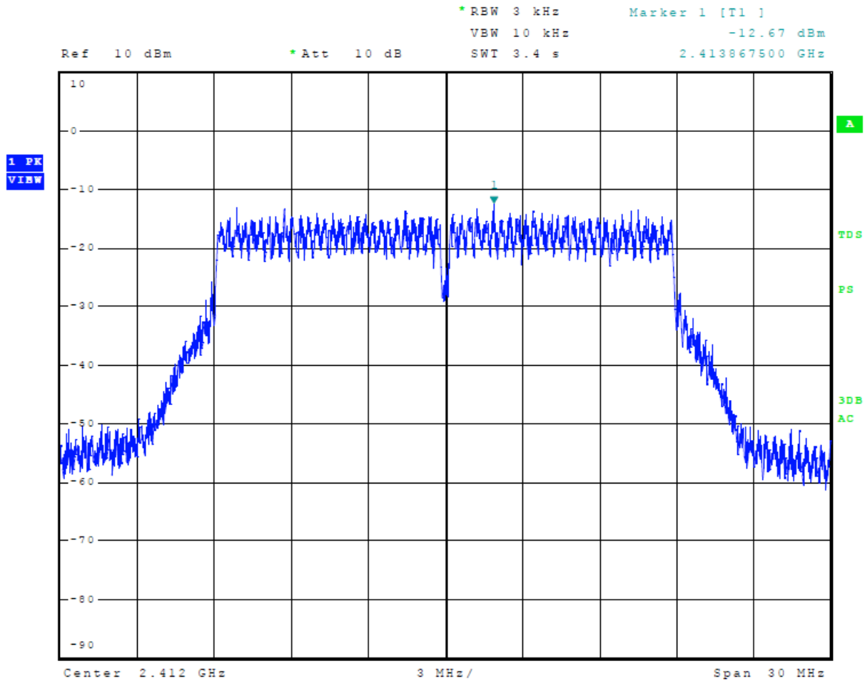
Figure 36 Plot of Transmitter Power Spectral Density Mode 8, 802.11n
