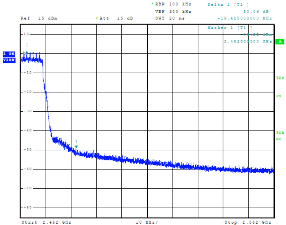
Figure 18 Plot of Transmitter Emissions High Band Edge Mode 8, 802.11n
