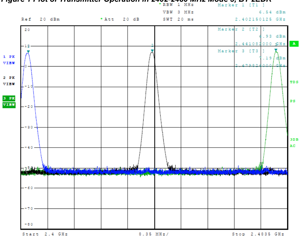
Figure 1 Plot of Transmitter Operation in 2402-2480 MHz Mode 3, BT 2EDR
