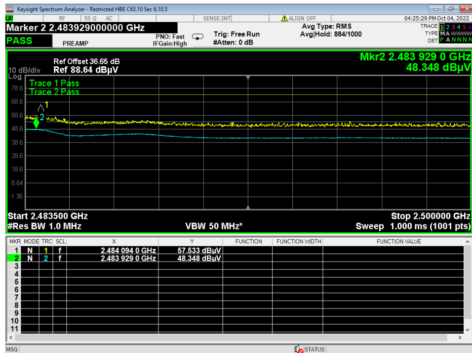
07 Higher Bandedge, Restricted, GFSK
