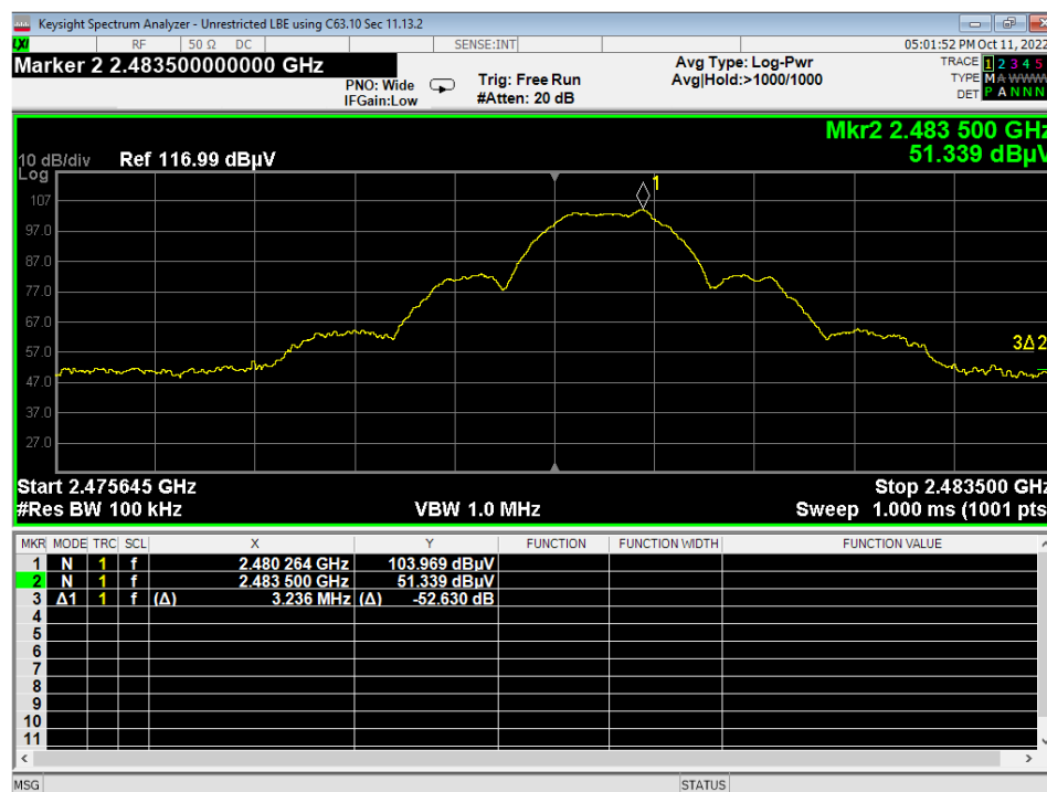
05 Higher Bandedge, Unrestricted, GFSK
