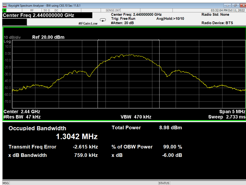
09 Occupied Bandwidth, Mid Channel, GFSK
