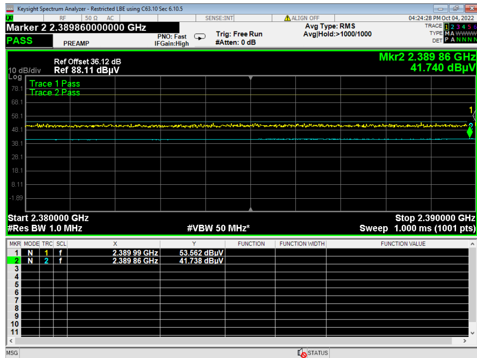
06 Lower Bandedge, Restricted, GFSK
