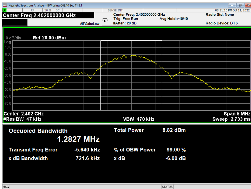
08 Occupied Bandwidth, Low Channel, GFSK
