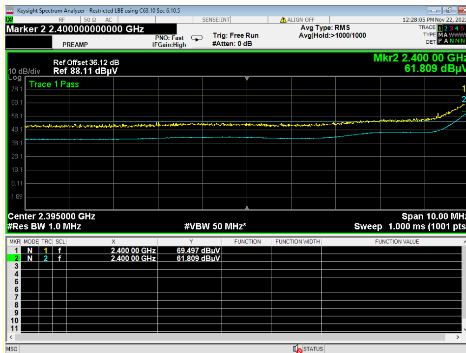
04 Lower Bandedge, Unrestricted, GFSK, 15.209 limits Disregard trace 2, duty cycle correction was added to peak level
