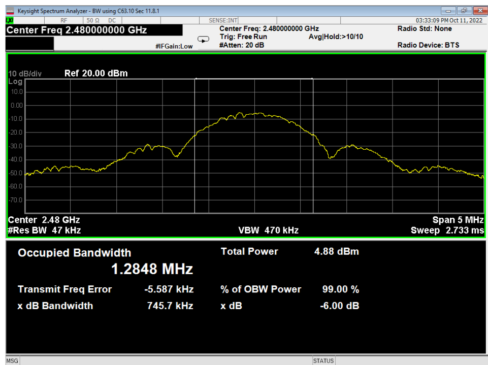
10 Occupied Bandwidth, High Channel, GFSK
