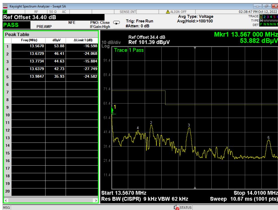
Figure 4 – Upper Bandedge
