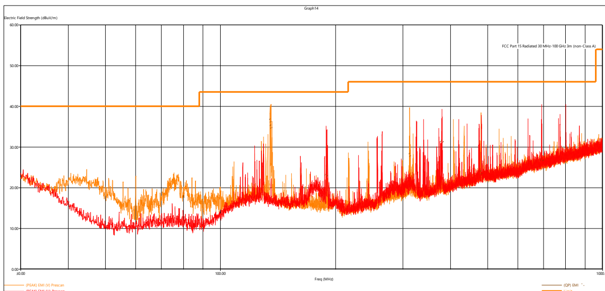
Figure 5 – NFC Radiated Emissions Plot, 30MHz – 1GHz
