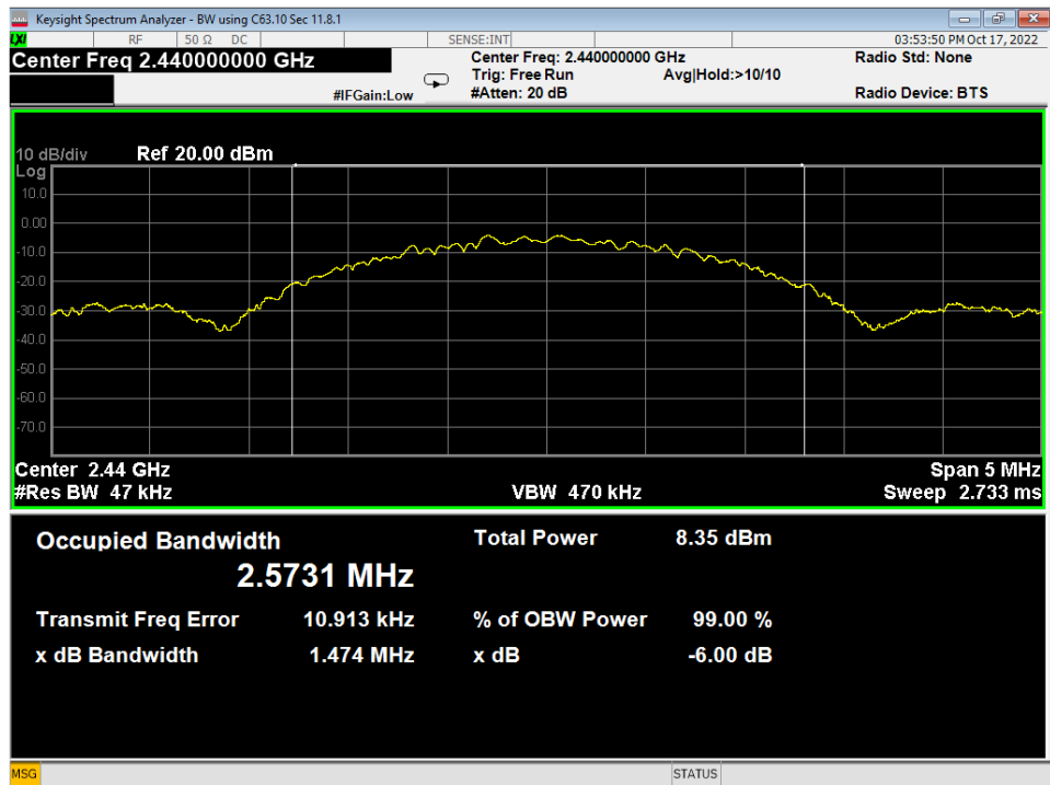
32 Occupied Bandwidth, Mid Channel, GMSK 2MB
