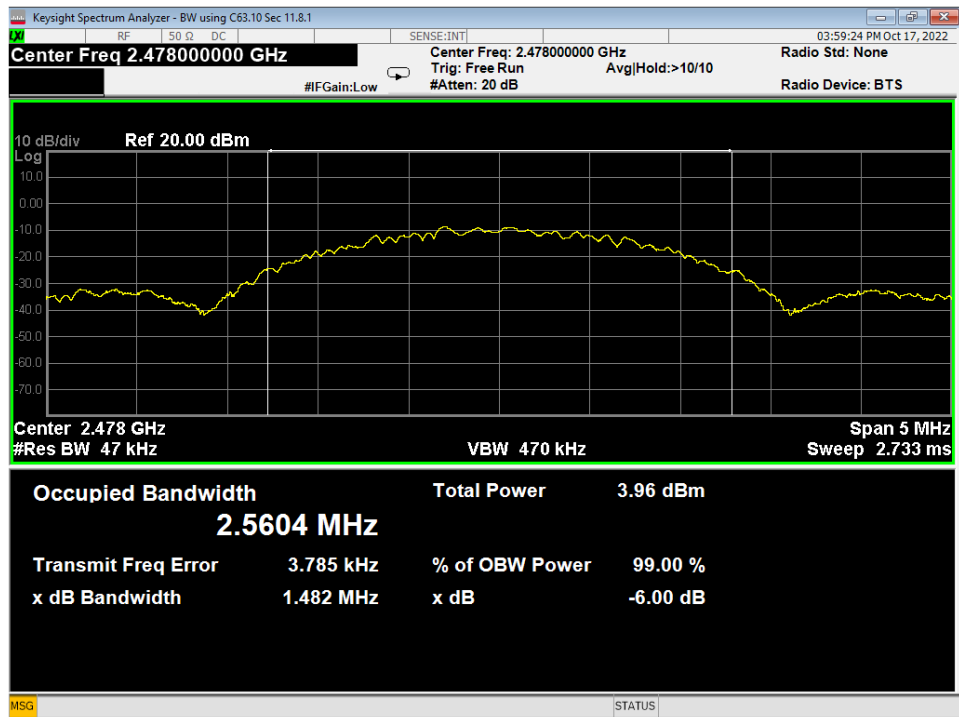
33 Occupied Bandwidth, High Channel, GMSK 2MB
