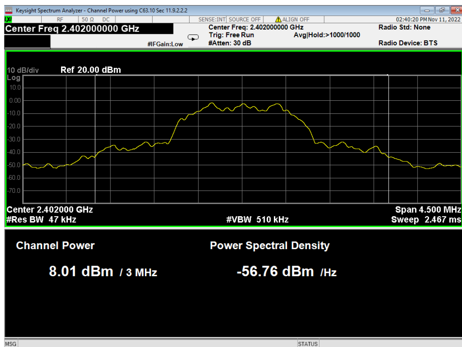
14 Average Power, Low Channel, 3EDR
