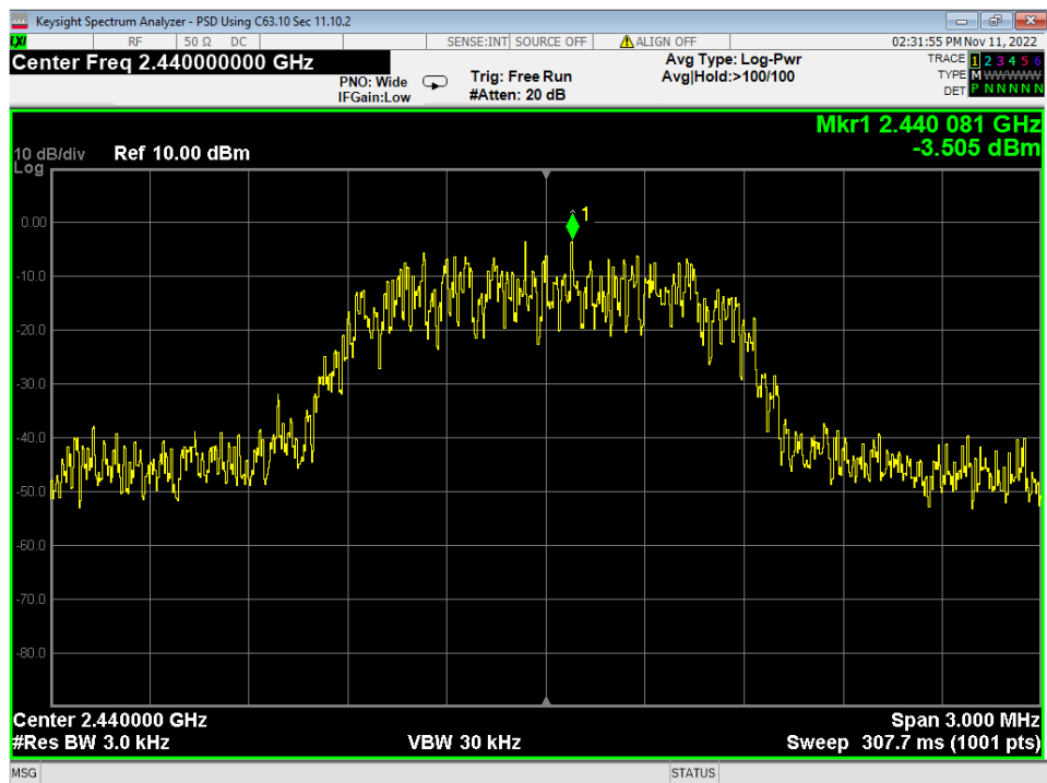
08 PSD, Mid Channel, 2EDR
