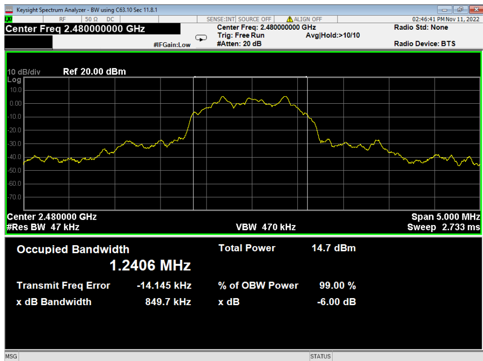
32 Occupied Bandwidth, High Channel, 3EDR
