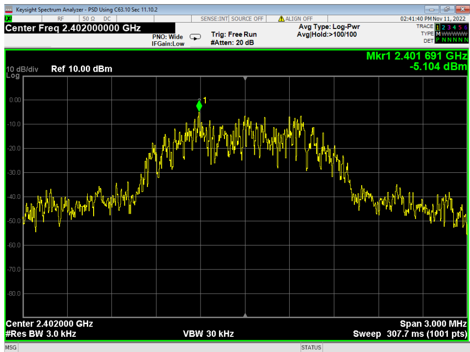
20 PSD, Low Channel, 3EDR
