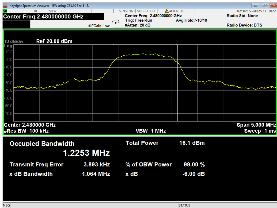
06 6dB Bandwidth, High Channel, 2EDR
