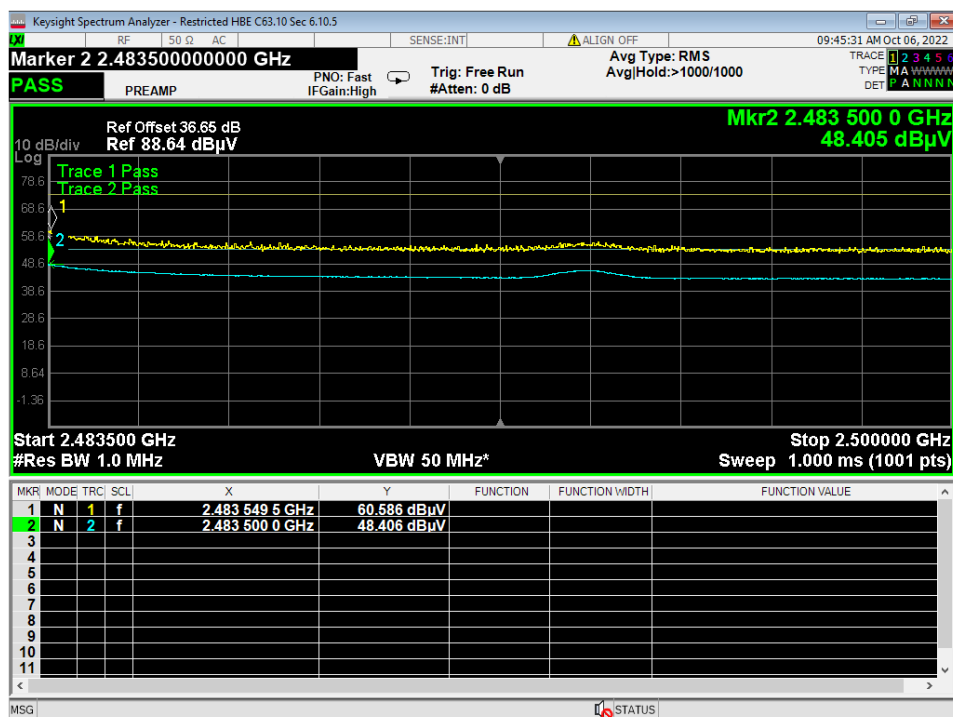
13 Higher Bandedge, Restricted, 2EDR
