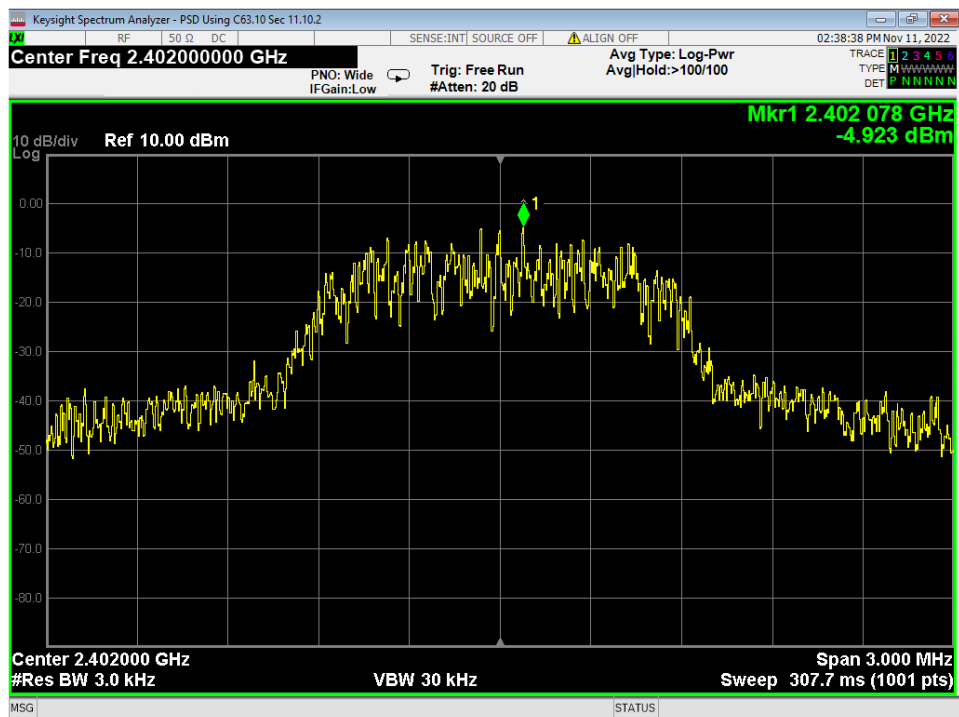
07 PSD, Low Channel, 2EDR
