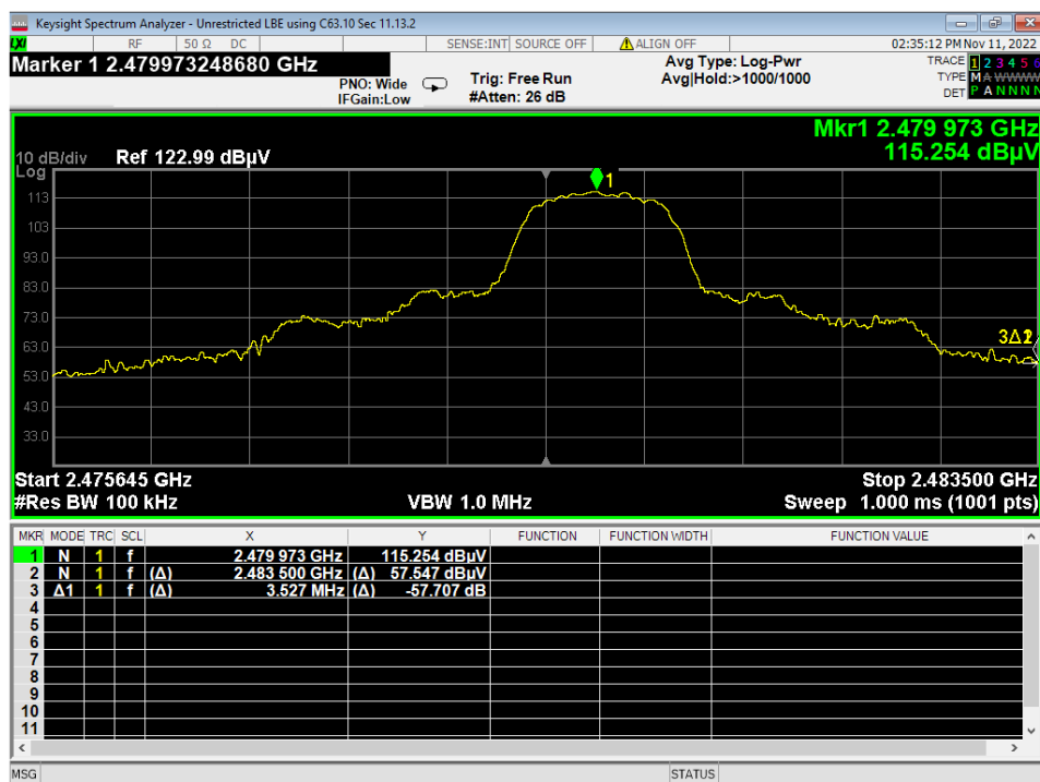
11 Higher Bandedge, Unrestricted, 2EDR
