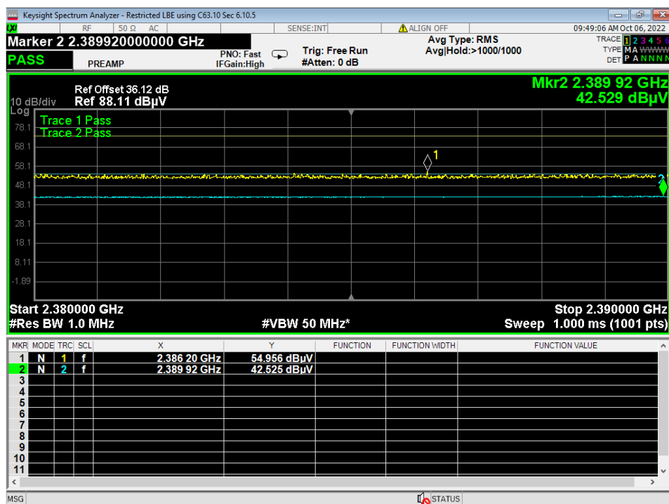
25 Lower Bandedge, Restricted, 3EDR
