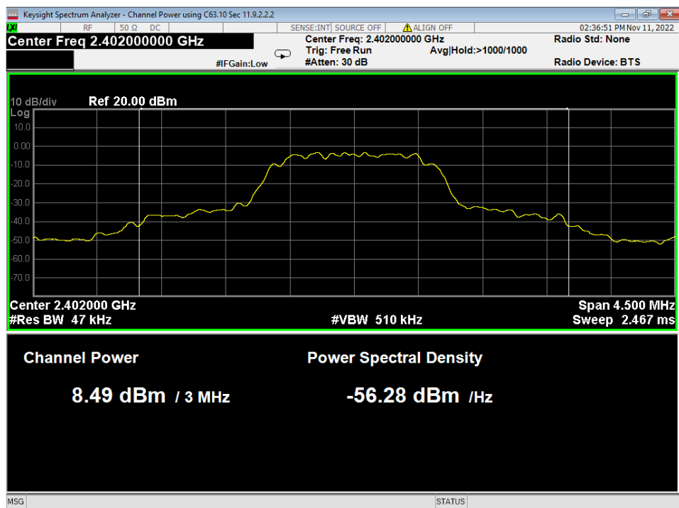
01 Power, Low Channel, 2EDR
