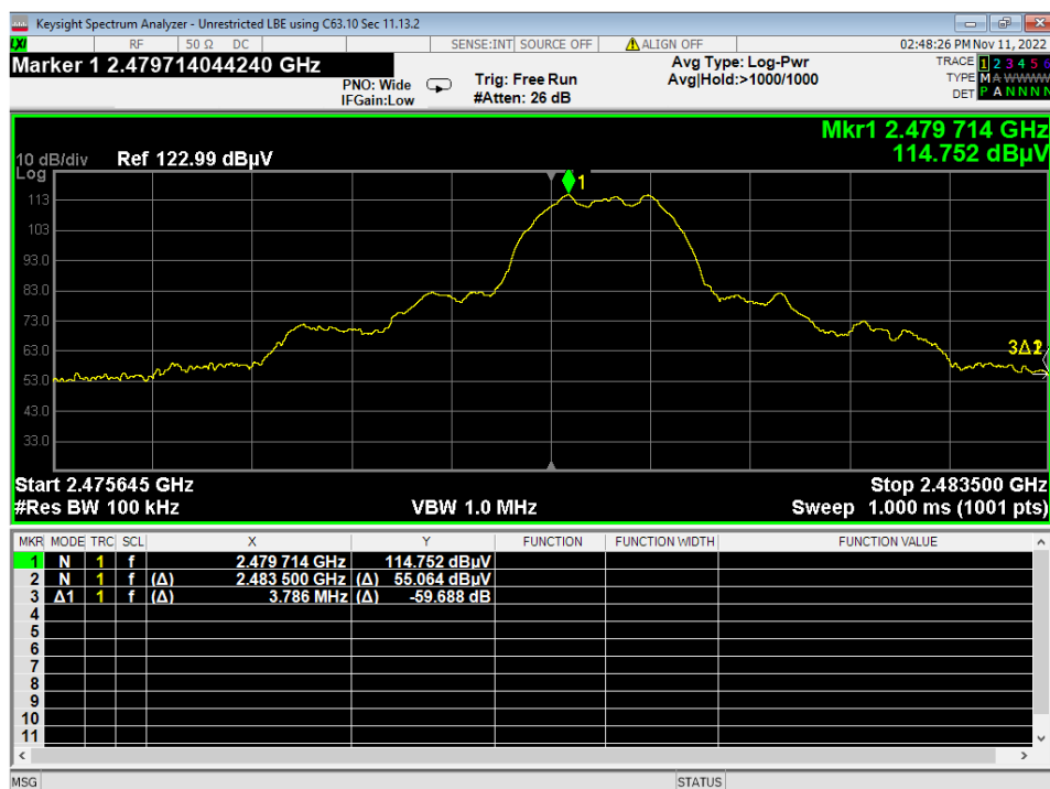
24 Higher Bandedge, Unrestricted, 3EDR
