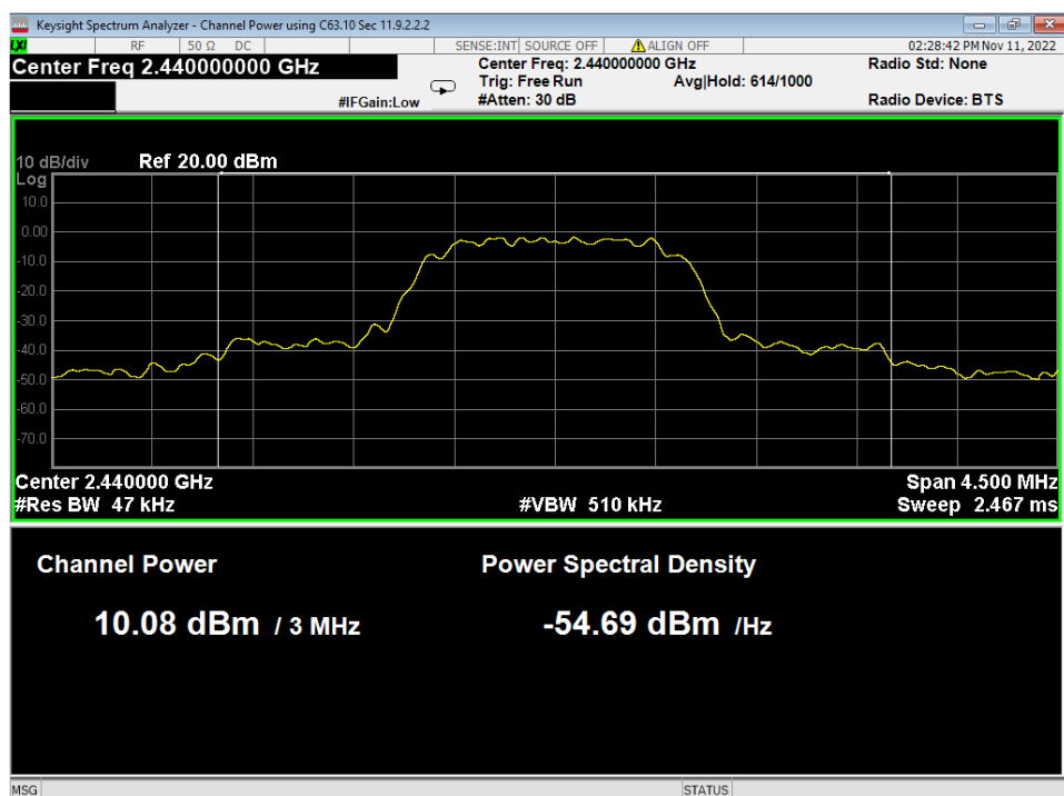
02 Power, Mid Channel, 2EDR
