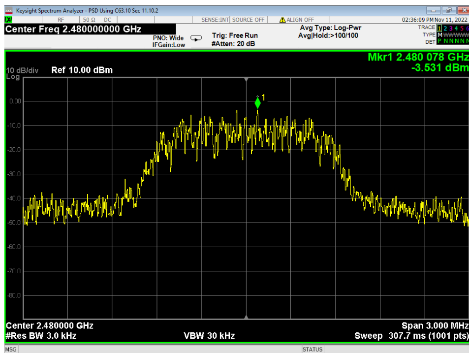
09 PSD, High Channel, 2EDR
