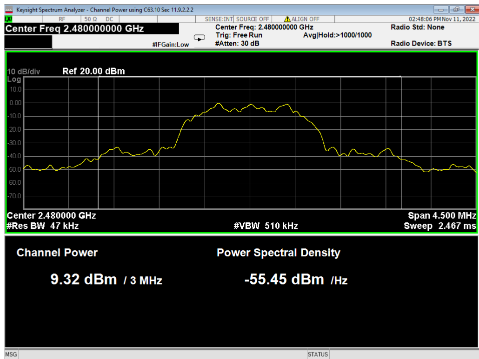
16 Average Power, High Channel, 3EDR
