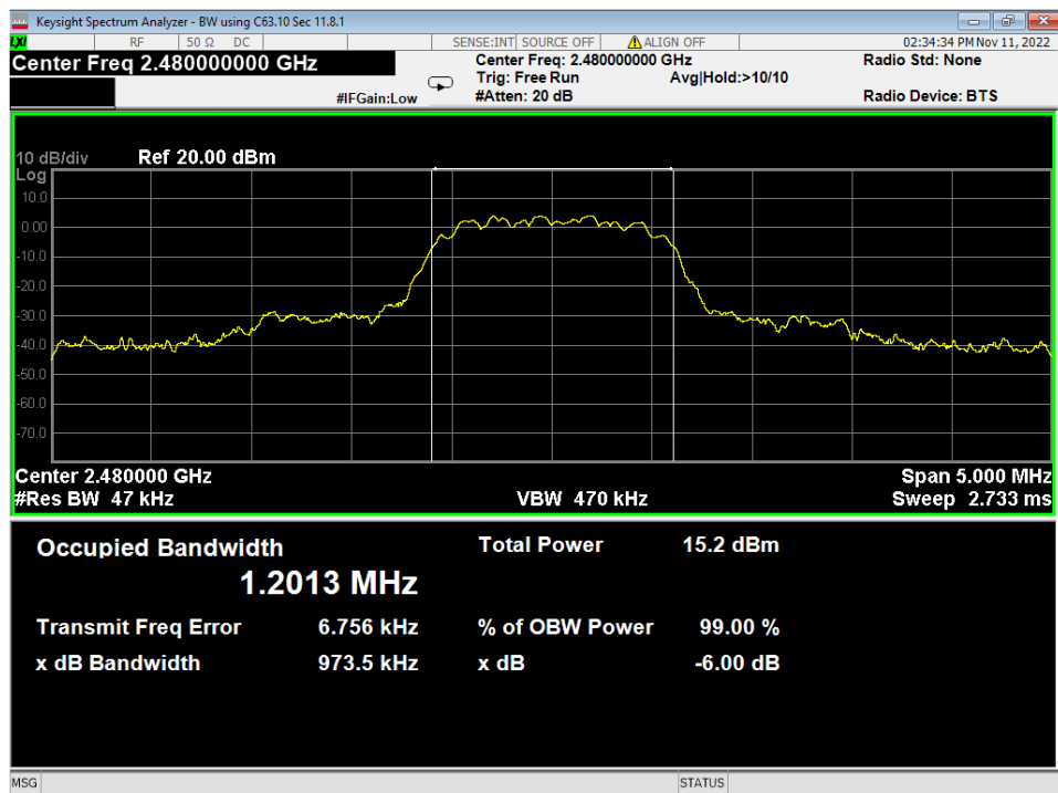
29 Occupied Bandwidth, High Channel, 2EDR
