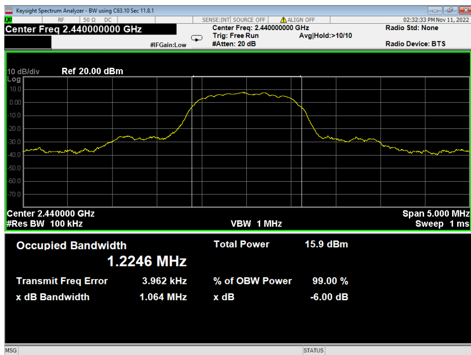
05 6dB Bandwidth, Mid Channel, 2EDR
