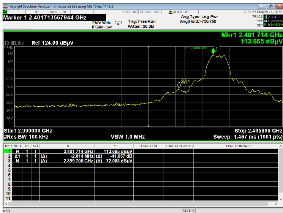
23 Lower Bandedge, Unrestricted, 3EDR
