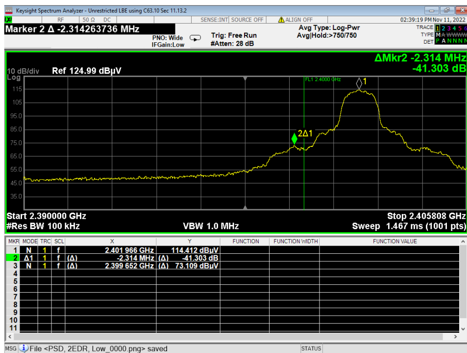
10 Lower Bandedge, Unrestricted, 2EDR
