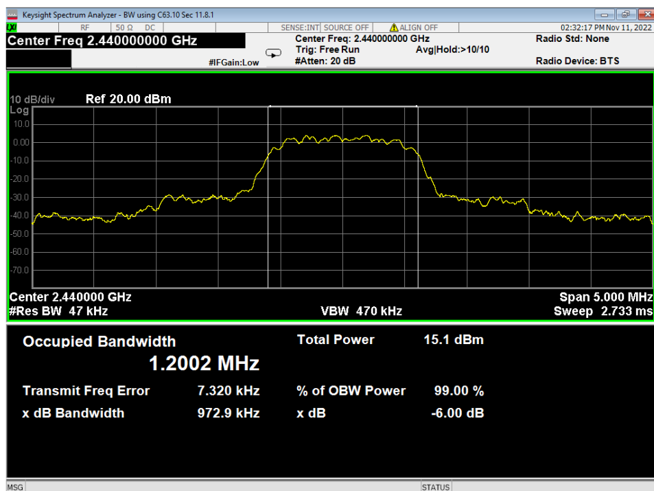
28 Occupied Bandwidth, Mid Channel, 2EDR
