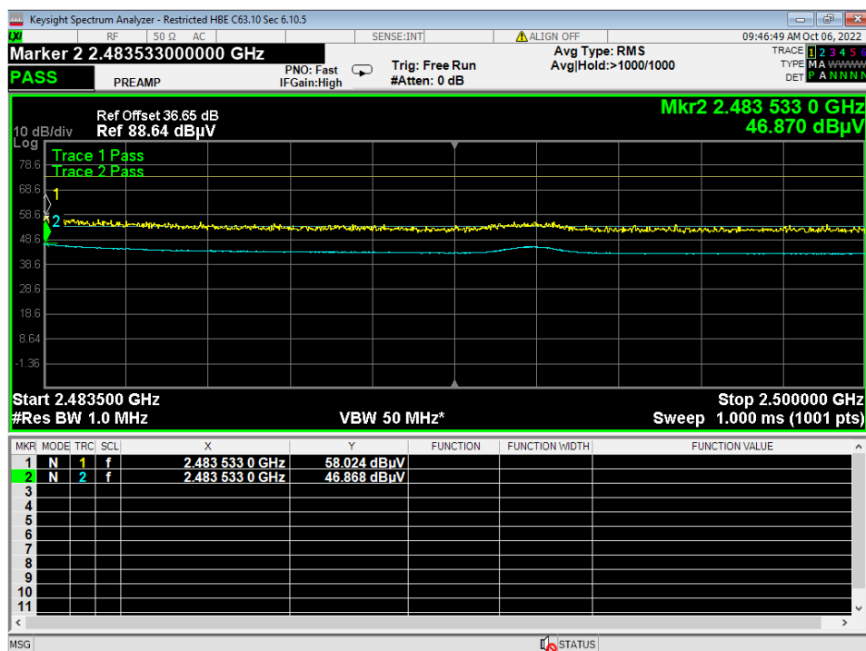
26 Higher Bandedge, Restricted, 3EDR
