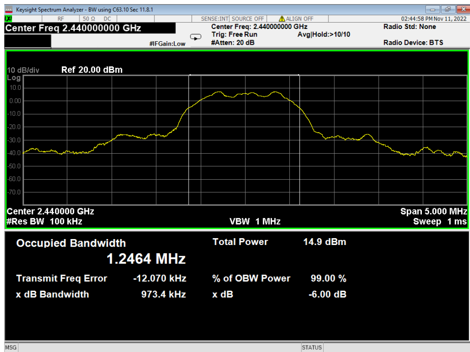
18 6dB Bandwidth, Mid Channel, 3EDR
