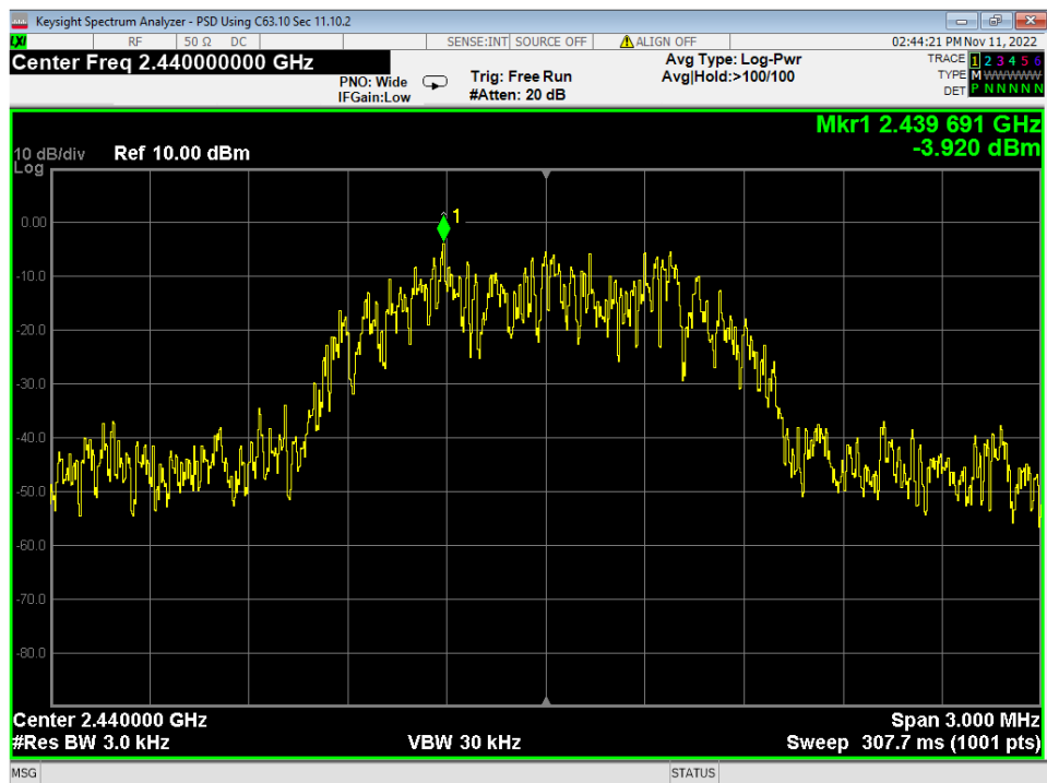
21 PSD, Mid Channel, 3EDR
