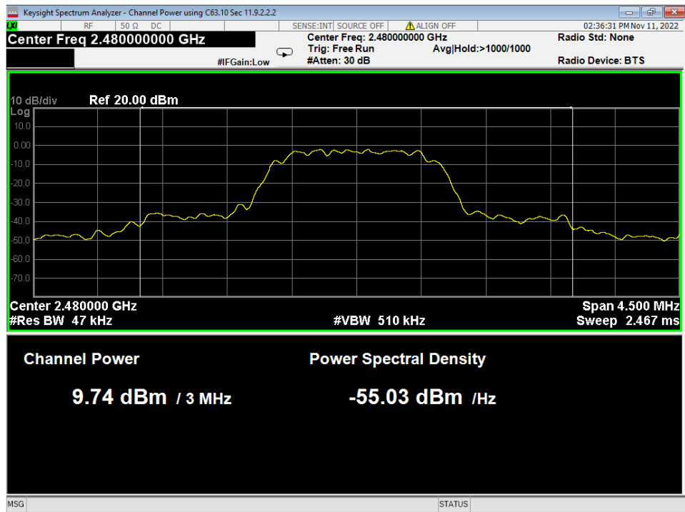
03 Power, High Channel, 2EDR
