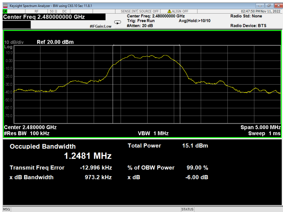
19 6dB Bandwidth, High Channel, 3EDR
