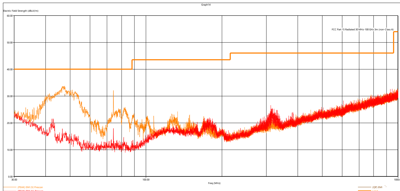
Figure 6 - Radiated Emissions Plot, BT EDR 3MB
