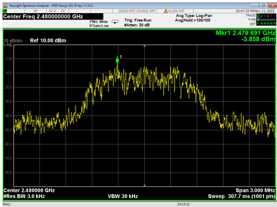
22 PSD, High Channel, 3EDR
