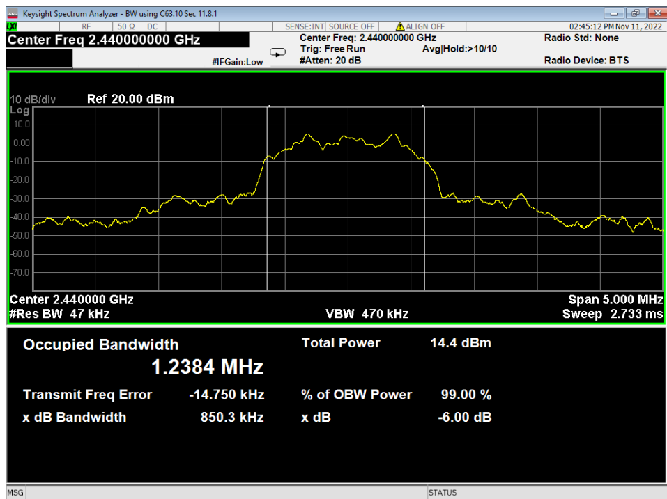
31 Occupied Bandwidth, Mid Channel, 3EDR
