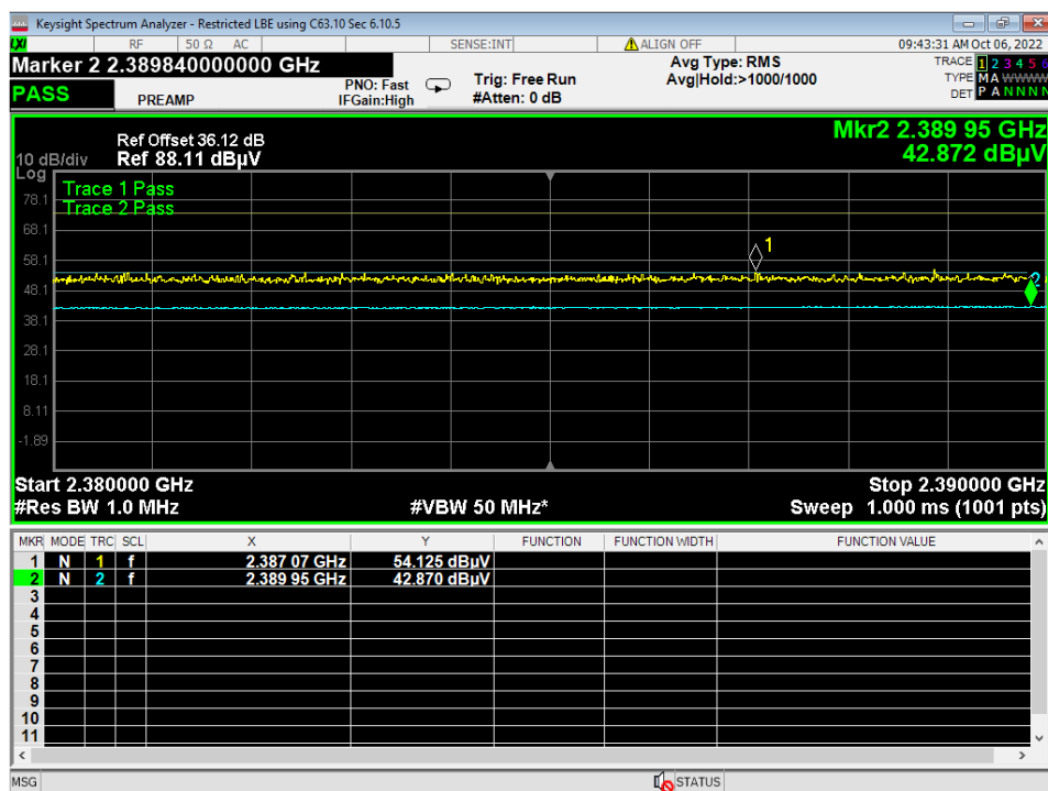
12 Lower Bandedge, Restricted, 2EDR
