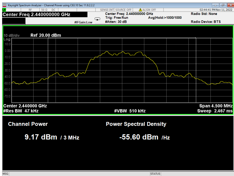
15 Average Power, Mid Channel, 3EDR
