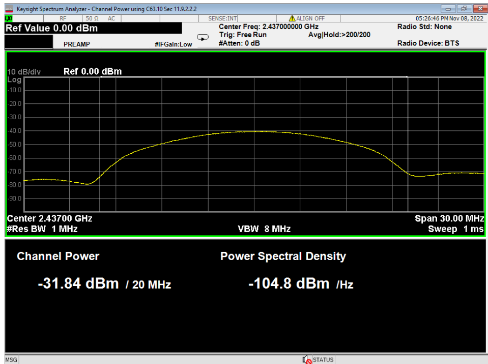
Figure 11 – Radiated Average Power Measurement, 802.11b 11MB
