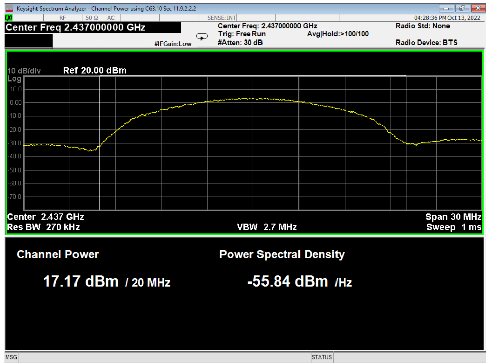
Figure 10 – Conducted Average Power Measurement, 802.11b 11MB
