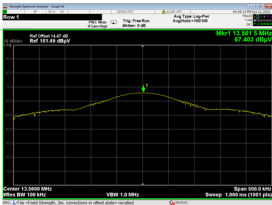
Figure 4 – Field Strength, 3m
