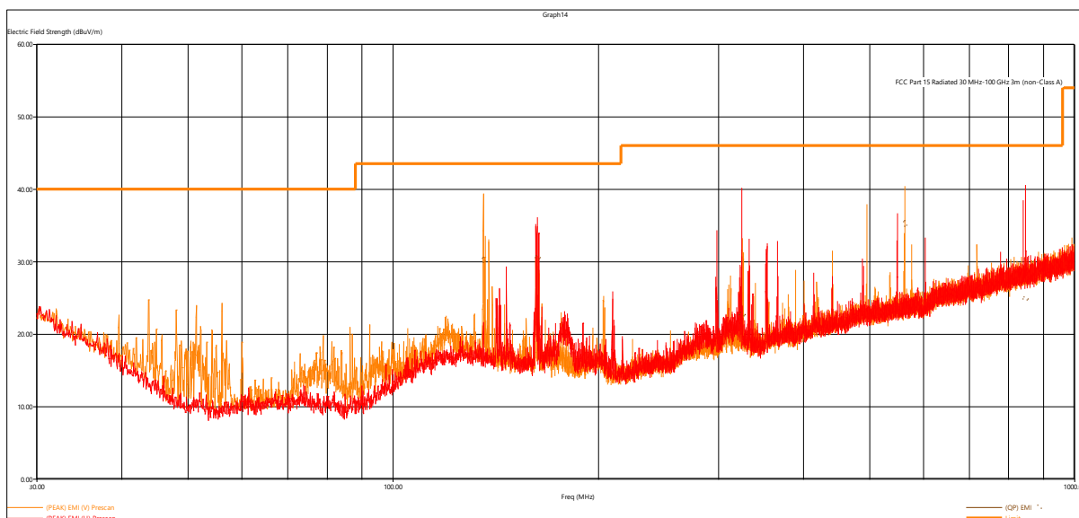
Figure 2 – NFC Radiated Emissions Plot, 30MHz – 1GHz
