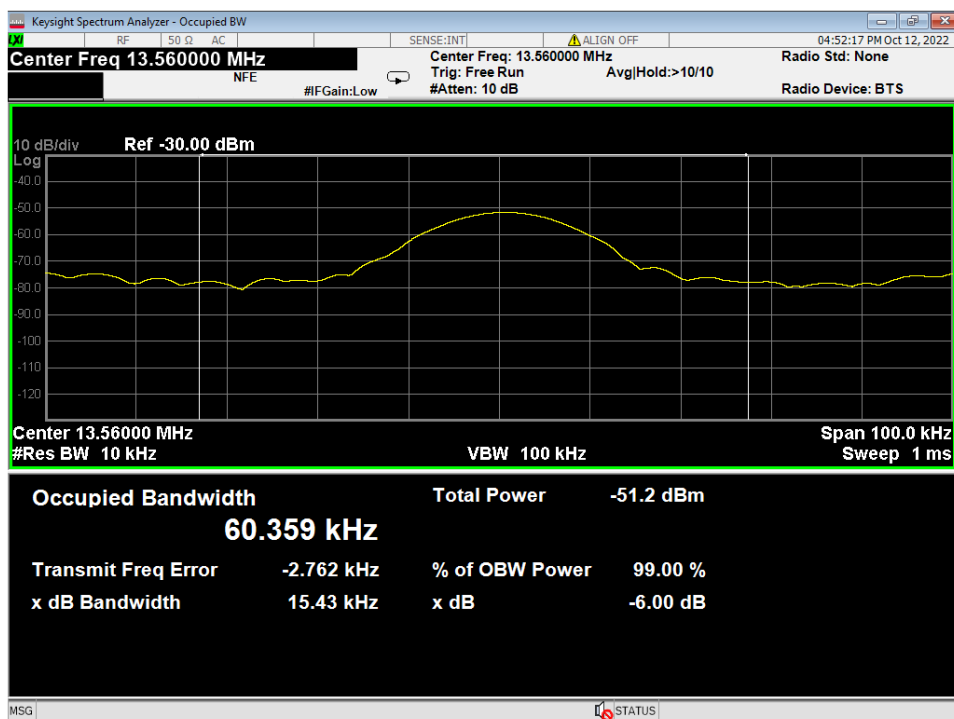
Figure 3 – NFC Occupied Bandwidth
