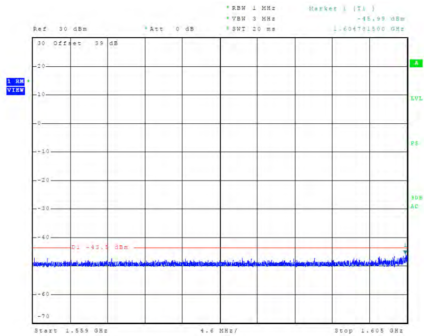
Figure 73 Plot of E.I.R.P. density of unwanted emissions (Mode B1 / Ch. 1)
