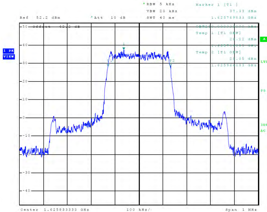
Figure 71 Plot of 99% OBW (Mode C8 / Channel 240)
