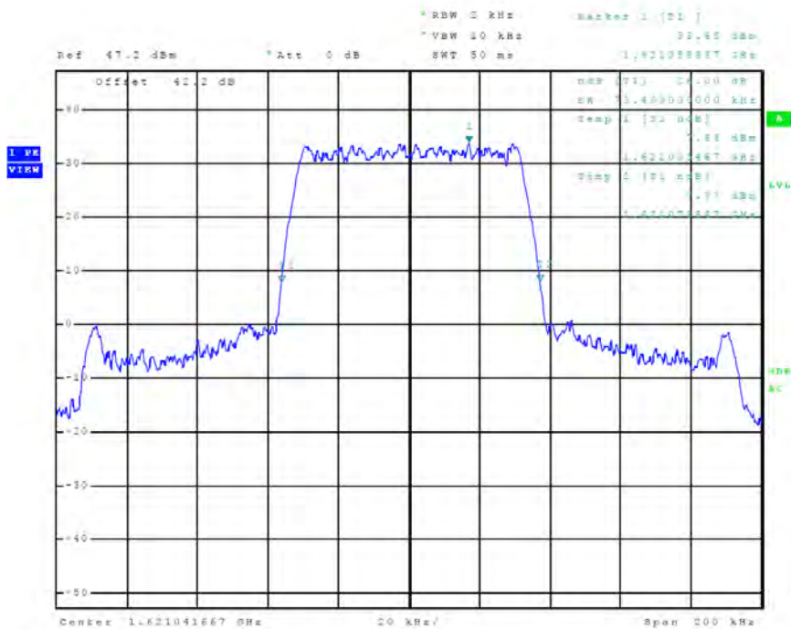
Figure 70 Plot of -26dB OBW (Mode C2 / Channel 121)
