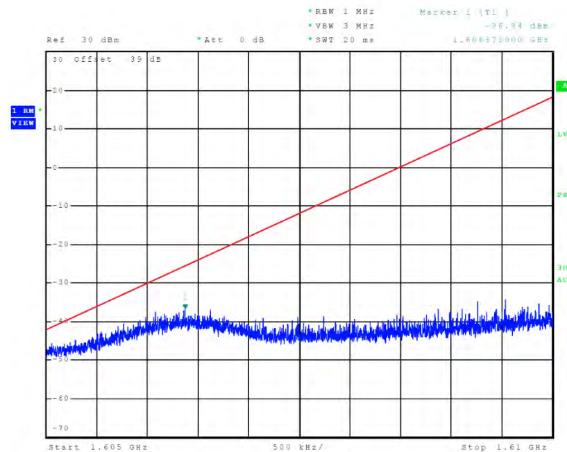
Figure 80 Plot of E.I.R.P. density of unwanted emissions (Mode C1 / Ch. 1)
