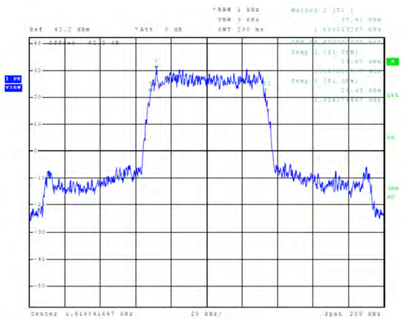
Figure 69 Plot of 99% OBW (Mode C2 / Channel 1)
