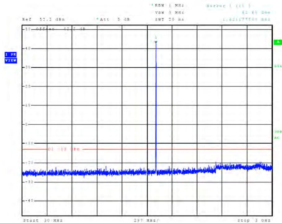
Figure 5 Plot of emissions across Frequency spectrum (Mode B1 / Ch. 121)
