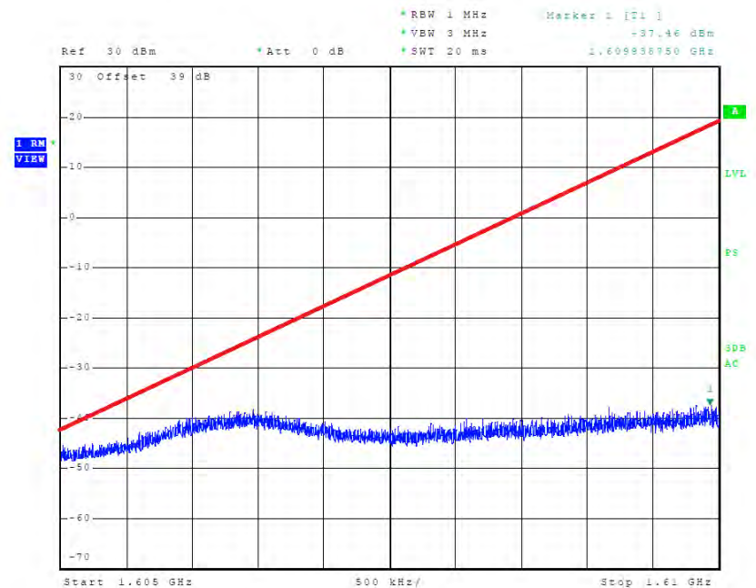
Figure 74 Plot of E.I.R.P. density of unwanted emissions (Mode B1 / Ch. 1)
