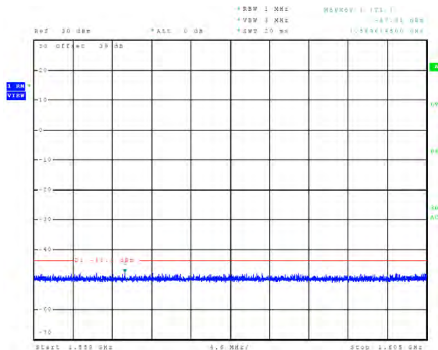
Figure 83 Plot of E.I.R.P. density of unwanted emissions (Mode C1 / Ch. 240)
