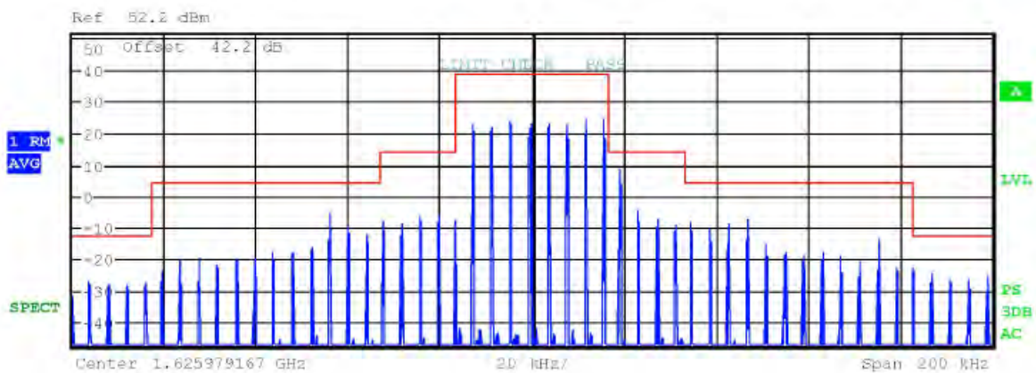
Figure 54 Plot of emissions with emission mask (Mode C1 / Ch. 121)
