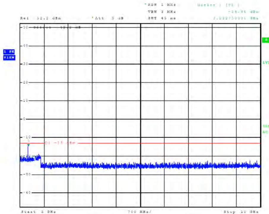
Figure 39 Plot of emissions across Frequency spectrum (Mode C8 / Ch. 1)
