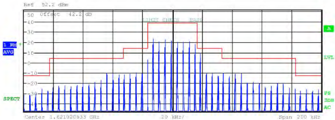
Figure 53 Plot of emissions with emission mask (Mode C1 / Ch. 1)
