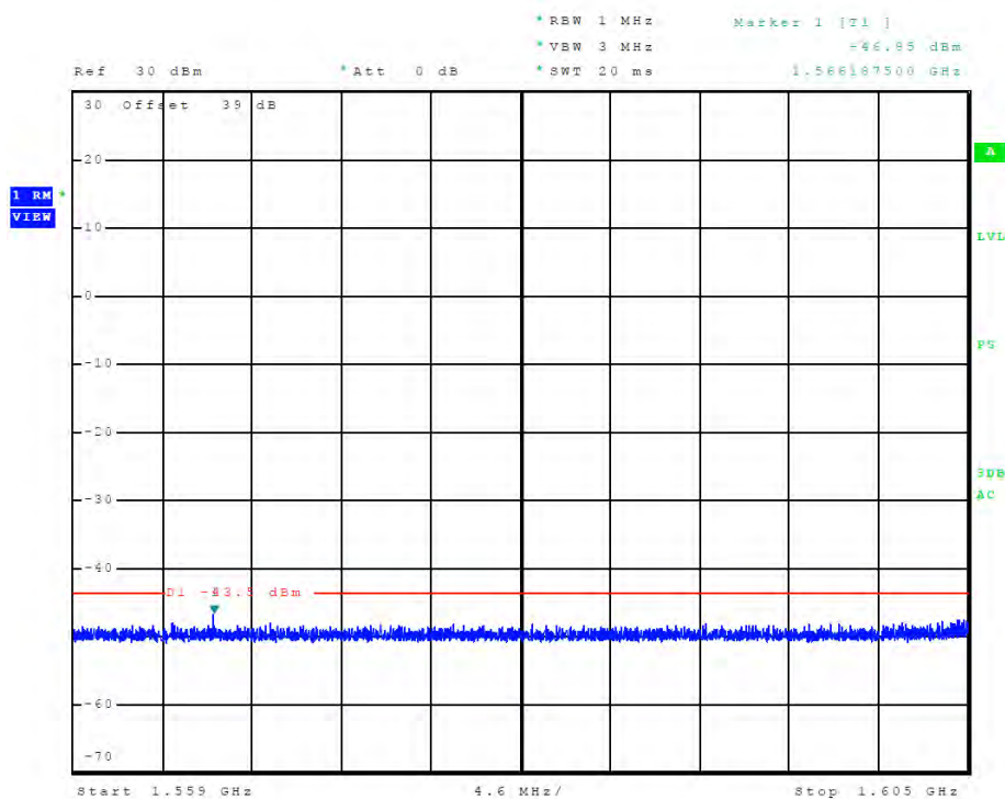
Figure 87 Plot of E.I.R.P. density of unwanted emissions (Mode C2 / Ch. 121)
