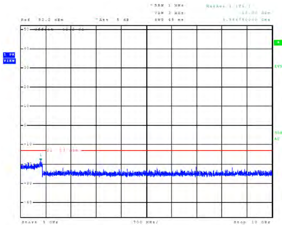
Figure 23 Plot of emissions across Frequency spectrum (Mode C1 / Ch. 240)
