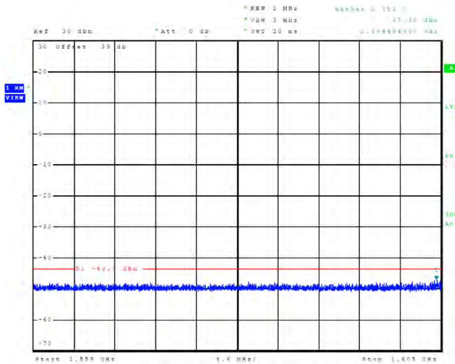
Figure 89 Plot of E.I.R.P. density of unwanted emissions (Mode C2 / Ch. 240)
