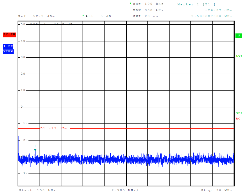
Figure 41 Plot of emissions across Frequency spectrum (Mode C8 / Ch. 121)
