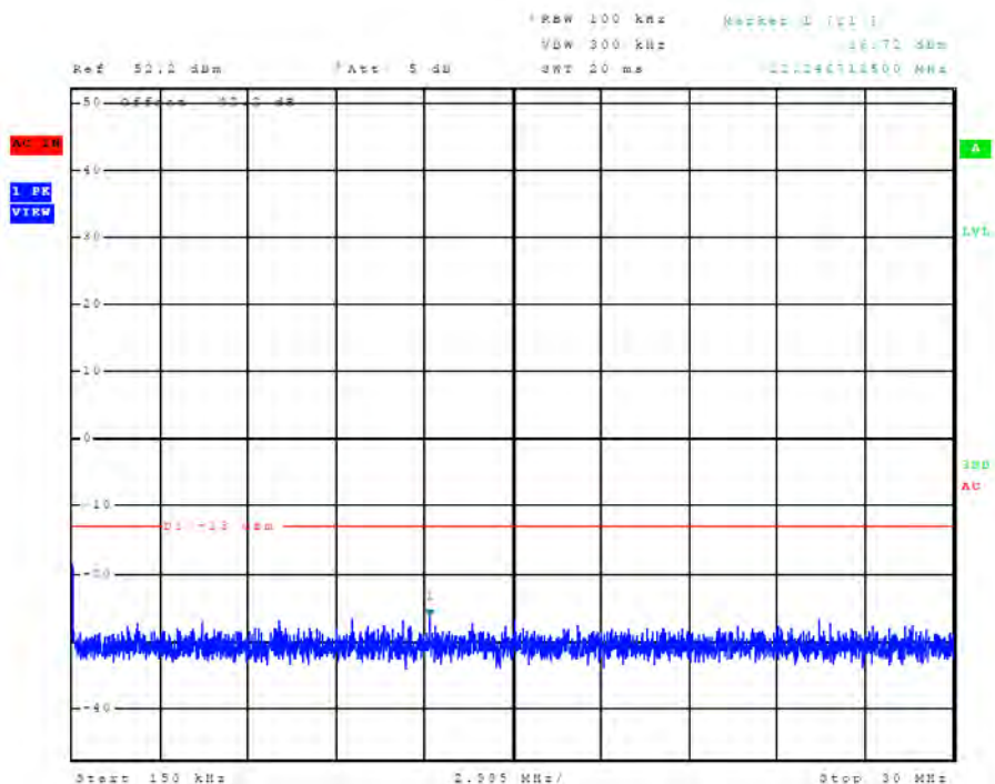
Figure 29 Plot of emissions across Frequency spectrum (Mode C2 / Ch. 121)
