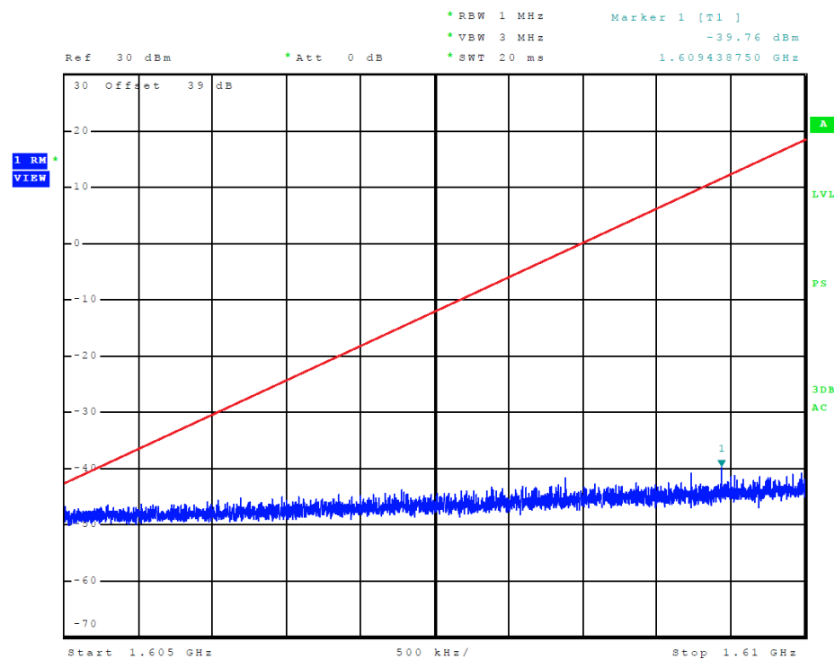
Figure 88 Plot of E.I.R.P. density of unwanted emissions (Mode C2 / Ch. 121)
