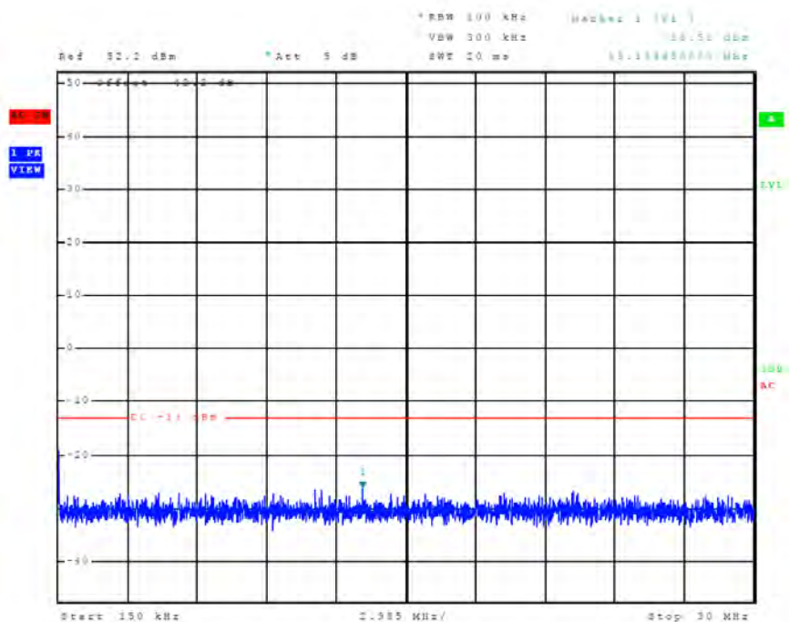
Figure 25 Plot of emissions across Frequency spectrum (Mode C2 / Ch. 1)
