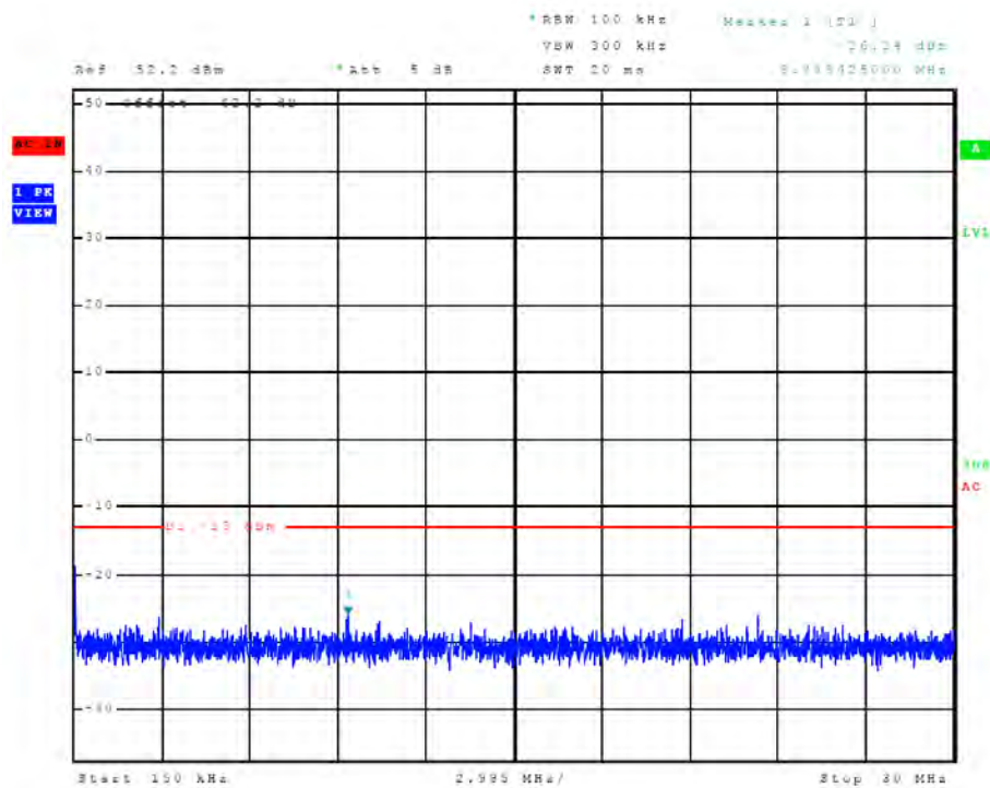
Figure 33 Plot of emissions across Frequency spectrum (Mode C2 / Ch. 240)
