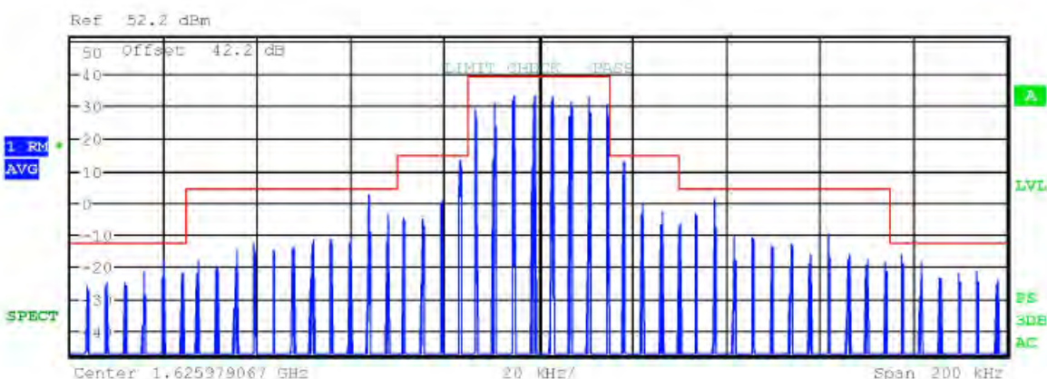
Figure 51 Plot of emissions with emission mask (Mode B1 / Ch. 240)
