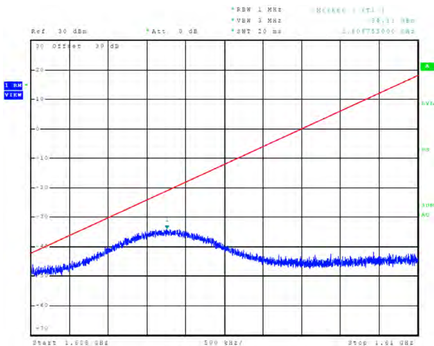
Figure 84 Plot of E.I.R.P. density of unwanted emissions (Mode C1 / Ch. 240)
