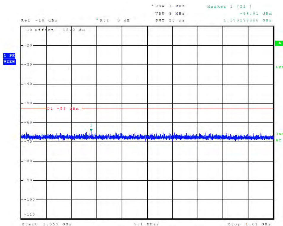
Figure 97 Plot of E.I.R.P. density of unwanted emissions carrier-off
