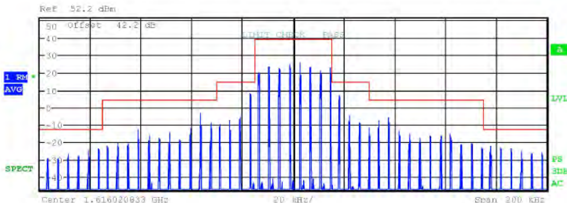
Figure 49 Plot of emissions with emission mask (Mode B1 / Ch. 1)
