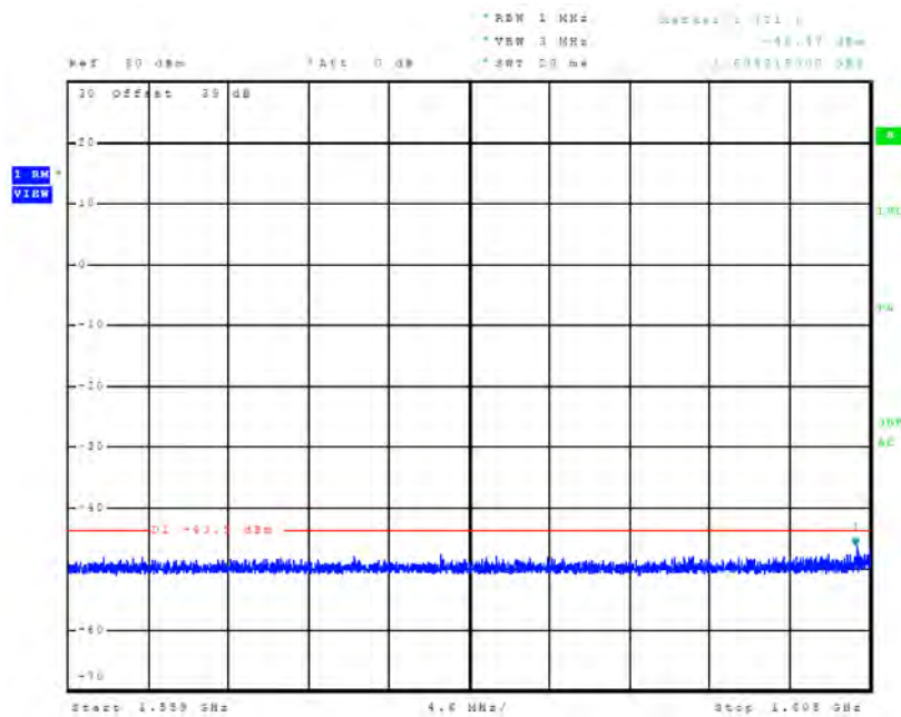
Figure 85 Plot of E.I.R.P. density of unwanted emissions (Mode C2 / Ch. 1)
