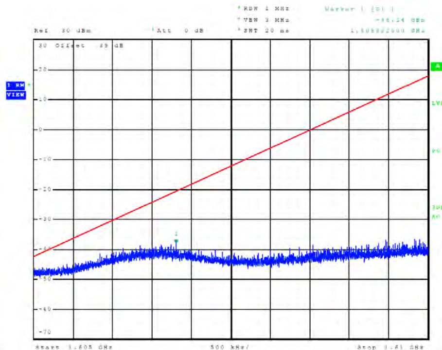
Figure 92 Plot of E.I.R.P. density of unwanted emissions (Mode C8 / Ch. 1)
