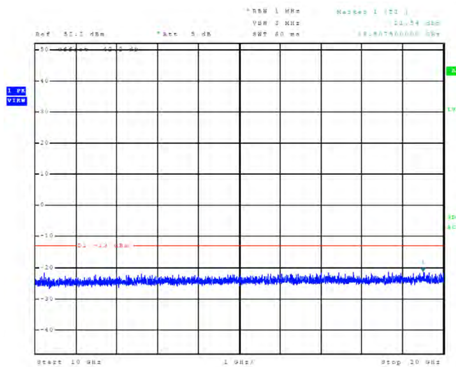
Figure 40 Plot of emissions across Frequency spectrum (Mode C8 / Ch. 1)
