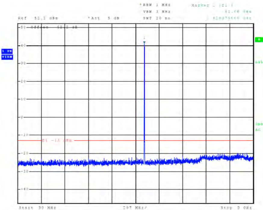
Figure 10 Plot of emissions across Frequency spectrum (Mode B1 / Ch. 240)
