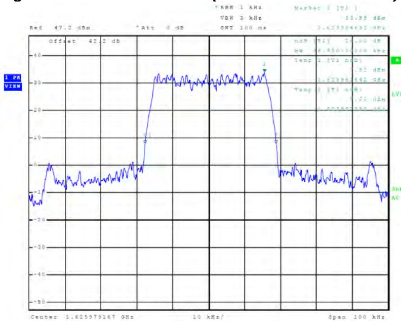
Figure 68 Plot of -26dB OBW (Mode C1 / Channel 240)
