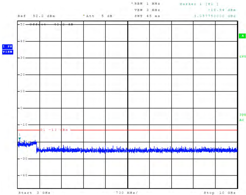
Figure 15 Plot of emissions across Frequency spectrum (Mode C1 / Ch. 1)
