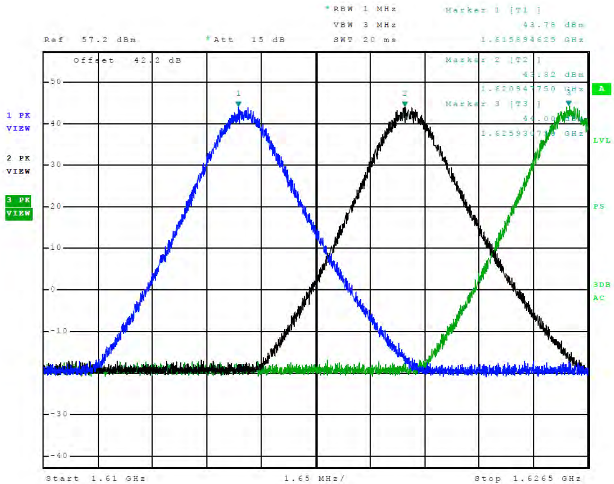
Figure 60 Plot of Operation across Frequency band (Mode C2)
