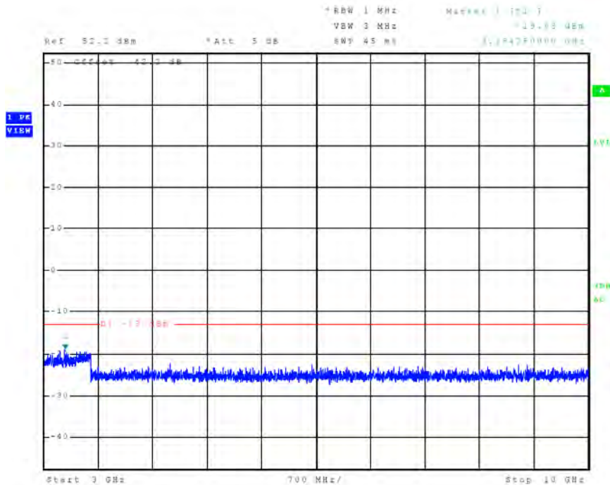
Figure 11 Plot of emissions across Frequency spectrum (Mode B1 / Ch. 240)
