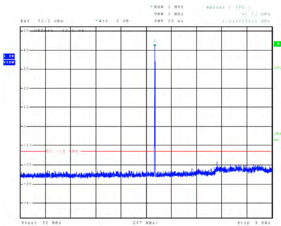
Figure 2 Plot of emissions across Frequency spectrum (Mode B1 / Ch. 1)
