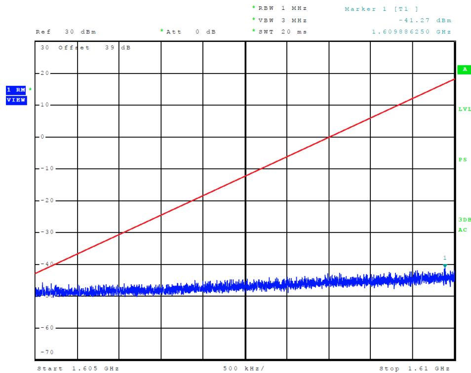
Figure 76 Plot of E.I.R.P. density of unwanted emissions (Mode B1 / Ch. 121)
