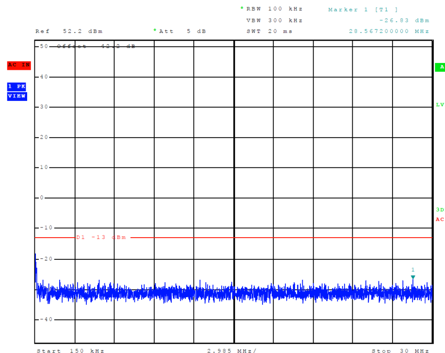
Figure 45 Plot of emissions across Frequency spectrum (Mode C8 / Ch. 240)
