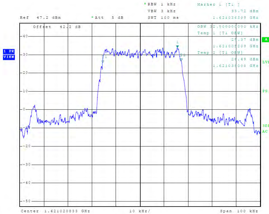
Figure 67 Plot of 99% OBW (Mode C1 / Channel 121)
