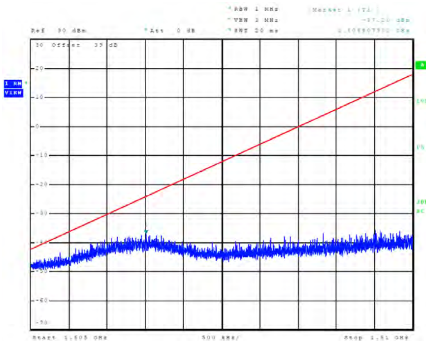
Figure 86 Plot of E.I.R.P. density of unwanted emissions (Mode C2 / Ch. 1)
