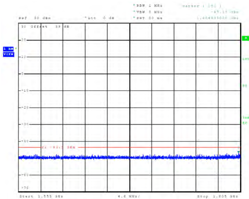
Figure 75 Plot of E.I.R.P. density of unwanted emissions (Mode B1 / Ch. 121)
