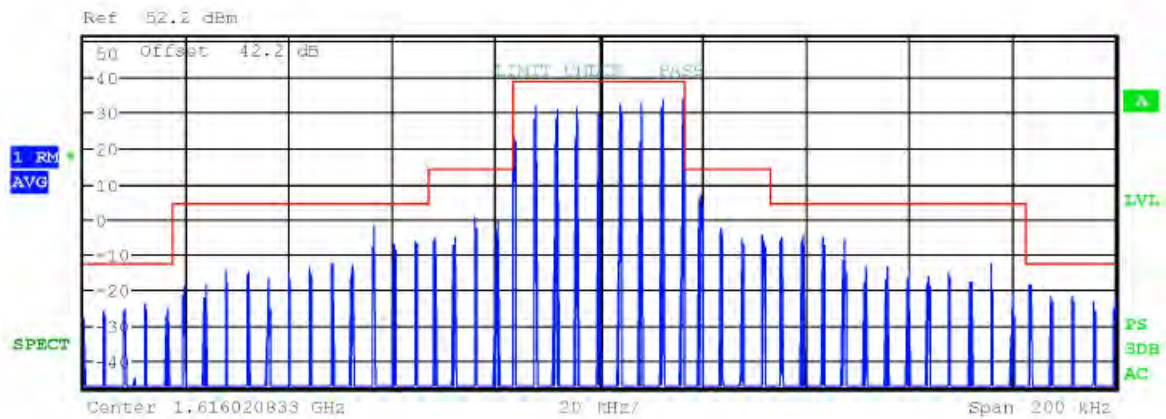
Figure 53 Plot of emissions with emission mask (Mode C1 / Ch. 1)
