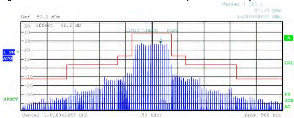
Figure 57 Plot of emissions with emission mask (Mode C2 / Ch. 1)
