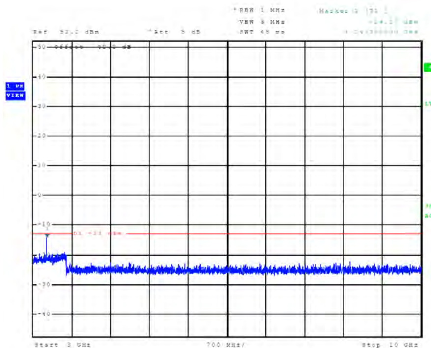
Figure 43 Plot of emissions across Frequency spectrum (Mode C8 / Ch. 121)
