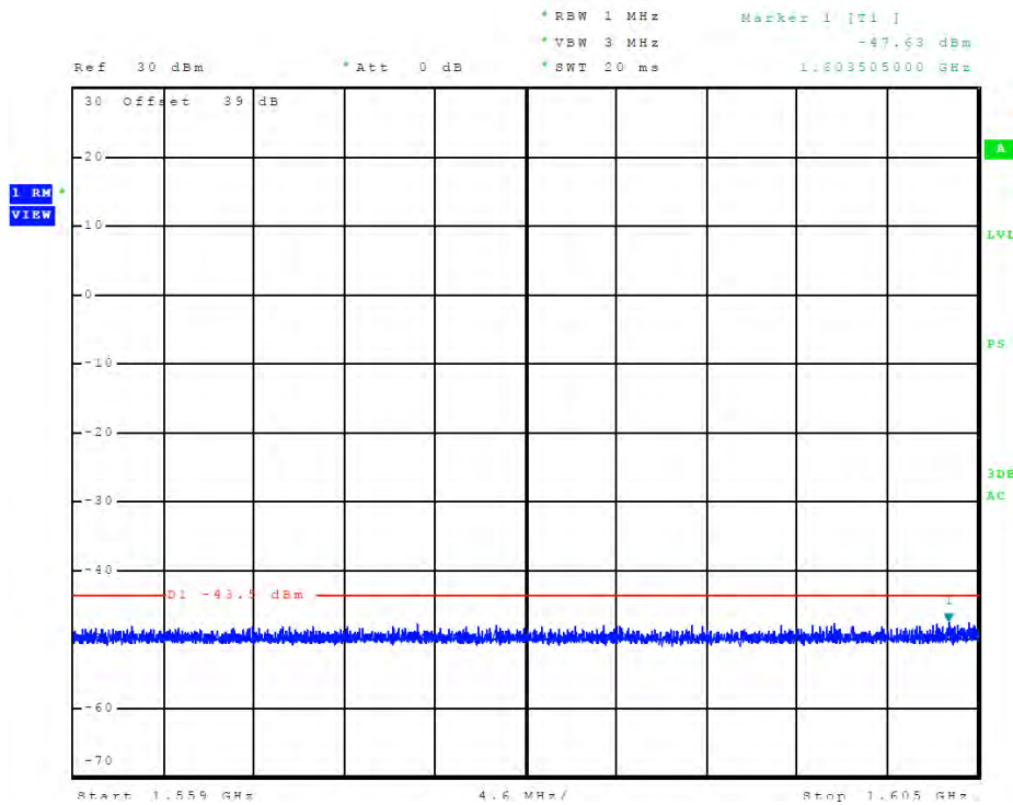
Figure 77 Plot of E.I.R.P. density of unwanted emissions (Mode B1 / Ch. 240)
