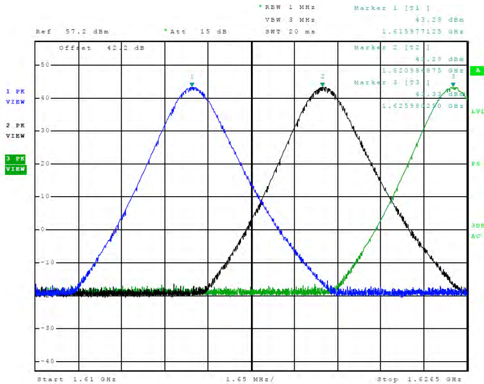
Figure 52 Plot of Operation across Frequency band (Mode B1)
