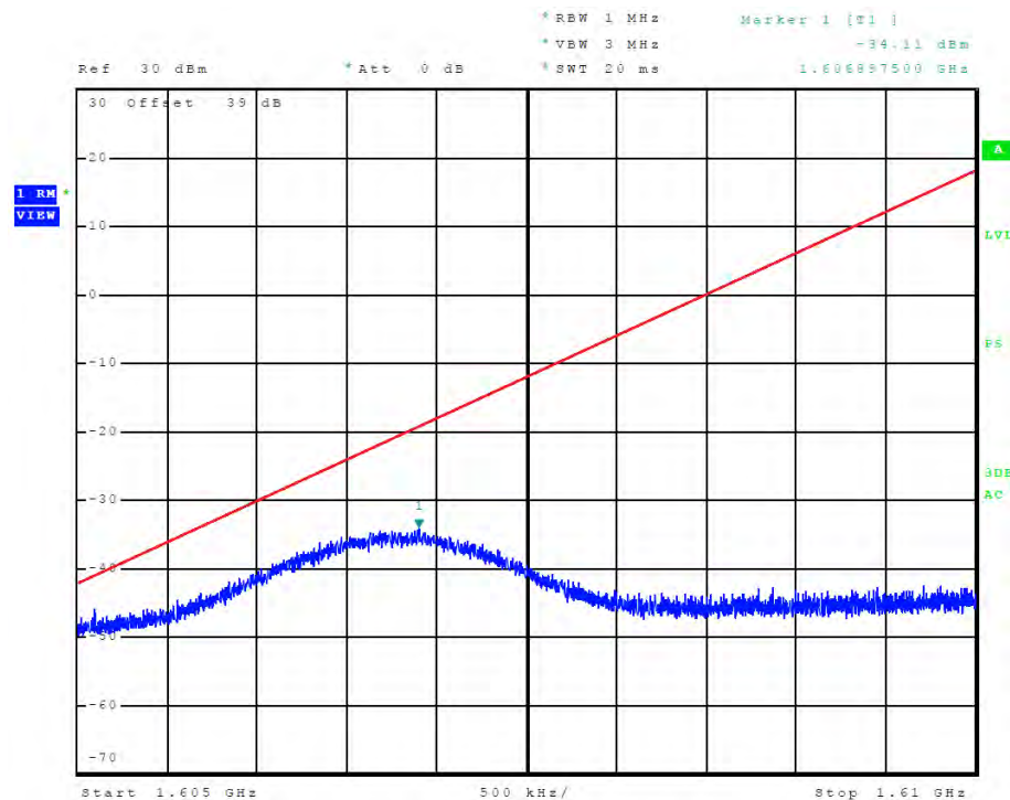
Figure 78 Plot of E.I.R.P. density of unwanted emissions (Mode B1 / Ch. 240)
