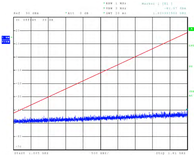
Figure 82 Plot of E.I.R.P. density of unwanted emissions (Mode C1 / Ch. 121)
