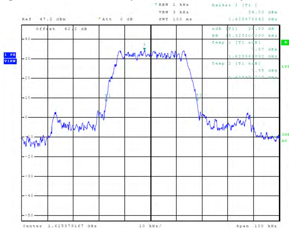
Figure 66 Plot of -26dB OBW (Mode B1 / Channel 240)
