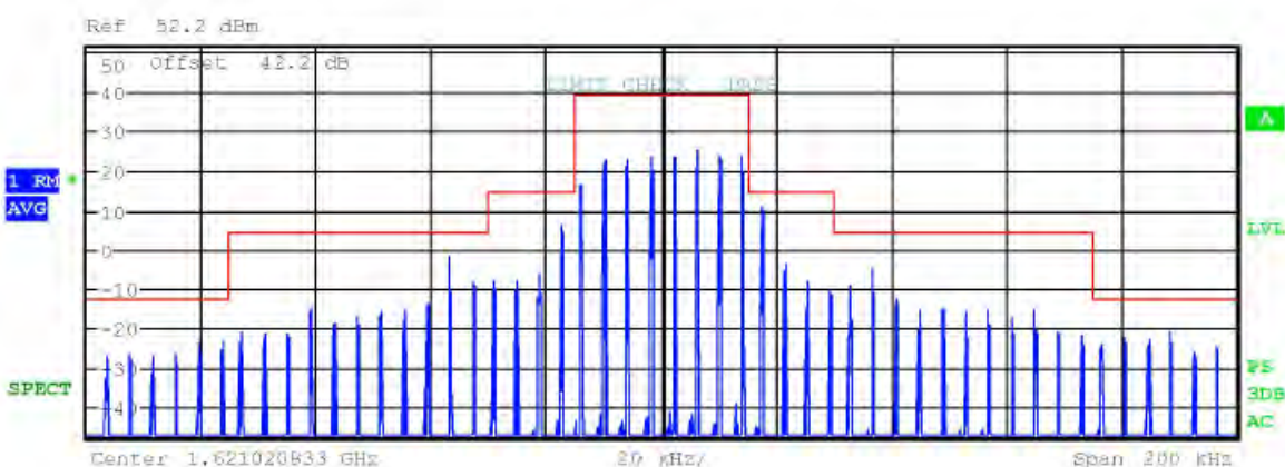
Figure 50 Plot of emissions with emission mask (Mode B1 / Ch. 101)
