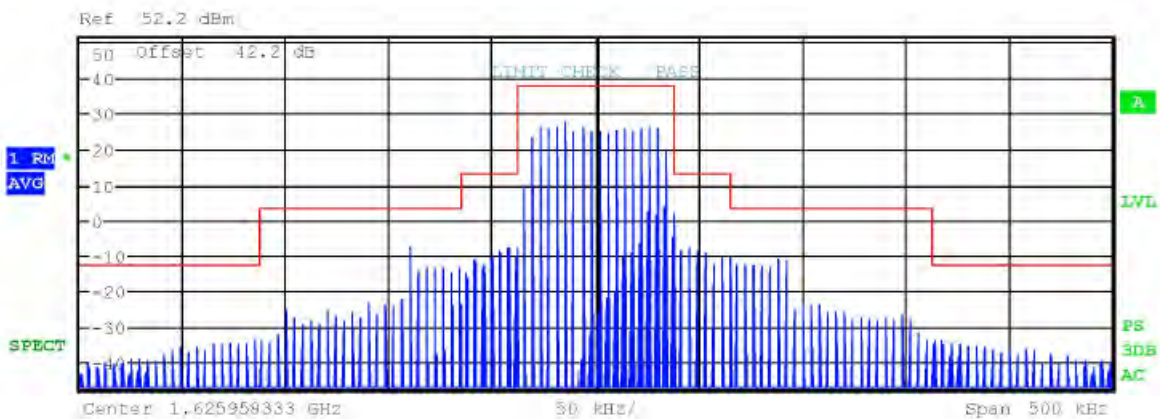
Figure 59 Plot of emissions with emission mask (Mode C2 / Ch. 240)
