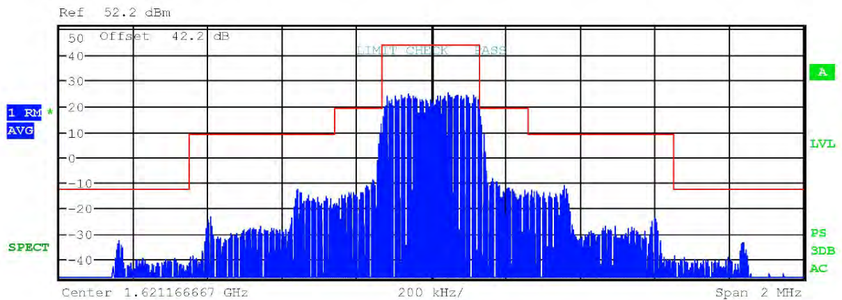
Figure 62 Plot of emissions with emission mask (Mode C8 / Ch. 121)
