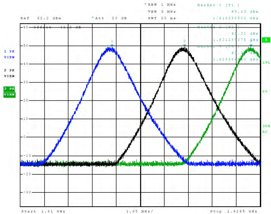
Figure 64 Plot of Operation across Frequency band (Mode C8)
