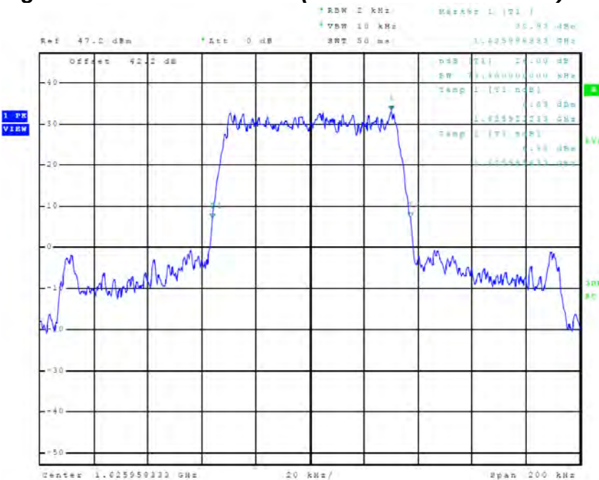
Figure 72 Plot of -26dB OBW (Mode C8 / Channel 240)
