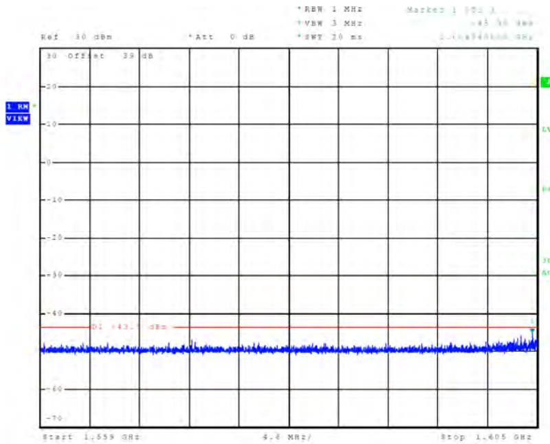
Figure 79 Plot of E.I.R.P. density of unwanted emissions (Mode C1 / Ch. 1)
