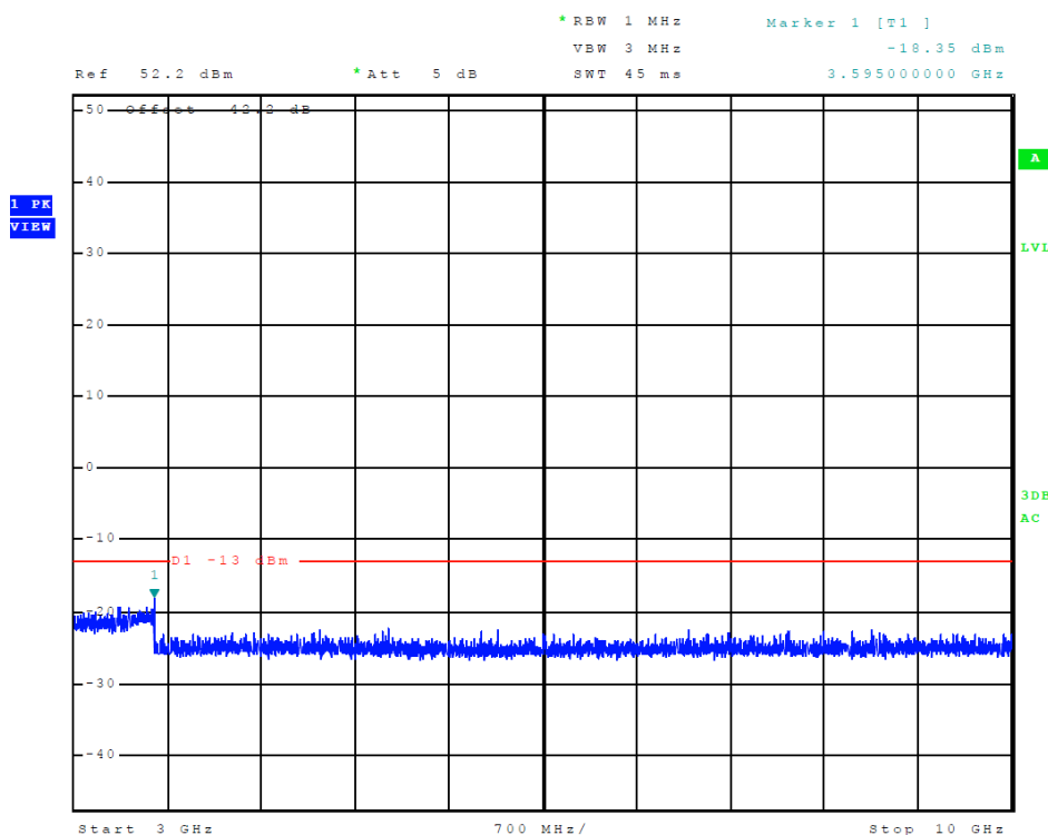
Figure 27 Plot of emissions across Frequency spectrum (Mode C2 / Ch. 1)
