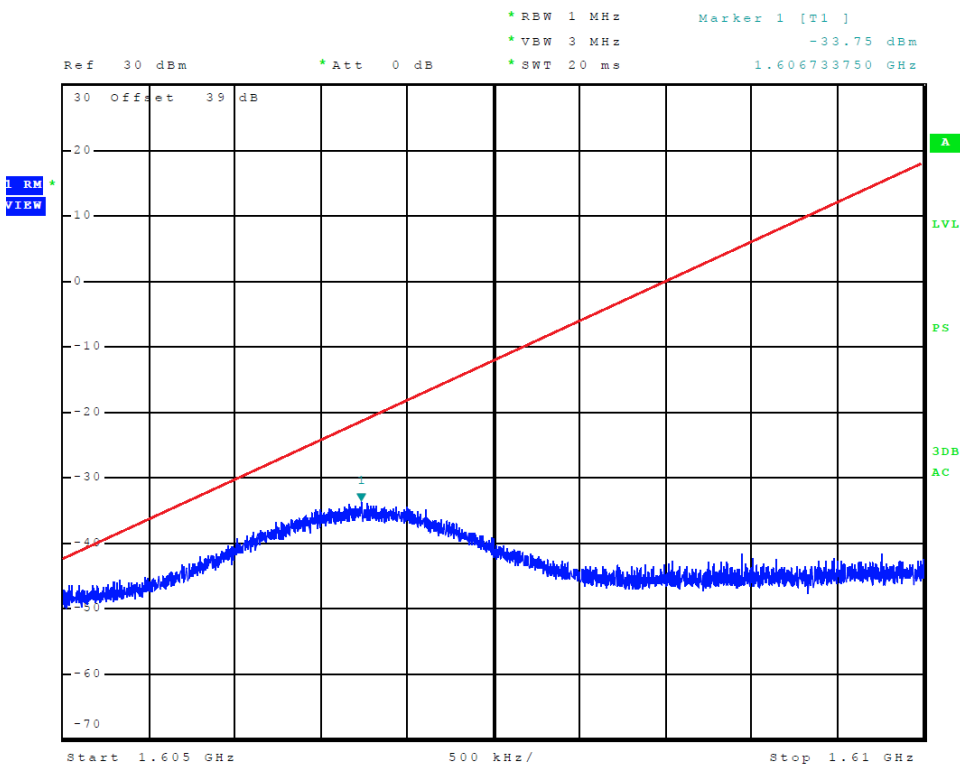
Figure 90 Plot of E.I.R.P. density of unwanted emissions (Mode C2 / Ch. 240)
