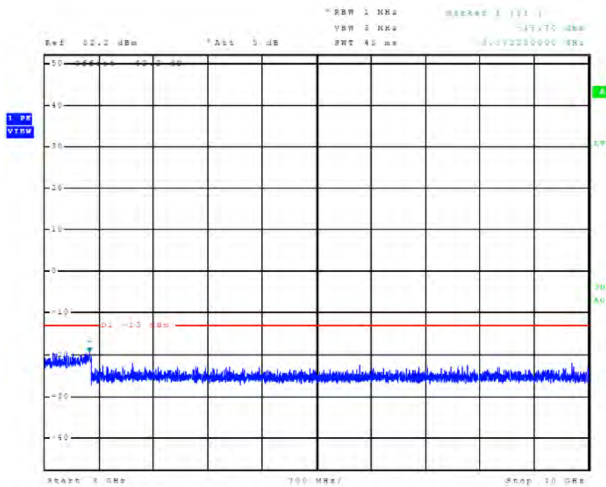
Figure 35 Plot of emissions across Frequency spectrum (Mode C2 / Ch. 240)
