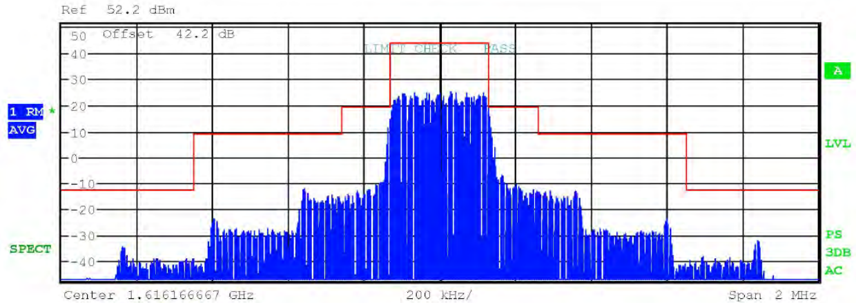
Figure 61 Plot of emissions with emission mask (Mode C8 / Ch. 1)
