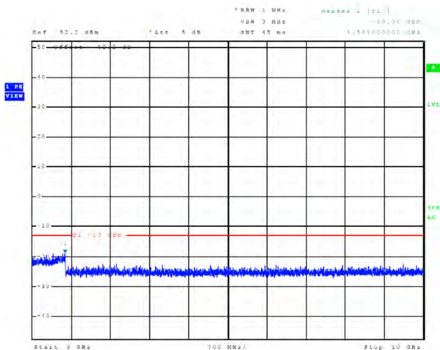
Figure 31 Plot of emissions across Frequency spectrum (Mode C2 / Ch. 121)
