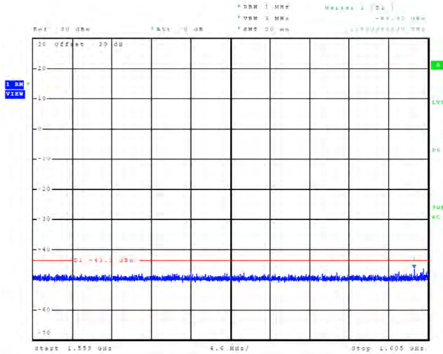
Figure 95 Plot of E.I.R.P. density of unwanted emissions (Mode C8 / Ch. 240)
