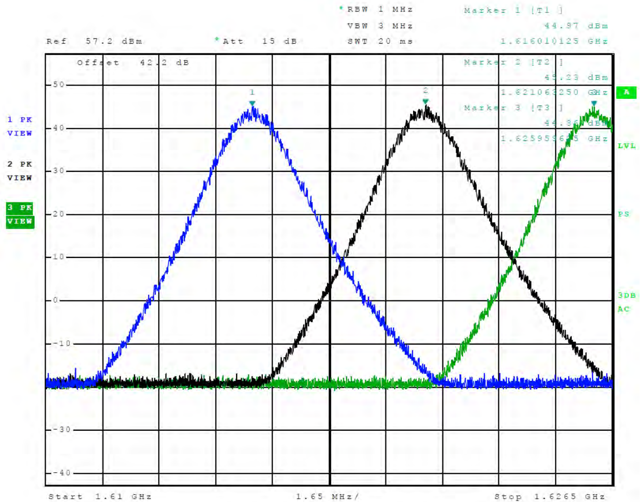
Figure 56 Plot of Operation across Frequency band (Mode C1)
