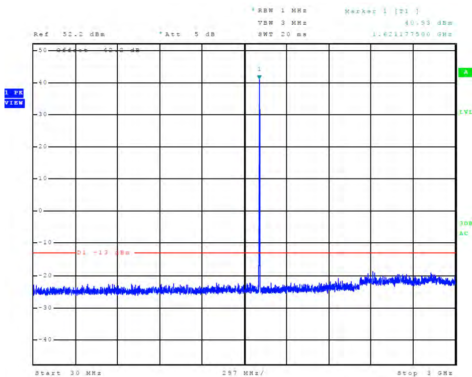
Figure 30 Plot of emissions across Frequency spectrum (Mode C2 / Ch. 121)
