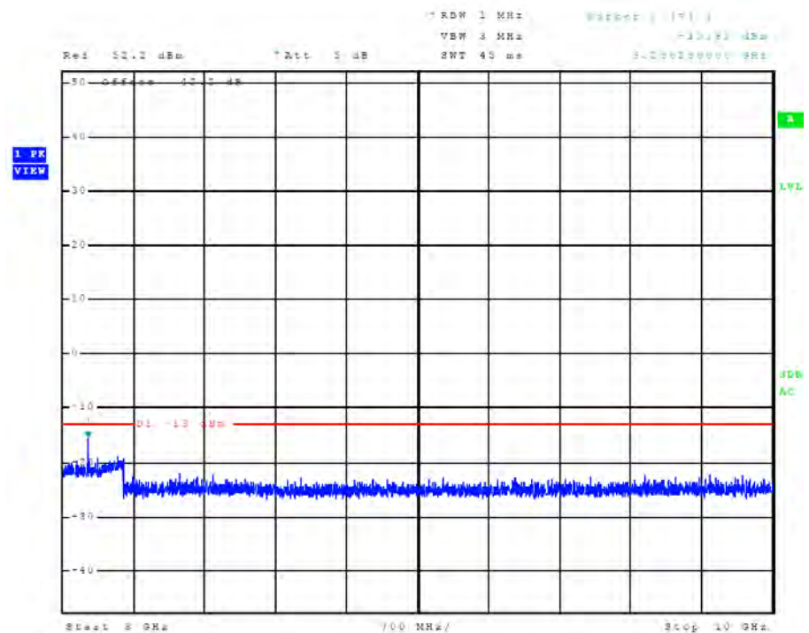
Figure 47 Plot of emissions across Frequency spectrum (Mode C8 / Ch. 240)
