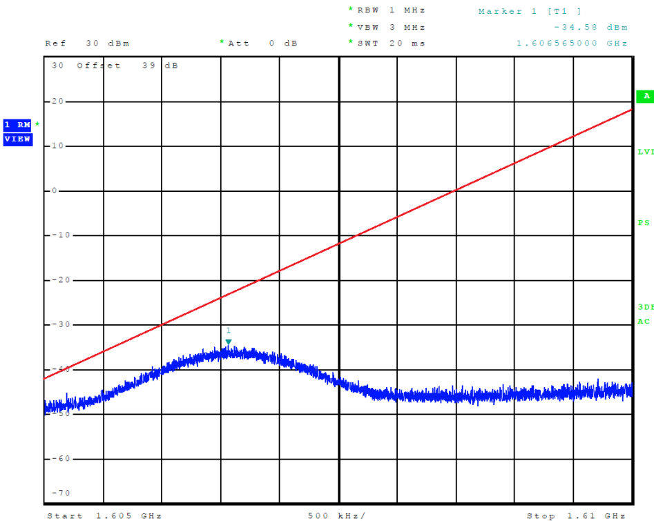
Figure 96 Plot of E.I.R.P. density of unwanted emissions (Mode C8 / Ch. 240)
