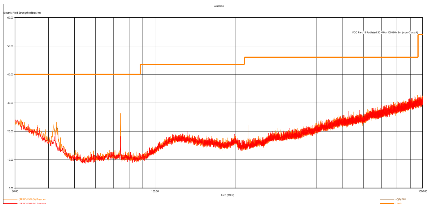
Figure 7 - Radiated Emissions Plot, GMSK 1MB
