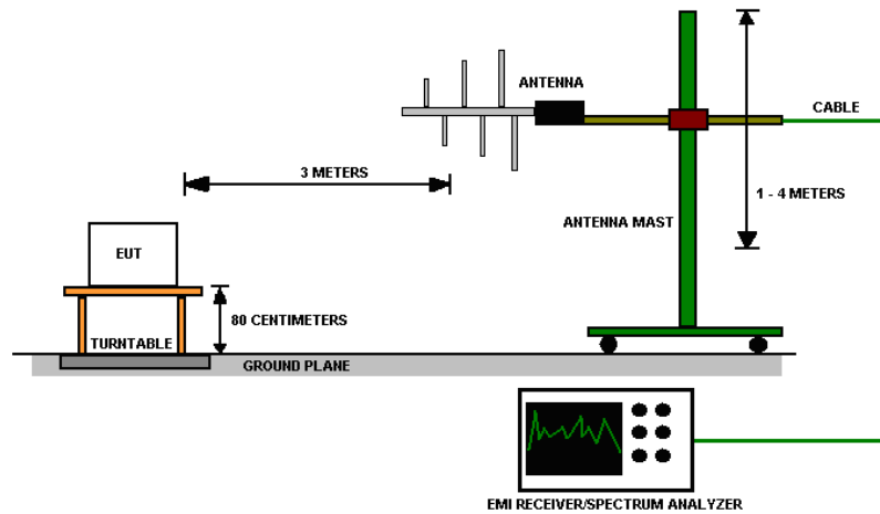
Figure 17 - Radiated Emissions Test Setup
