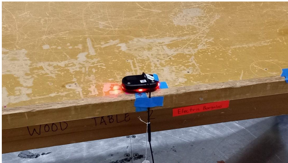
30 MHz – 1 GHz Test Setup
