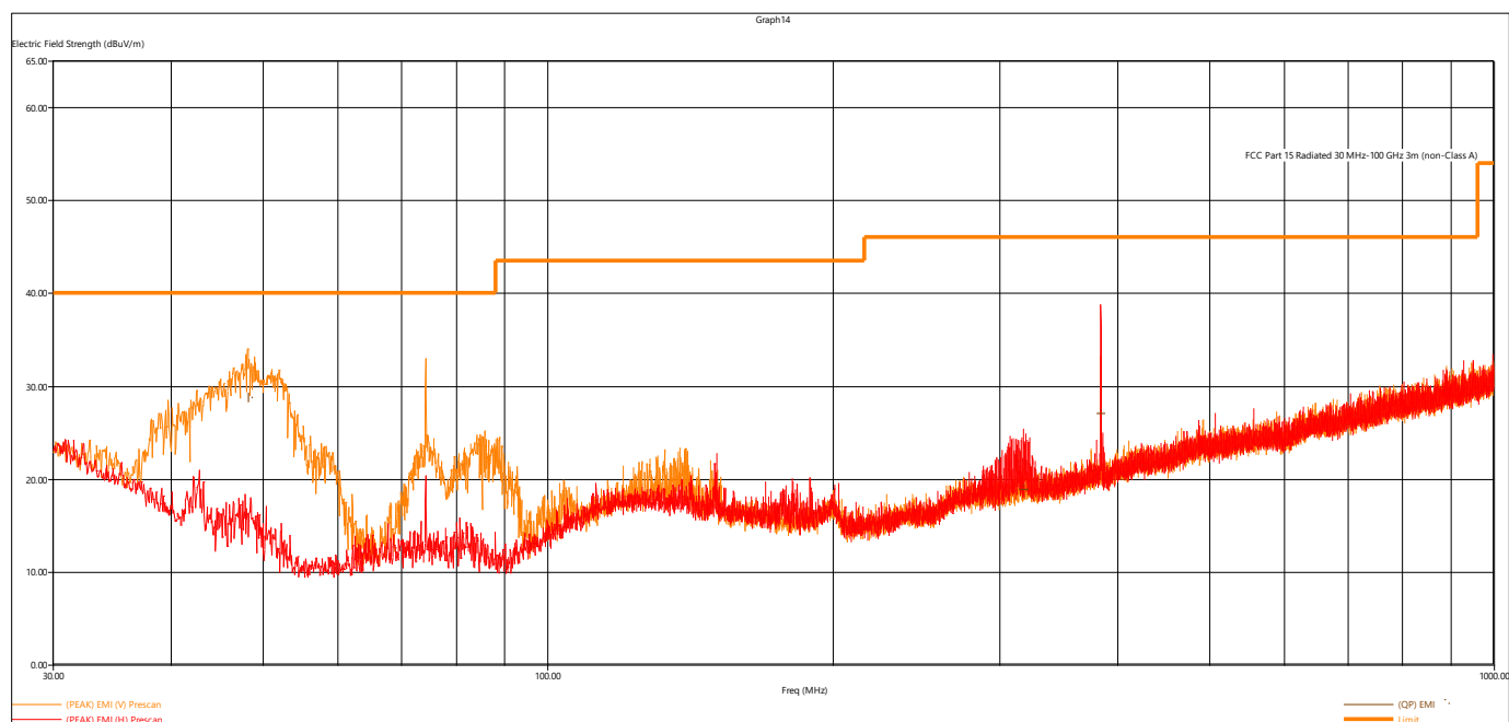
Figure 7 - Radiated Emissions Plot, GFSK
