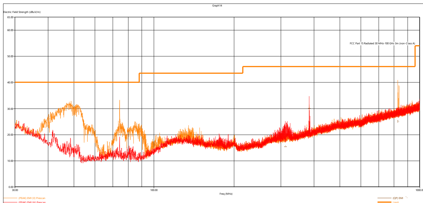
Figure 9 - Radiated Emissions Plot, GMSK 2MB
