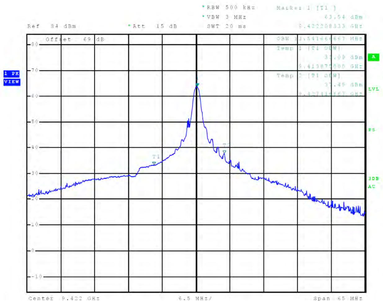
Figure 21 99% Occupied Bandwidth Plot, 96 nm
