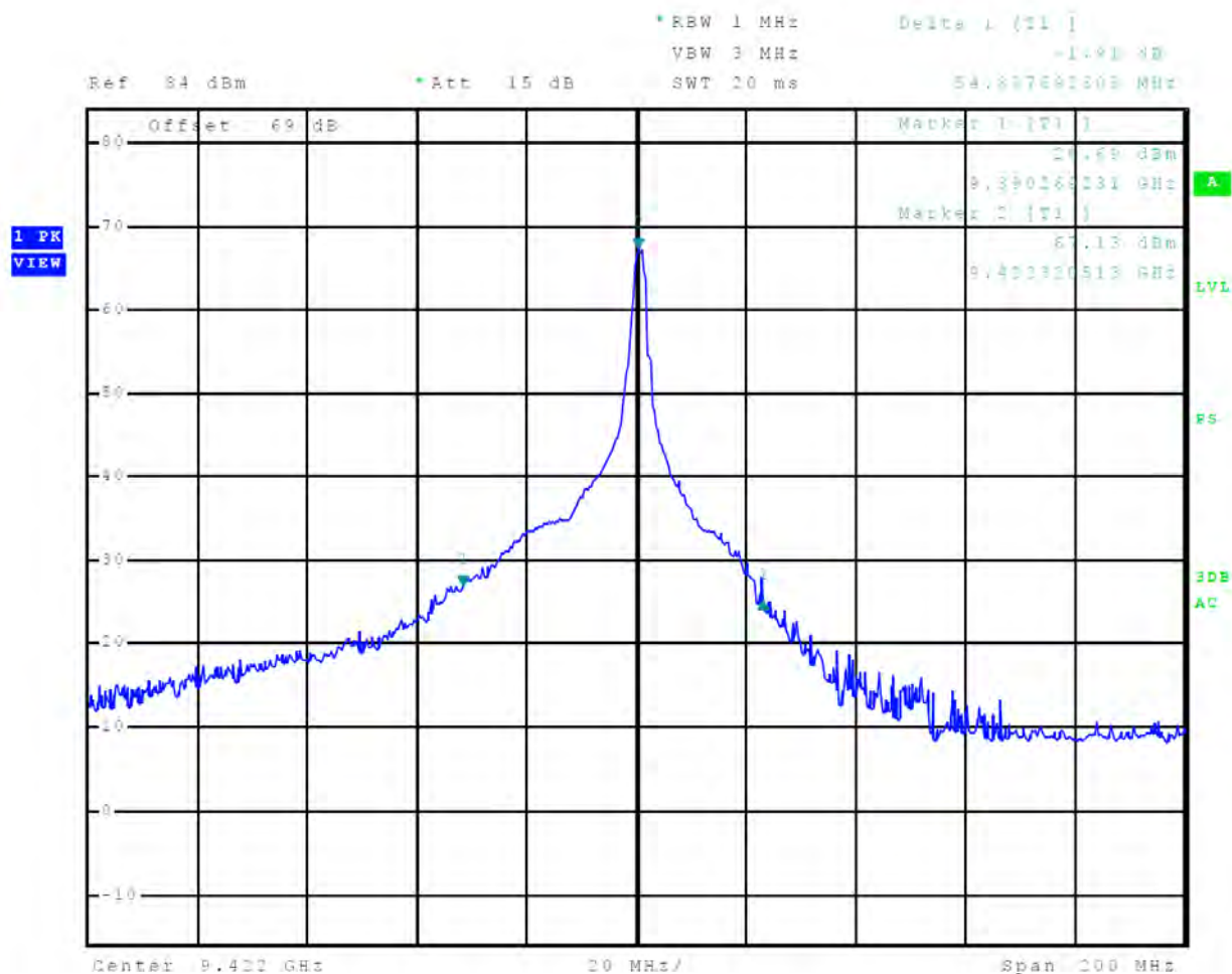
Figure 38 40-dB Occupied Bandwidth Plot, 48 nm
