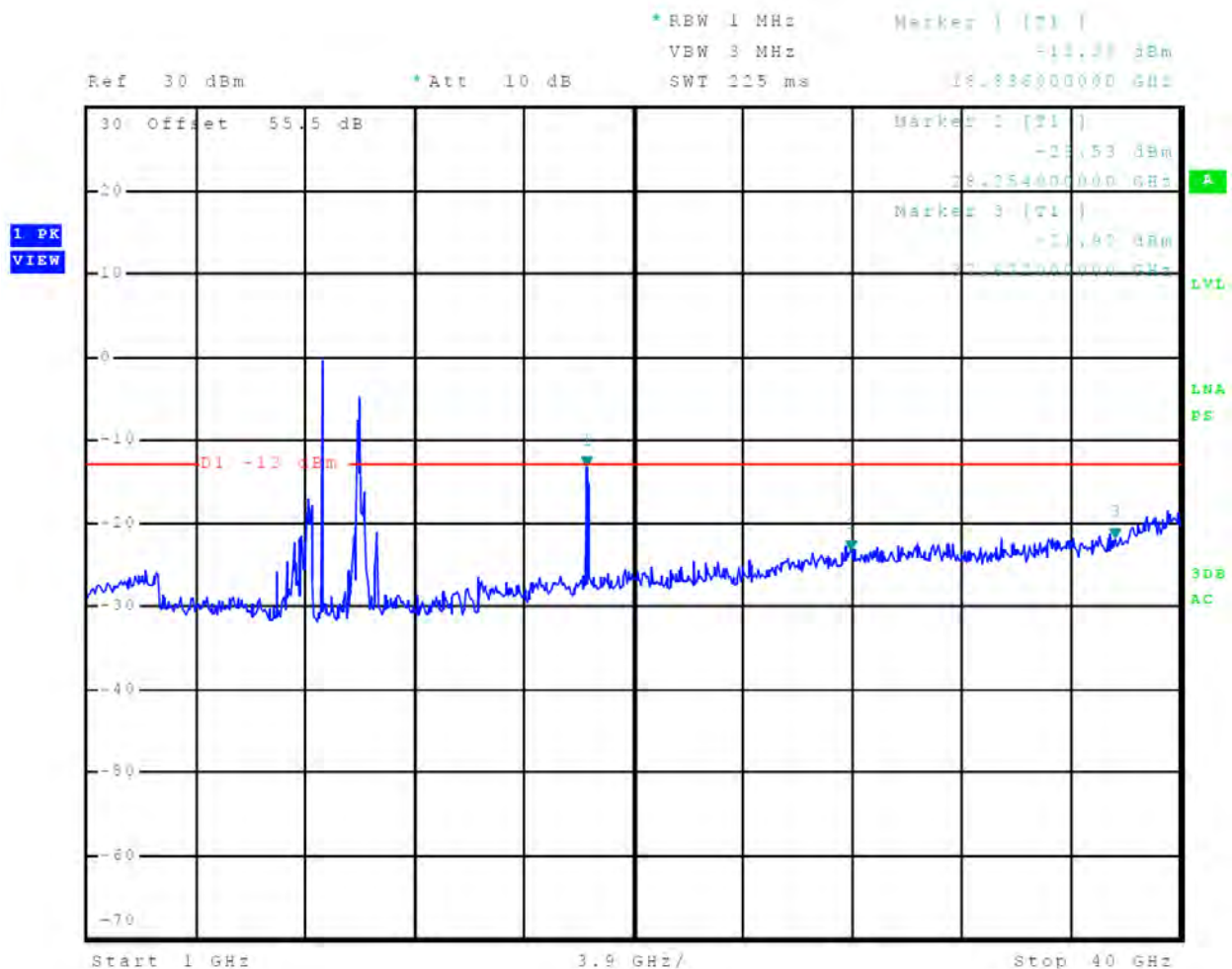
Figure 69 Out-of-Band Emissions 1/2 nm
