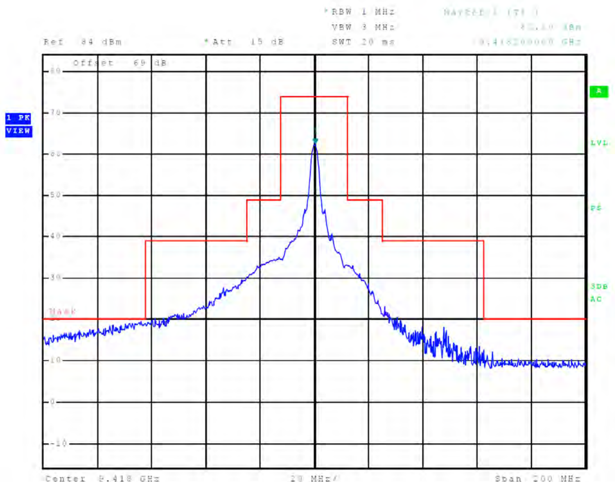
Figure 48 Emissions Mask, 1.5 nm
