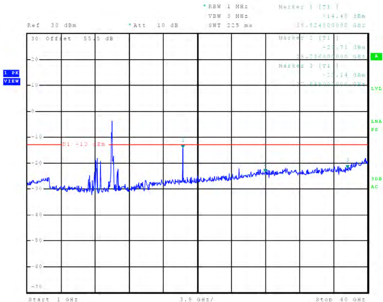
Figure 83 Out-of-Band Emissions 6 nm
