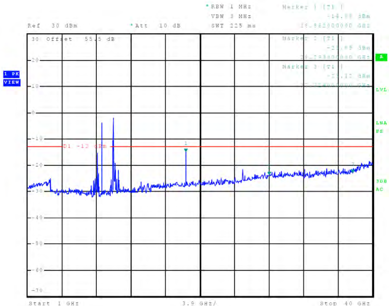
Figure 91 Out-of-Band Emissions 24 nm
