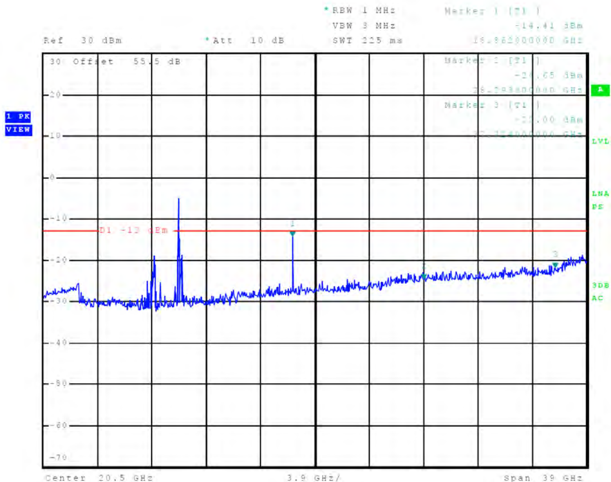
Figure 93 Out-of-Band Emissions 36 nm
