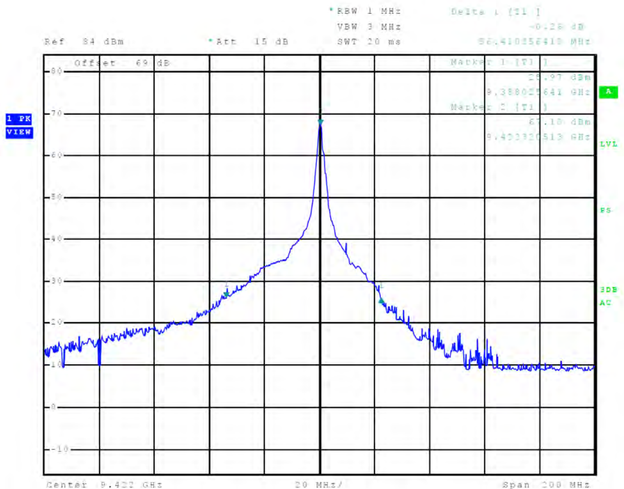
Figure 39 40-dB Occupied Bandwidth Plot, 64 nm
