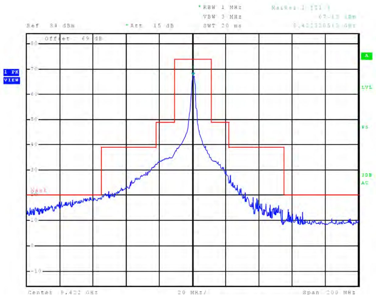
Figure 58 Emissions Mask, 48 nm
