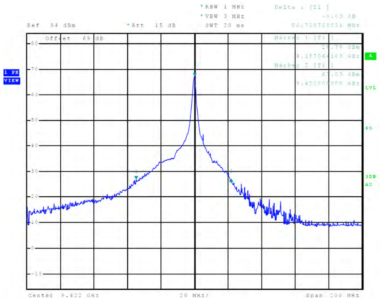
Figure 41 40-dB Occupied Bandwidth Plot, 96 nm
