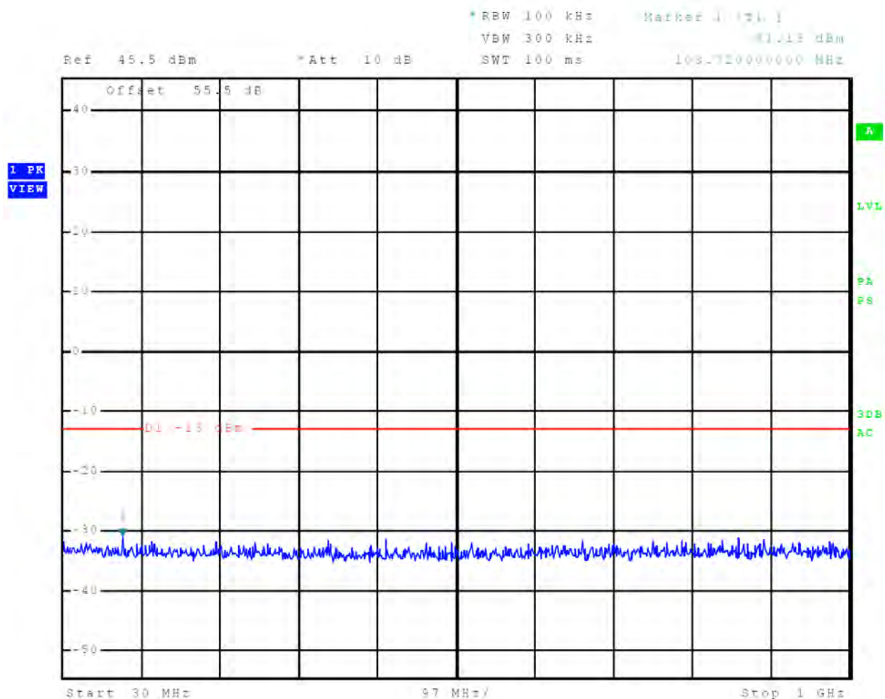
Figure 70 Out-of-Band Emissions 3/4 nm
