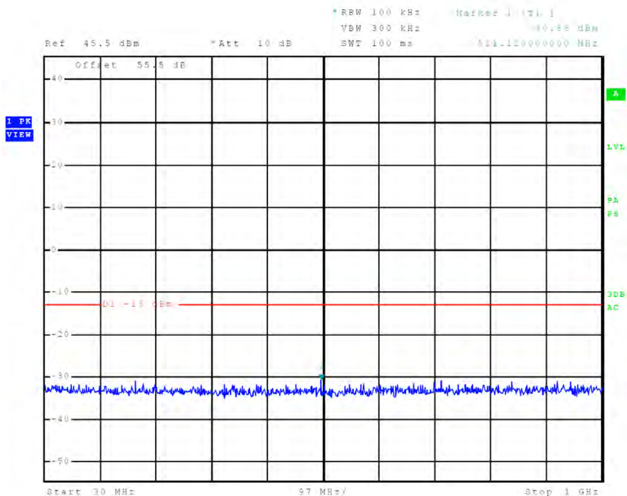
Figure 78 Out-of-Band Emissions 3 nm
