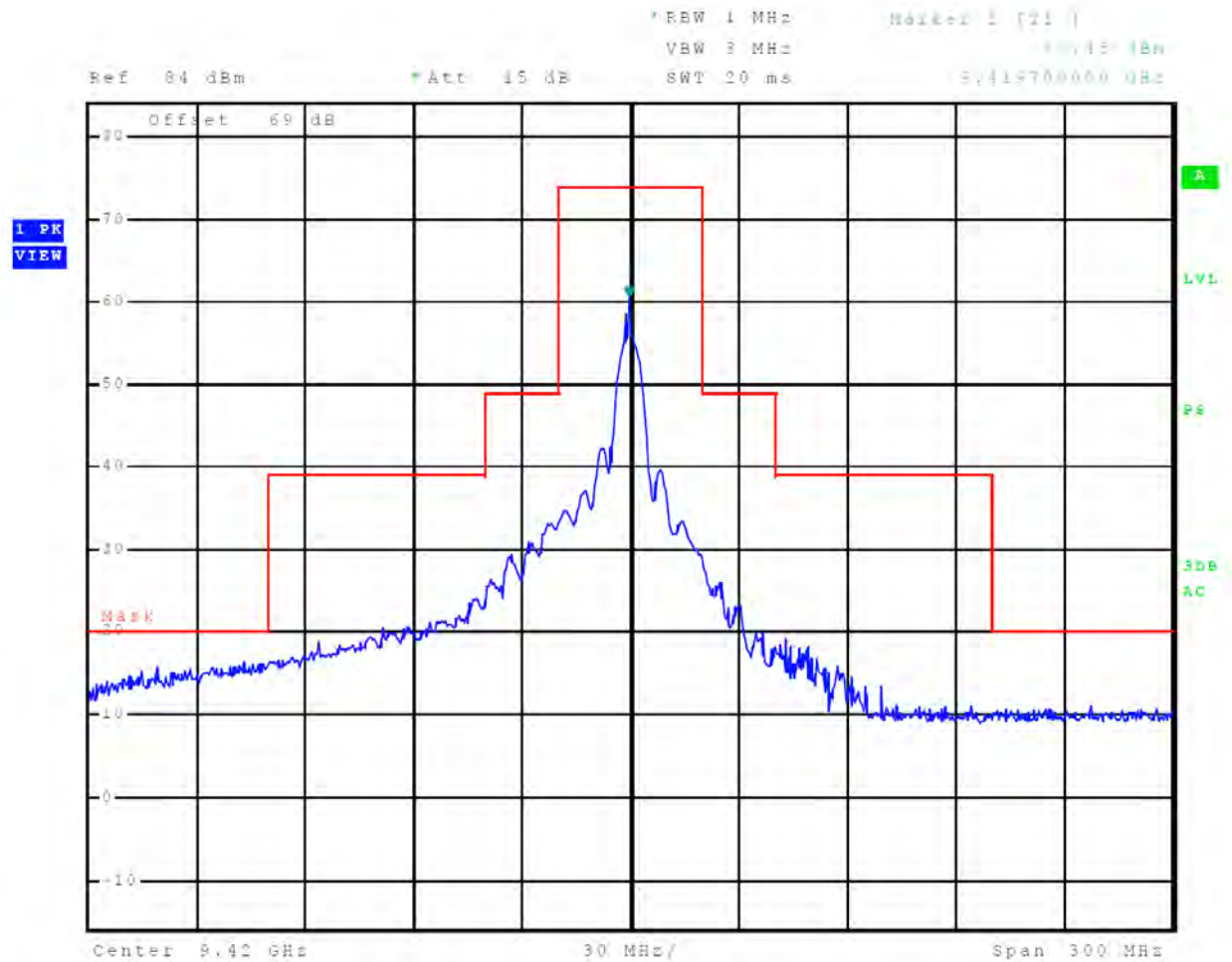
Figure 46 Emissions Mask, 3/4 nm
