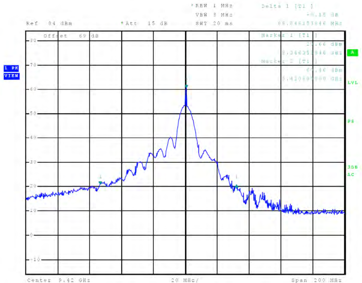
Figure 24 40-dB Occupied Bandwidth Plot, 1/4 nm
