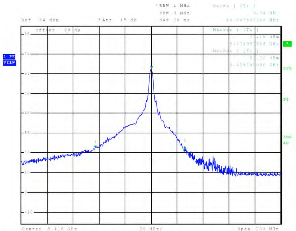
Figure 28 40-dB Occupied Bandwidth Plot, 1.5 nm
