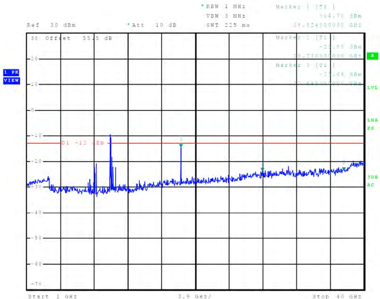
Figure 75 Out-of-Band Emissions 1.5 nm
