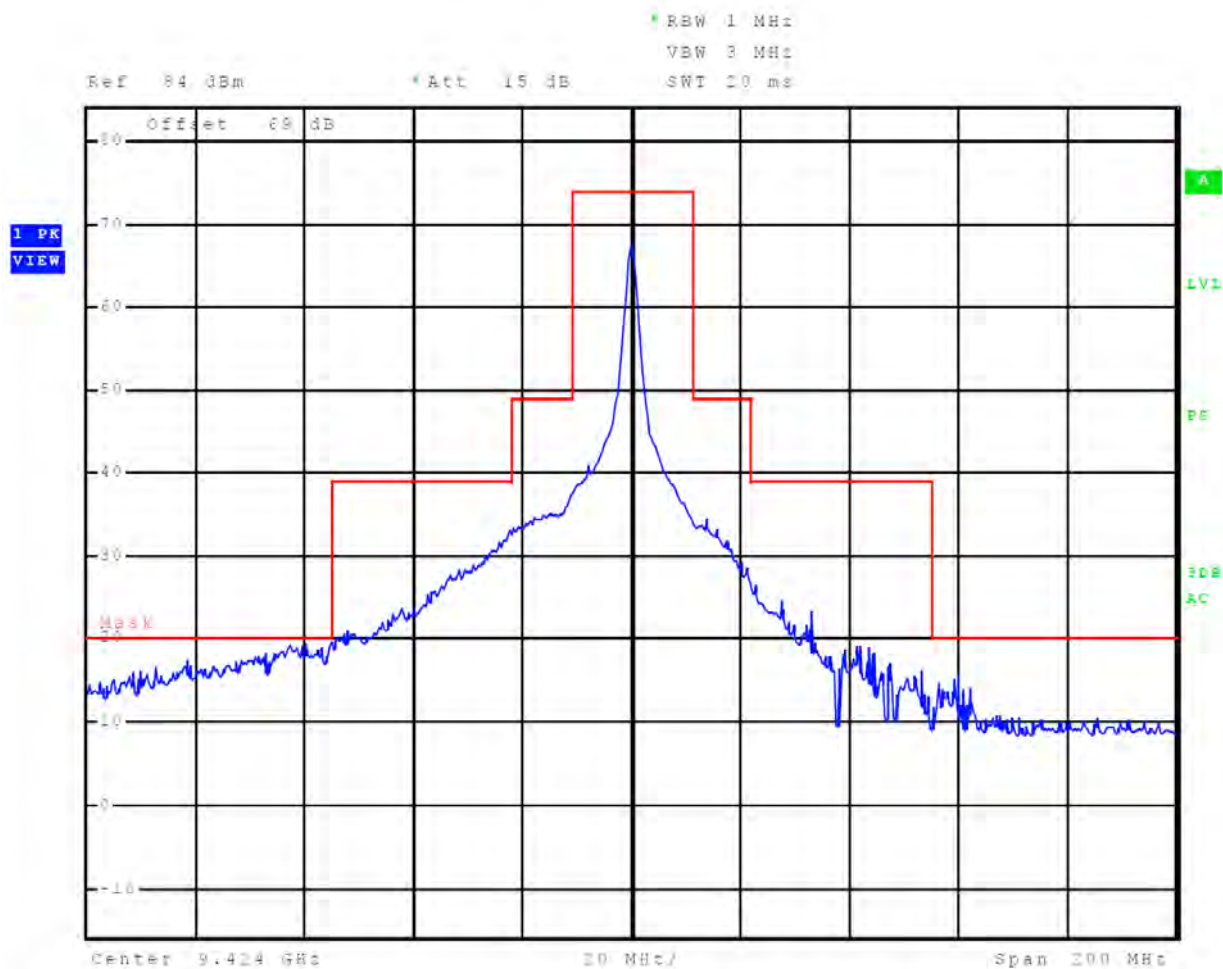
Figure 51 Emissions Mask, 4 nm
