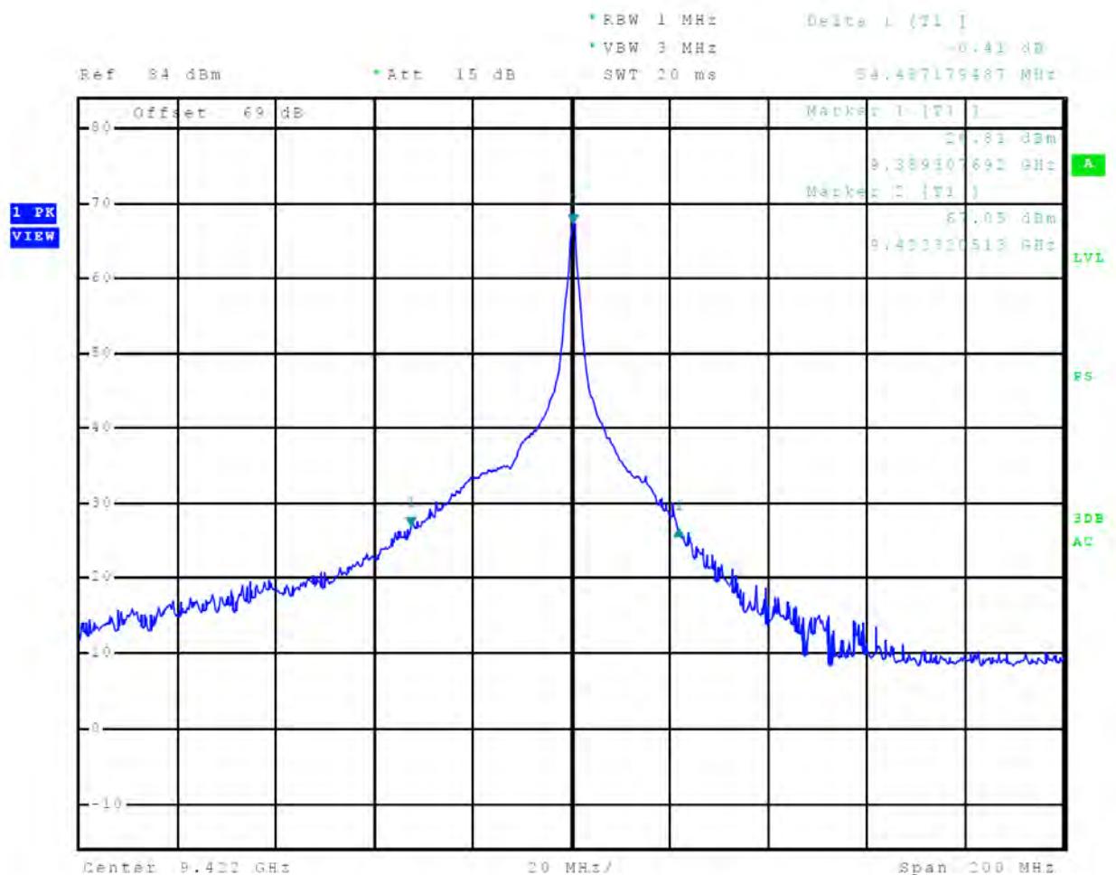
Figure 40 40-dB Occupied Bandwidth Plot, 72 nm
