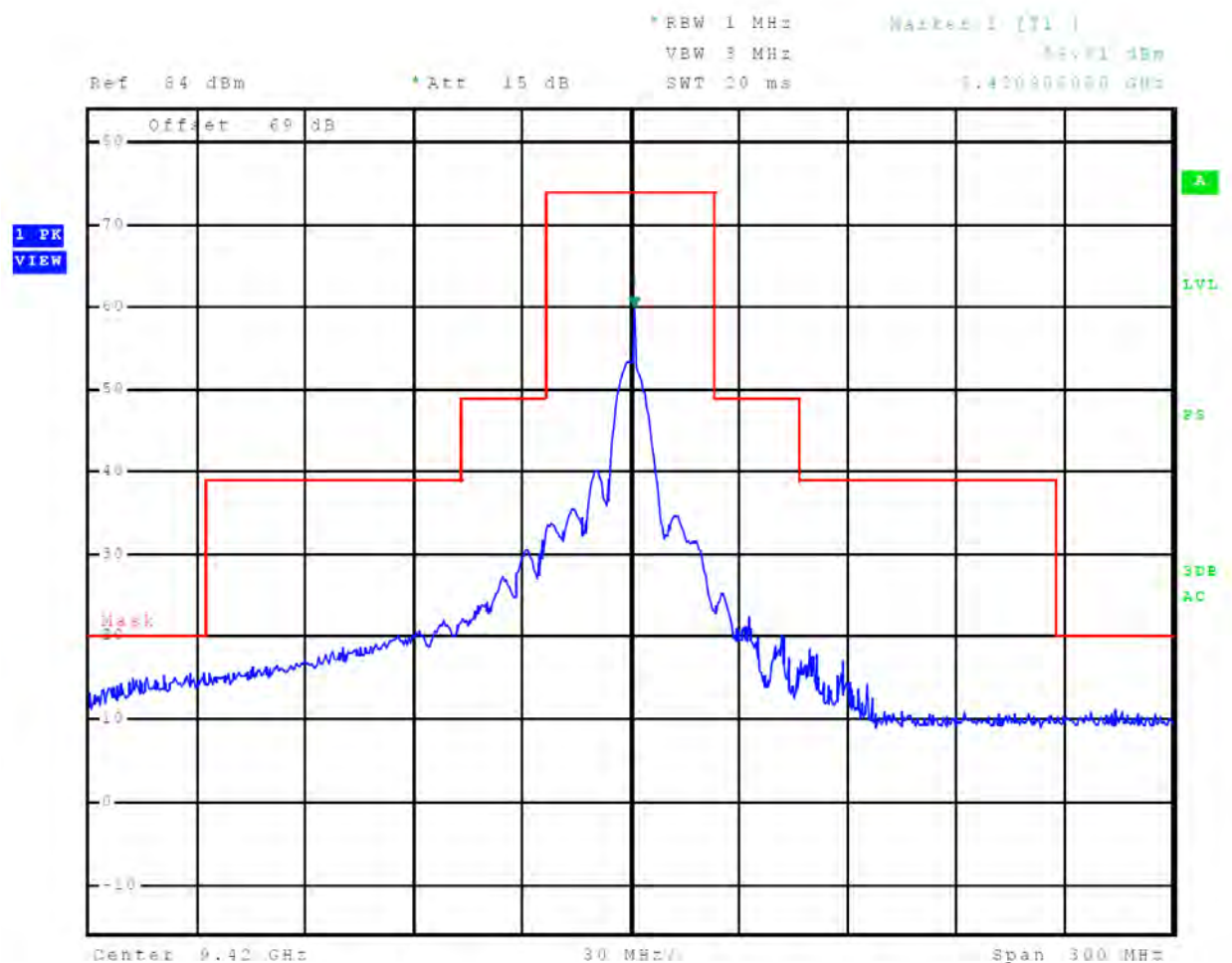
Figure 42 Emissions Mask, 1/16 nm
