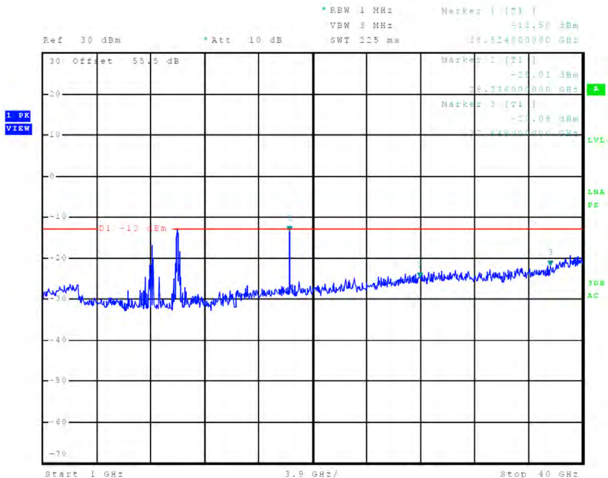
Figure 71 Out-of-Band Emissions 3/4 nm
