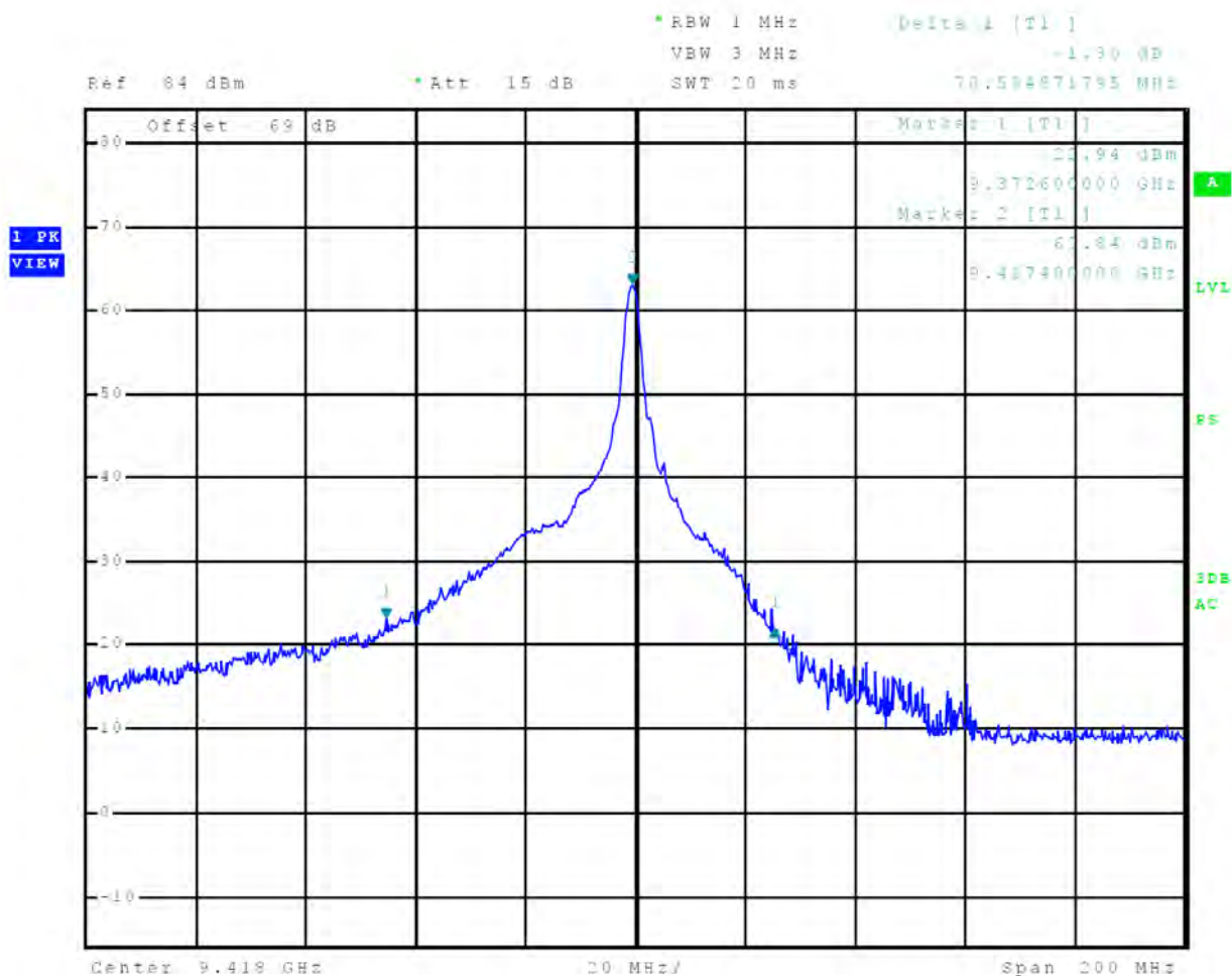
Figure 29 40-dB Occupied Bandwidth Plot, 2 nm
