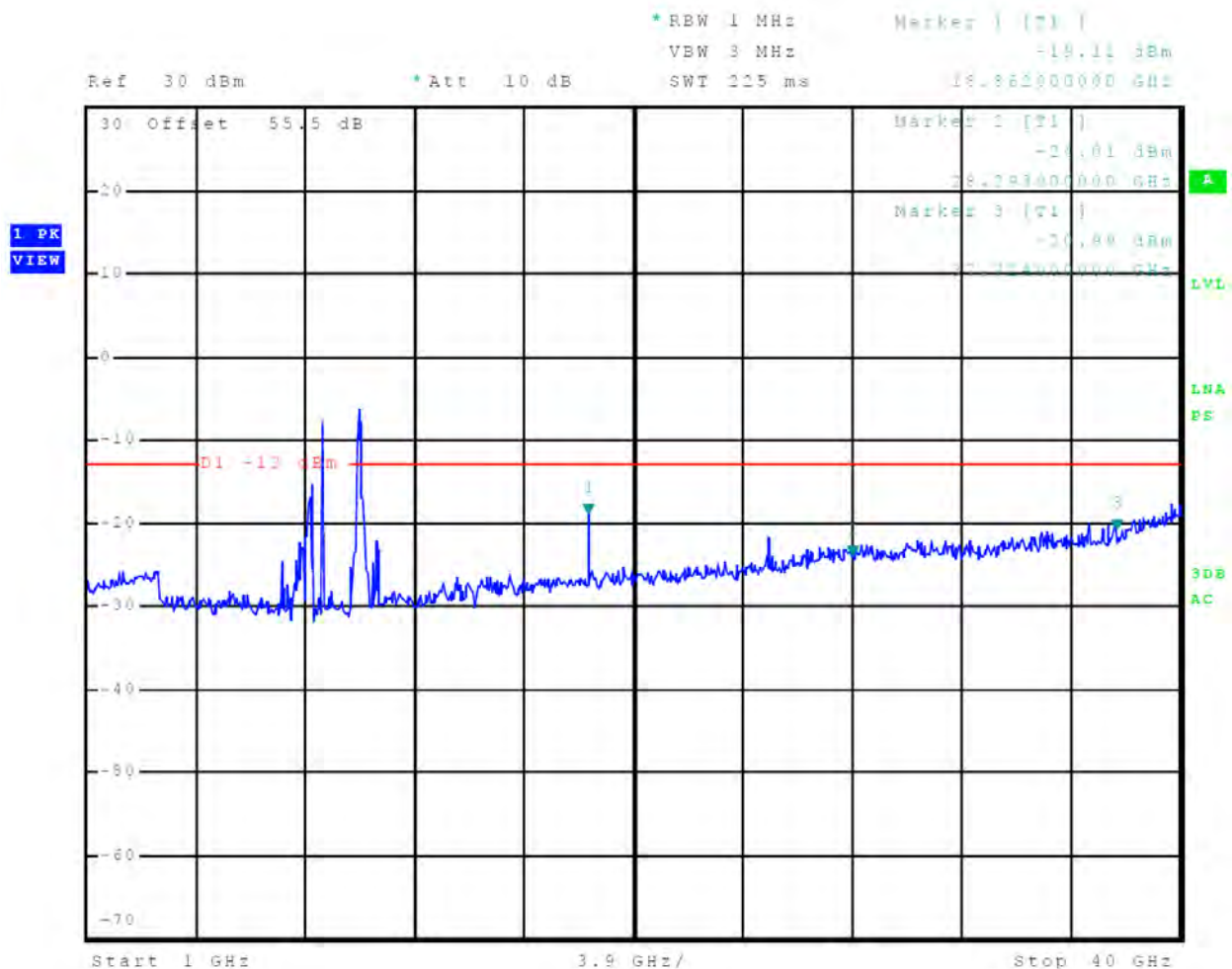
Figure 87 Out-of-Band Emissions 12 nm
