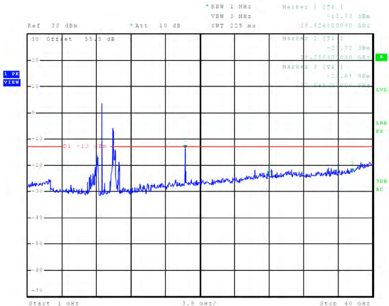
Figure 73 Out-of-Band Emissions 1 nm
