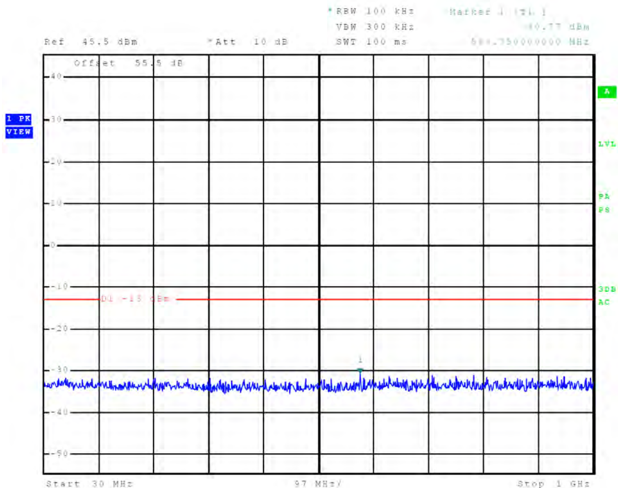
Figure 66 Out-of-Band Emissions 1/4 nm
