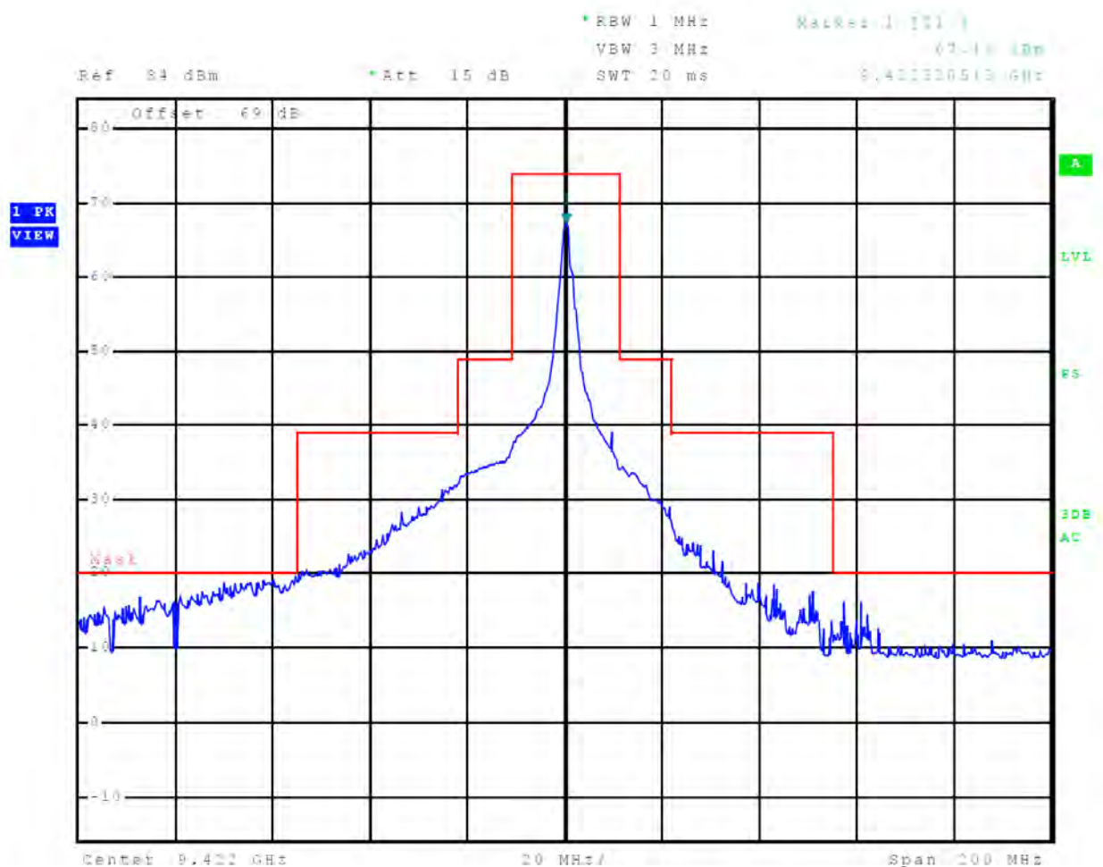
Figure 59 Emissions Mask, 64 nm
