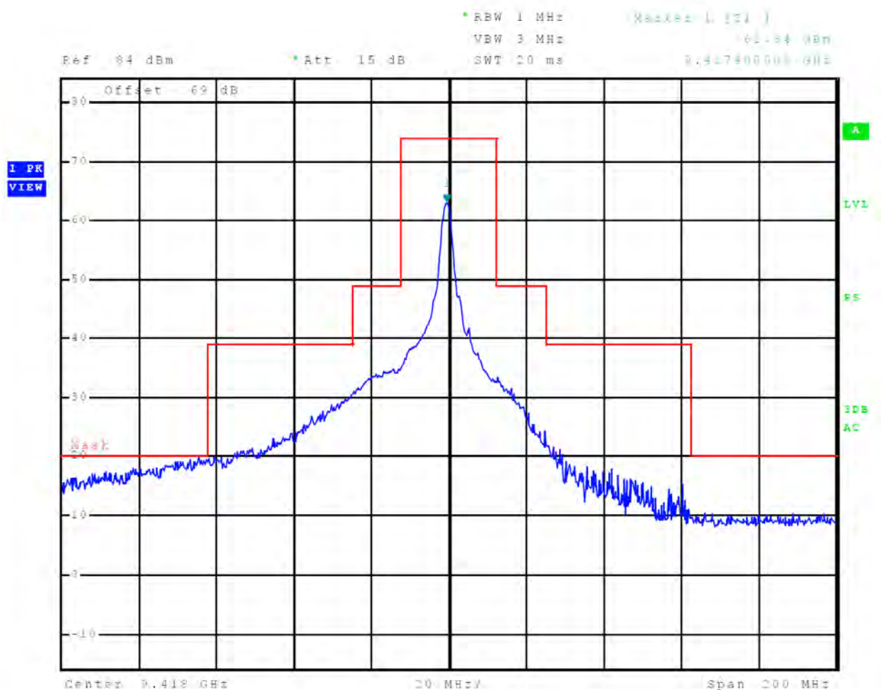
Figure 49 Emissions Mask, 2 nm
