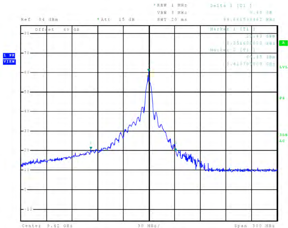
Figure 26 40-dB Occupied Bandwidth Plot, 3/4 nm
