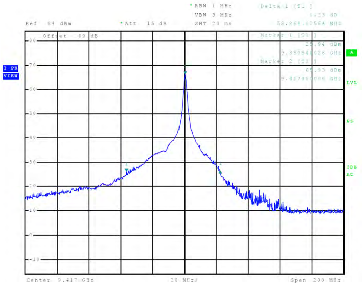
Figure 30 40-dB Occupied Bandwidth Plot, 3 nm
