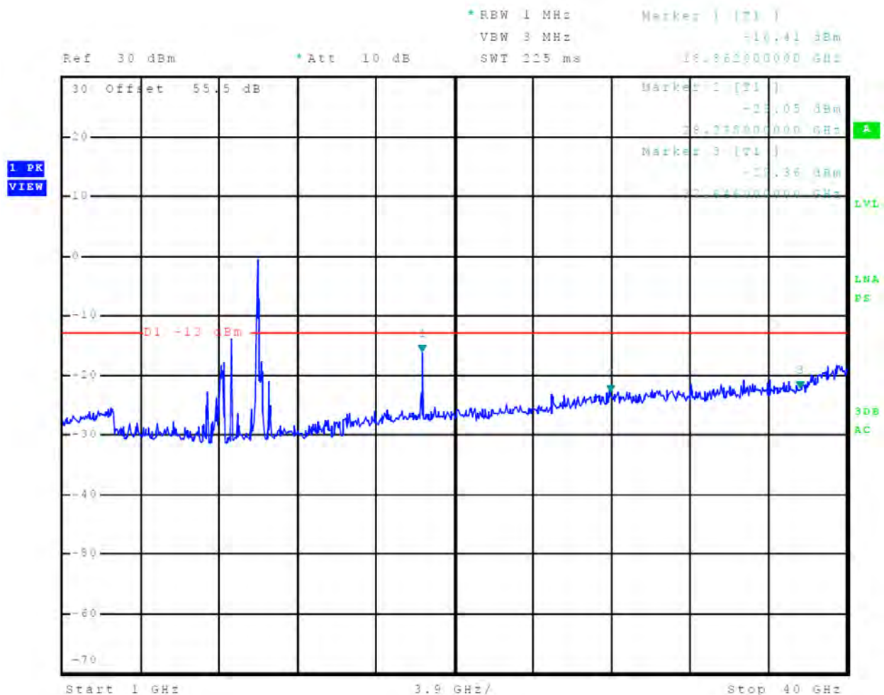
Figure 101 Out-of-Band Emissions 96 nm
