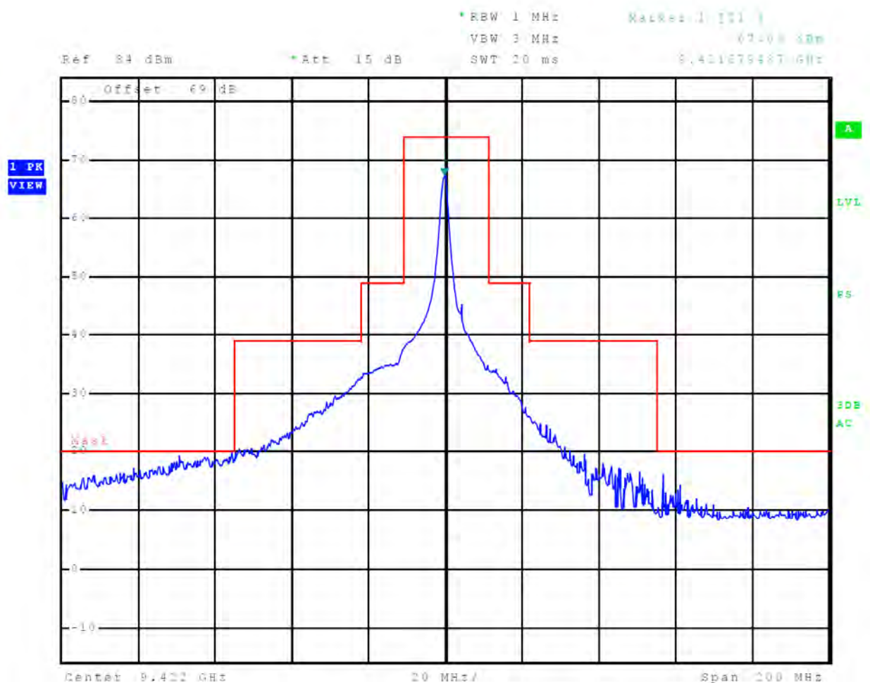
Figure 56 Emissions Mask, 24 nm
