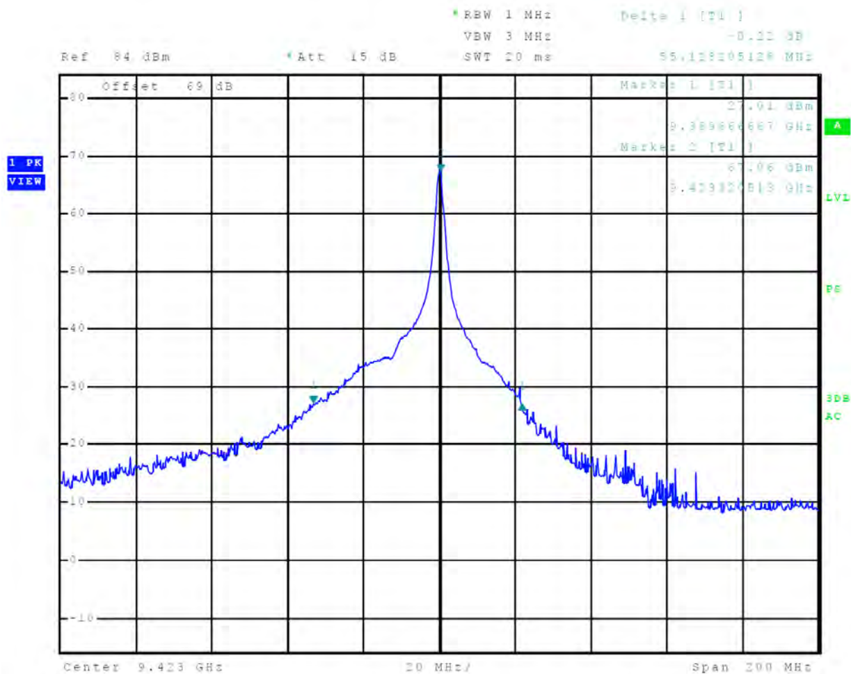
Figure 32 40-dB Occupied Bandwidth Plot, 6 nm
