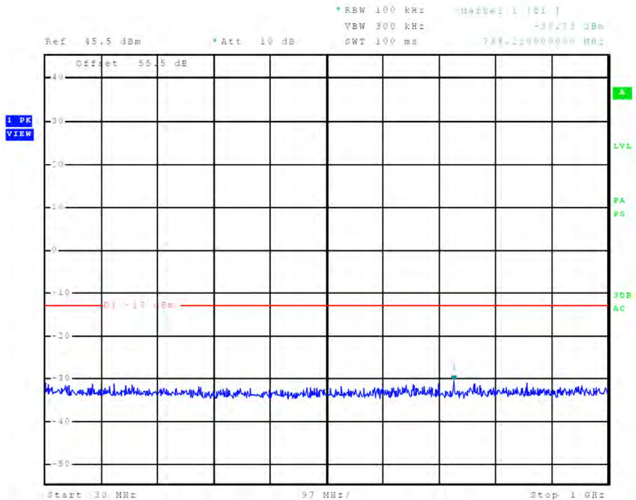
Figure 90 Out-of-Band Emissions 24 nm
