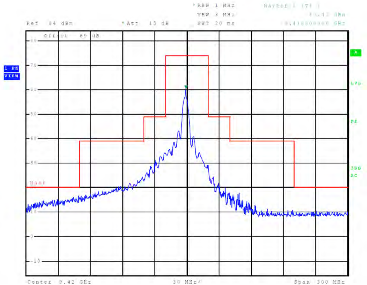
Figure 47 Emissions Mask, 1 nm
