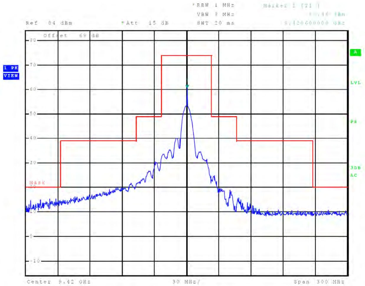
Figure 44 Emissions Mask, 1/4 nm
