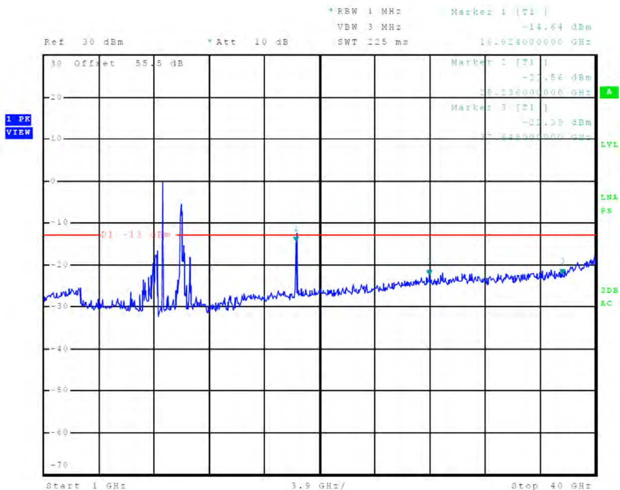
Figure 63 Out-of-Band Emissions 1/16 nm
