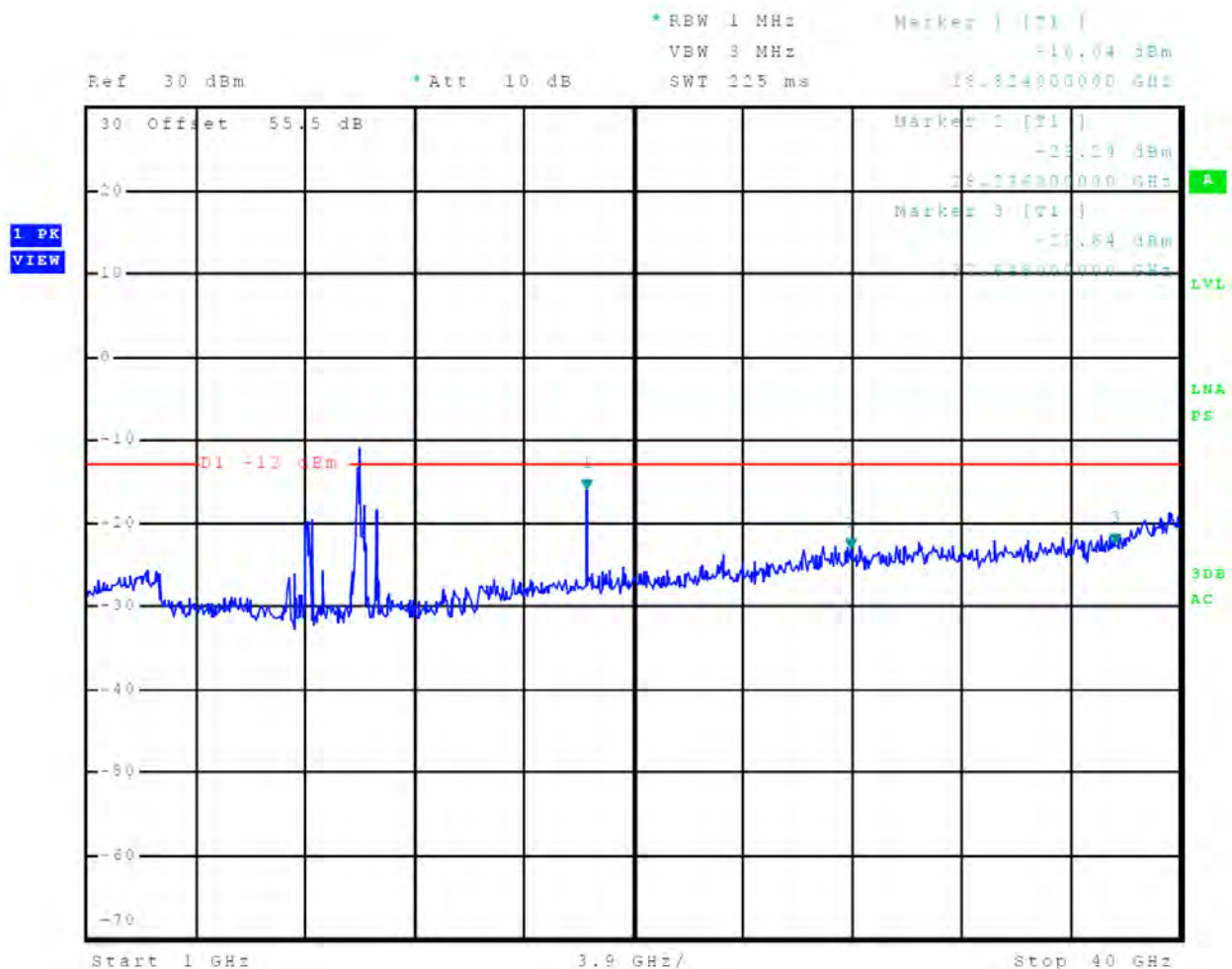
Figure 81 Out-of-Band Emissions 4 nm
