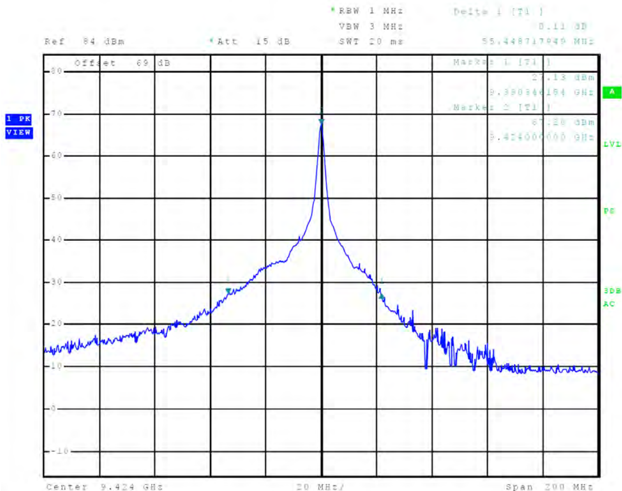
Figure 31 40-dB Occupied Bandwidth Plot, 4 nm
