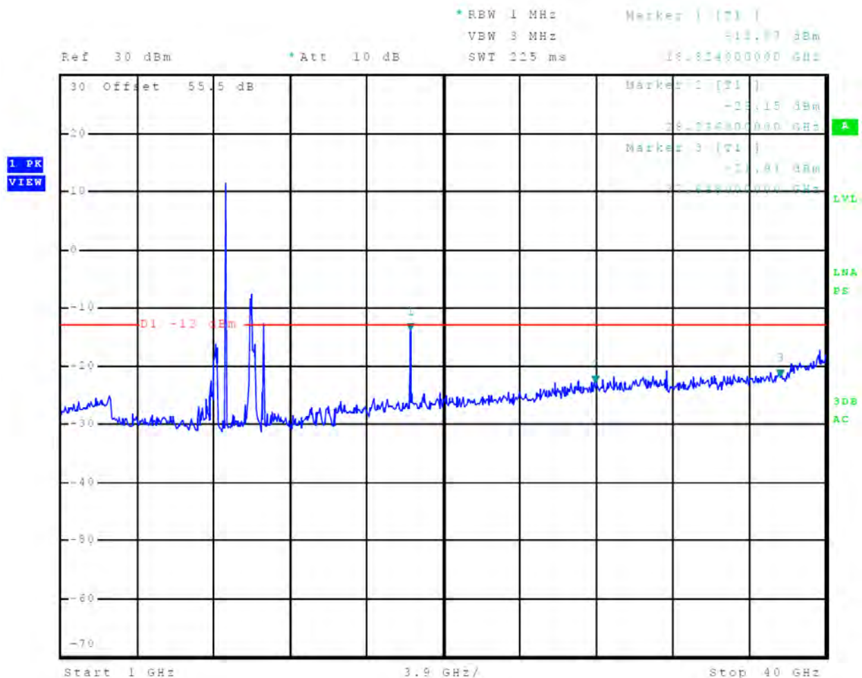
Figure 79 Out-of-Band Emissions 3 nm
