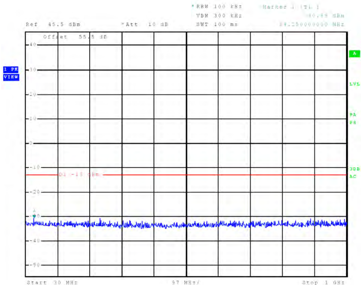
Figure 76 Out-of-Band Emissions 2 nm
