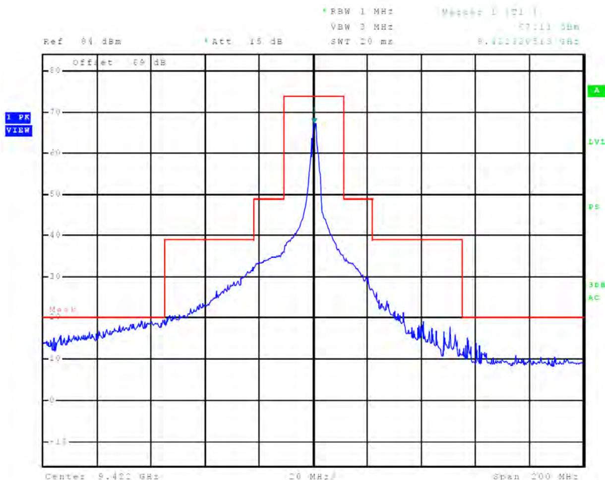
Figure 55 Emissions Mask, 18 nm
