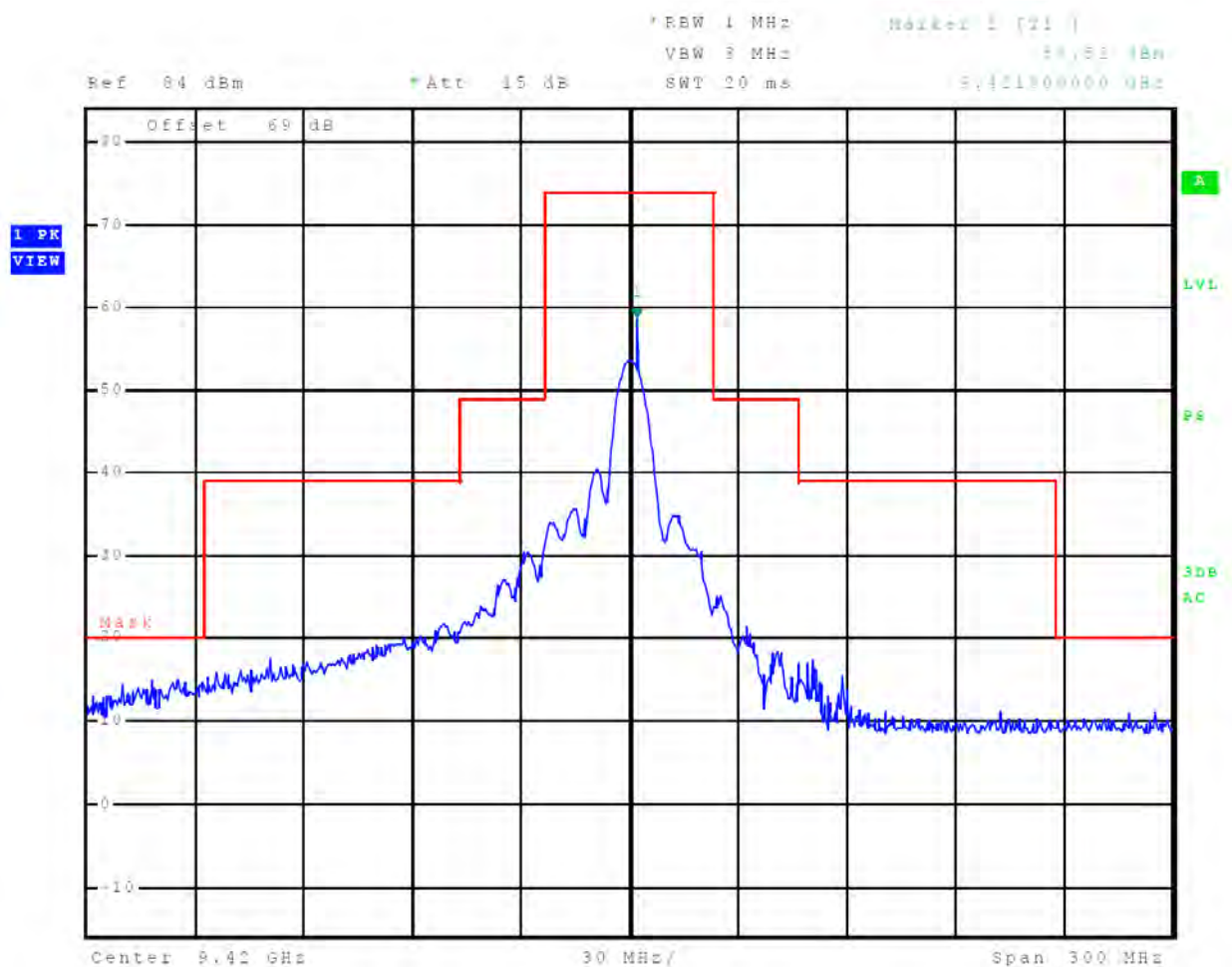
Figure 45 Emissions Mask, 1/2 nm
