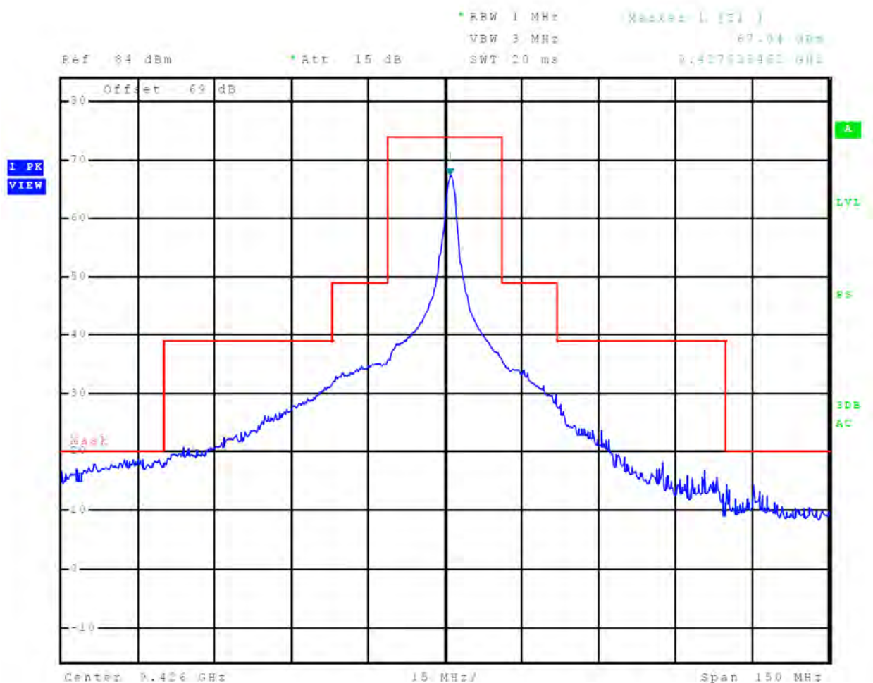
Figure 50 Emissions Mask, 3 nm
