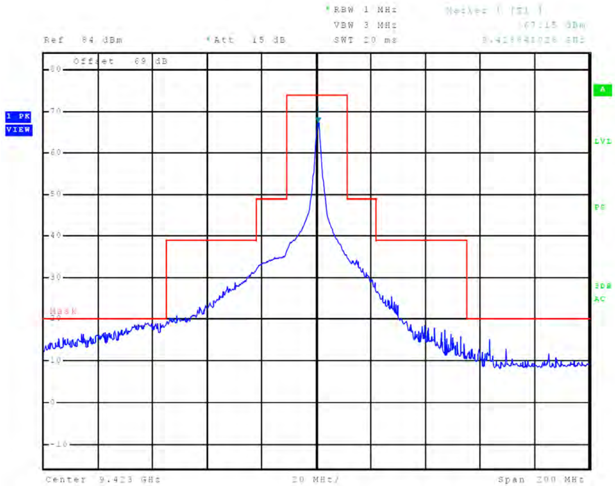
Figure 52 Emissions Mask, 6 nm
