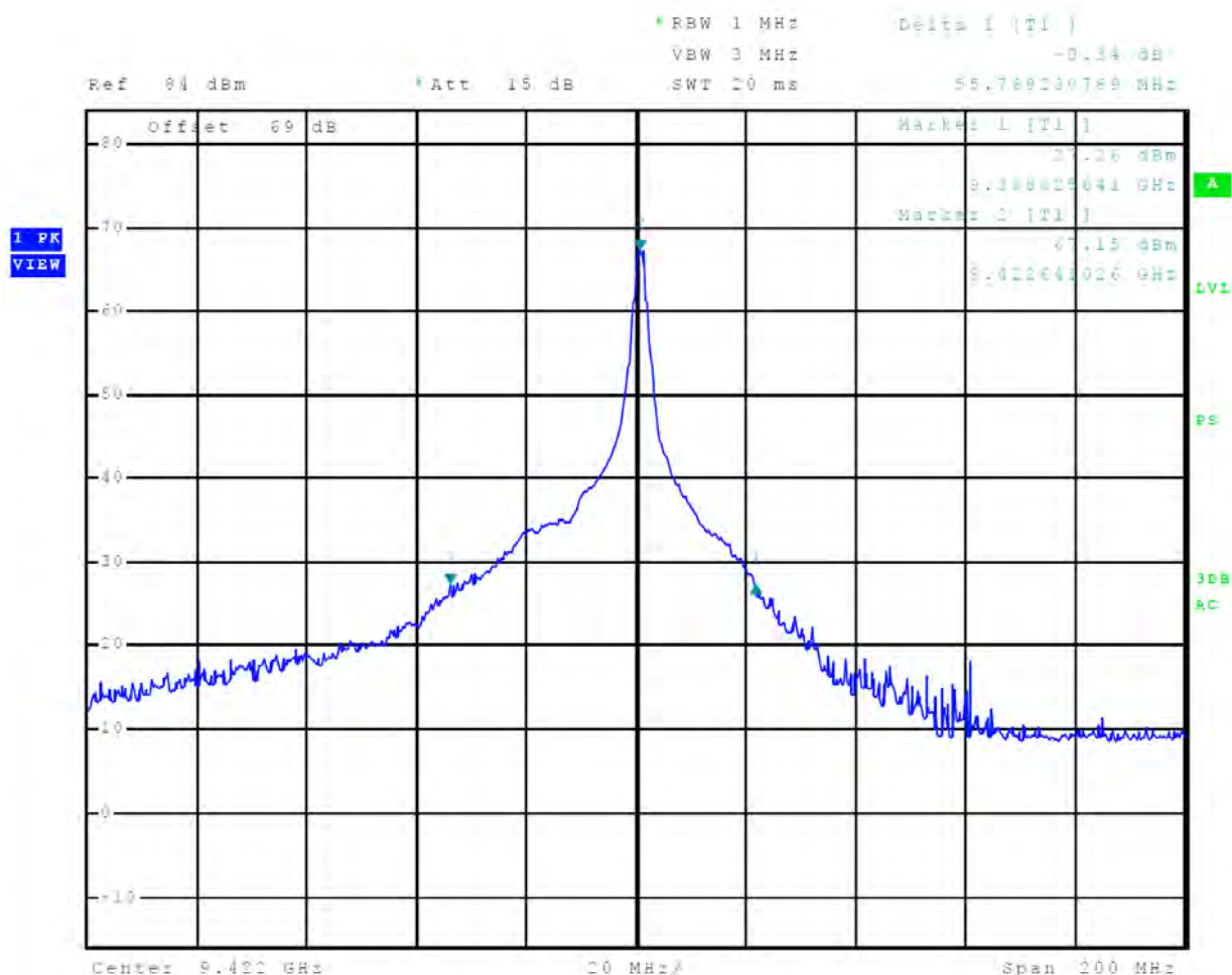
Figure 34 40-dB Occupied Bandwidth Plot, 12 nm
