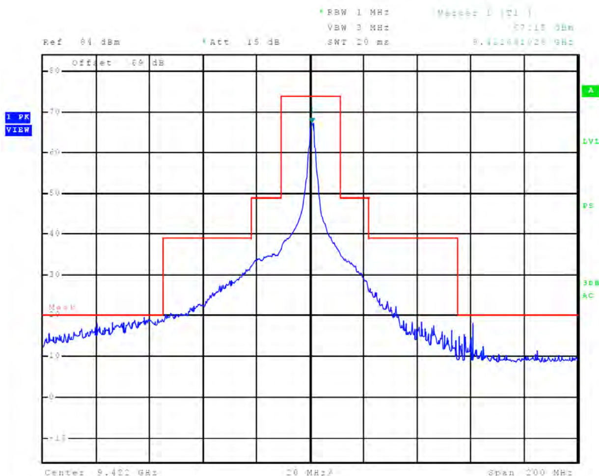
Figure 54 Emissions Mask, 12 nm
