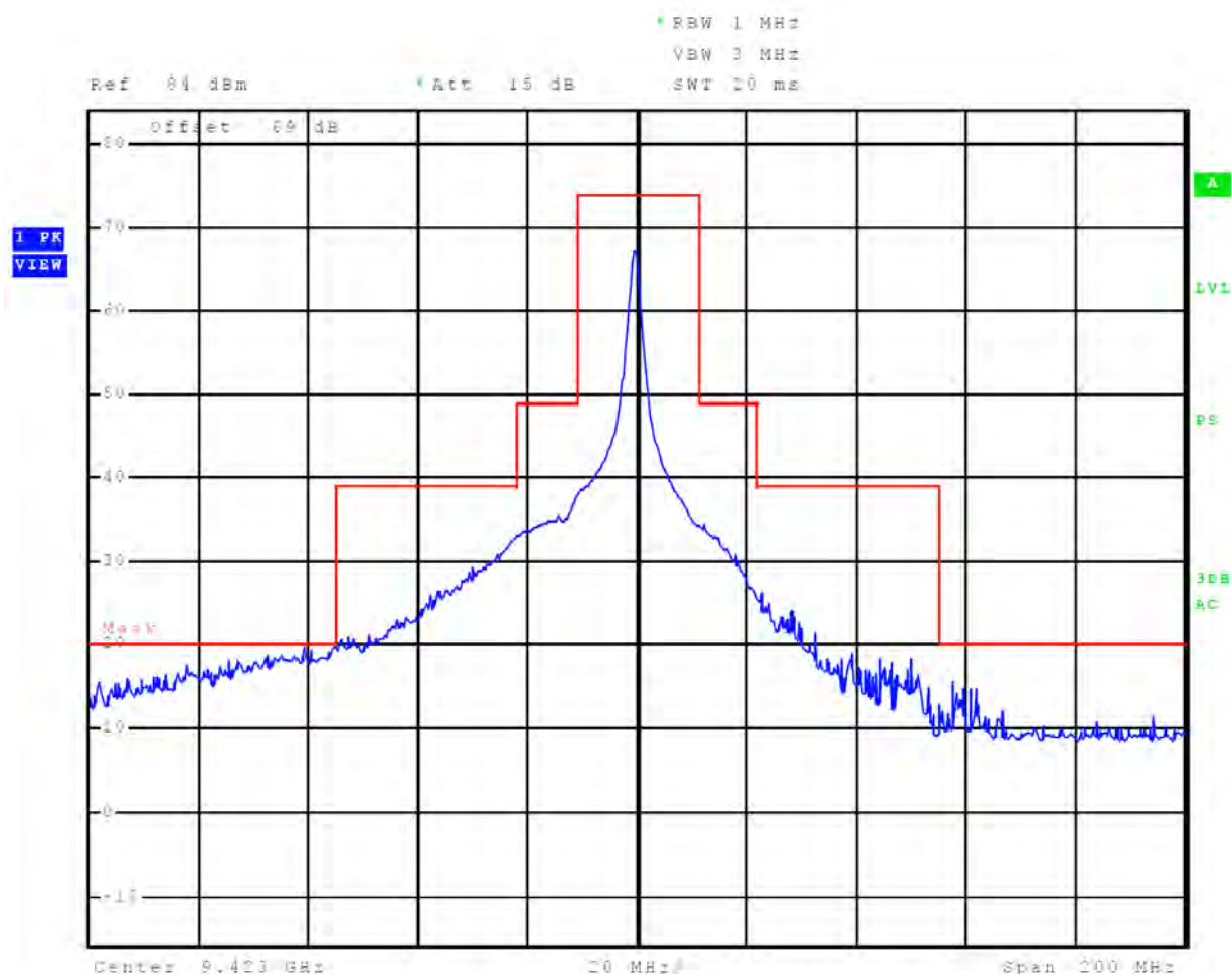
Figure 53 Emissions Mask, 8 nm
