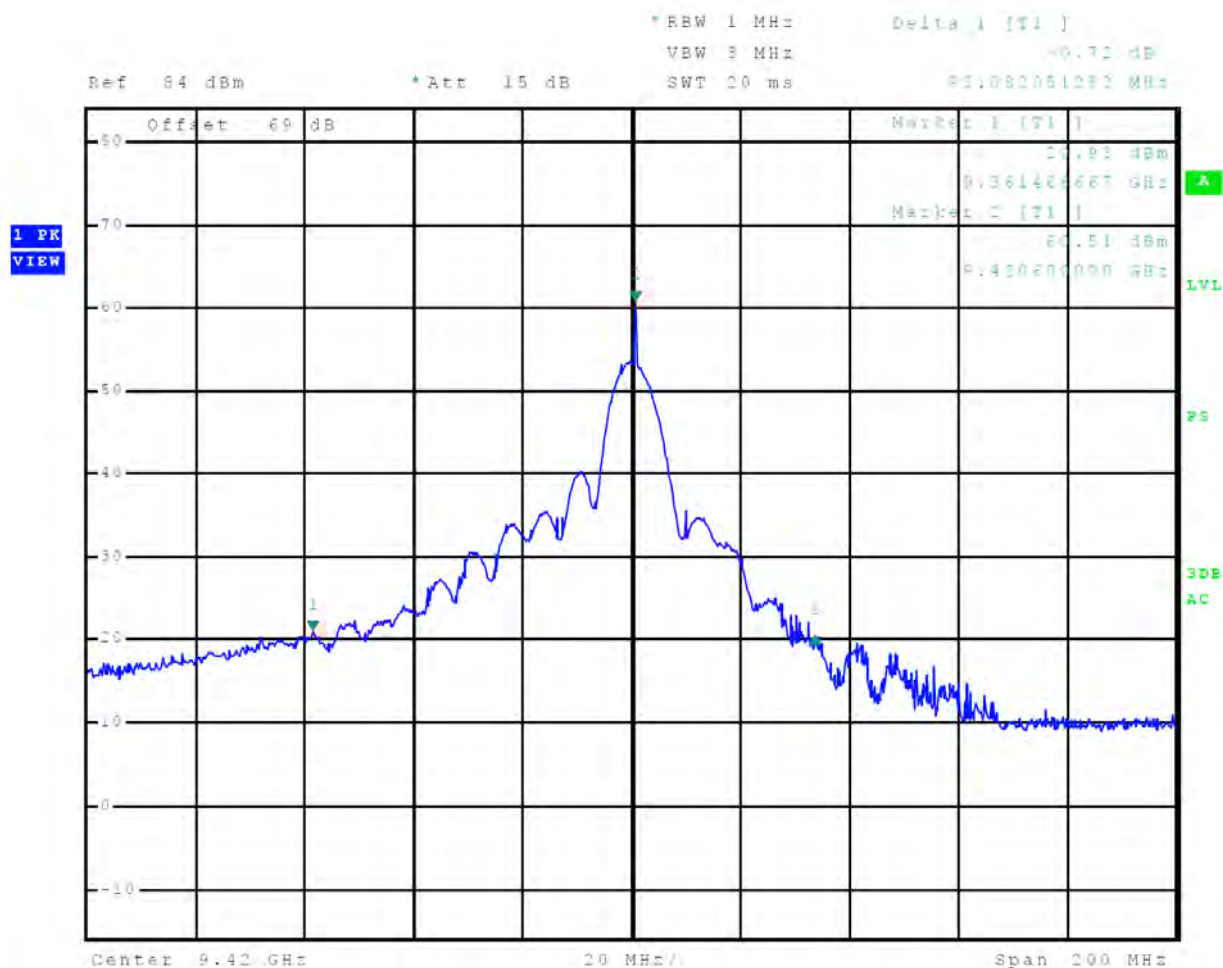
Figure 22 40-dB Occupied Bandwidth Plot, 1/16 nm
