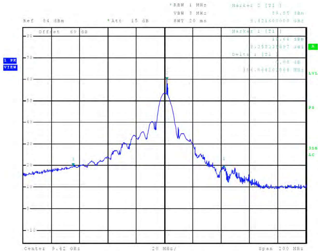
Figure 25 40-dB Occupied Bandwidth Plot, 1/2 nm
