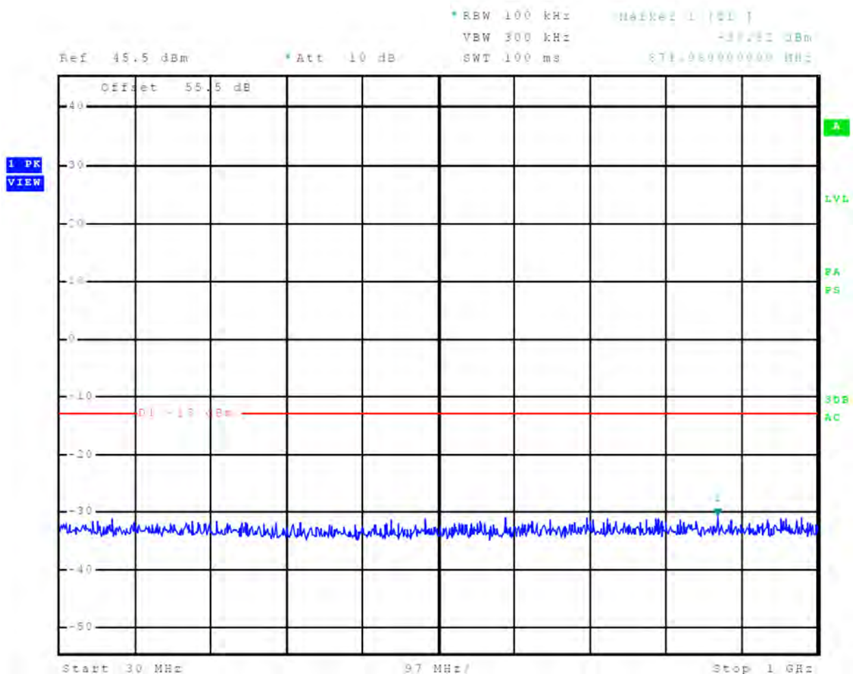
Figure 86 Out-of-Band Emissions 12 nm
