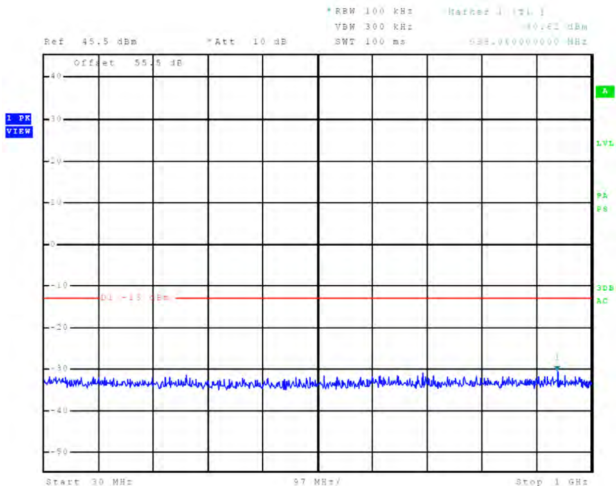
Figure 64 Out-of-Band Emissions 1/8 nm
