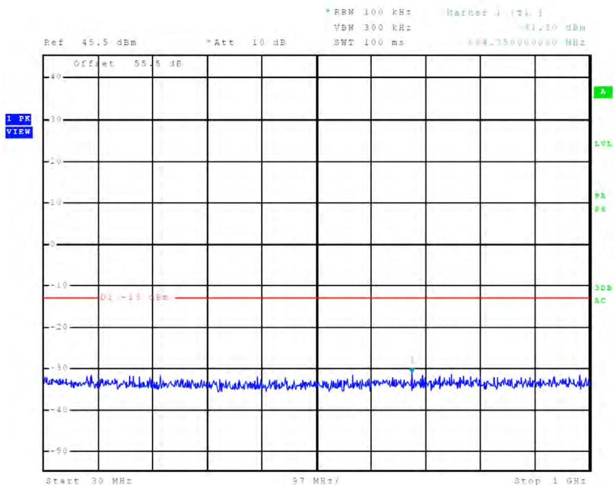
Figure 82 Out-of-Band Emissions 6 nm
