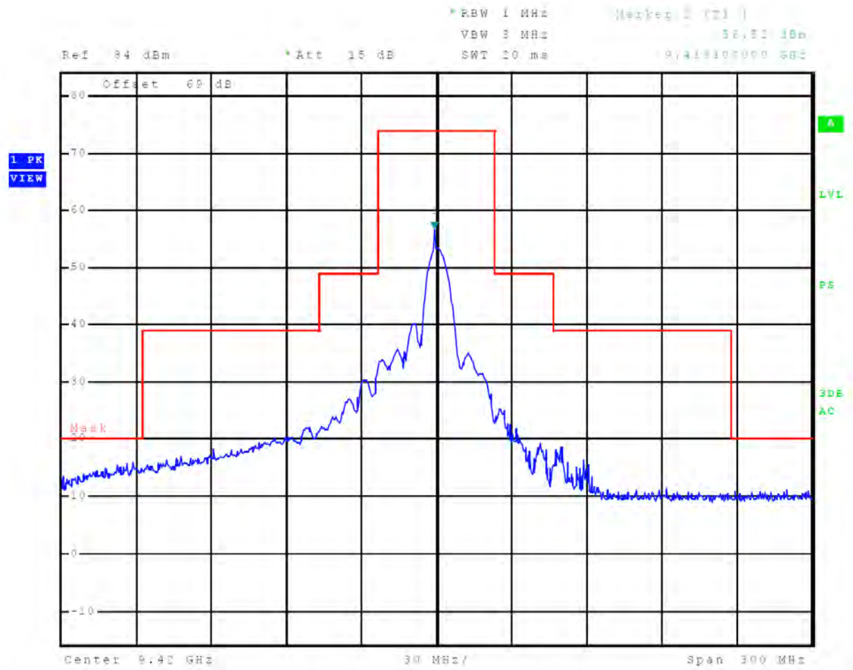
Figure 43 Emissions Mask, 1/8 nm
