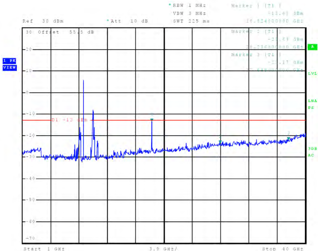
Figure 77 Out-of-Band Emissions 2 nm
