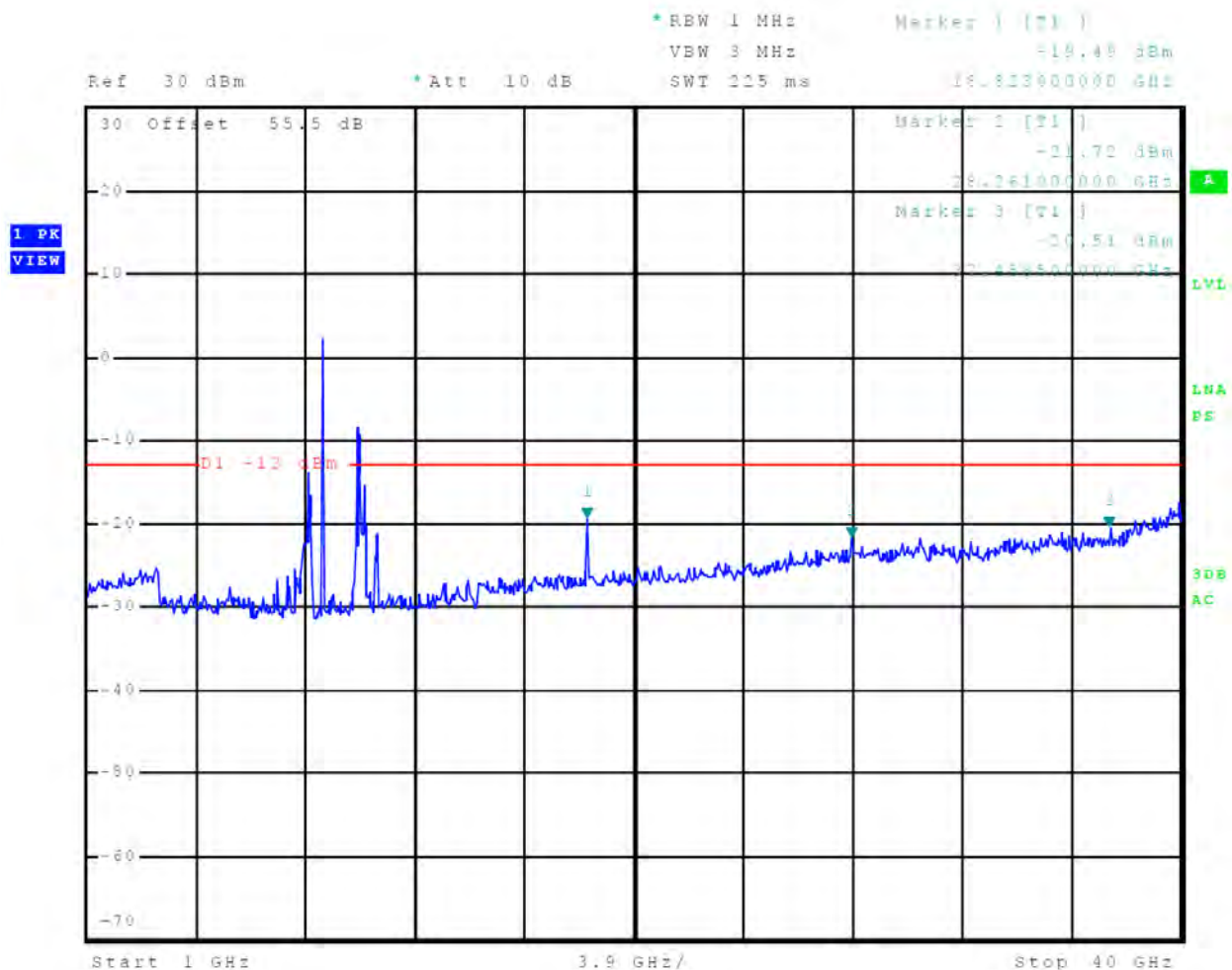
Figure 97 Out-of-Band Emissions 64 nm
