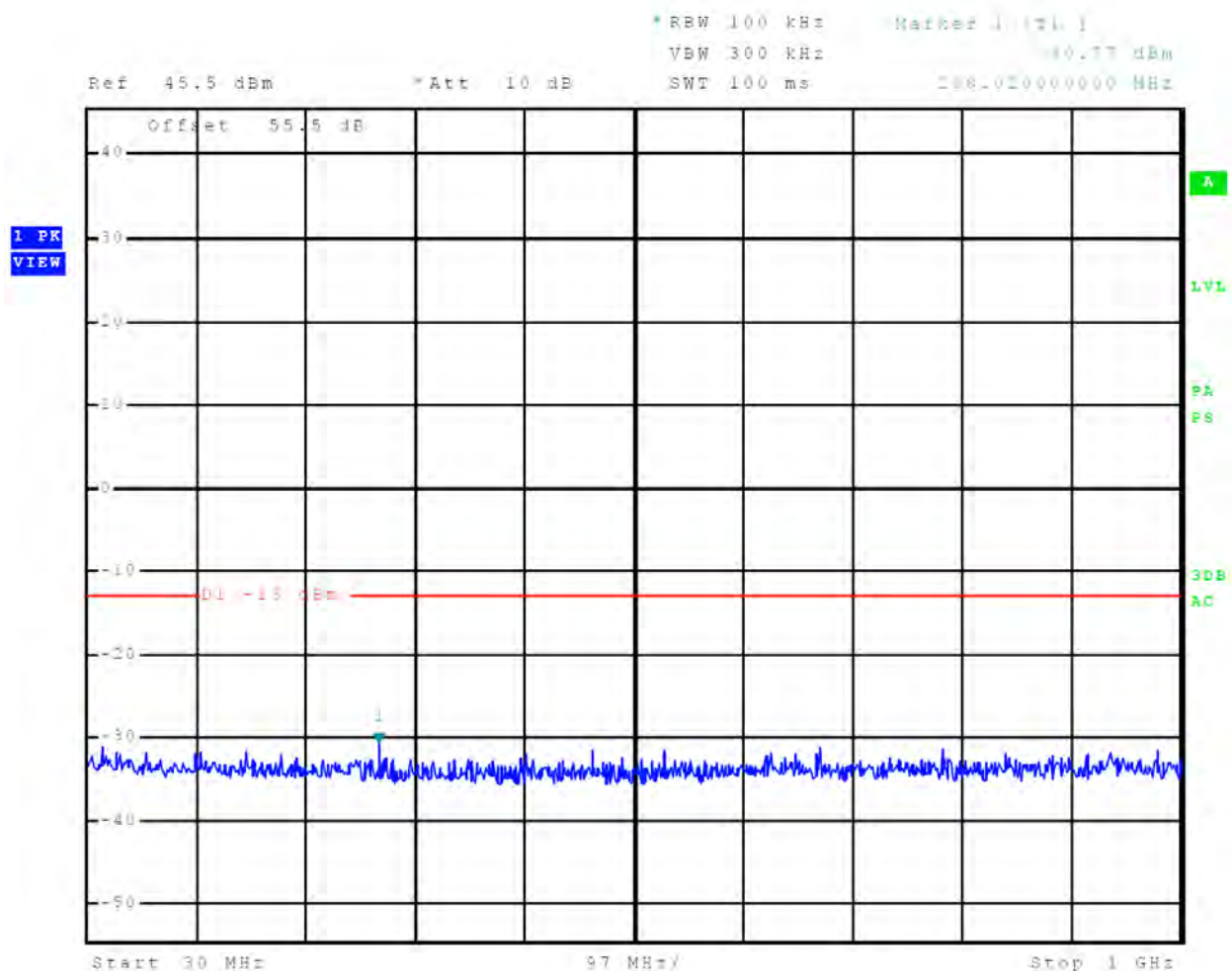
Figure 68 Out-of-Band Emissions 1/2 nm
