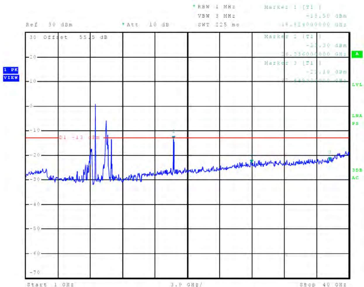
Figure 67 Out-of-Band Emissions 1/4 nm
