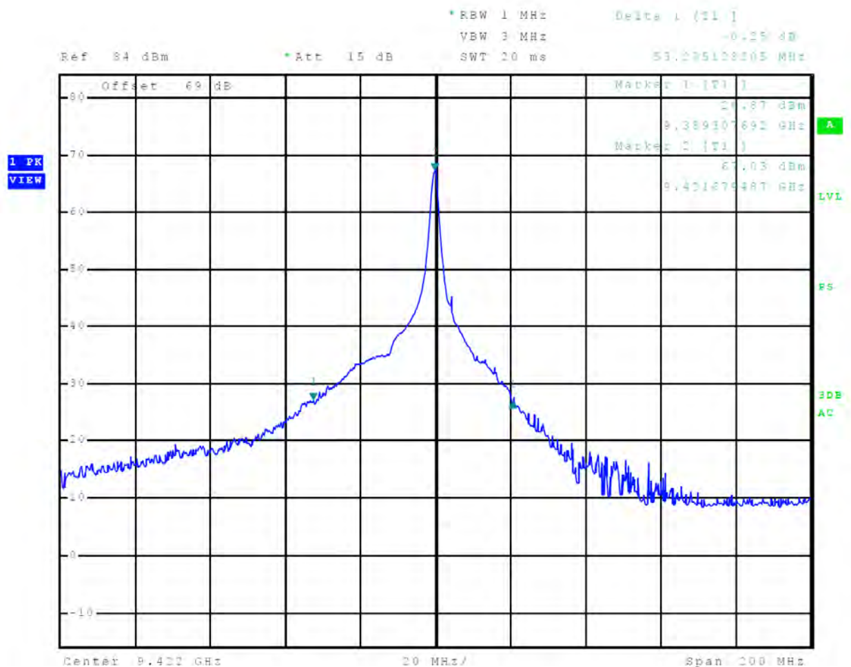
Figure 36 40-dB Occupied Bandwidth Plot, 24 nm
