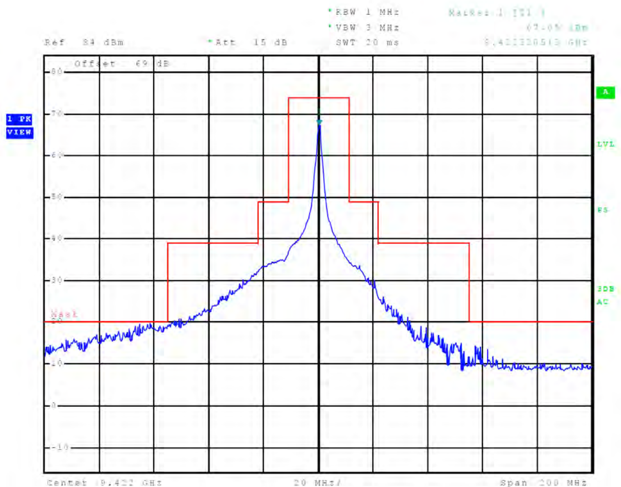
Figure 60 Emissions Mask, 72 nm
