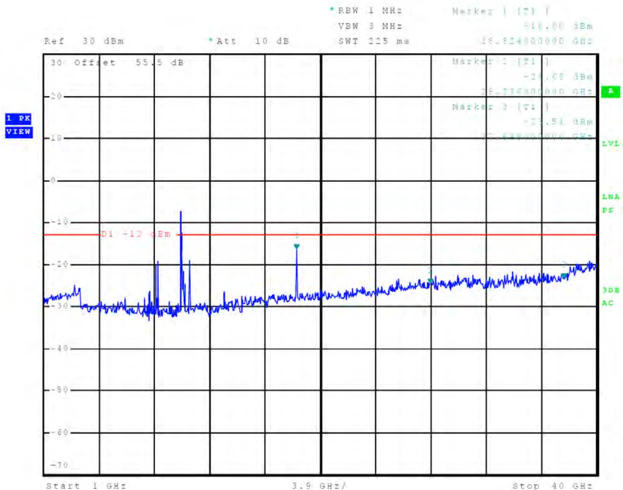
Figure 85 Out-of-Band Emissions 8 nm
