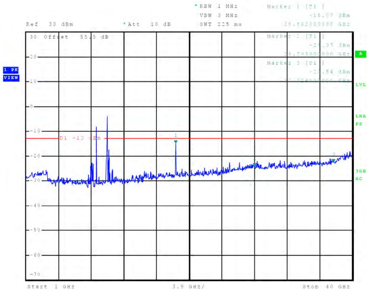
Figure 89 Out-of-Band Emissions 18 nm
