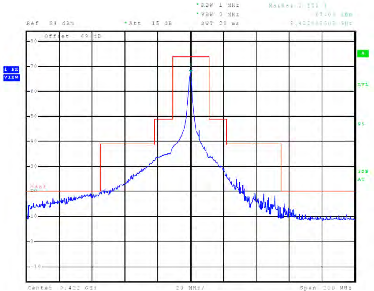
Figure 61 Emissions Mask, 96 nm
