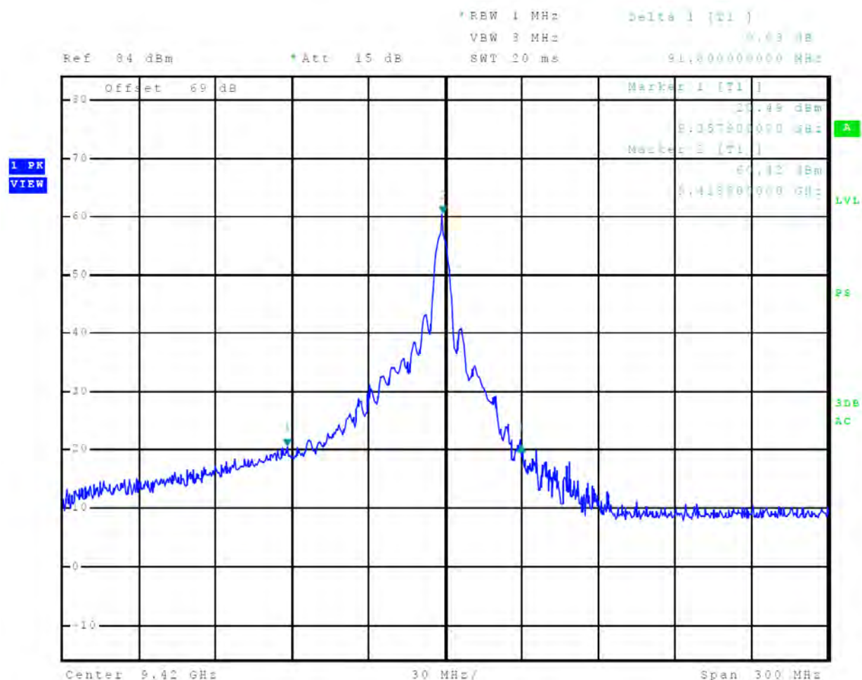
Figure 27 40-dB Occupied Bandwidth Plot, 1 nm
