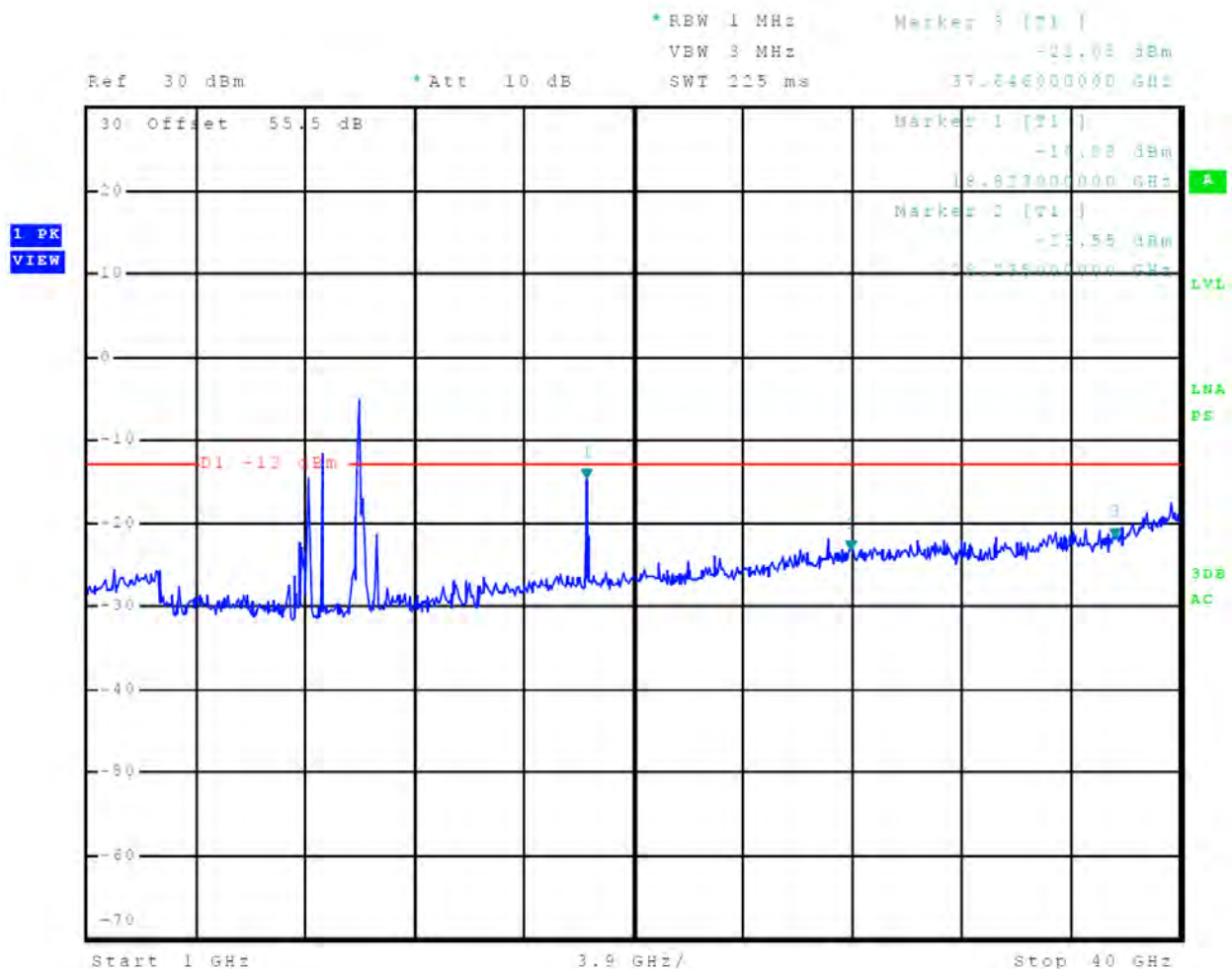
Figure 99 Out-of-Band Emissions 72 nm
