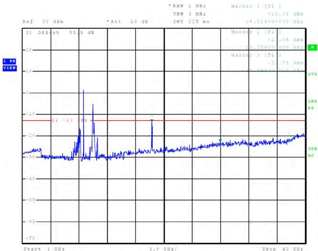
Figure 65 Out-of-Band Emissions 1/8 nm
