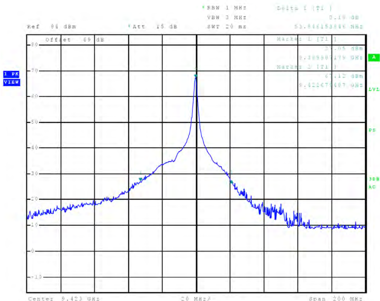
Figure 33 40-dB Occupied Bandwidth Plot, 8 nm
