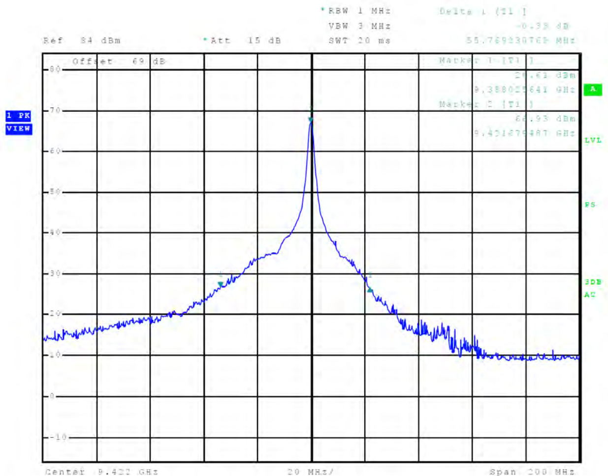
Figure 37 40-dB Occupied Bandwidth Plot, 36 nm
