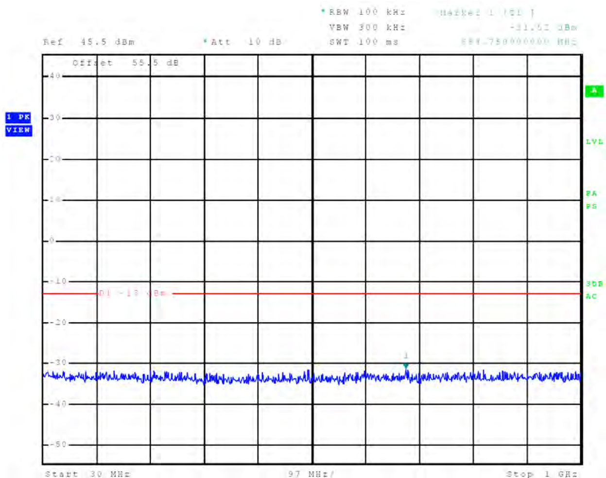
Figure 88 Out-of-Band Emissions 18 nm
