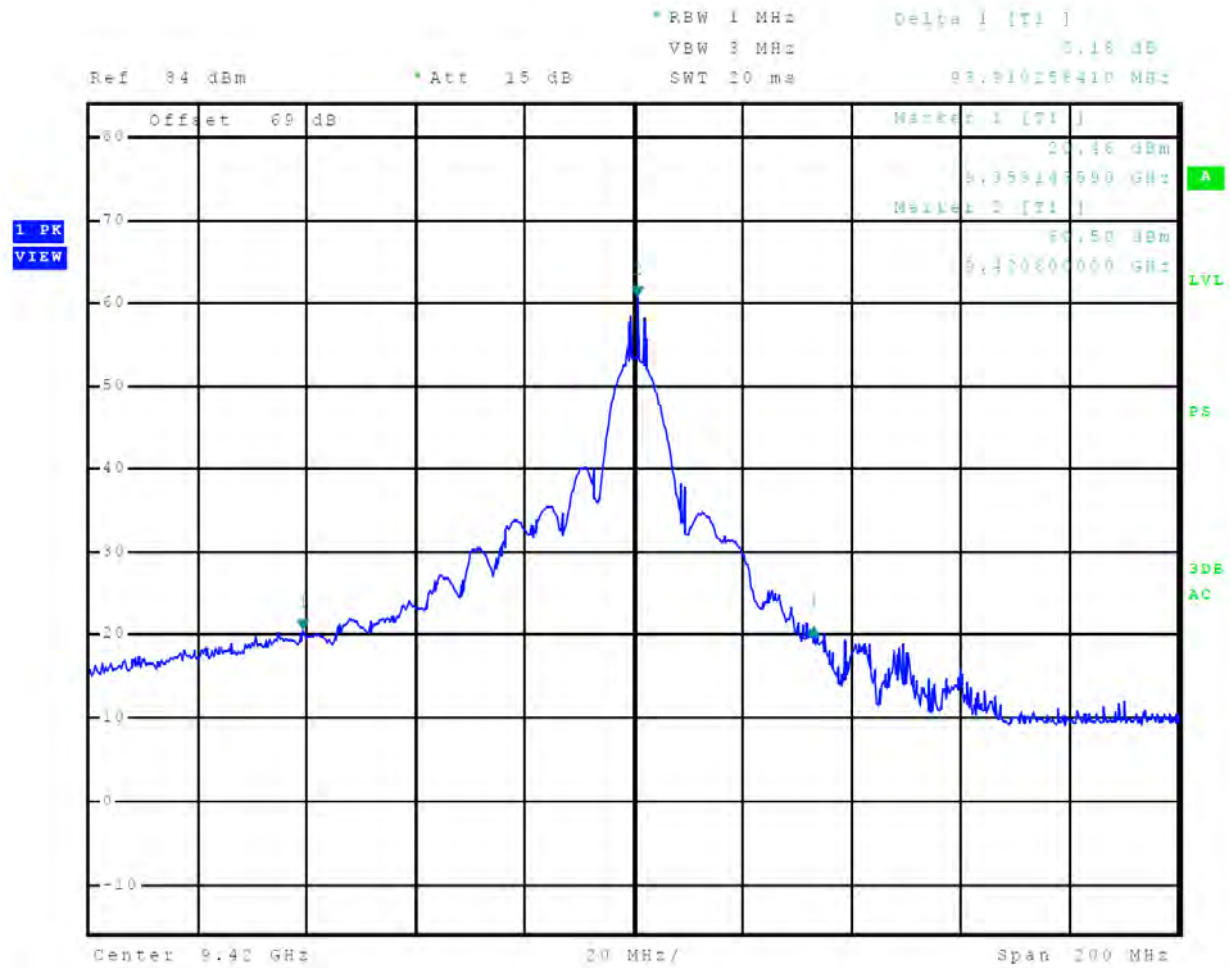
Figure 23 40-dB Occupied Bandwidth Plot, 1/8 nm
