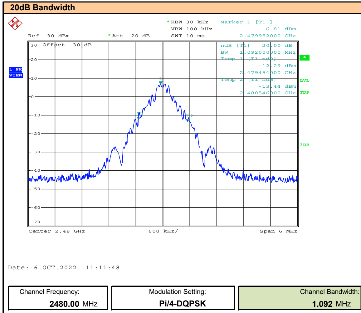
Plot 14.2 – BT EDR 2MB 20dB BW
