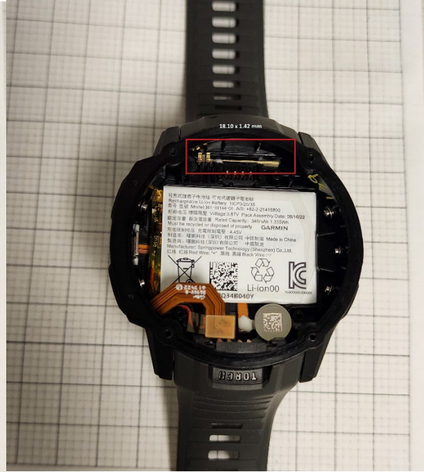
BLE Antenna Markings on the Right Picture: 18.10 x 1.42 mm
