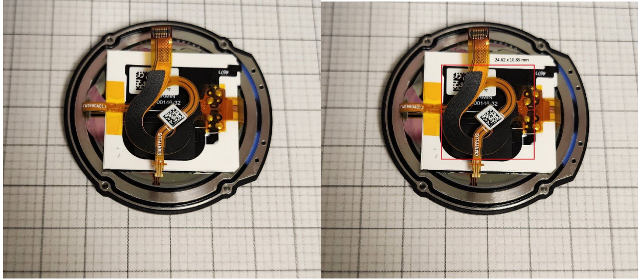
NFC Antenna Markings on the Right Picture: 24.62 x 10.85 mm
