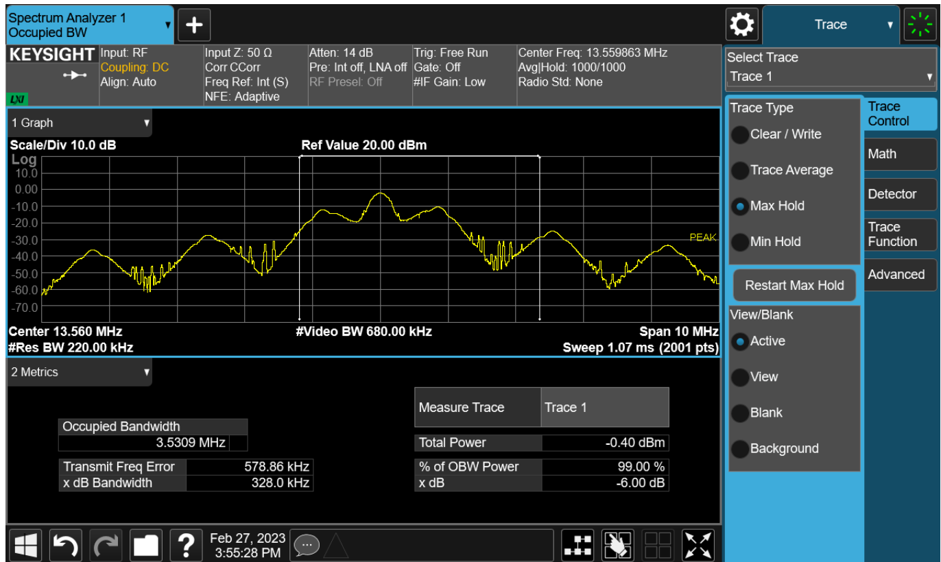
Figure TR22.2: Occupied bandwidth data for Type B NFC
