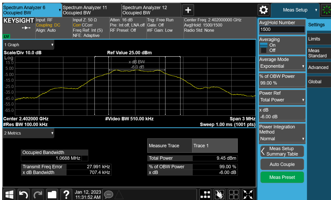
Figure TR8.2: Spectral data for BLE 1 Mbps on the Low frequency.
