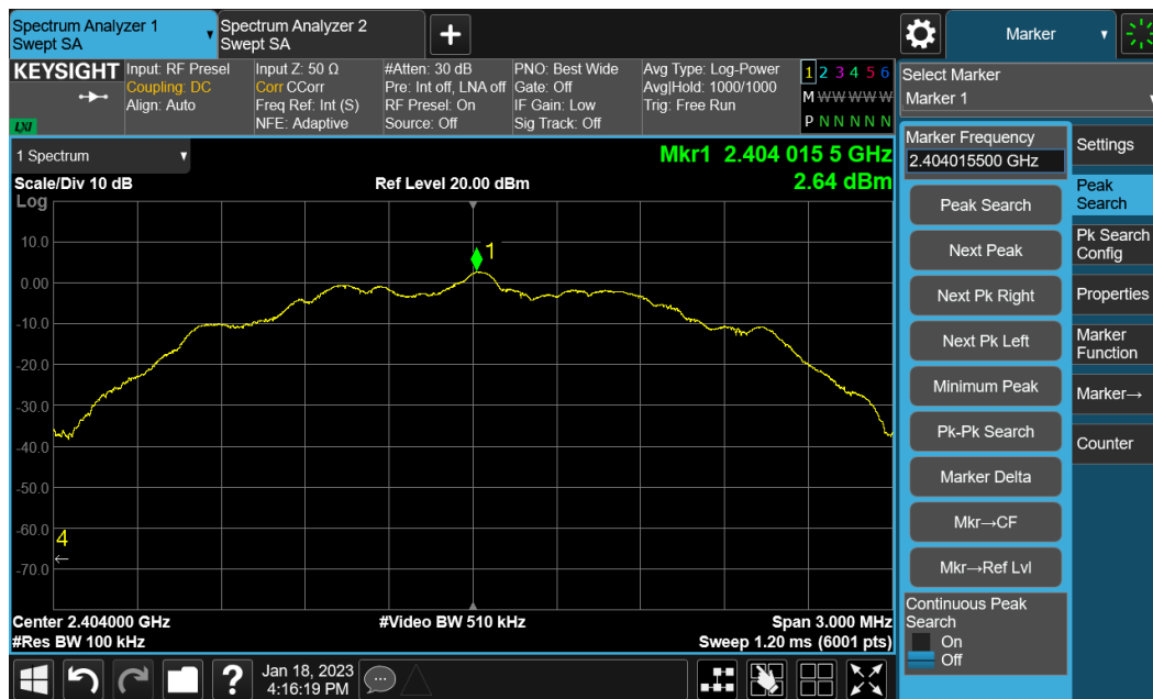
Figure TR12.3: BLE carrier at 2 Mbps data rate, 2404 MHz channel
