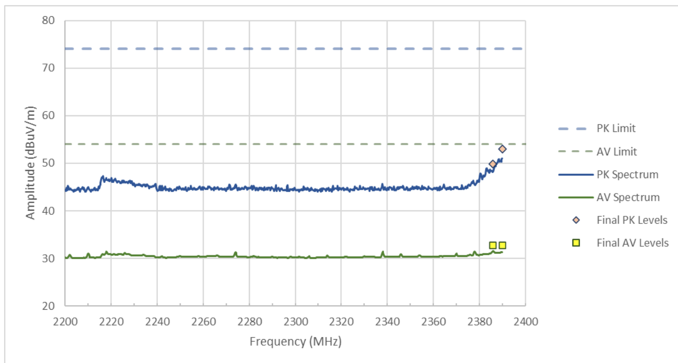
Figure RE07.1: FCC restricted band spectral data from 2200 to 2390 MHz
