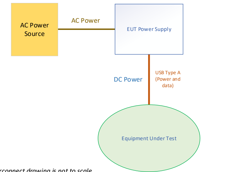
This interconnect drawing is not to scale. It does not indicate the placement of devices. Figure 1: Block diagram of equipment arrangement A1
