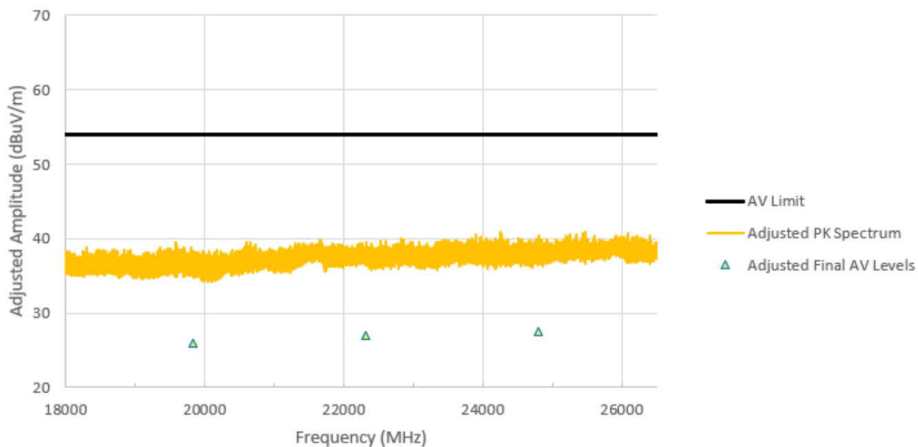
Figure RE15.6: High Channel Final Adjusted Average Level Data
