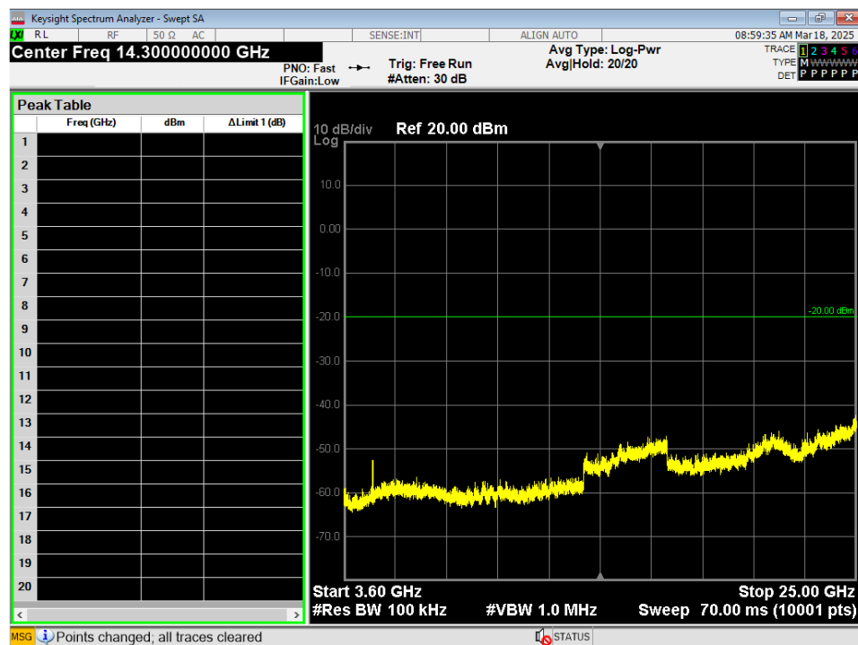
Figure 9 - Conducted Emissions Plot, GMSK, 3.6GHz – 25GHz
