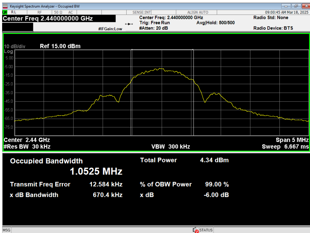
02 Occupied BW, BLE 1MB, 2440MHz
