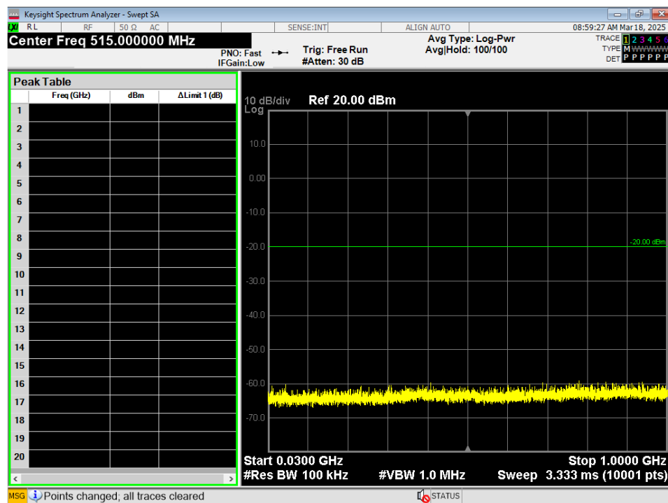
Figure 7 - Conducted Emissions Plot, GMSK, 30MHz – 1GHz
