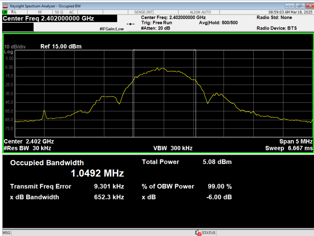
01 Occupied BW, BLE 1MB, 2402MHz
