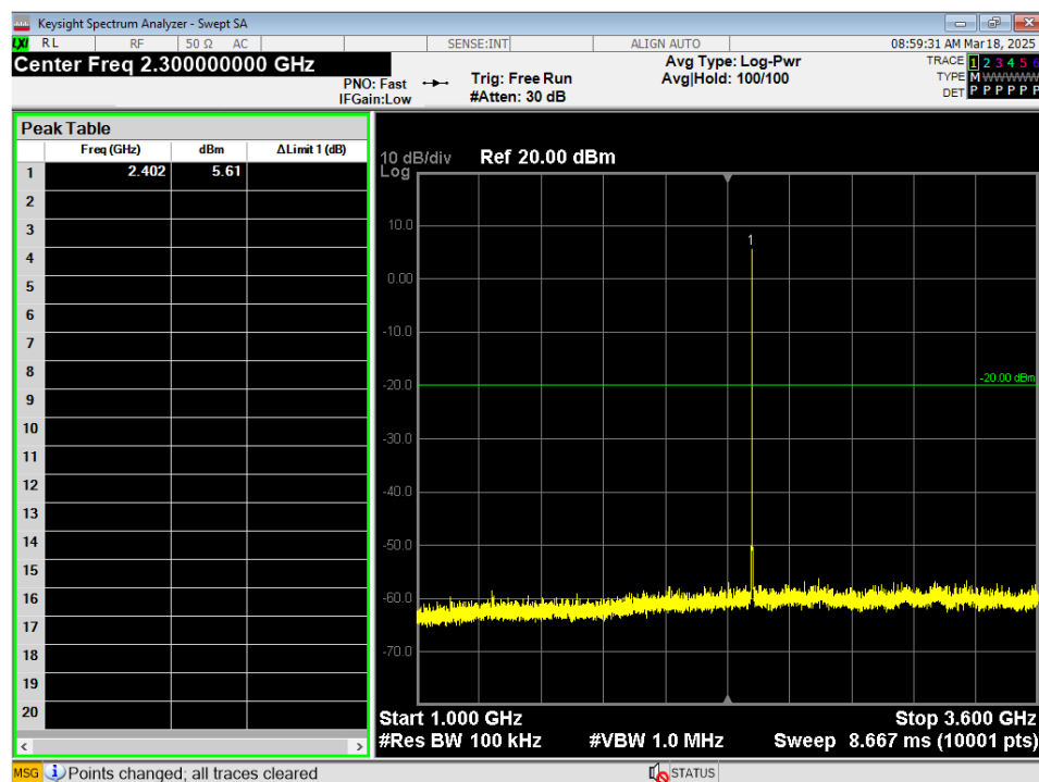
Figure 8 - Conducted Emissions Plot, GMSK, 1GHz – 3.6GHz
