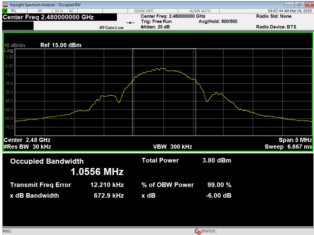
03 Occupied BW, BLE 1MB, 2480MHz
