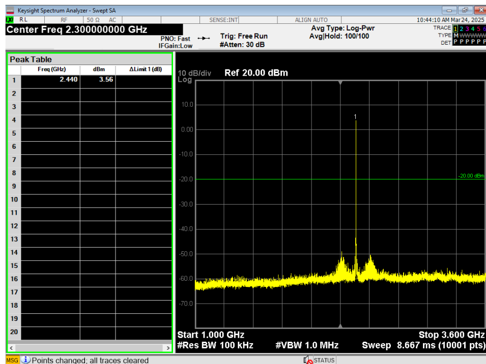
Figure 8 - Conducted Emissions Plot, GMSK, 1GHz – 3.6GHz, Mid
