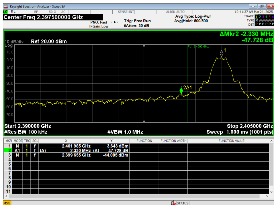
10 Lower Bandedge, Unrestricted, GMSK
