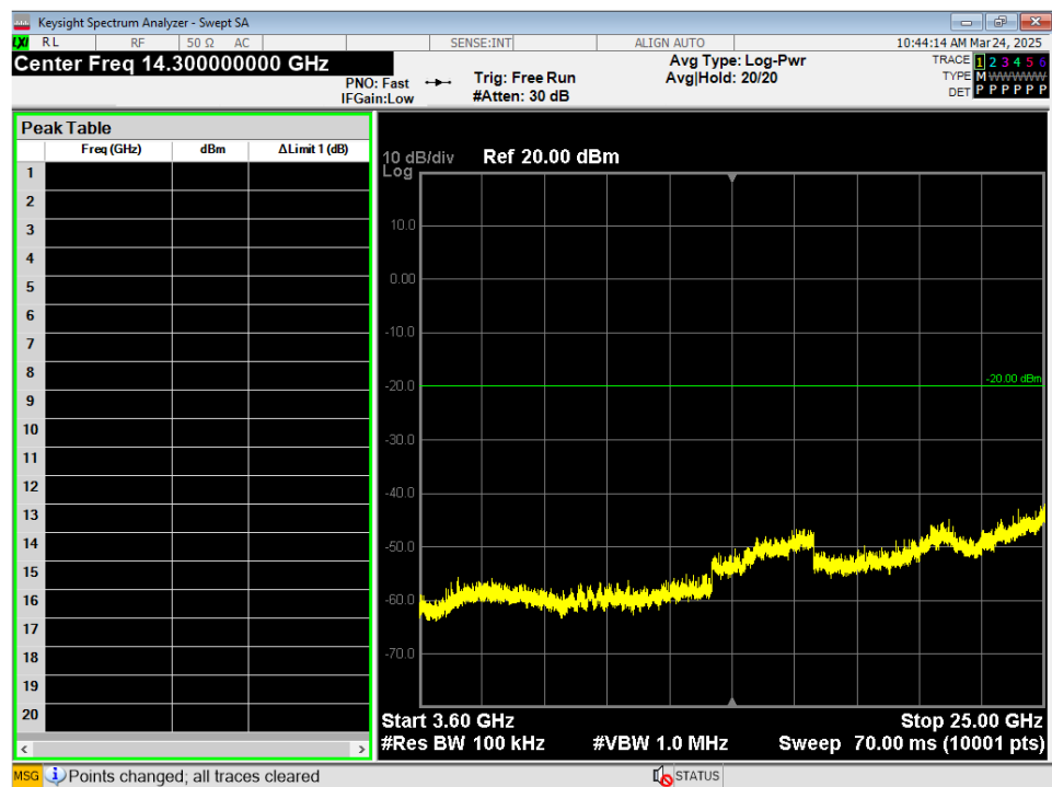
Figure 9 - Conducted Emissions Plot, GMSK, 3.6GHz – 25GHz, Mid
