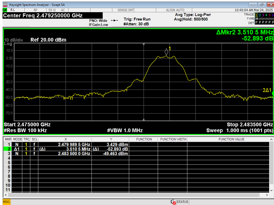
11 Higher Bandedge, Unrestricted, GMSK
