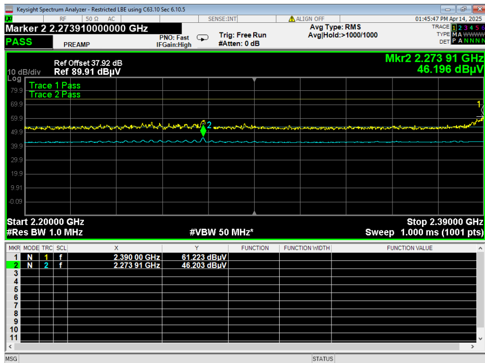
12 Lower Bandedge, Restricted, GMSK
