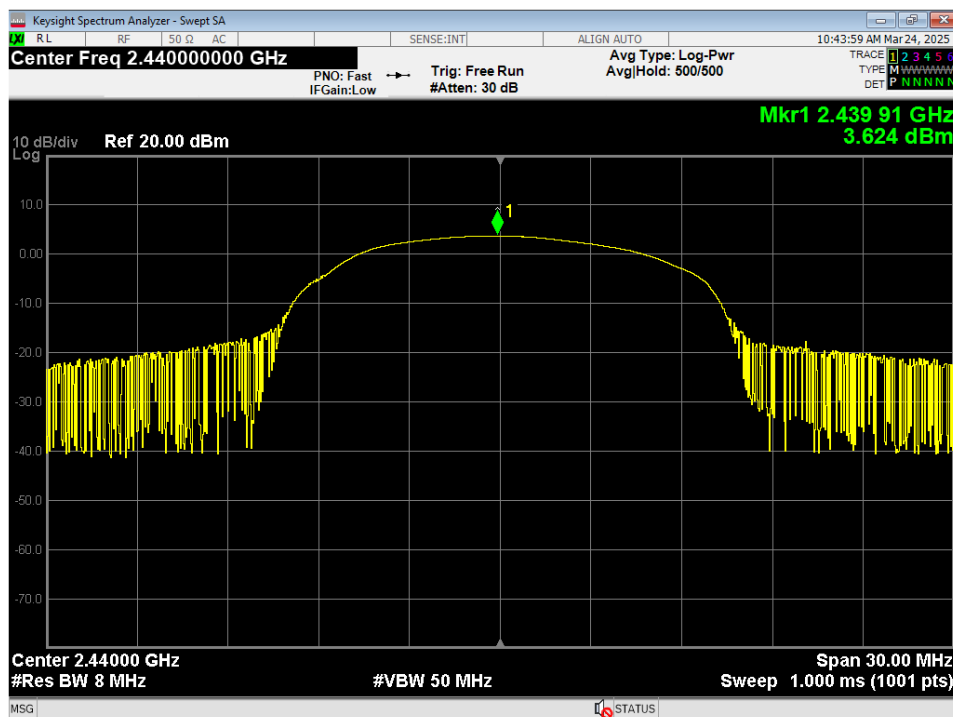
02 Peak Power, Mid Channel, GMSK
