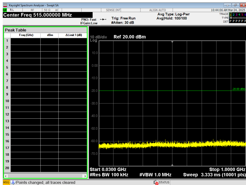
Figure 7 - Conducted Emissions Plot, GMSK, 30MHz – 1GHz, Mid
