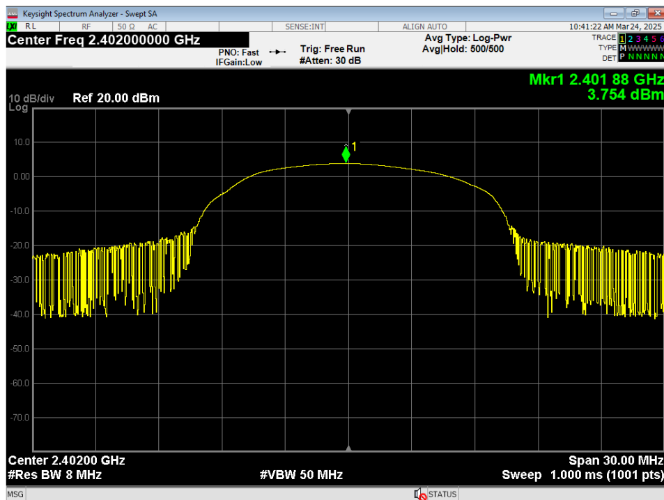
01 Peak Power, Low Channel, GMSK
