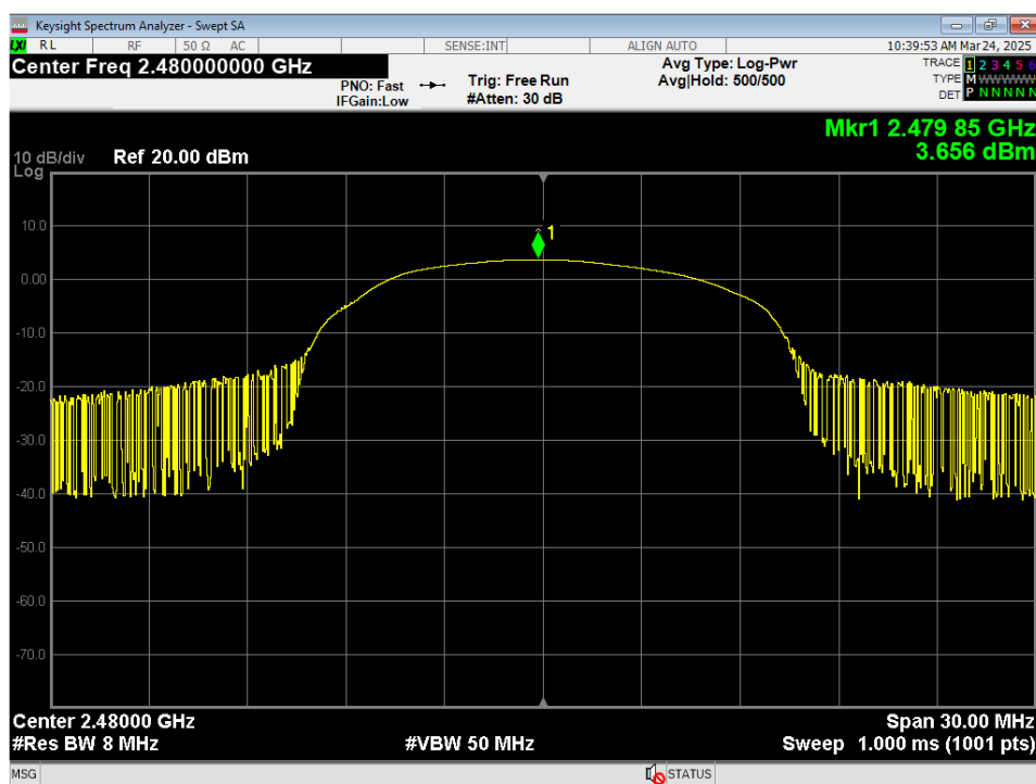
03 Peak Power, High Channel, GMSK
