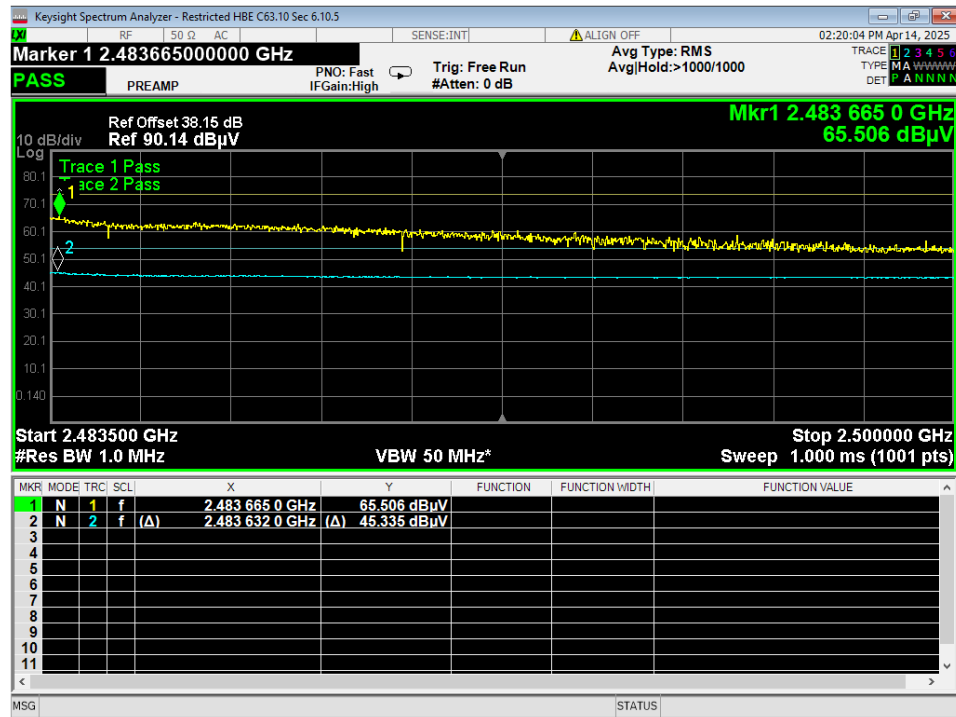
13 Higher Bandedge, Restricted, GMSK
