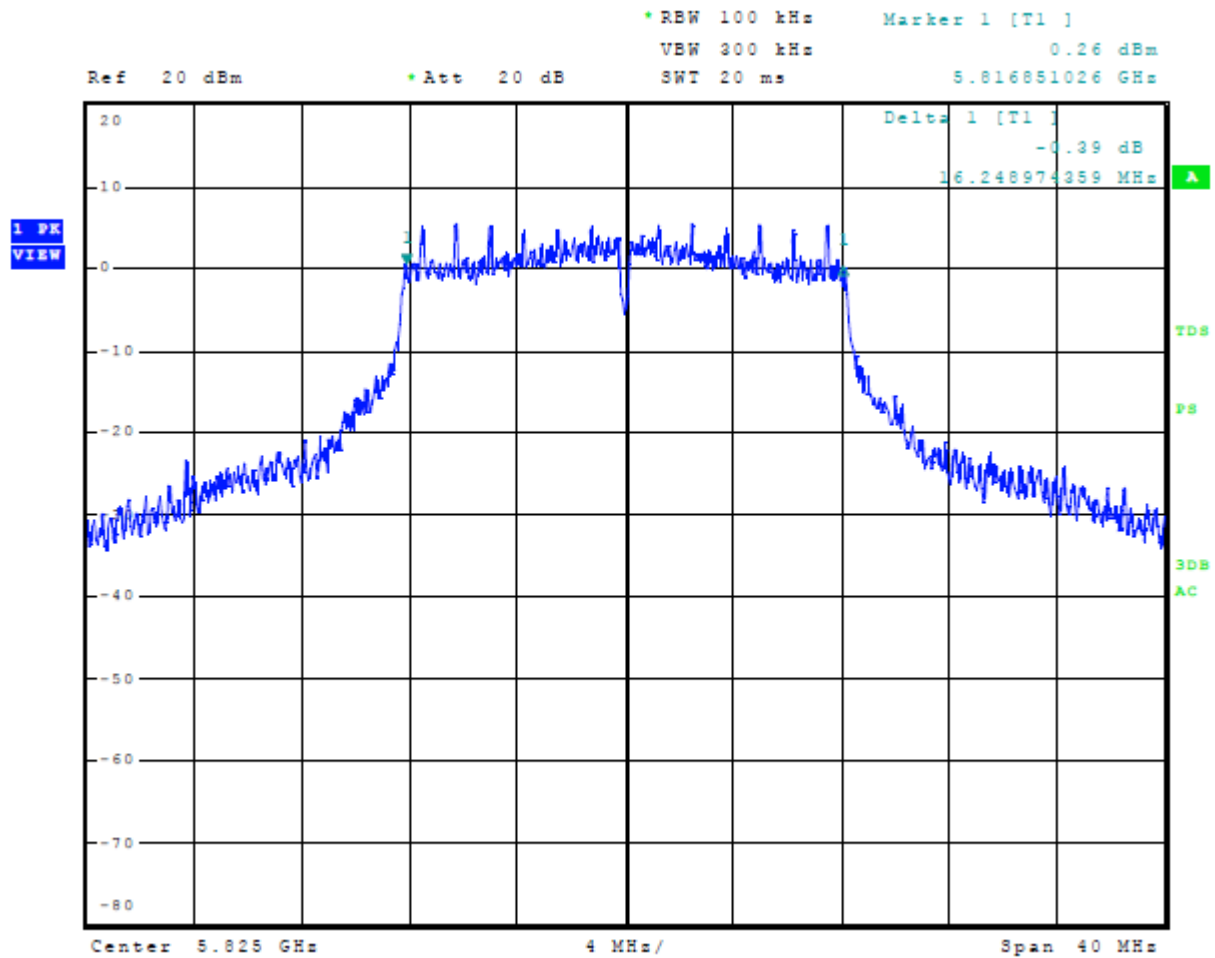
Figure 43 Plot of 6-dB Occupied Bandwidth 5725-5850 MHz Mode 9 U-NII-3 (802.11a)
