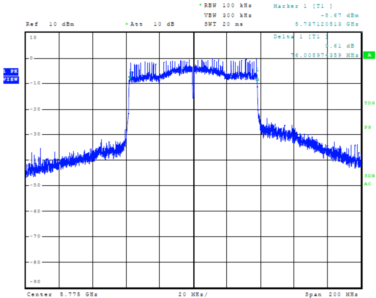
Figure 46 Plot of 6-dB Occupied Bandwidth 5725-5850 MHz Mode 12 U-NII-3 (802.11ac80)
