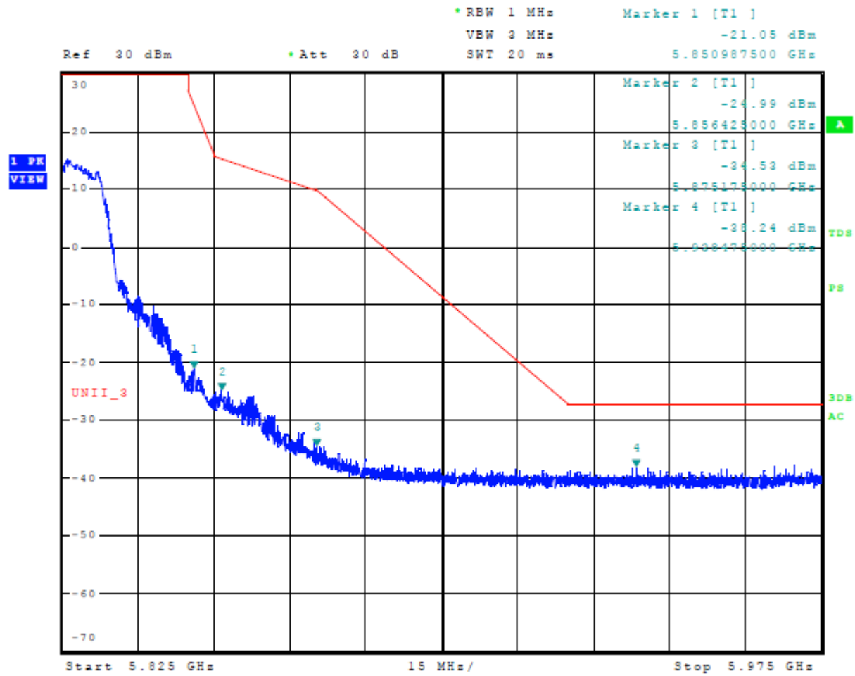
Figure 23 Plot of Upper Band Edge Across 5725-5850 MHz Mode 9 U-NII-3 (802.11a)
