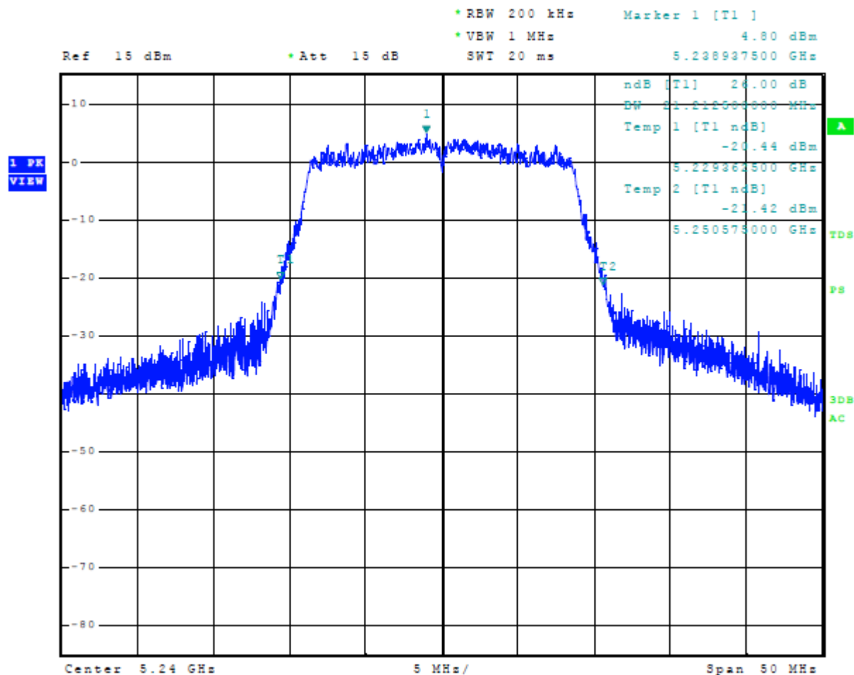
Figure 28 Plot of 26-dB Occupied Bandwidth 5150-5250 MHz Mode 6 U-NII-1 (802.11n)
