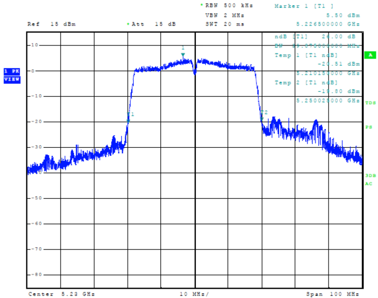
Figure 29 Plot of 26-dB Occupied Bandwidth 5150-5250 MHz Mode 7 U-NII-1 (802.11n40)
