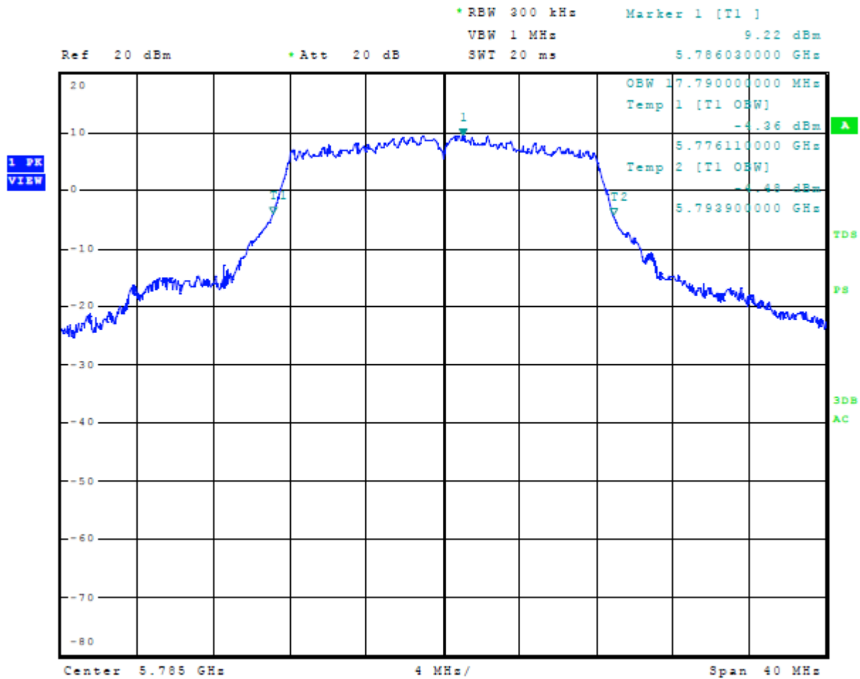
Figure 39 Plot of 99% Occupied Bandwidth 5725-5850 MHz Mode 9 U-NII-3 (802.11a)
