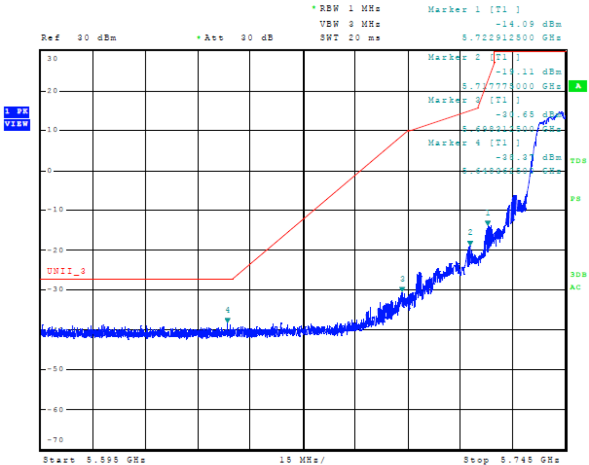
Figure 15 Plot of Lower Band Edge Across 5725-5850 MHz Mode 9 U-NII-3 (802.11a)
