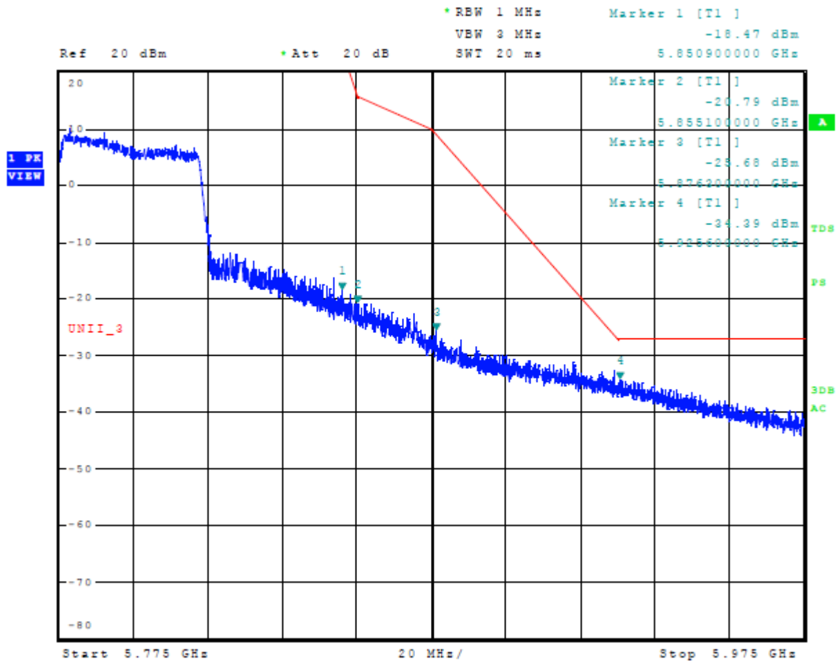
Figure 26 Plot of Upper Band Edge Across 5725-5850 MHz Mode 12 U-NII-3 (802.11ac80)
