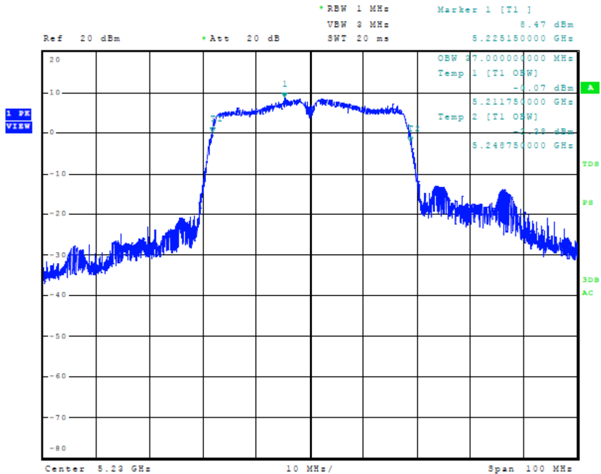
Figure 37 Plot of 99% Occupied Bandwidth 5150-5250 MHz Mode 7 U-NII-1 (802.11n40)
