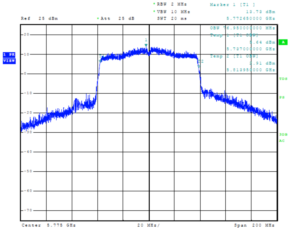
Figure 42 Plot of 99% Occupied Bandwidth 5725-5850 MHz Mode 12 U-NII-3 (802.11ac80)
