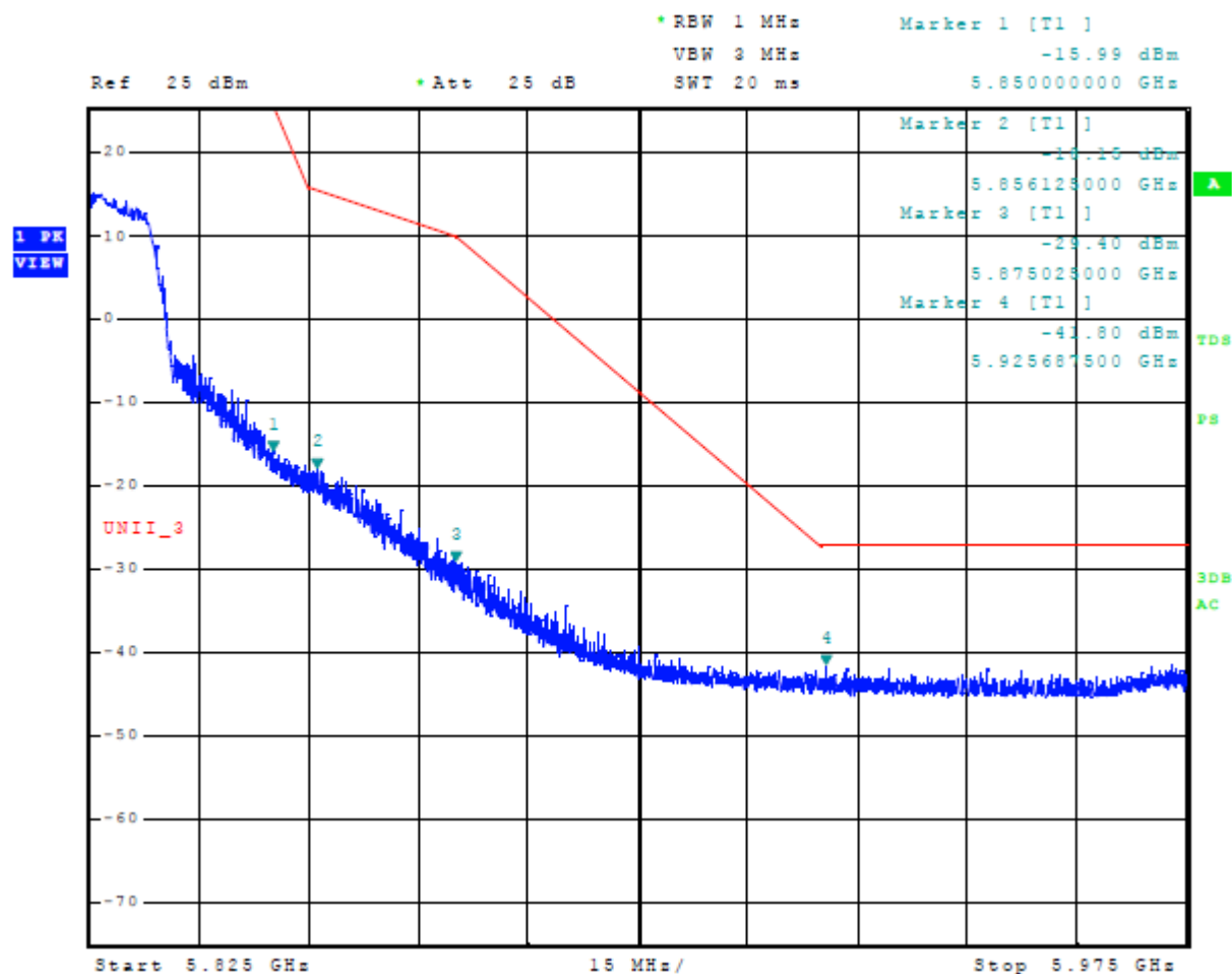
Figure 24 Plot of Upper Band Edge Across 5725-5850 MHz Mode 10 U-NII-3 (802.11n)
