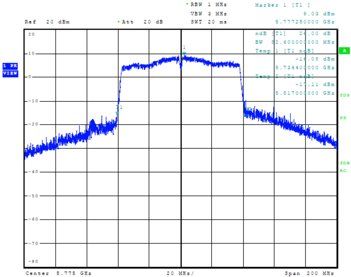
Figure 34 Plot of 26-dB Occupied Bandwidth 5725-5850 MHz Mode 12 U-NII-3 (802.11ac80)
