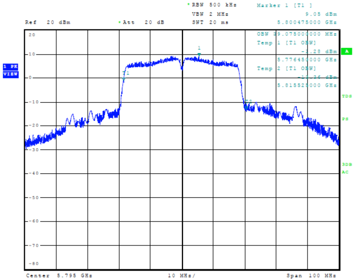
Figure 41 Plot of 99% Occupied Bandwidth 5725-5850 MHz Mode 11 U-NII-3 (802.11n40)
