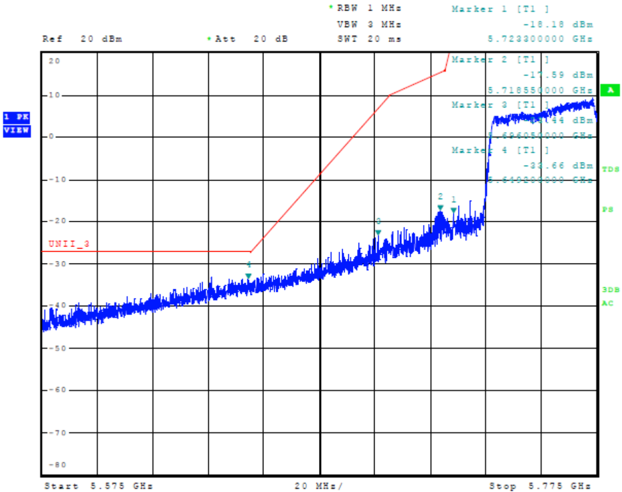
Figure 18 Plot of Lower Band Edge Across 5725-5850 MHz Mode 12 U-NII-3 (802.11ac80)
