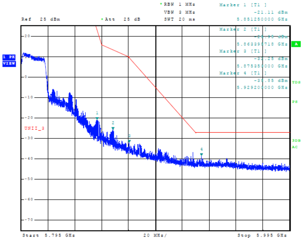
Figure 25 Plot of Upper Band Edge Across 5725-5850 MHz Mode 11 U-NII-3 (802.11n40)
