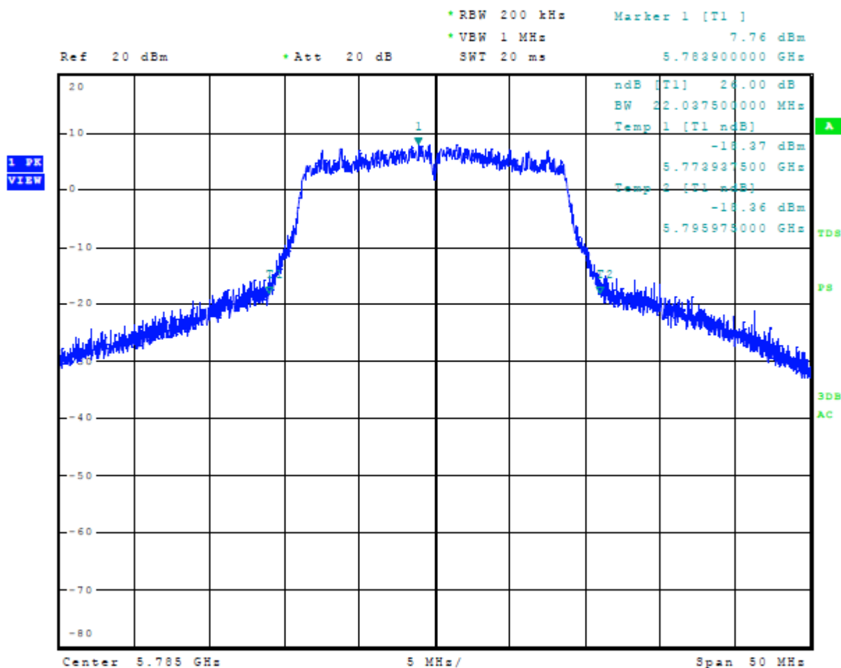
Figure 32 Plot of 26-dB Occupied Bandwidth 5725-5850 MHz Mode 10 U-NII-3 (802.11n)
