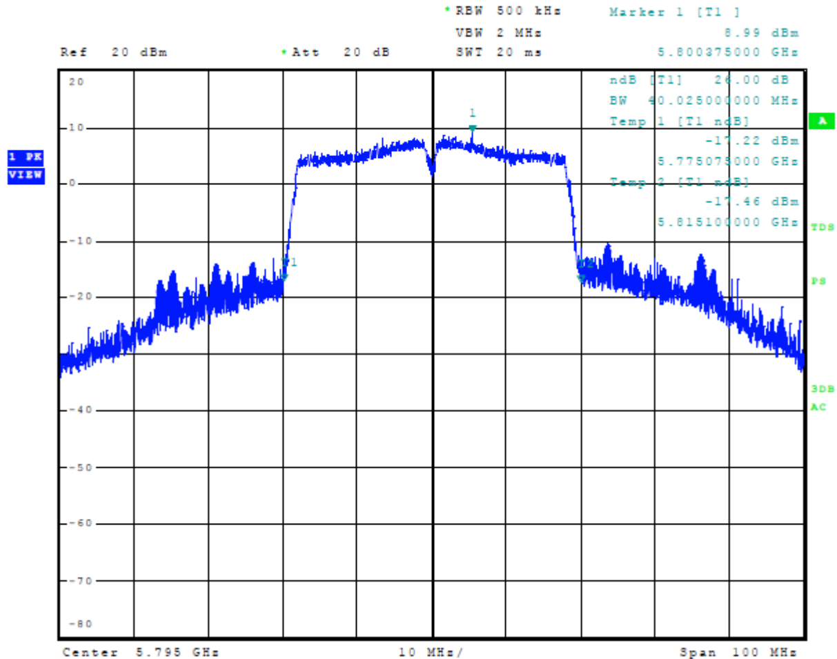
Figure 33 Plot of 26-dB Occupied Bandwidth 5725-5850 MHz Mode 11 U-NII-3 (802.11n40)
