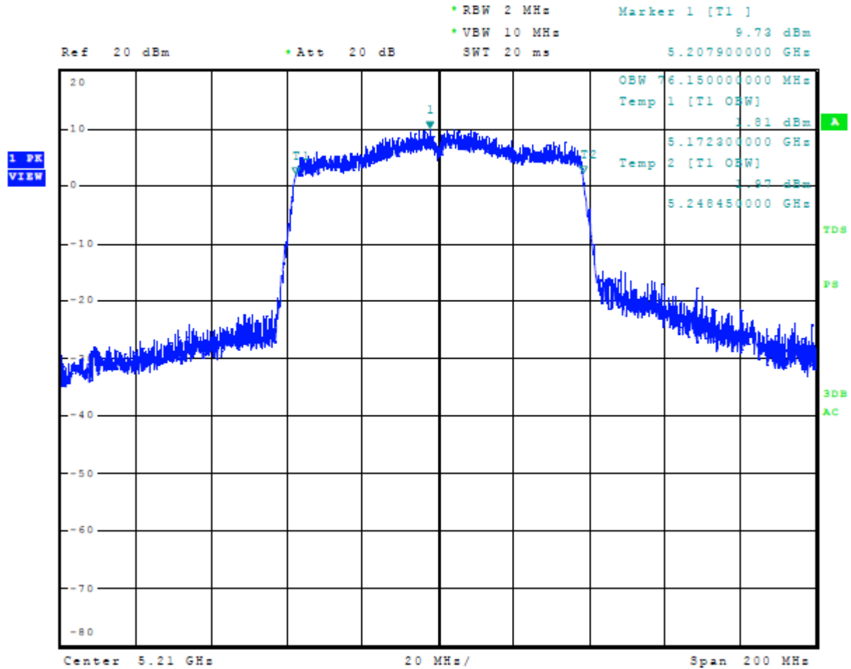
Figure 38 Plot of 99% Occupied Bandwidth 5150-5250 MHz Mode 8 U-NII-1 (802.11ac80)
