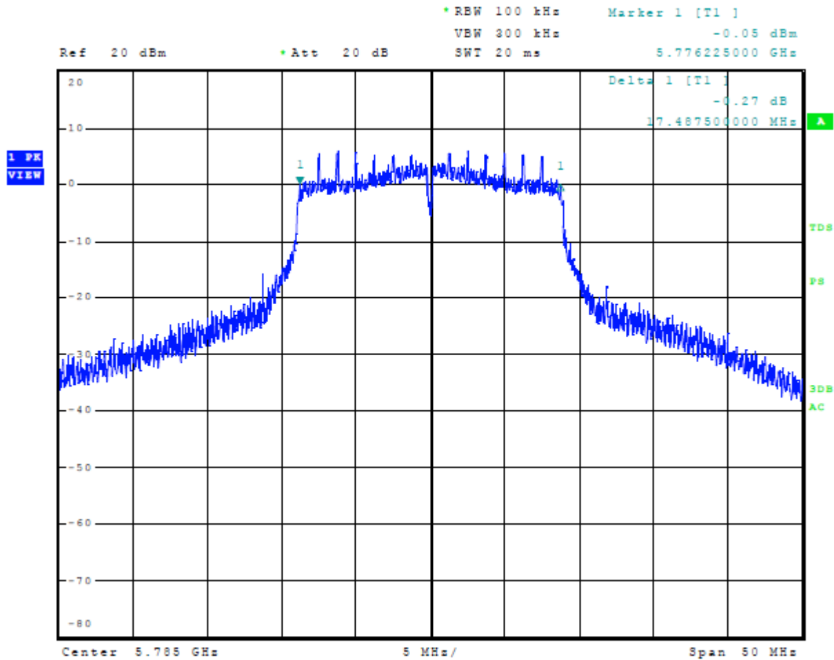
Figure 44 Plot of 6-dB Occupied Bandwidth 5725-5850 MHz Mode 10 U-NII-3 (802.11n)
