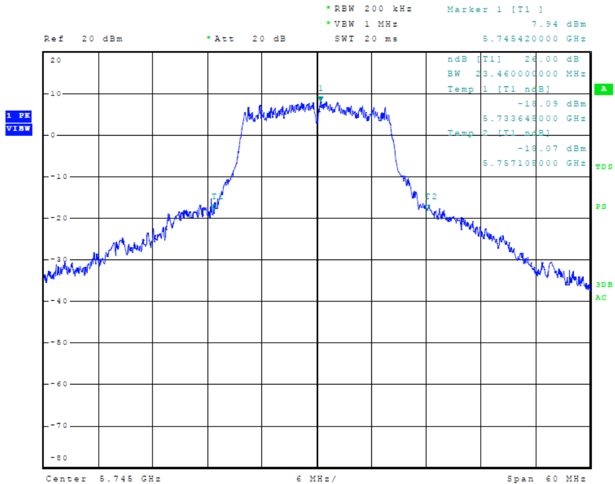
Figure 31 Plot of 26-dB Occupied Bandwidth 5725-5850 MHz Mode 9 U-NII-3 (802.11a)
