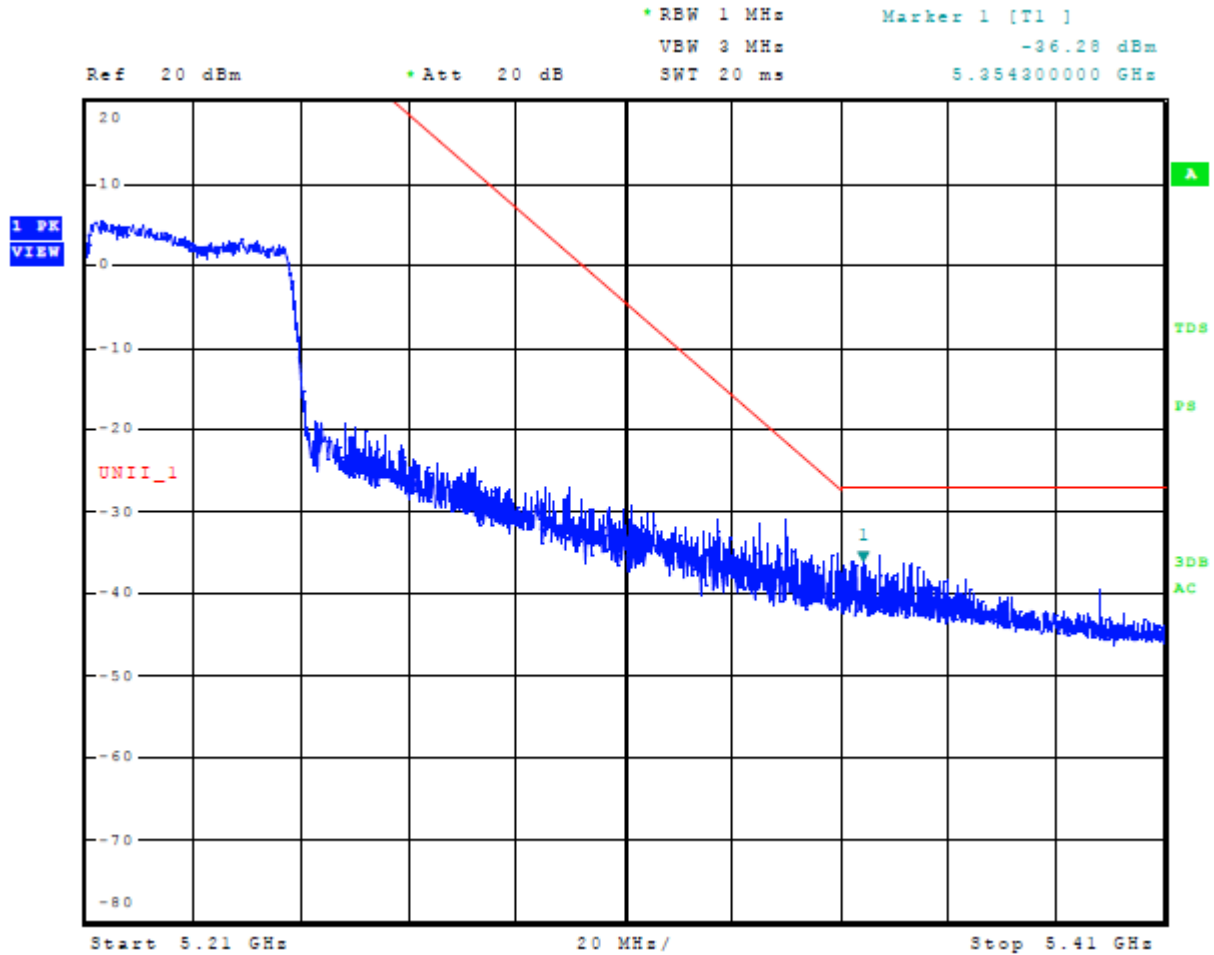
Figure 22 Plot of Upper Band Edge Across 5150-5250 MHz Mode 8 U-NII-1 (802.11ac80)
