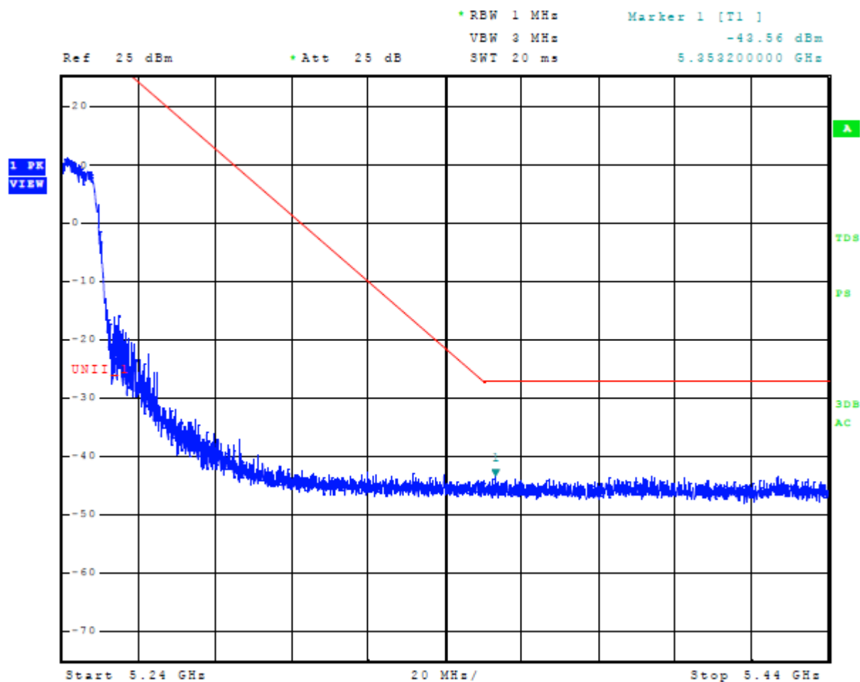
Figure 20 Plot of Upper Band Edge Across 5150-5250 MHz Mode 6 U-NII-1 (802.11n)
