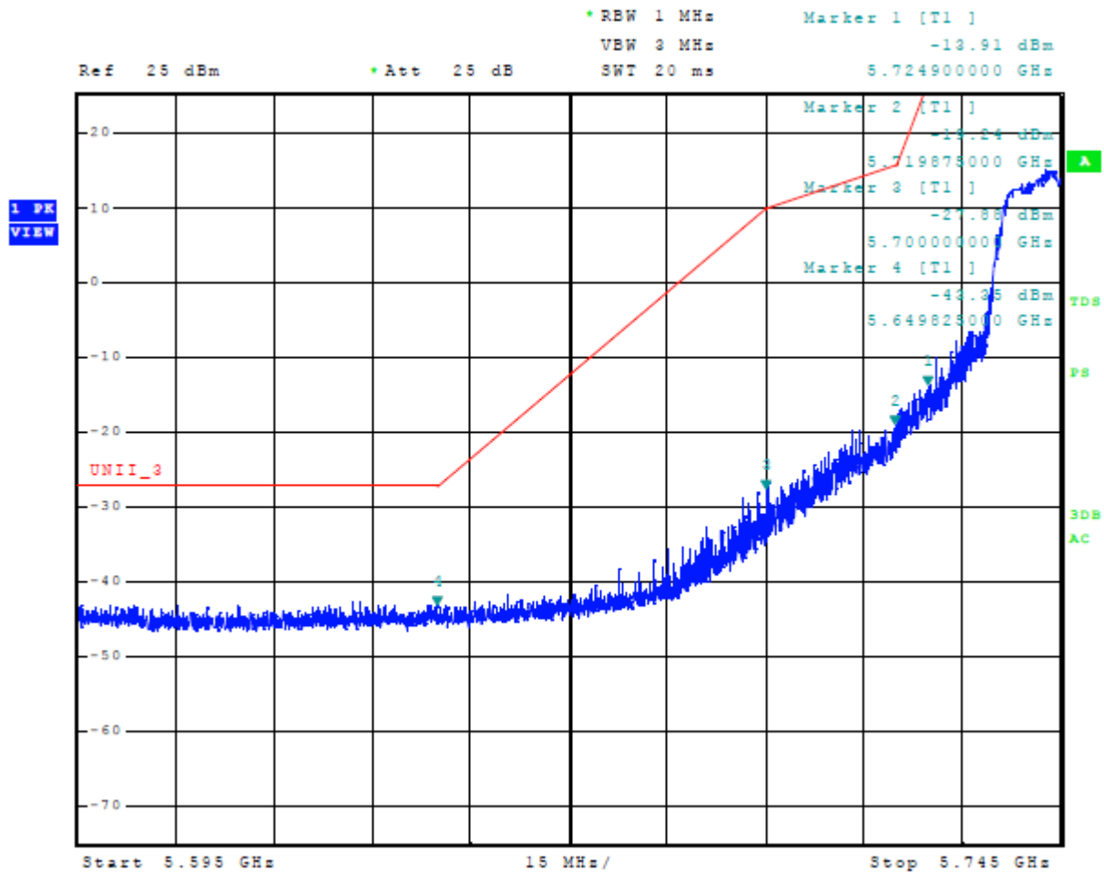
Figure 16 Plot of Lower Band Edge Across 5725-5850 MHz Mode 10 U-NII-3 (802.11n)
