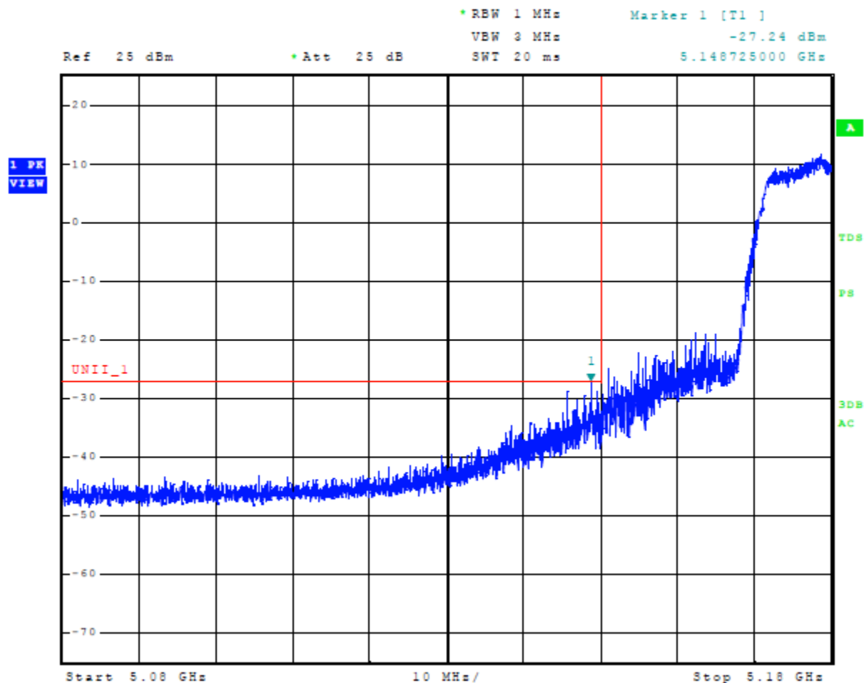
Figure 12 Plot of Lower Band Edge Across 5150-5250 MHz Mode 6 U-NII-1 (802.11n)
