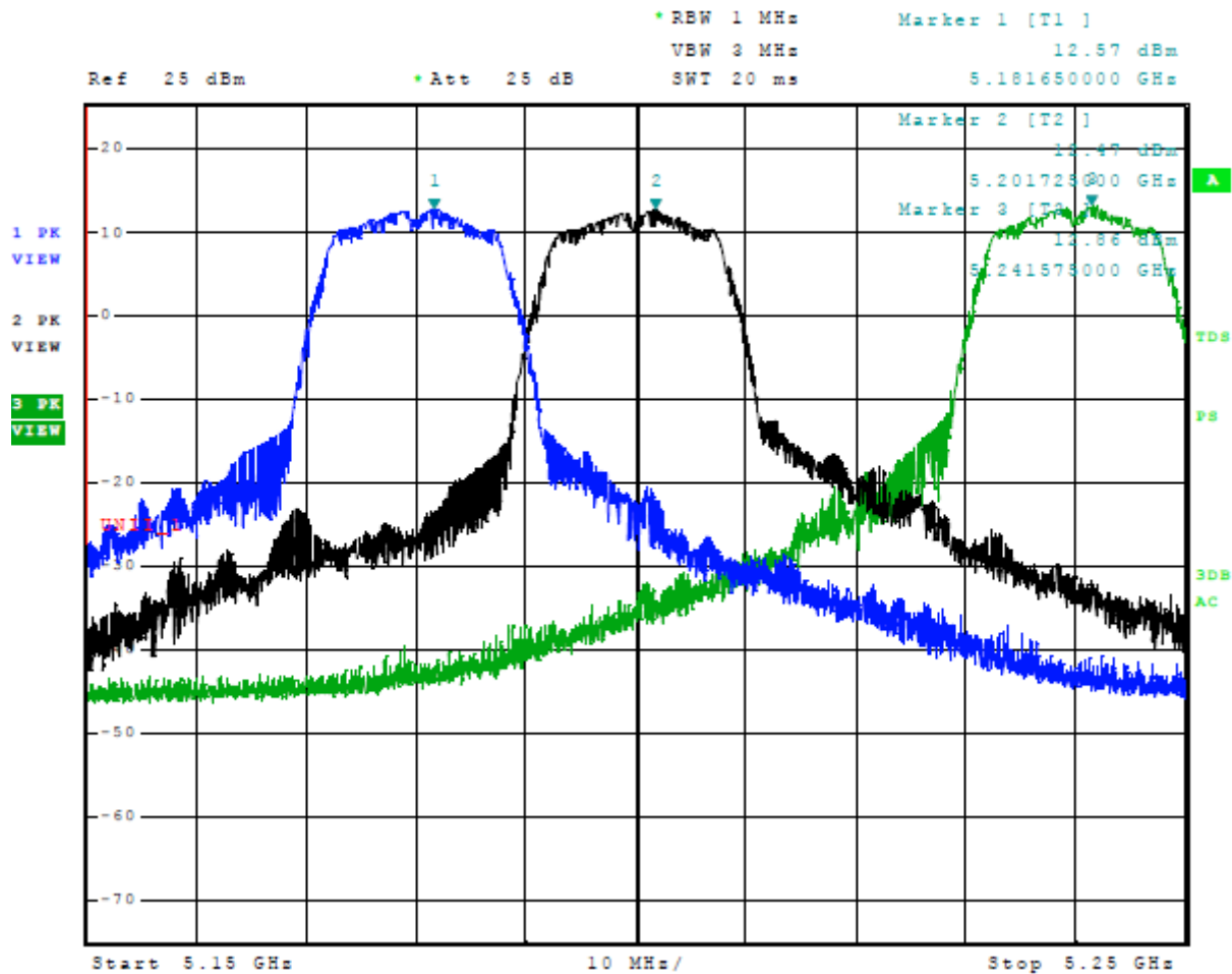
Figure 3 Plot of Transmitter Emissions Across 5150-5250 MHz Mode 5 U-NII-1 (802.11a)
