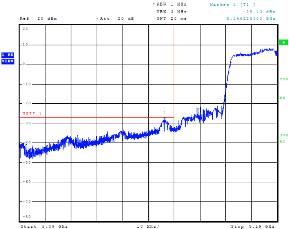
Figure 13 Plot of Lower Band Edge Across 5150-5250 MHz Mode 7 U-NII-1 (802.11n40)
