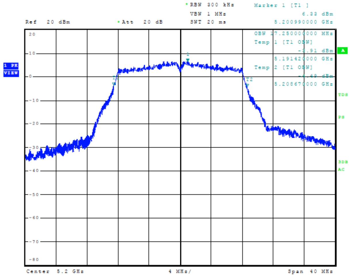
Figure 35 Plot of 99% Occupied Bandwidth 5150-5250 MHz Mode 5 U-NII-1 (802.11a)
