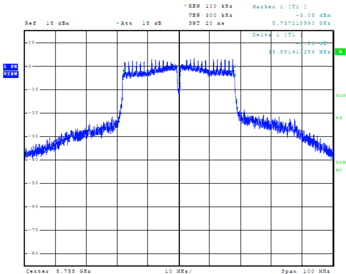
Figure 45 Plot of 6-dB Occupied Bandwidth 5725-5850 MHz Mode 11 U-NII-3 (802.11n40)
