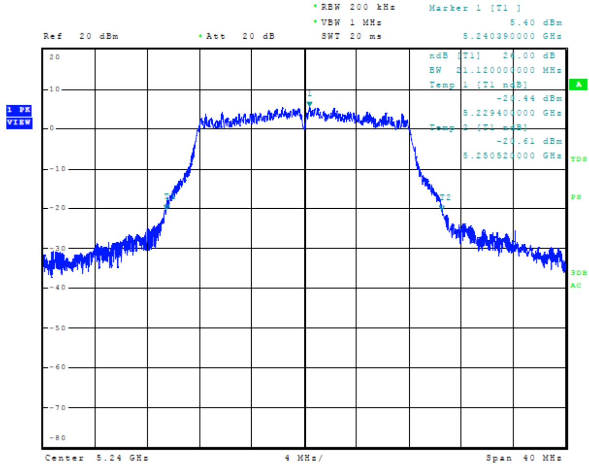
Figure 27 Plot of 26-dB Occupied Bandwidth 5150-5250 MHz Mode 5 U-NII-1 (802.11a)
