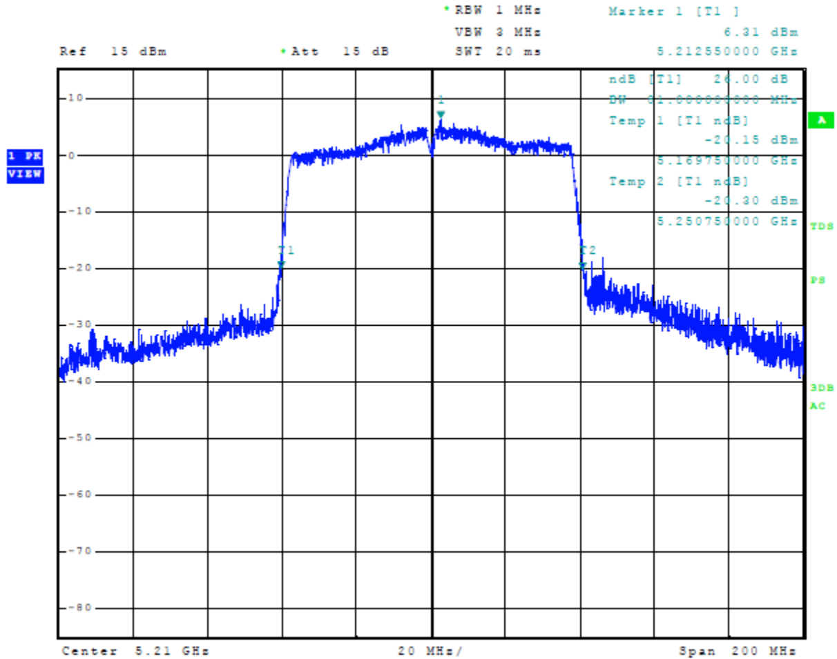
Figure 30 Plot of 26-dB Occupied Bandwidth 5150-5250 MHz Mode 8 U-NII-1 (802.11ac80)
