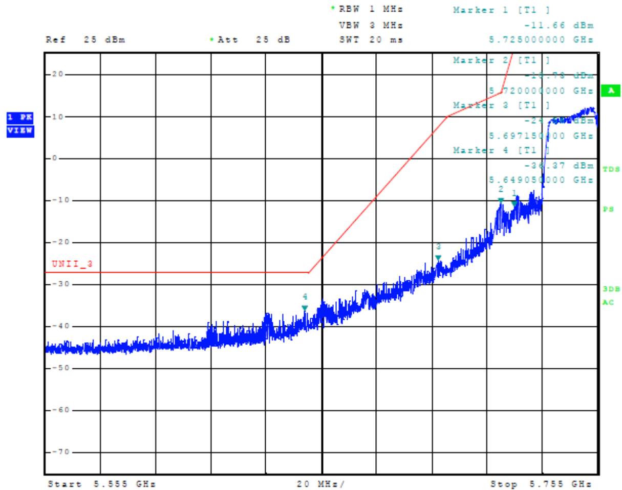
Figure 17 Plot of Lower Band Edge Across 5725-5850 MHz Mode 11 U-NII-3 (802.11n40)
