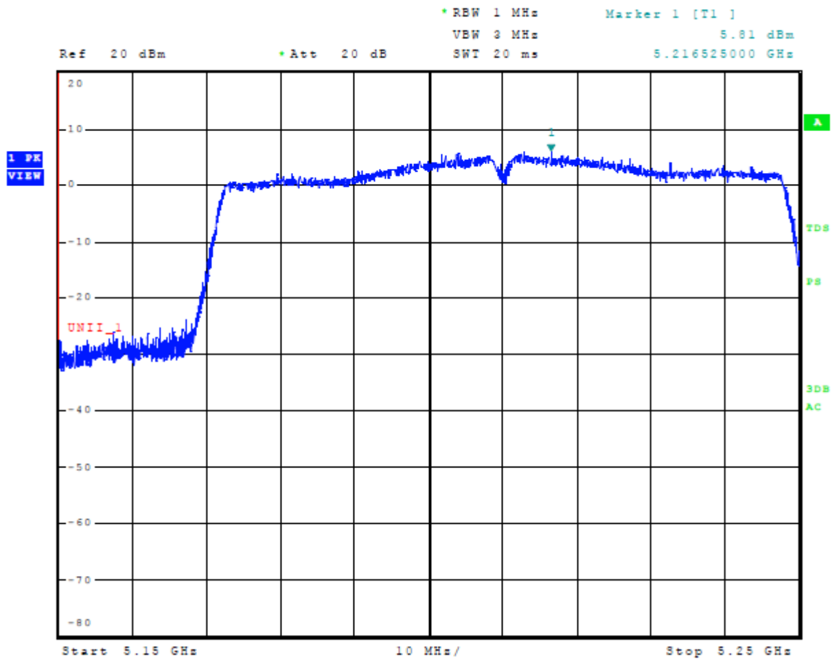
Figure 6 Plot of Transmitter Emissions Across 5150-5250 MHz Mode 8 U-NII-1 (802.11ac80)
