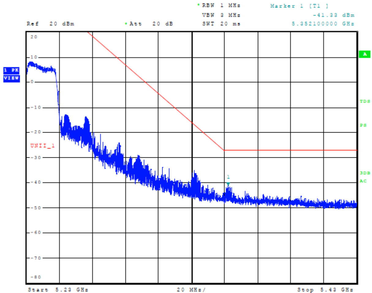
Figure 21 Plot of Upper Band Edge Across 5150-5250 MHz Mode 7 U-NII-1 (802.11n40)
