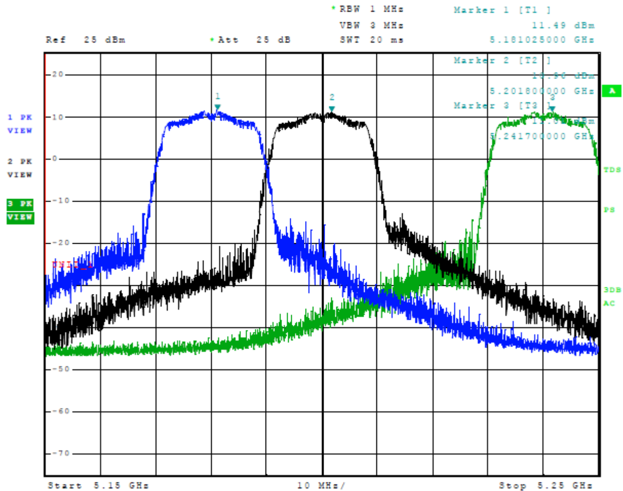
Figure 4 Plot of Transmitter Emissions Across 5150-5250 MHz Mode 6 U-NII-1 (802.11n)
