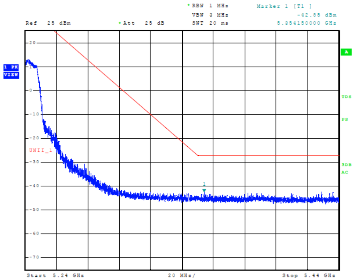
Figure 19 Plot of Upper Band Edge Across 5150-5250 MHz Mode 5 U-NII-1 (802.11a)
