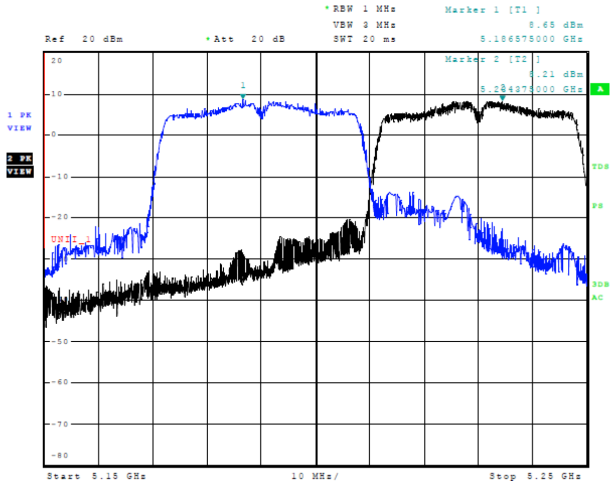
Figure 5 Plot of Transmitter Emissions Across 5150-5250 MHz Mode 7 U-NII-1 (802.11n40)
