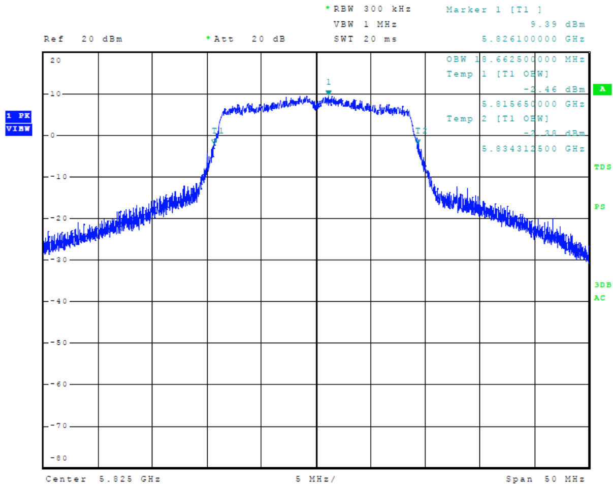
Figure 40 Plot of 99% Occupied Bandwidth 5725-5850 MHz Mode 10 U-NII-3 (802.11n)
