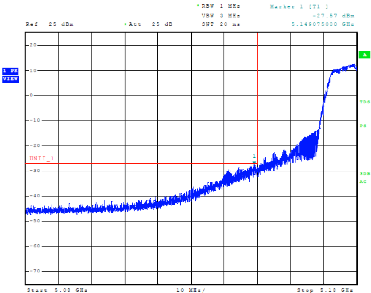
Figure 11 Plot of Lower Band Edge Across 5150-5250 MHz Mode 5 U-NII-1 (802.11a)
