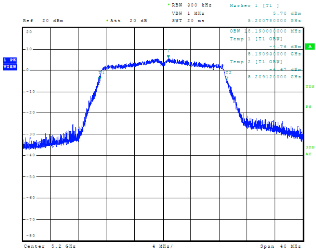
Figure 36 Plot of 99% Occupied Bandwidth 5150-5250 MHz Mode 6 U-NII-1 (802.11n)
