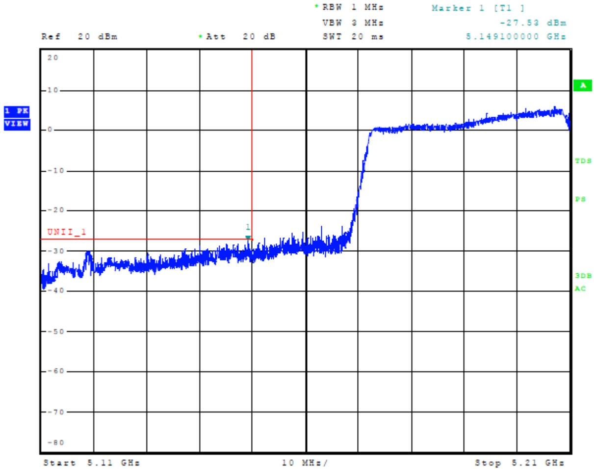
Figure 14 Plot of Lower Band Edge Across 5150-5250 MHz Mode 8 U-NII-1 (802.11ac80)
