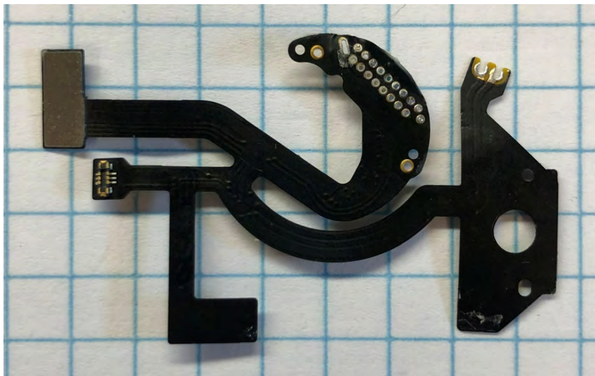
Back PCBA#2
