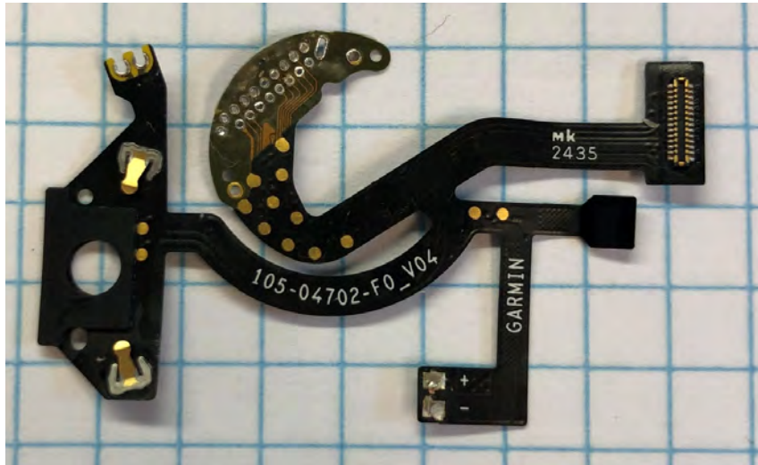
Front PCBA#2
