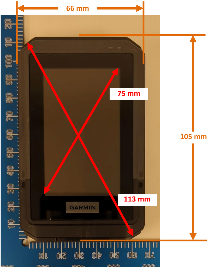
Photograph 1: Overall Dimensions
