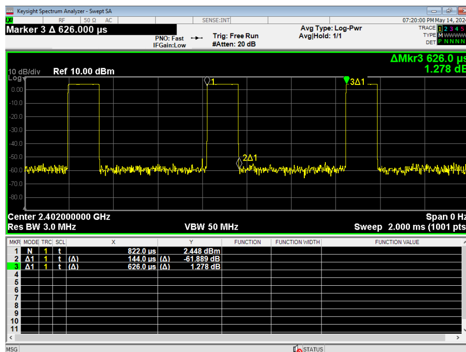
Figure 5 – Duty Cycle, GMSK 2MB, Measured
