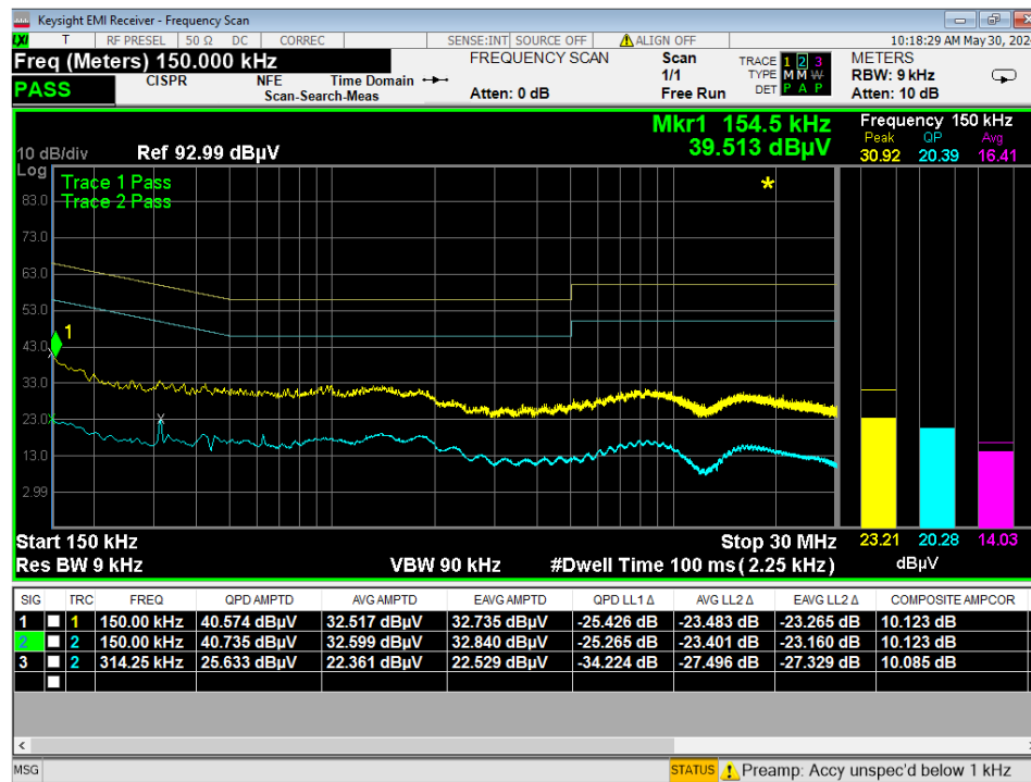
Figure 17 - Conducted Emissions Plot, Line, IDLE, 120VAC 60Hz
