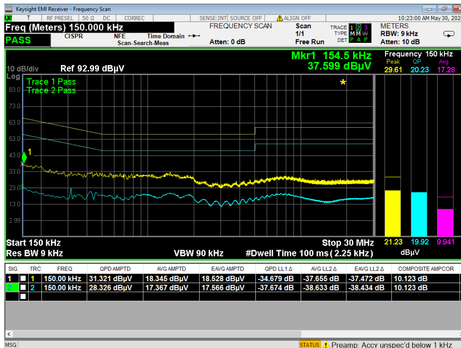
Figure 16 - Conducted Emissions Plot, Neutral, TX, 120VAC 60Hz
