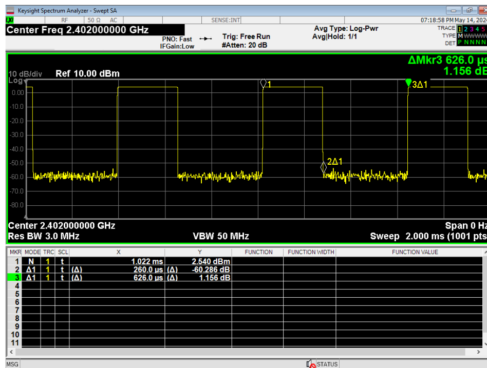
Figure 4 – Duty Cycle, GMSK 1MB, Measured
