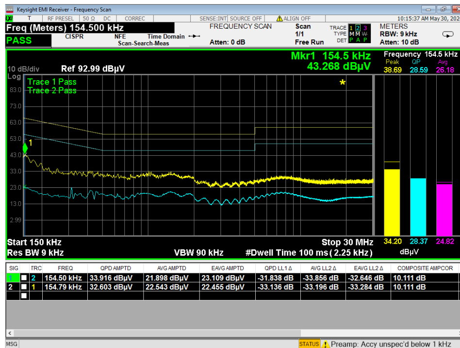
Figure 18 - Conducted Emissions Plot, Neutral, IDLE, 120VAC 60Hz
