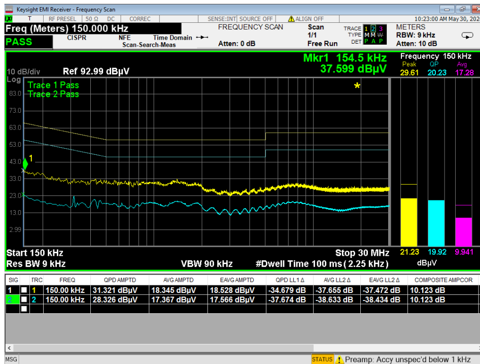
Figure 7 - Conducted Emissions Plot, Neutral, TX, 120VAC/60Hz
