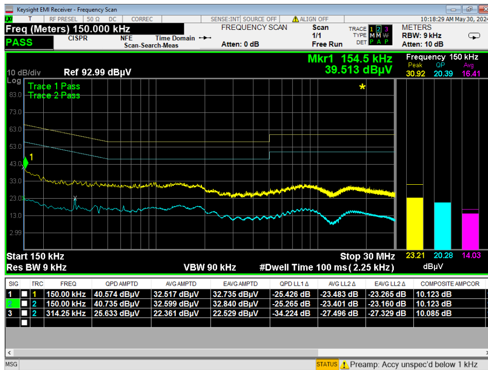
Figure 8 - Conducted Emissions Plot, Line, IDLE, 120VAC/60Hz
