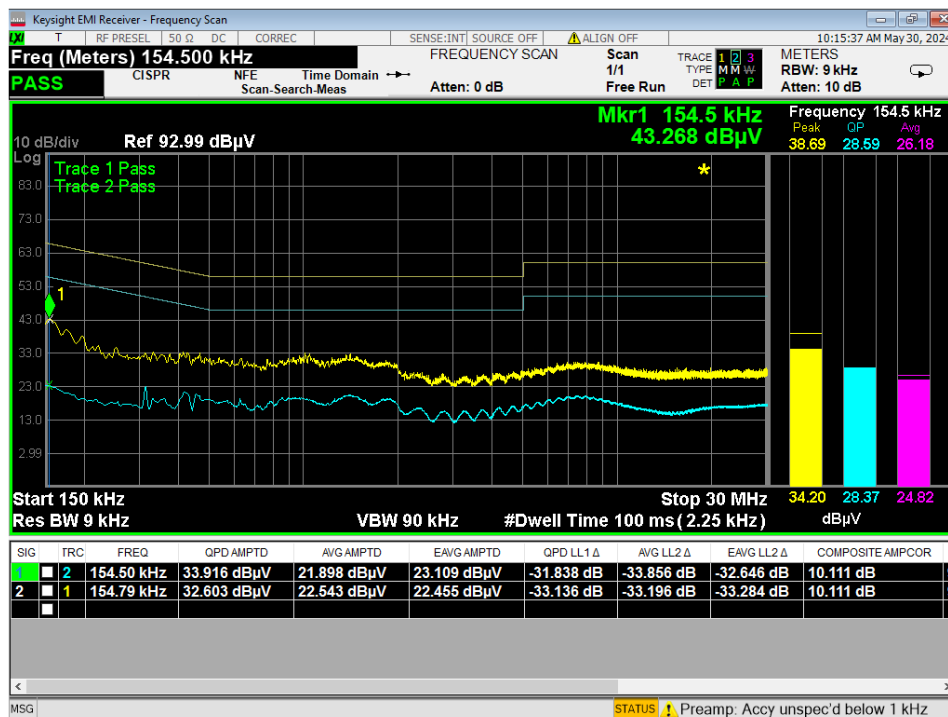
Figure 9 - Conducted Emissions Plot, Neutral, IDLE, 120VAC/60Hz
