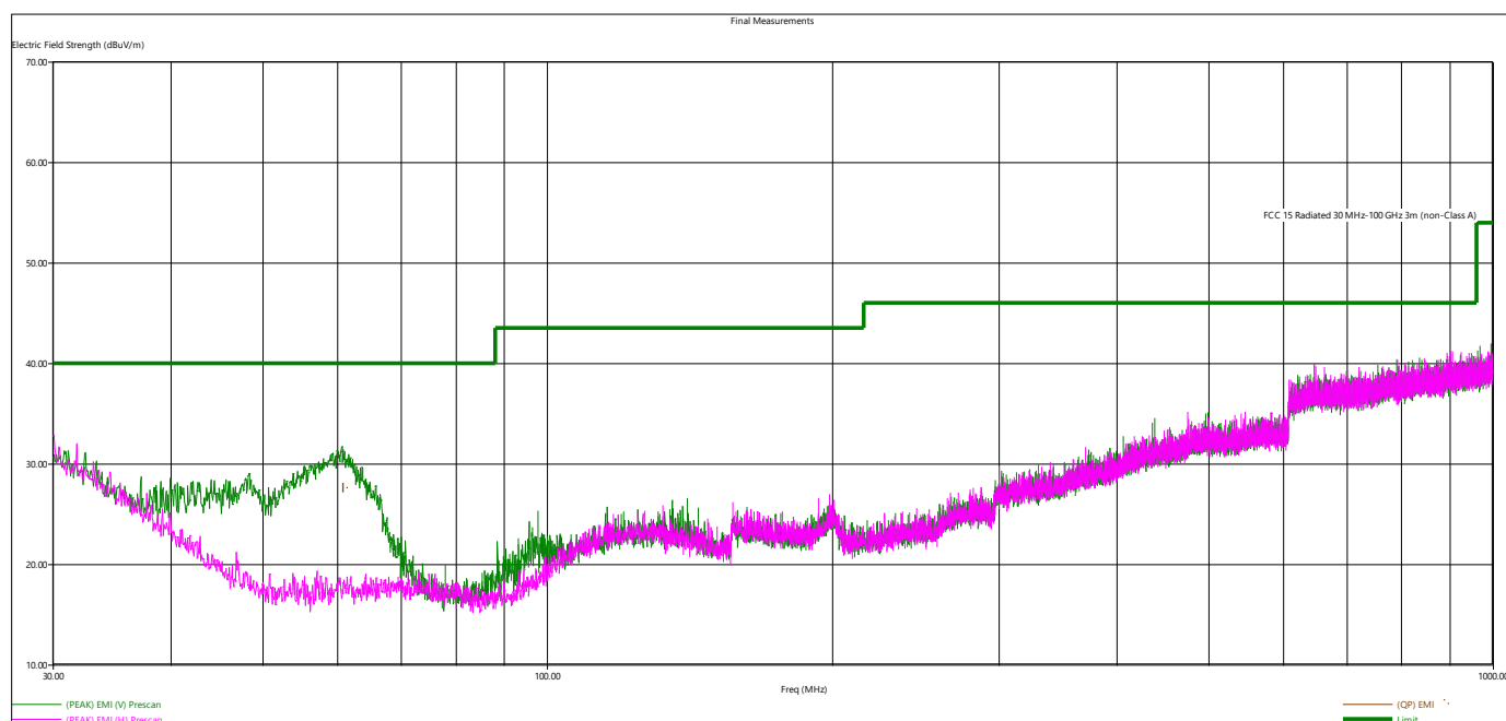
Figure 5 - Radiated Emissions Plot, GFSK, Low Channel
