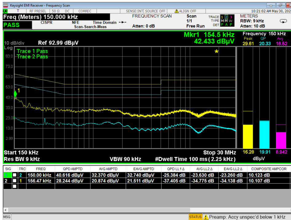
Figure 6 - Conducted Emissions Plot, Line, TX, 120VAC/60Hz
