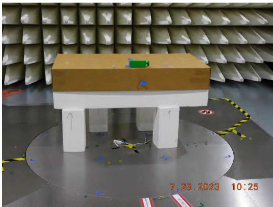
Figure RE04.6: EUT test setup, front view (Y Orientation)
