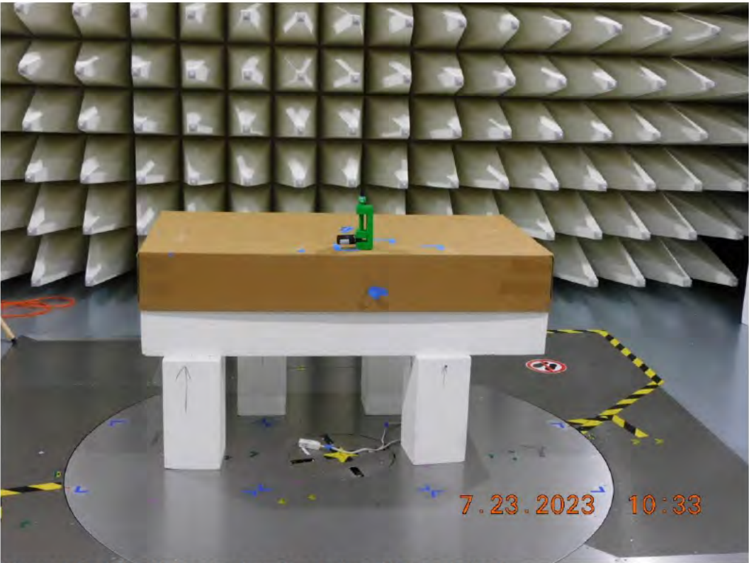
Figure RE04.4: EUT test setup, front view (X Orientation)
