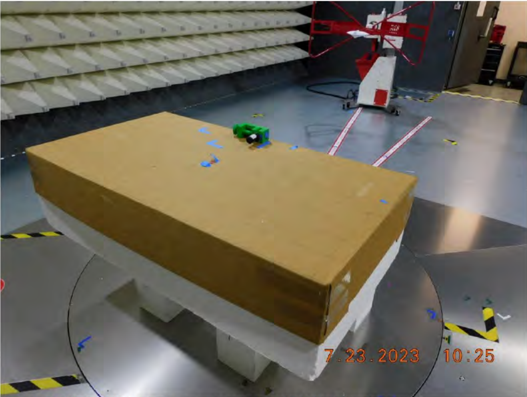
Figure RE03.3: EUT test setup, reverse view (Y Orientation).
