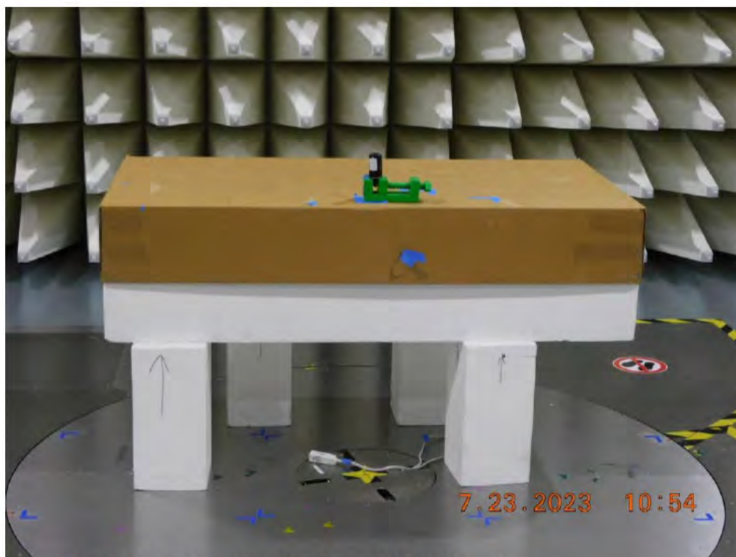
Figure RE03.4: EUT test setup, front view (Z Orientation).
