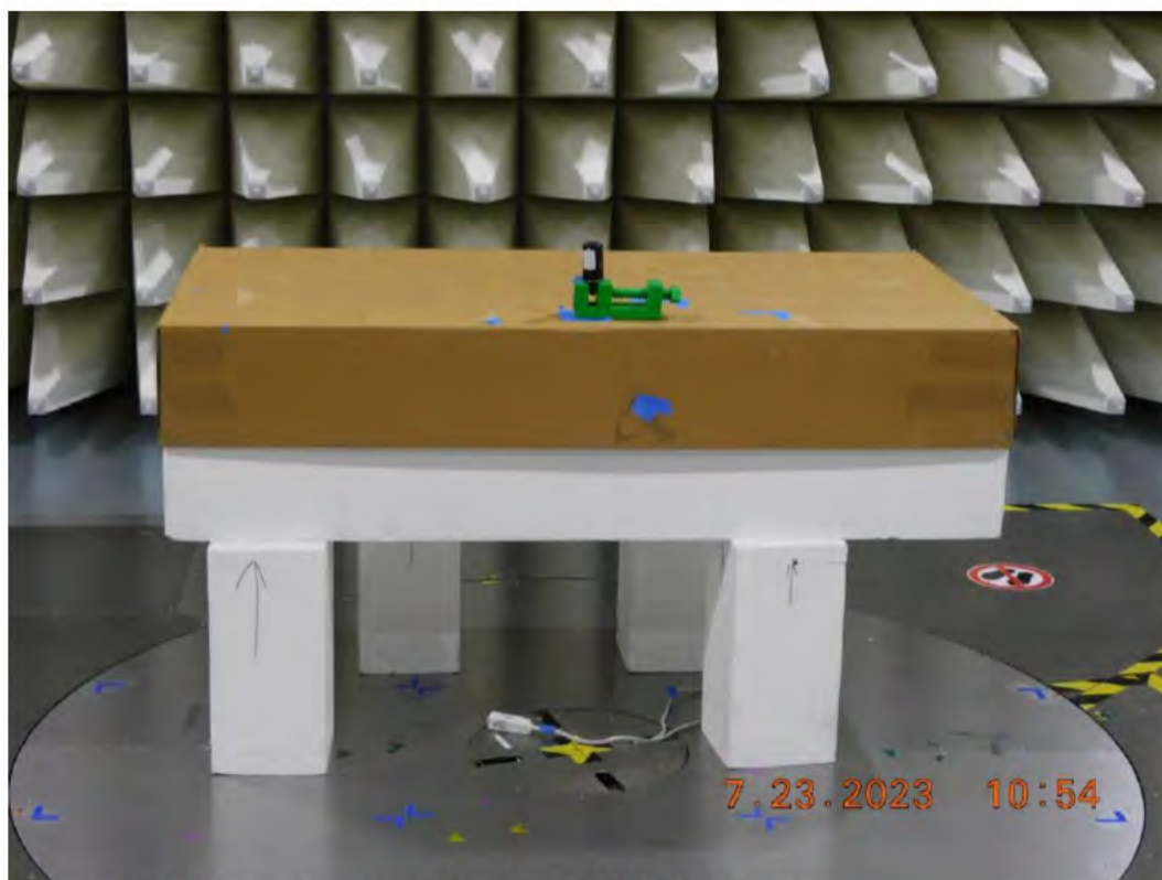
Figure RE04.8: EUT test setup, front view (Z Orientation)
