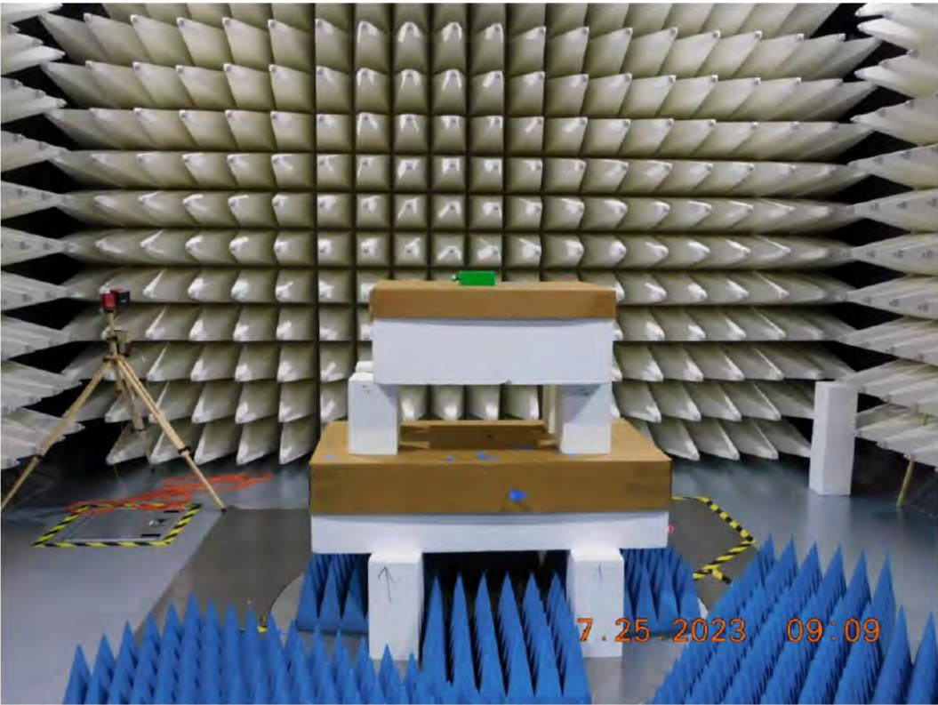
Figure RE02.3: EUT test setup, Front View (Y Orientation)
