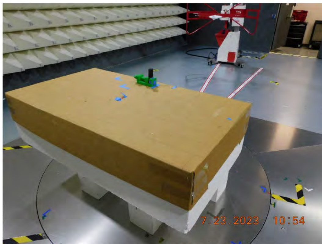
Figure RE03.5: EUT test setup, reverse view (Z Orientation).
