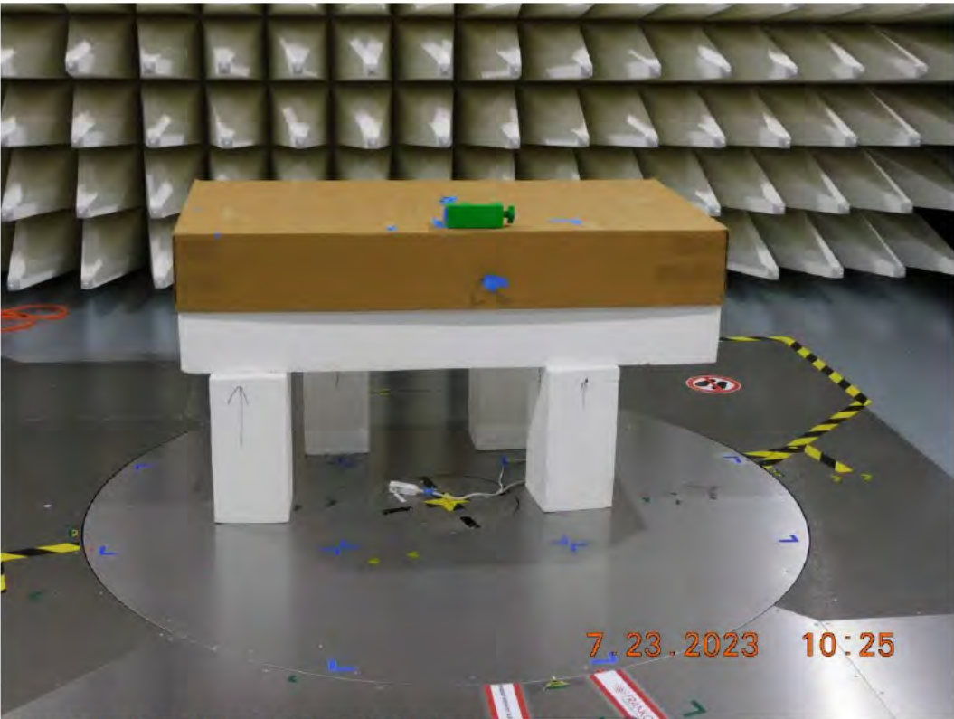
Figure RE03.2: EUT test setup, front view (Y Orientation).
