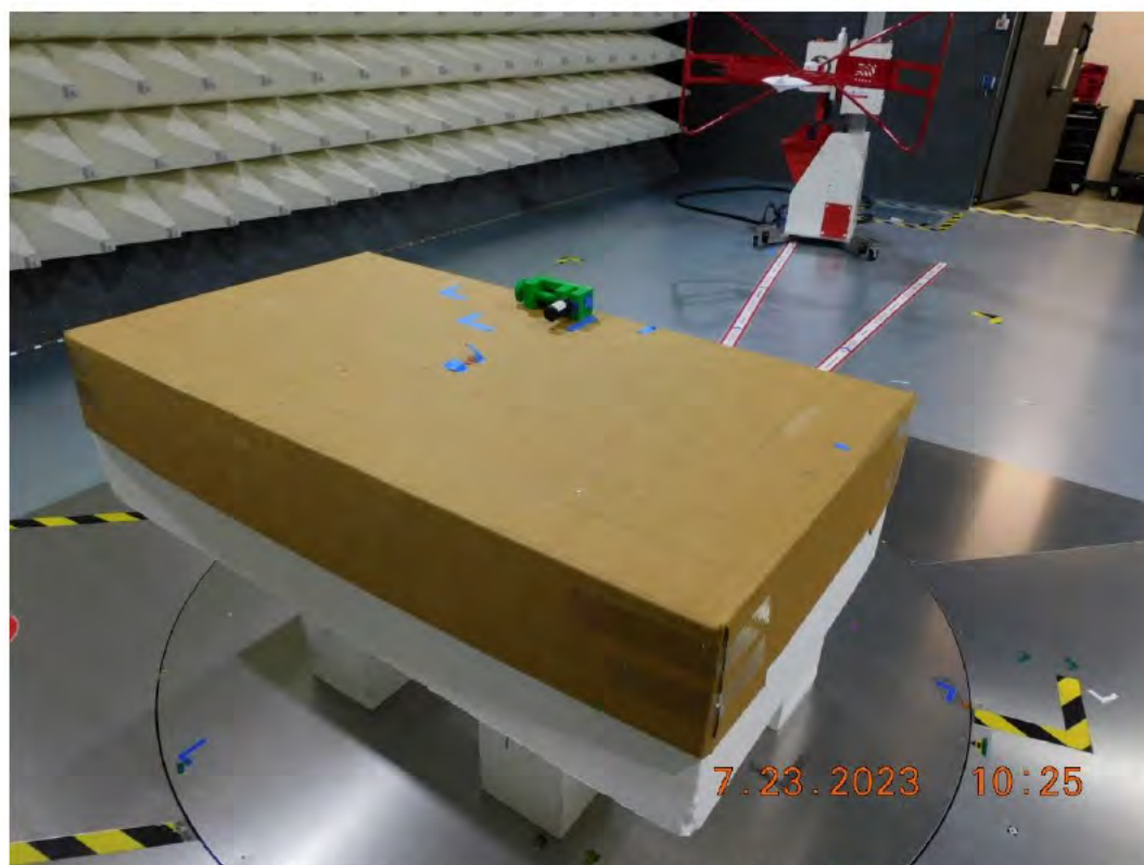
Figure RE04.7: EUT test setup, reverse view (Y Orientation)
