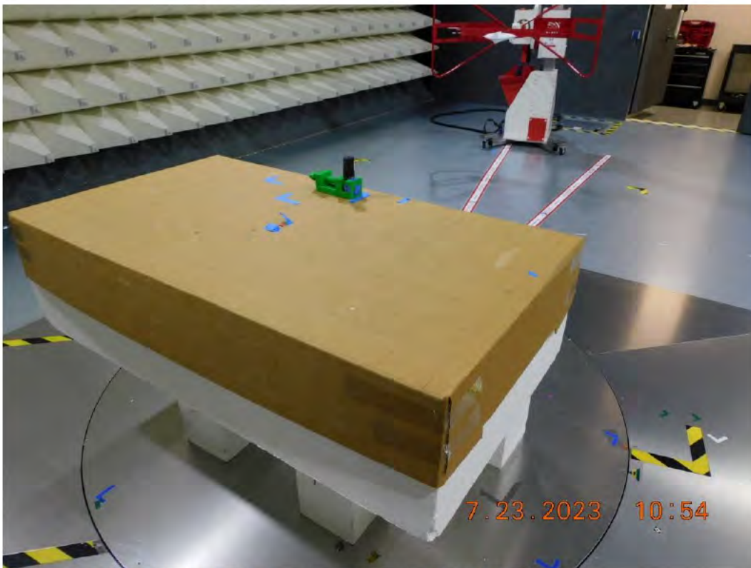
Figure RE07.9: EUT test setup, reverse view (Z Orientation)
