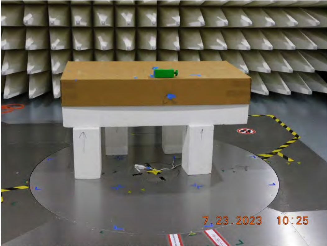
Figure RE07.6: EUT test setup, front view (Y Orientation)
