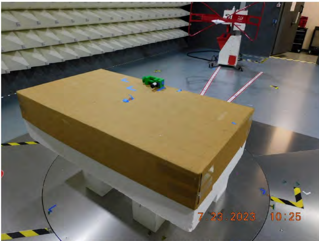
Figure RE07.7: EUT test setup, reverse view (Y Orientation)
