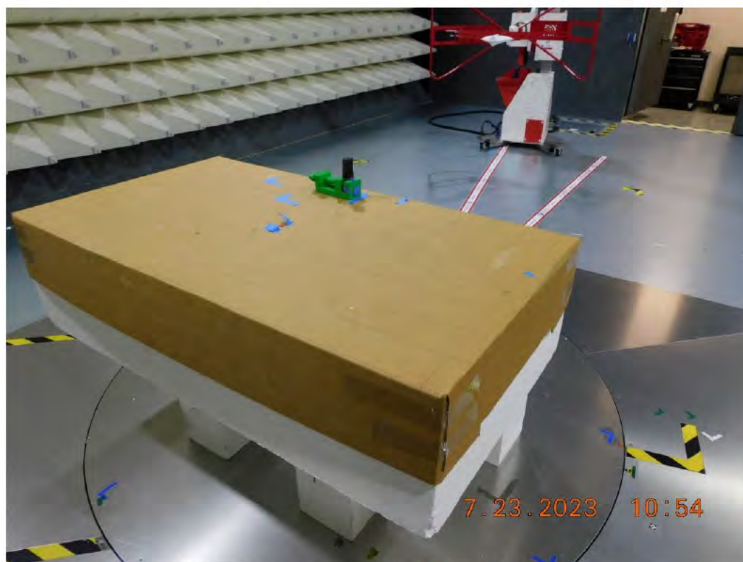
Figure RE04.9: EUT test setup, reverse view (Z Orientation)
