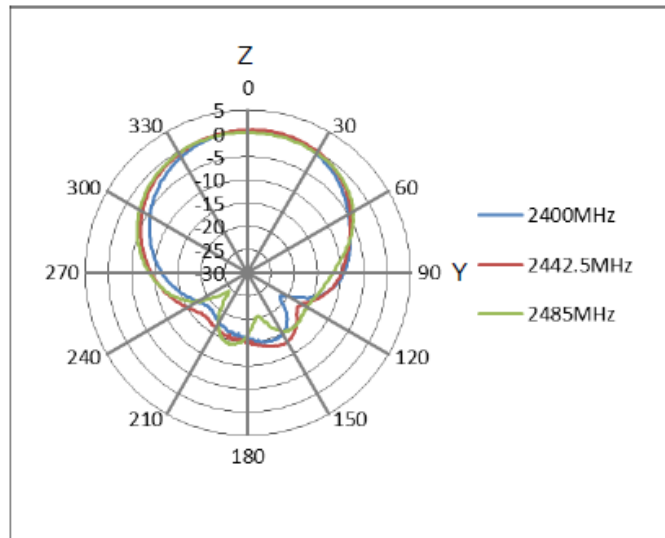
Bluetooth (2400~2485MHz)
