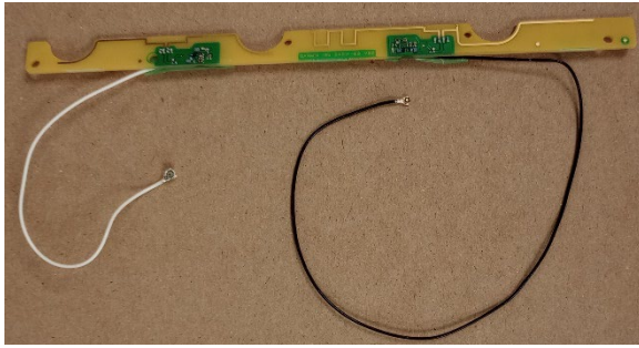
A04797 GNSS Antenna PCB Front
