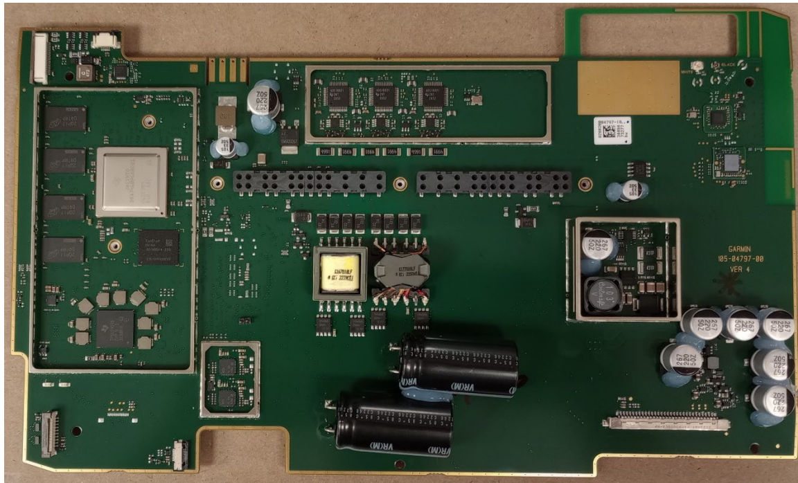
B04797 Main PCB Front Without Shields
