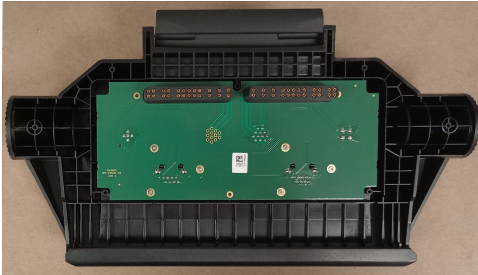
04797 Cradle Interior with PCB Installed (Cradle used with both A04797 & B04797)
