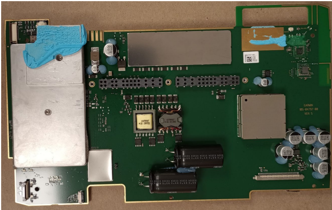
B04797 Main PCB Front With Shields
