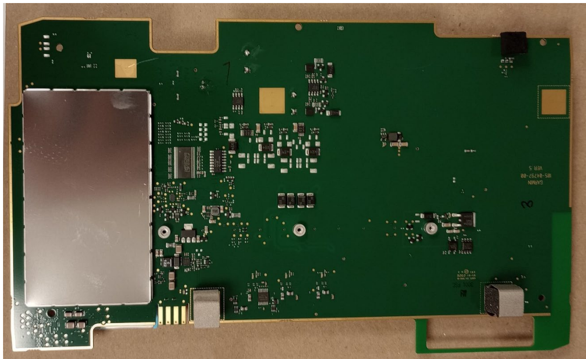
A04797 Main PCB Back With Shields
