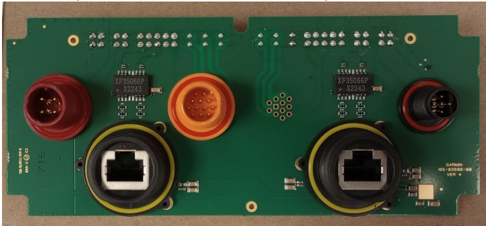
04797 Cradle PCB Front (Cradle used with both A04797 & B04797)
