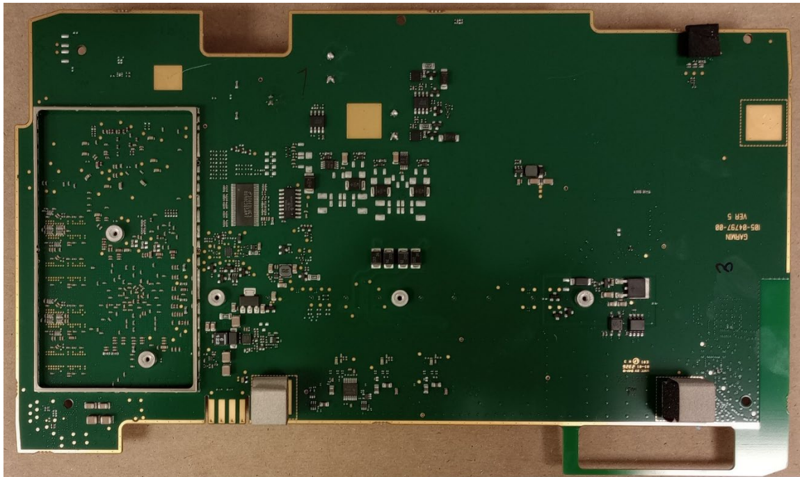
B04797 Main PCB Back Without Shields
