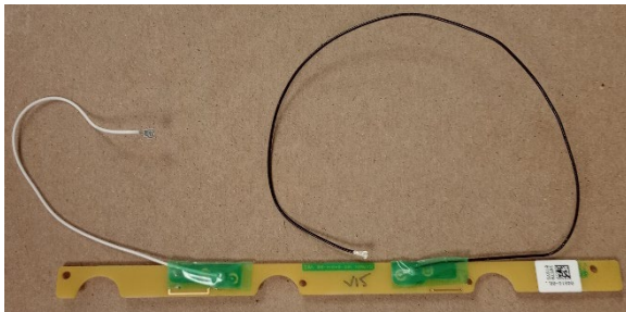
B04797 GNSS Antenna PCB Back
