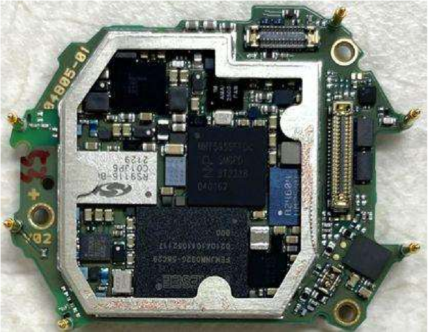
Figure E14.4 – Internal – DUT, Main PCB, Shield Removed
