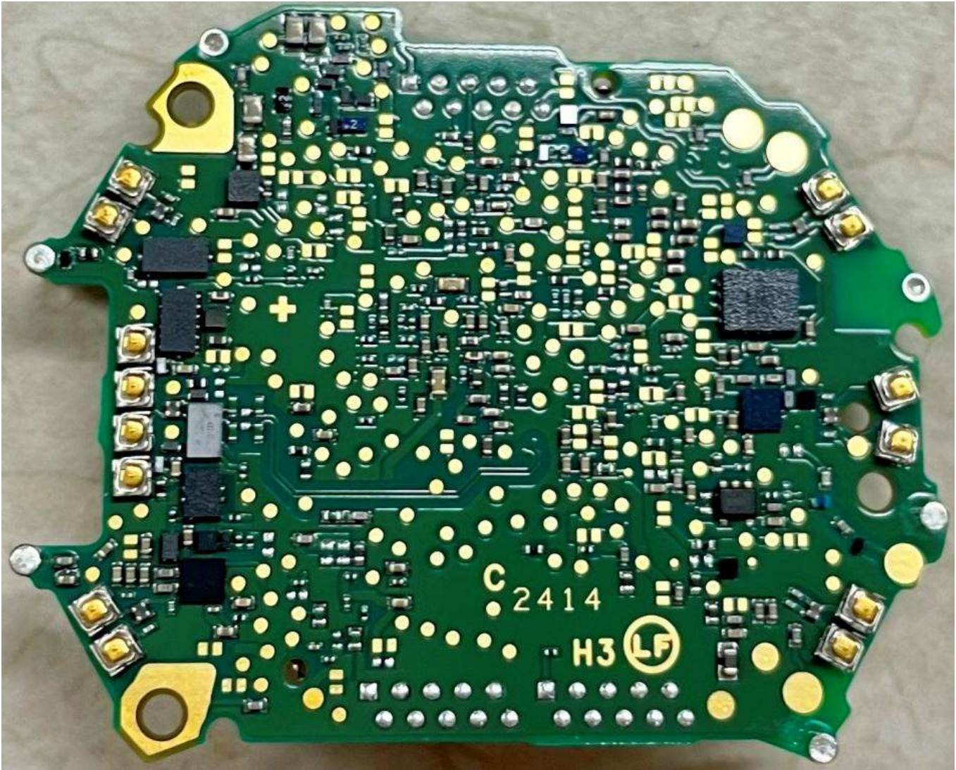
Figure E14.5 – Internal – DUT, Main PCB, Bottom Side
