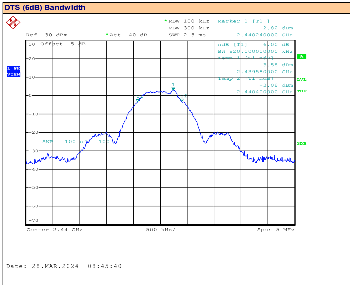
Plot 8.4 – 6dB DTS Bandwidth BLE1
