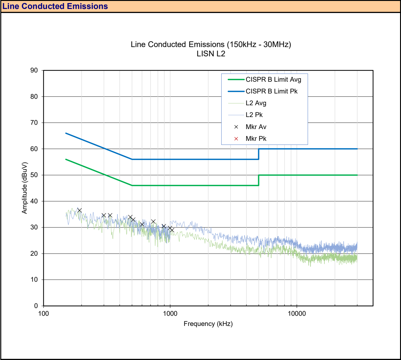
Plot 19.2 – Power Line Conducted Emissions, Line 2
