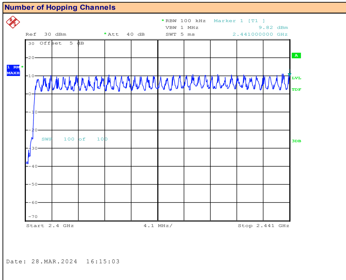
Plot 12.3 – Number of Hopping Channels, BT 2EDR
