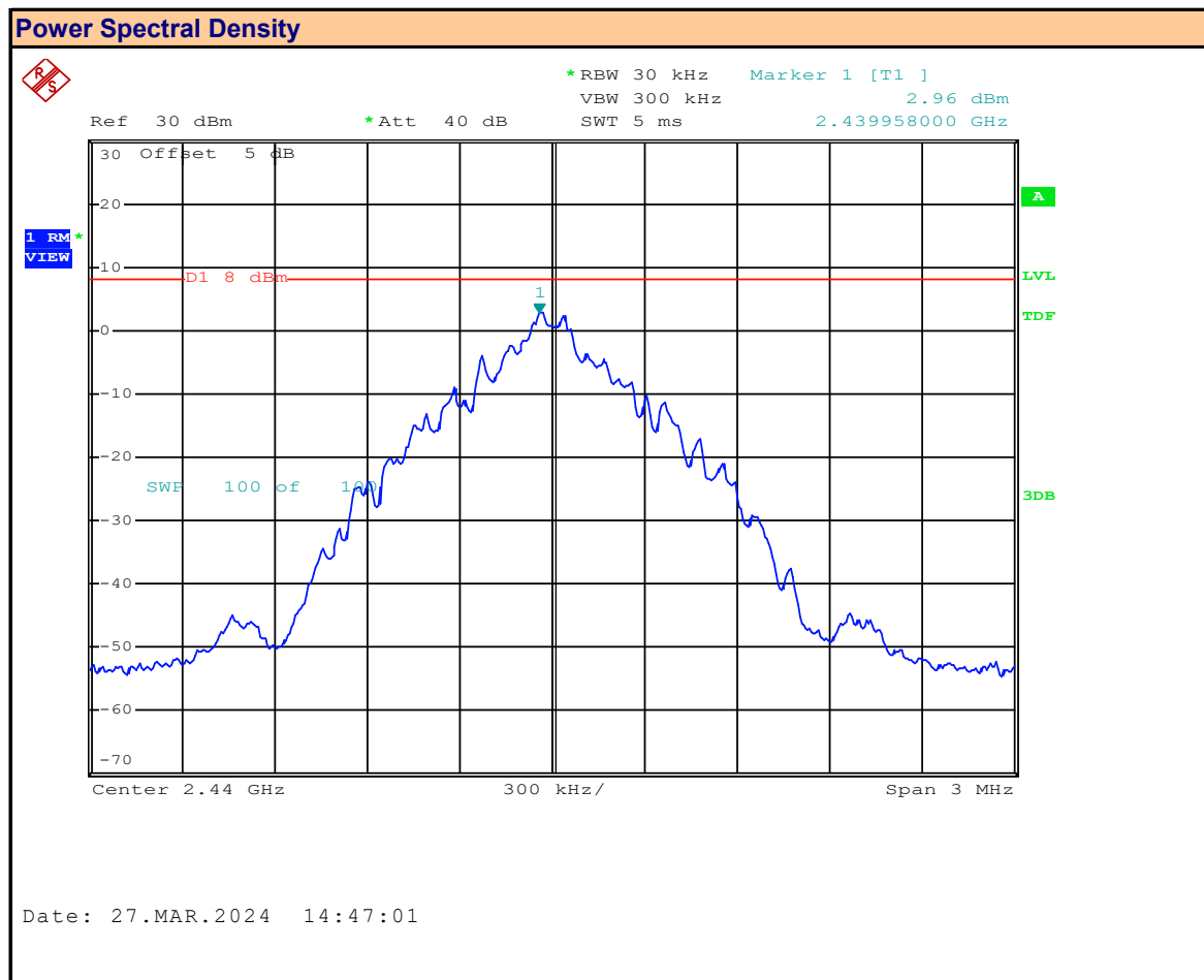
Plot 11.7 – Power Spectral Density, BT BR
