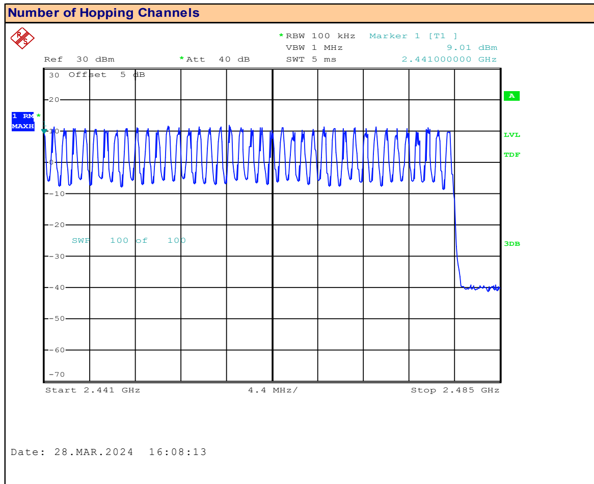
Plot 12.2 – Number of Hopping Channels, BT BR
