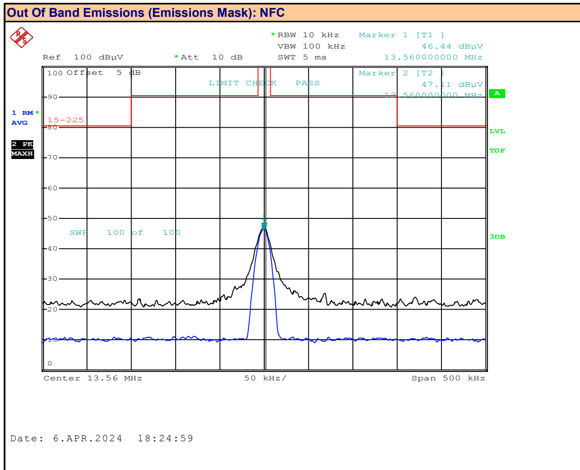
Plot 8.4 – Emissions Mask, NFC, Side
