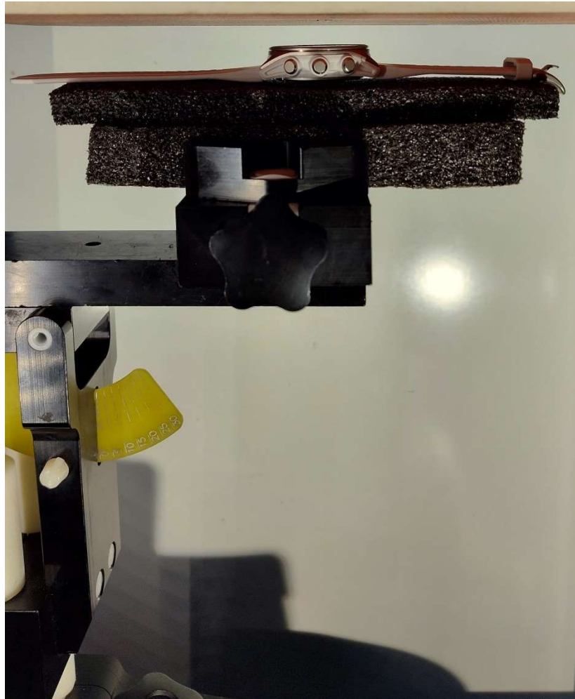
Figure E15.14 – Photo – Setup: Face, DUT Front 10mm – Silicone Band (F23)
