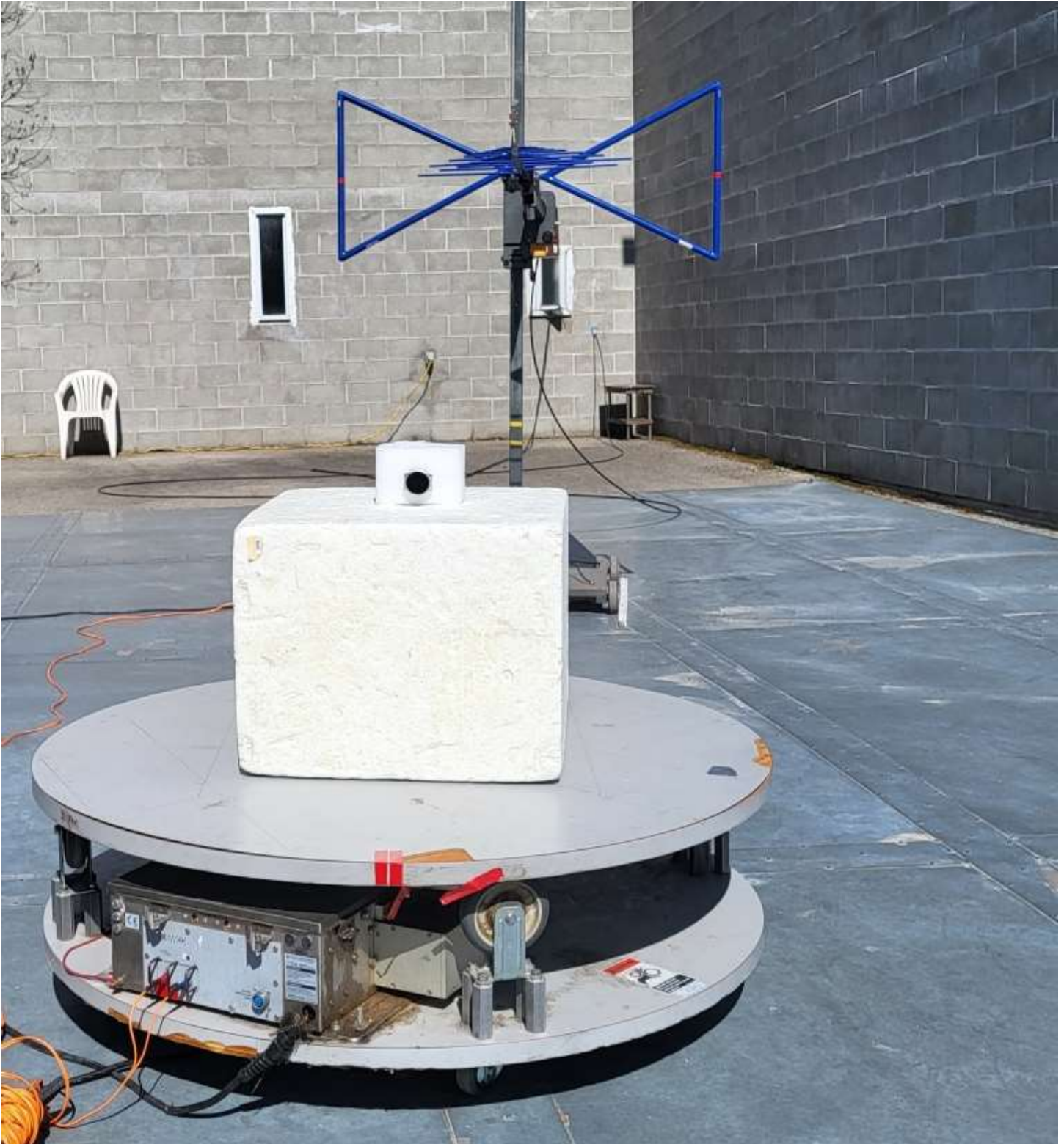
Figure E15.3 – Setup, Radiated Measurements 30 – 1000MHz
