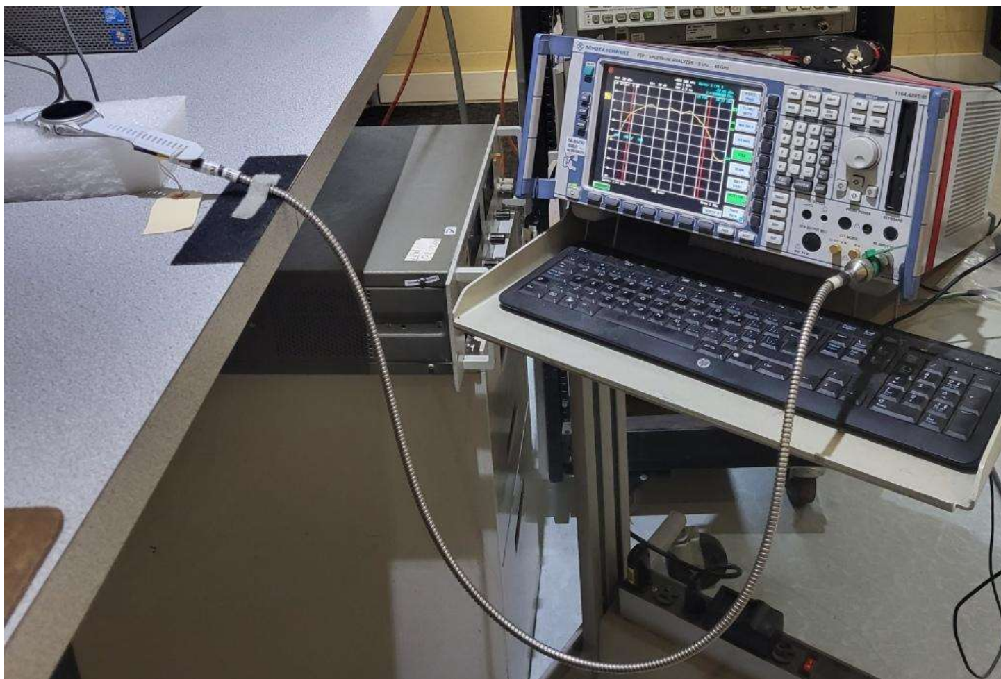
Figure E15.1 – Setup, Antenna Port Conducted Measurements
