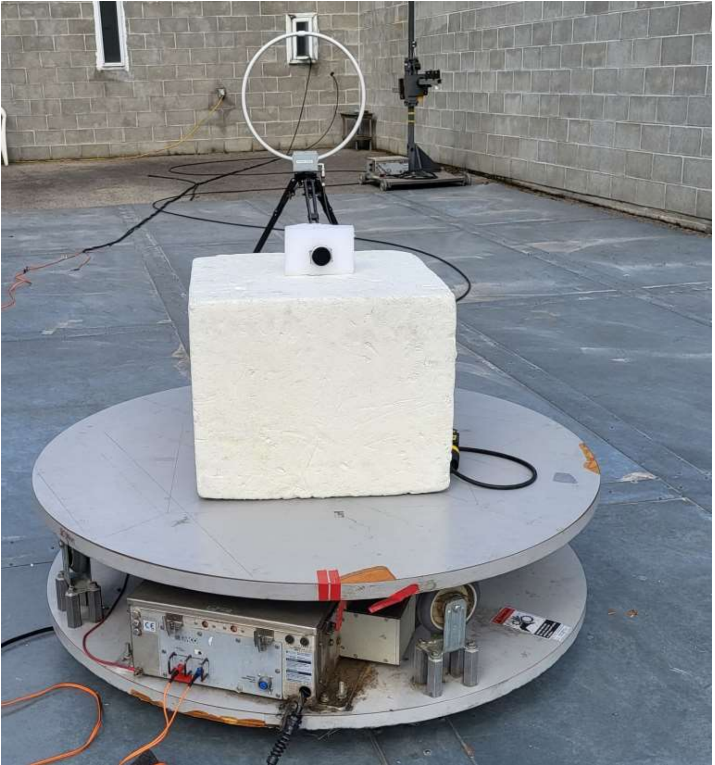
Figure E15.2 – Setup, Radiated Measurements Below 30MHz
