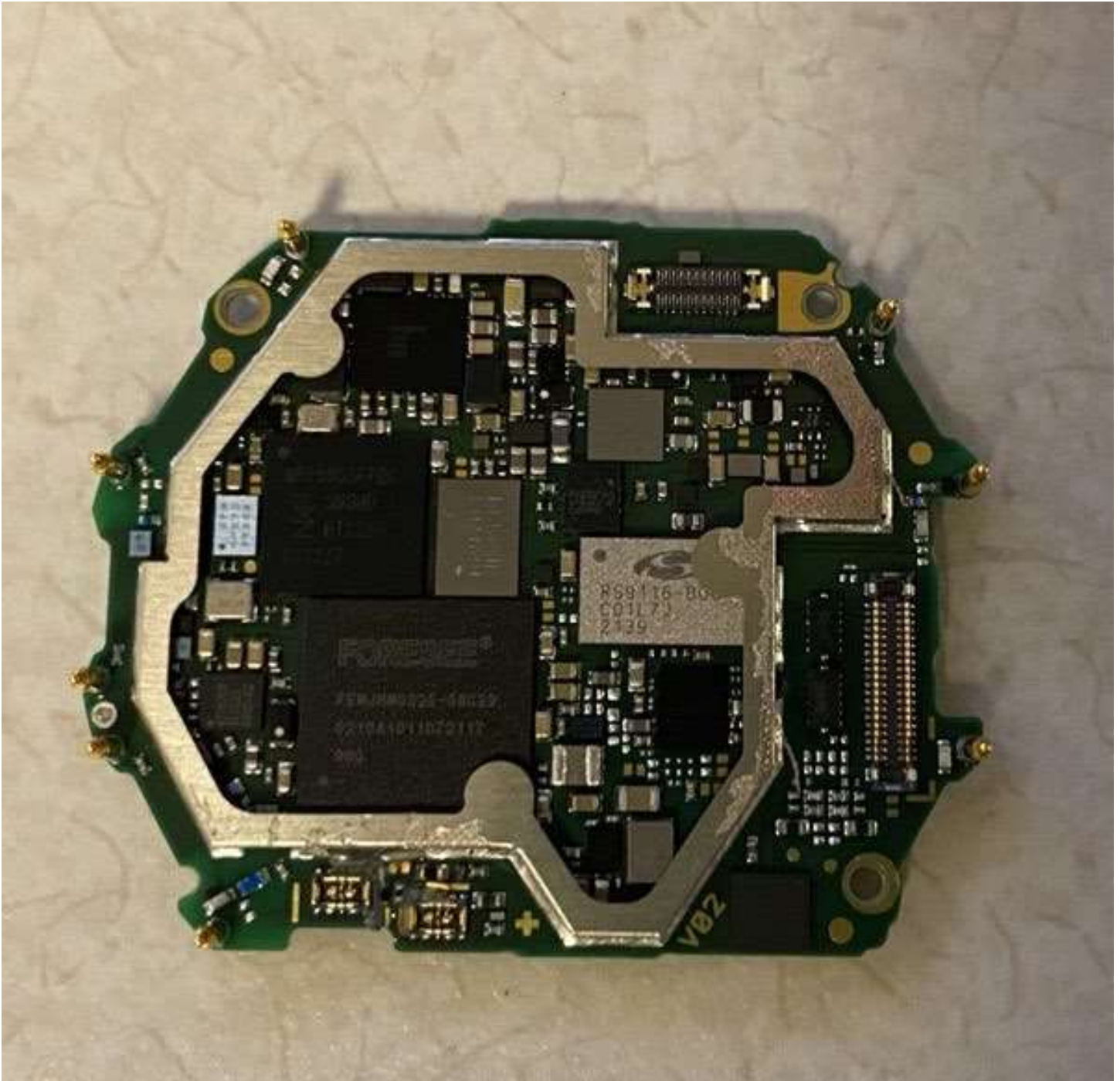
Figure E14.4 – Internal – DUT, Main PCB, Shield Removed
